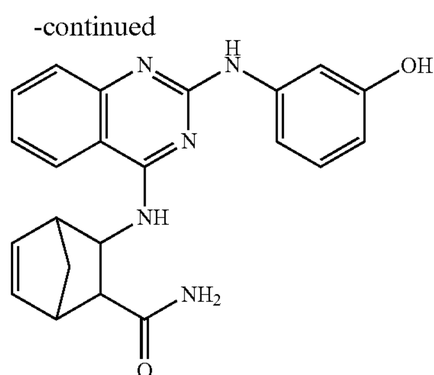
102 (racemic, 2-exo-3-exo)
