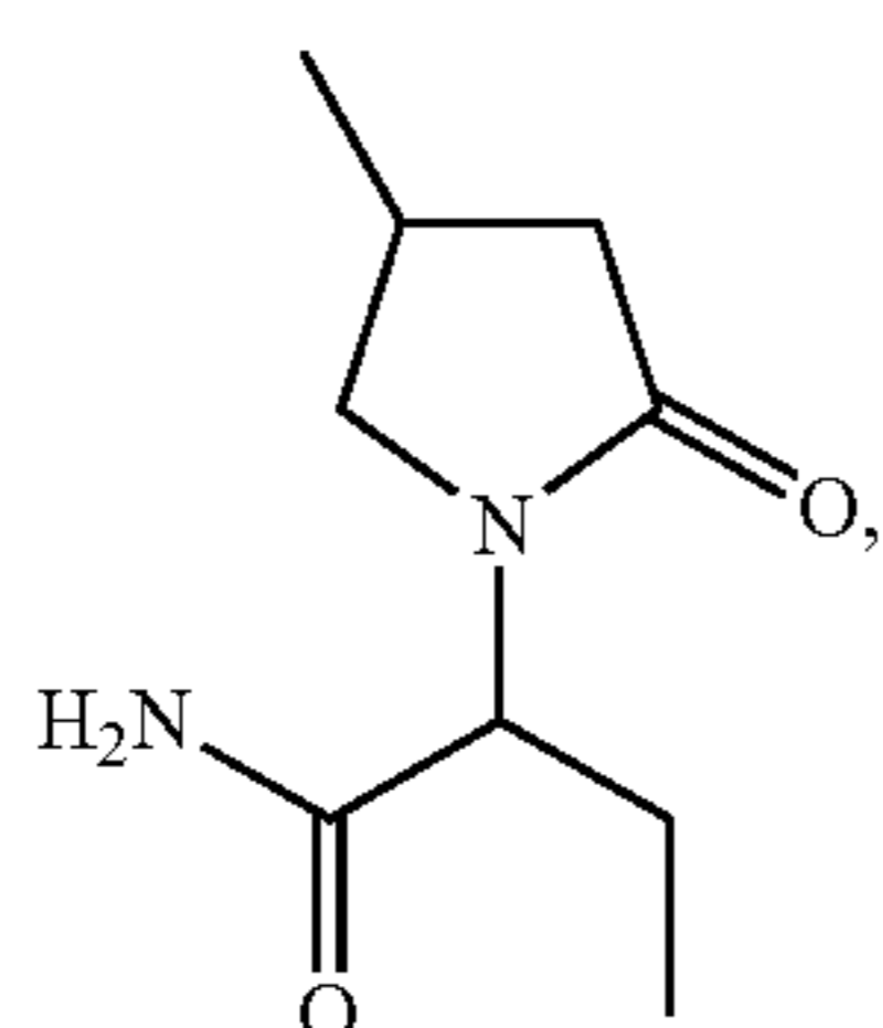
2-(4-methyl-2-oxo-pyrrolidino)-butylamide;
