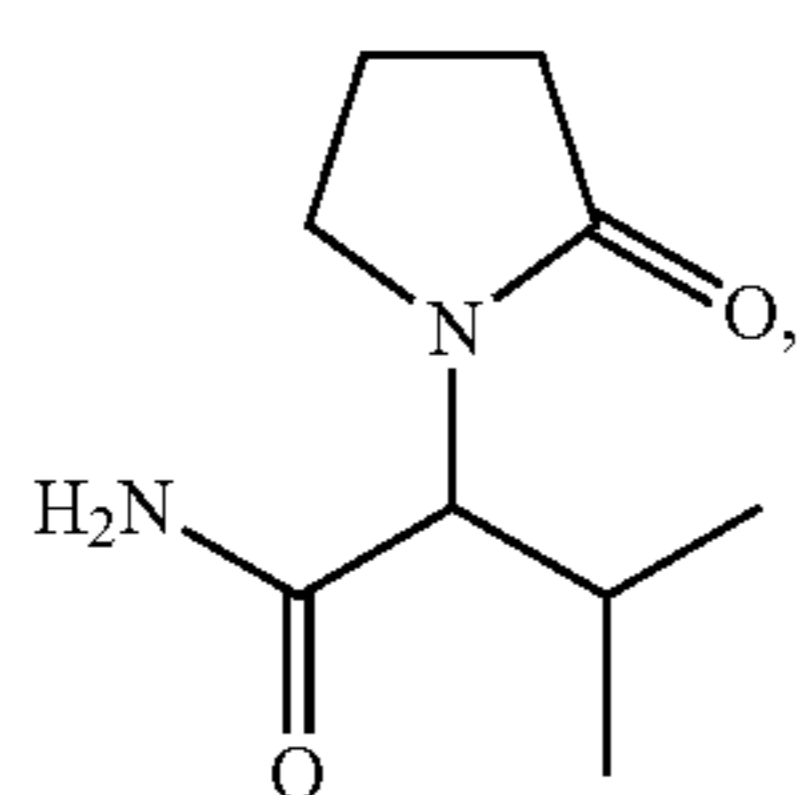
2-(2-oxo-pyrrolidino)-3-methyl-butylamide;
