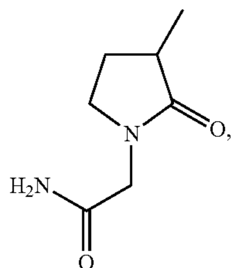
(3-methyl-2-oxo-pyrrolidino)-acetamide;
