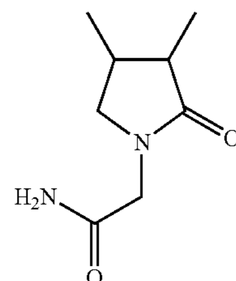
(3,4-dimethyl-2-oxo-pyrrolidino)-acetamide;
