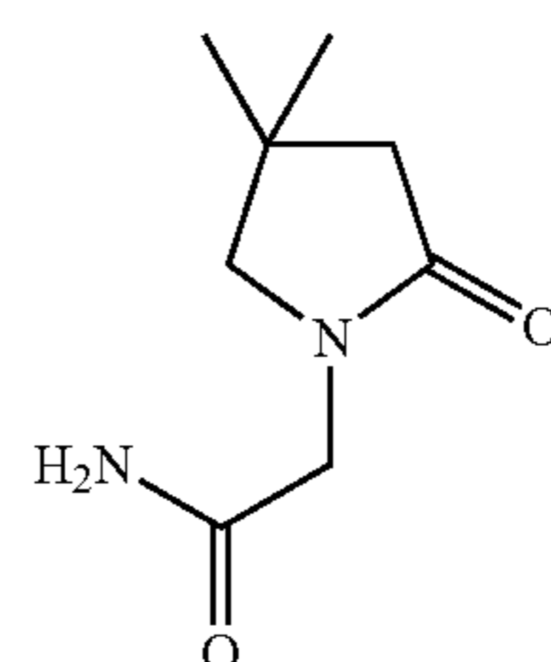
(3,4-dimethyl-2-oxo-pyrrolidino)-acetamide;
