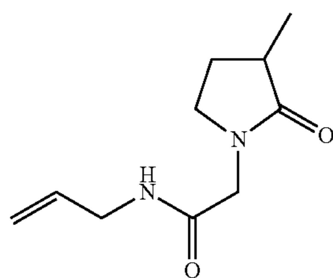
N-allyl-(3-methyl-2-oxo-pyrrolidino)-acetamide;
