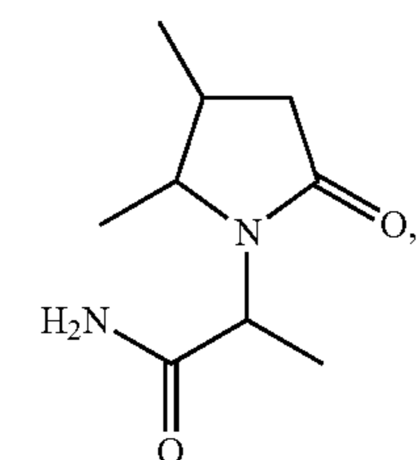
2-(4,5-dimethyl-2-oxo-pyrrolidino)-propionamide;
