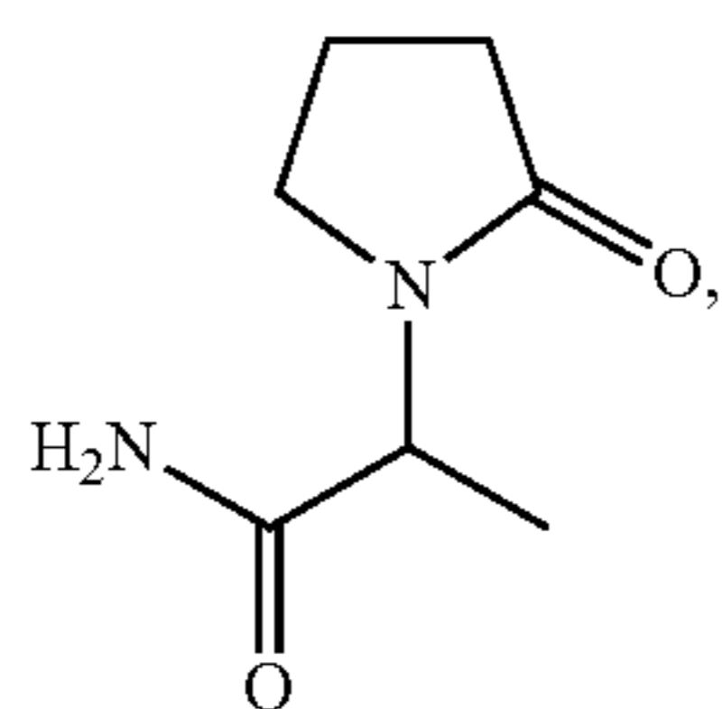
2-(2-oxo-pyrrolidino)-propionamide;
