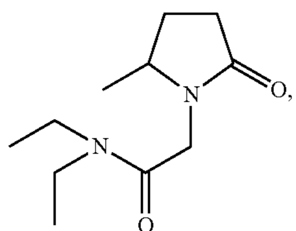
(5-methyl-2-oxo-pyrrolidino)-N,N-diethylacetamide;
