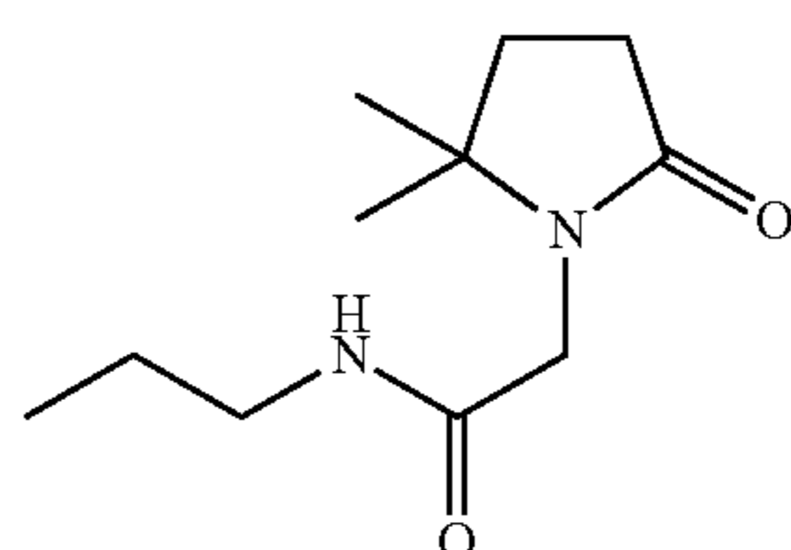
N-n-propyl-(5,5-dimethyl-2-oxo-pyrrolidino)-acetamide;
