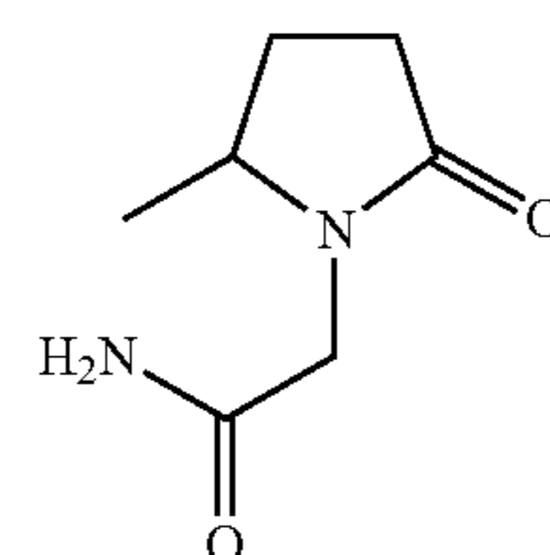
(5-methyl-2-oxo-pyrrolidino)-acetamide;
