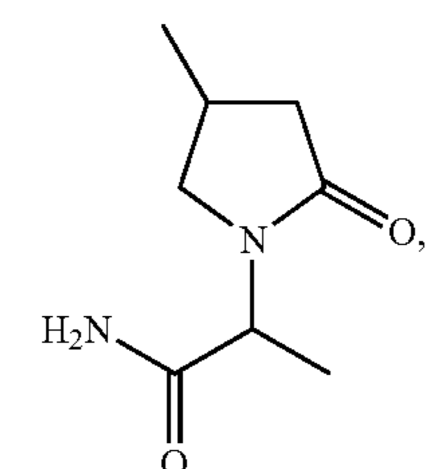
2-(4-methyl-2-oxo-pyrrolidino)-propionamide;
