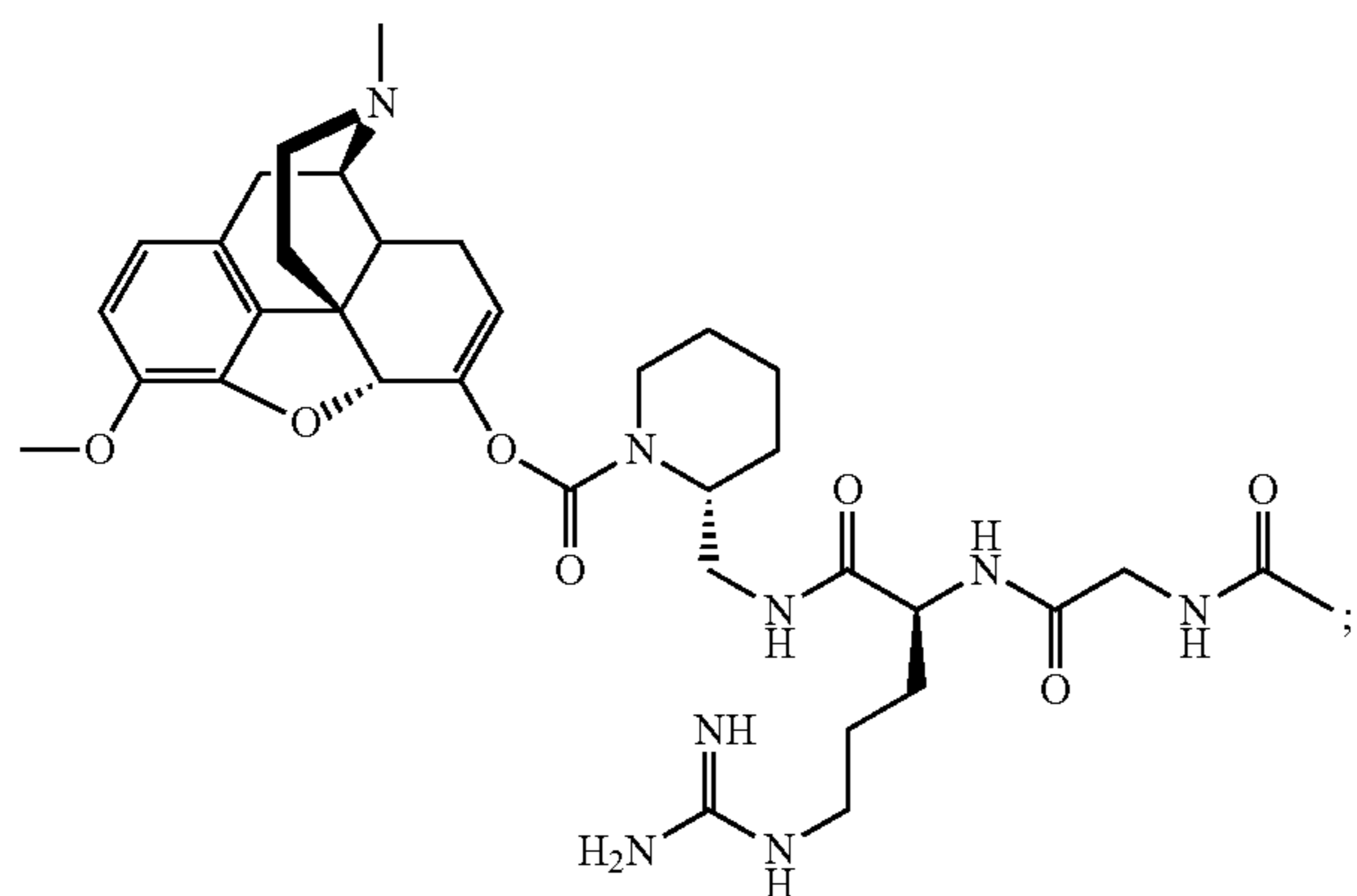
Compound KC-36:
