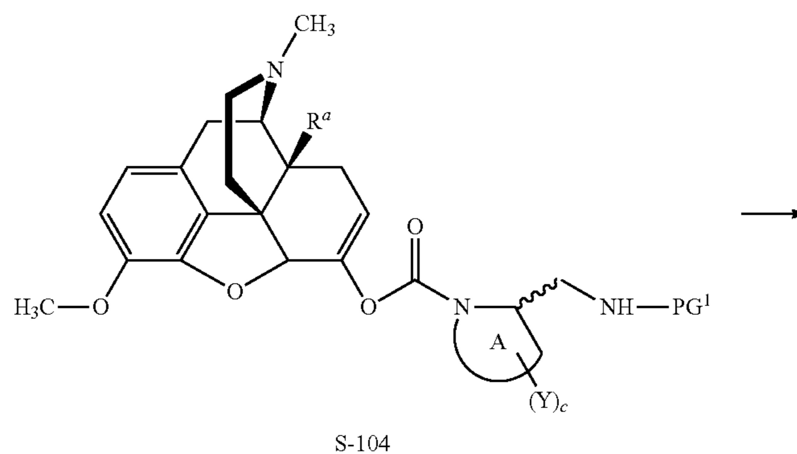
Scheme 2
