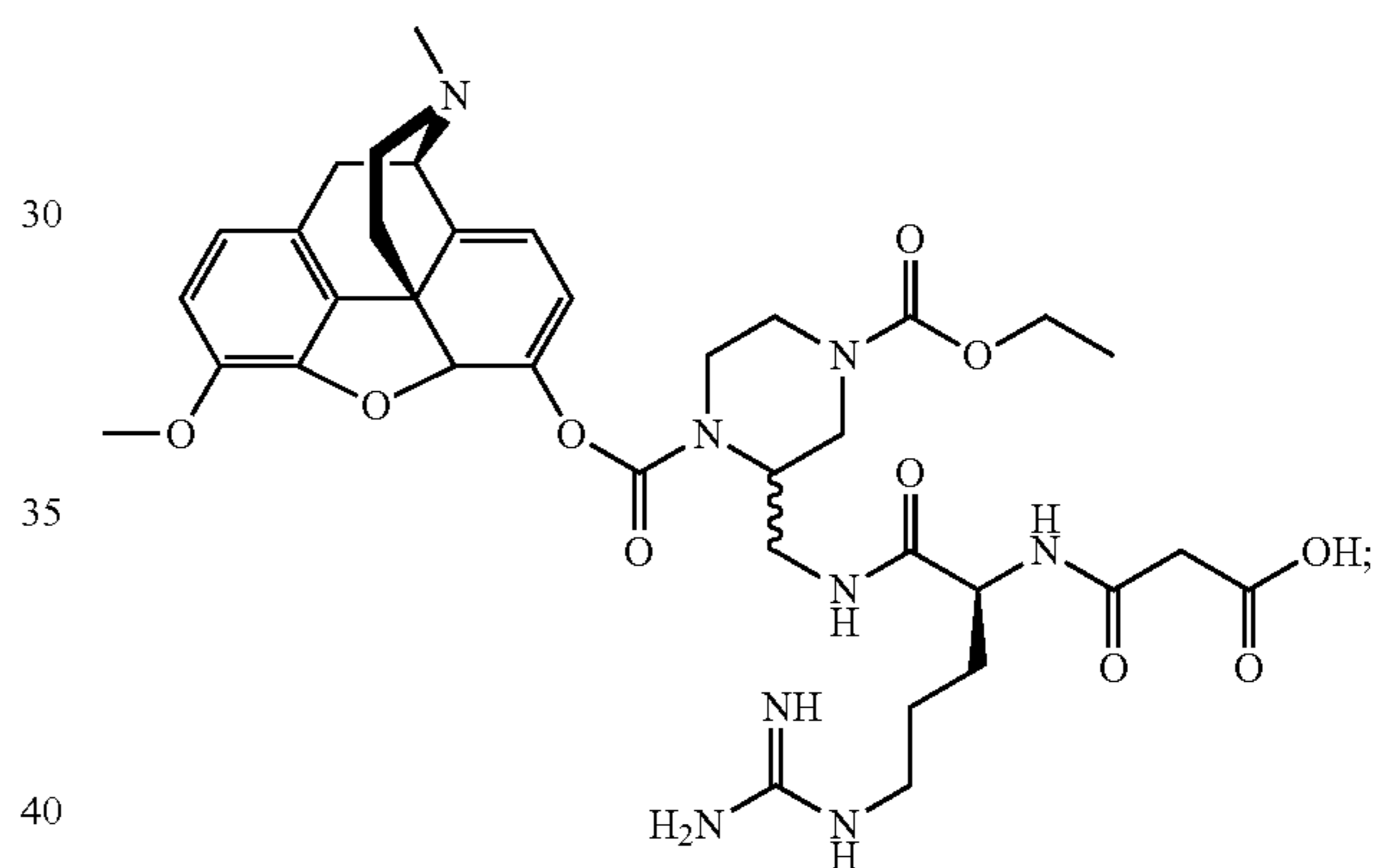
Compound KC-44:
