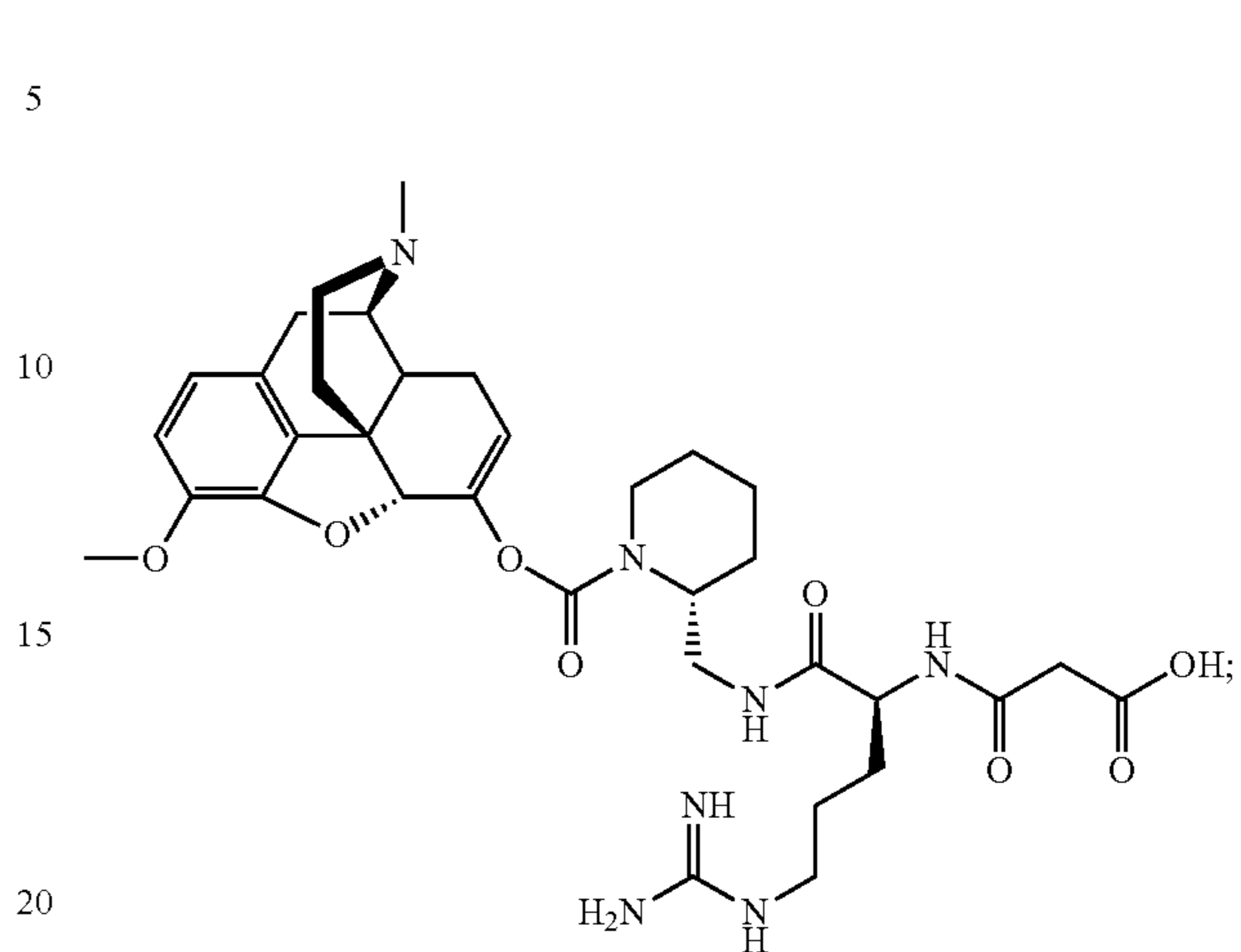
Compound KC-39:
