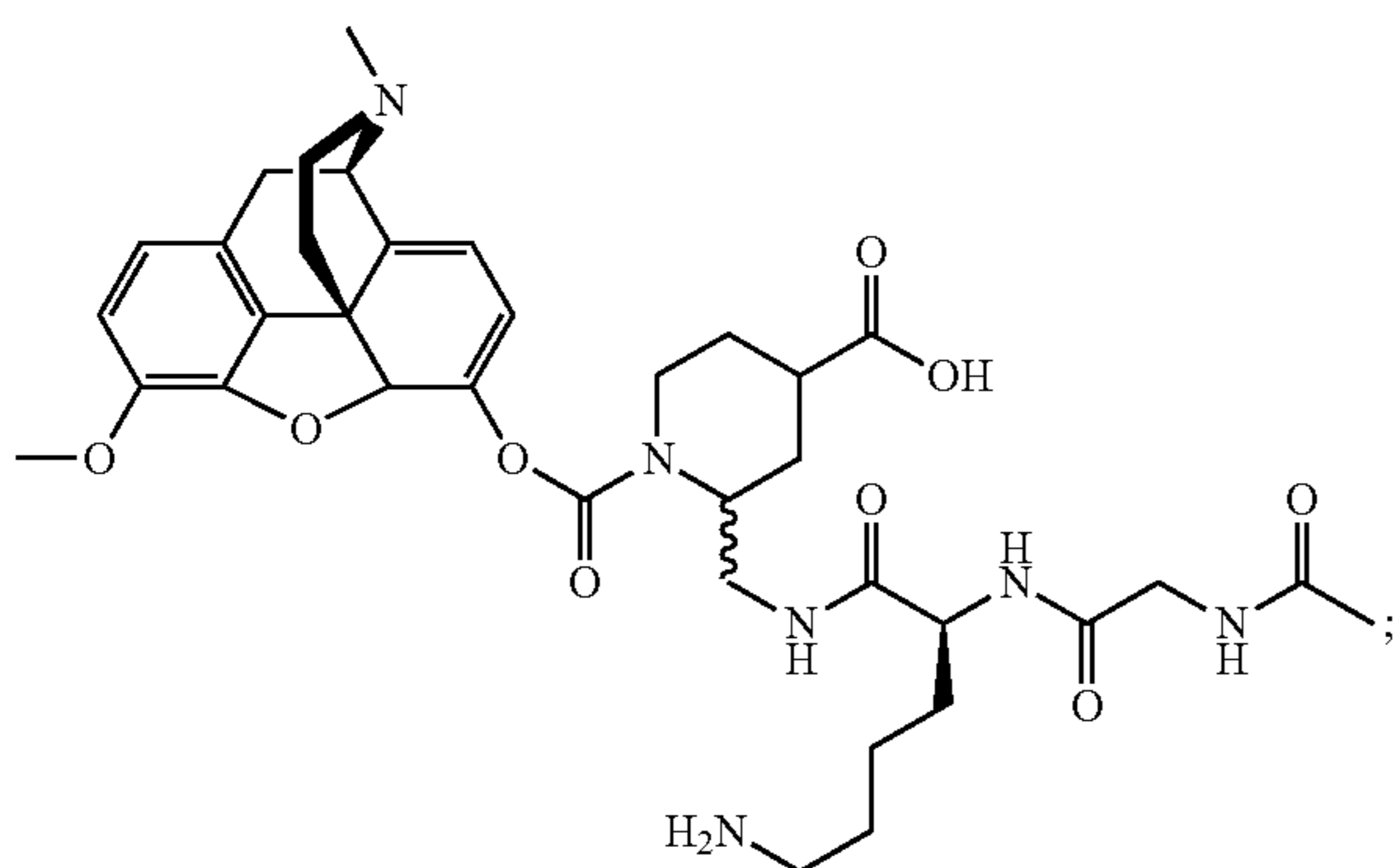
Compound KC-50:
