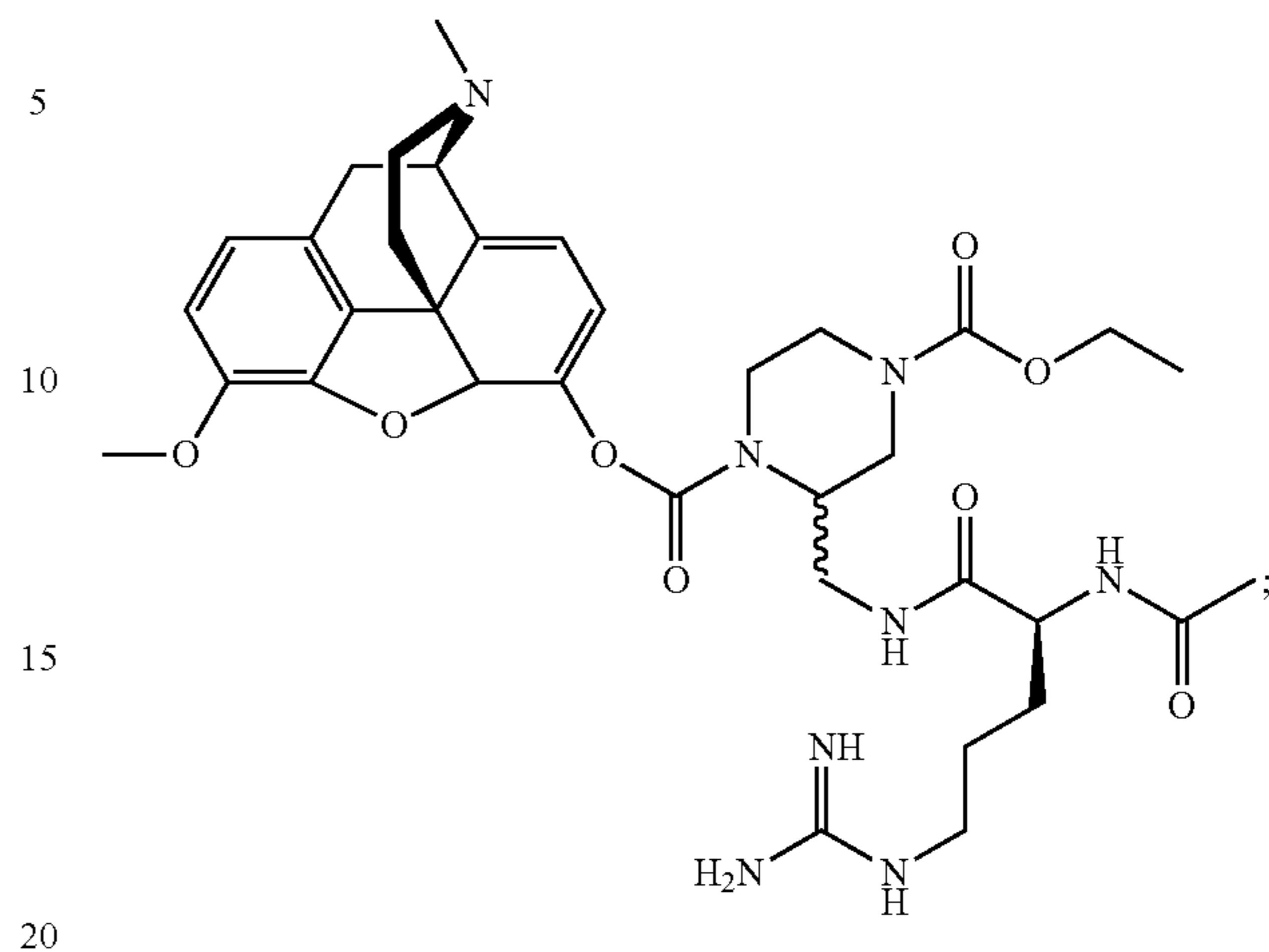
Compound KC-43:
