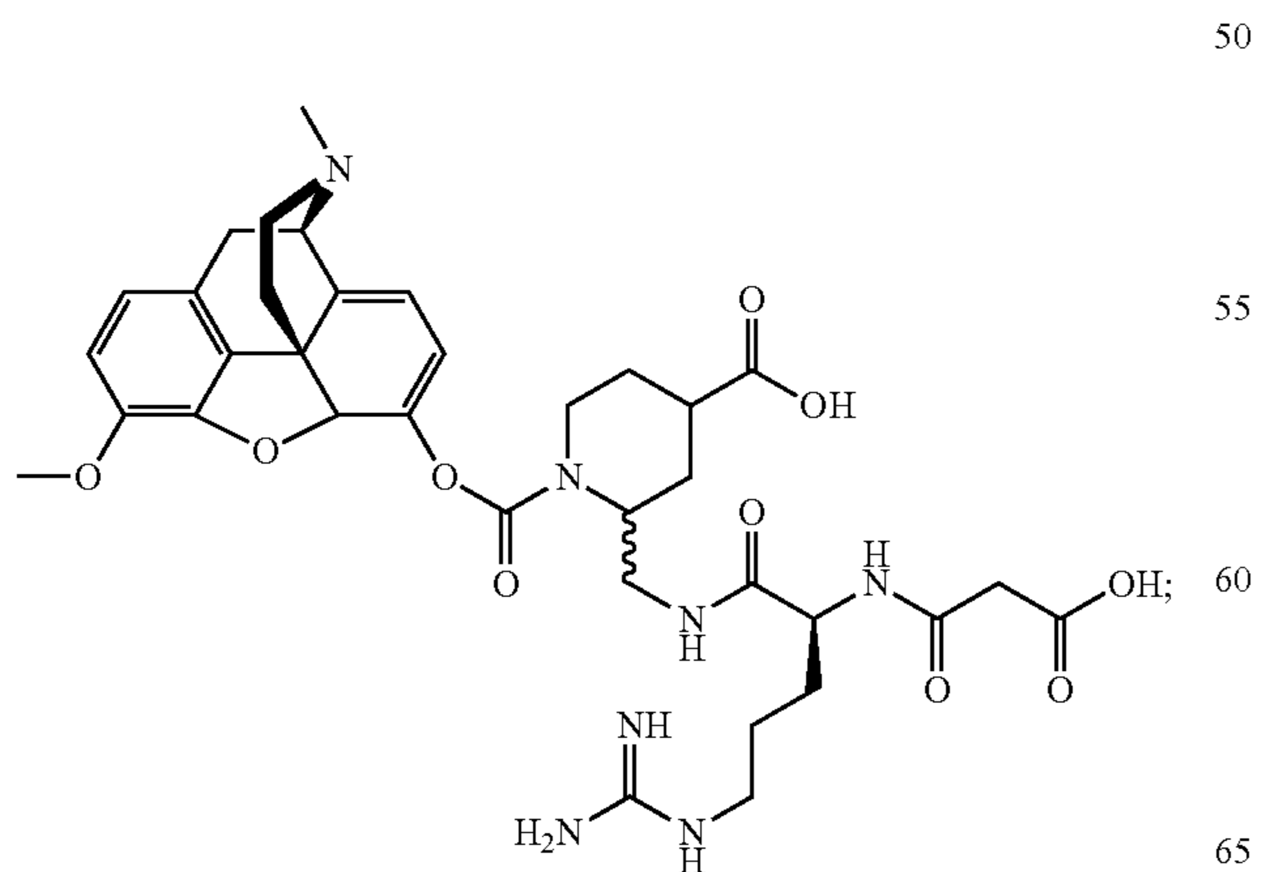
Compound KC-48:
