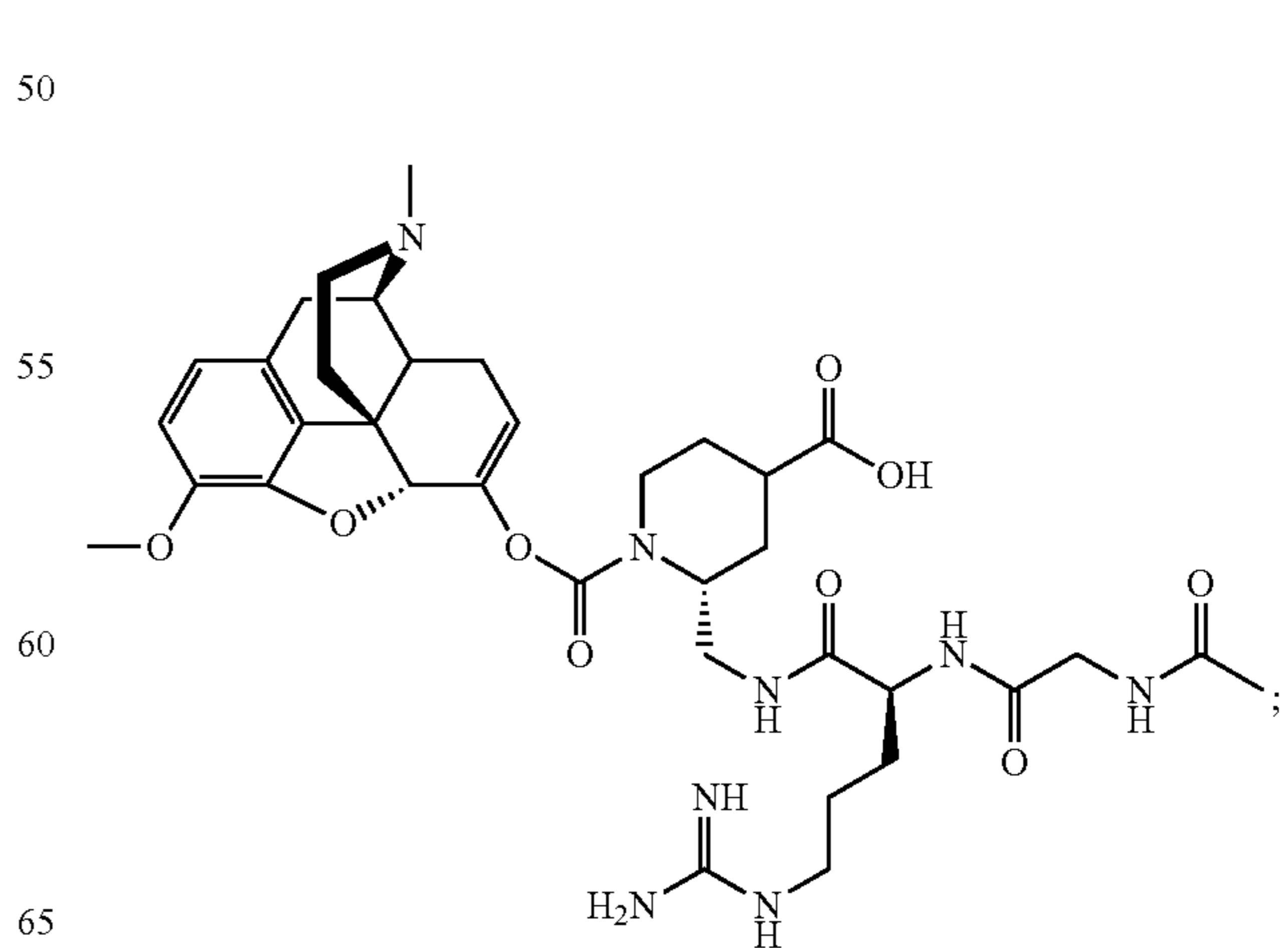
Compound KC-40:
