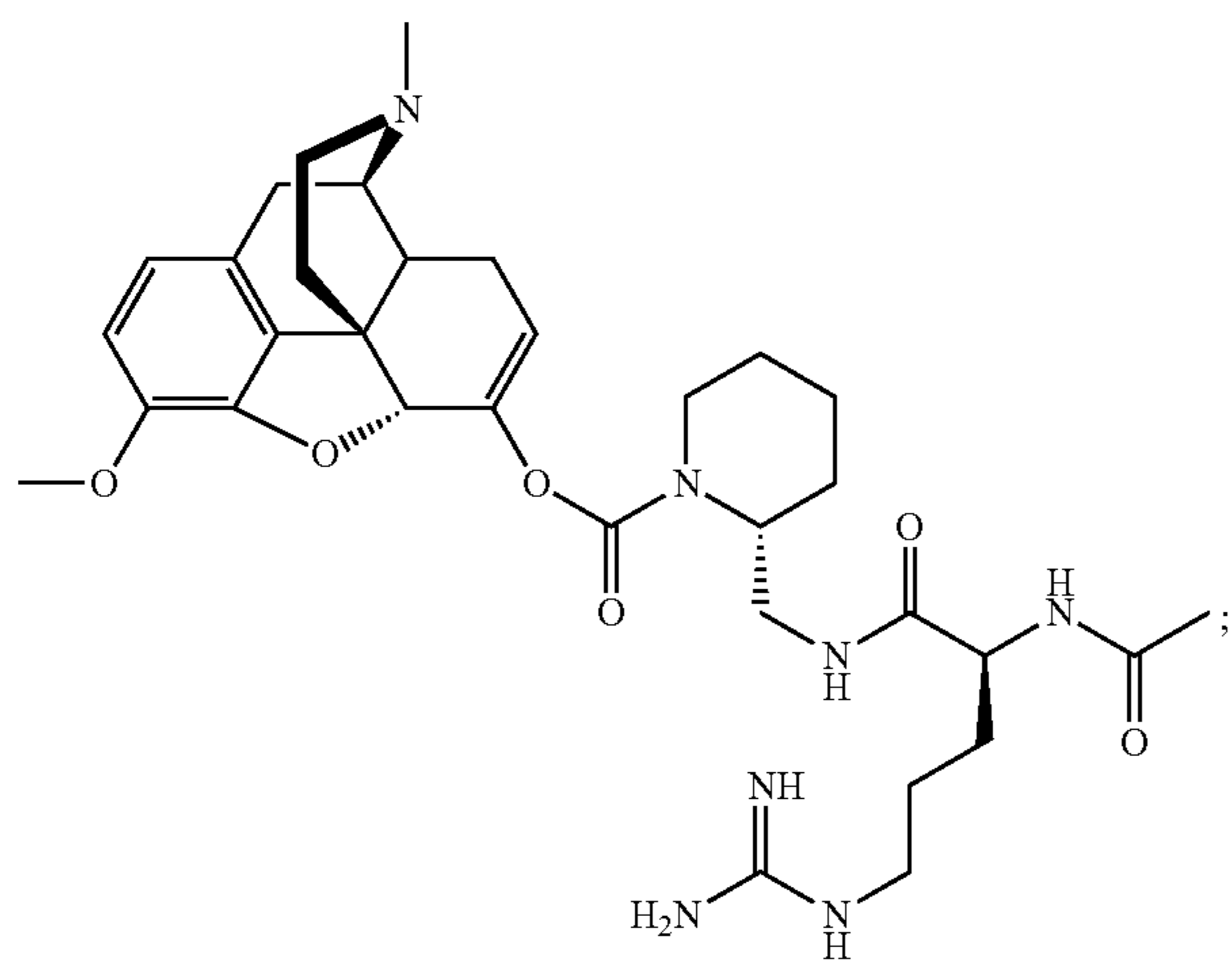
Compound KC-38:
