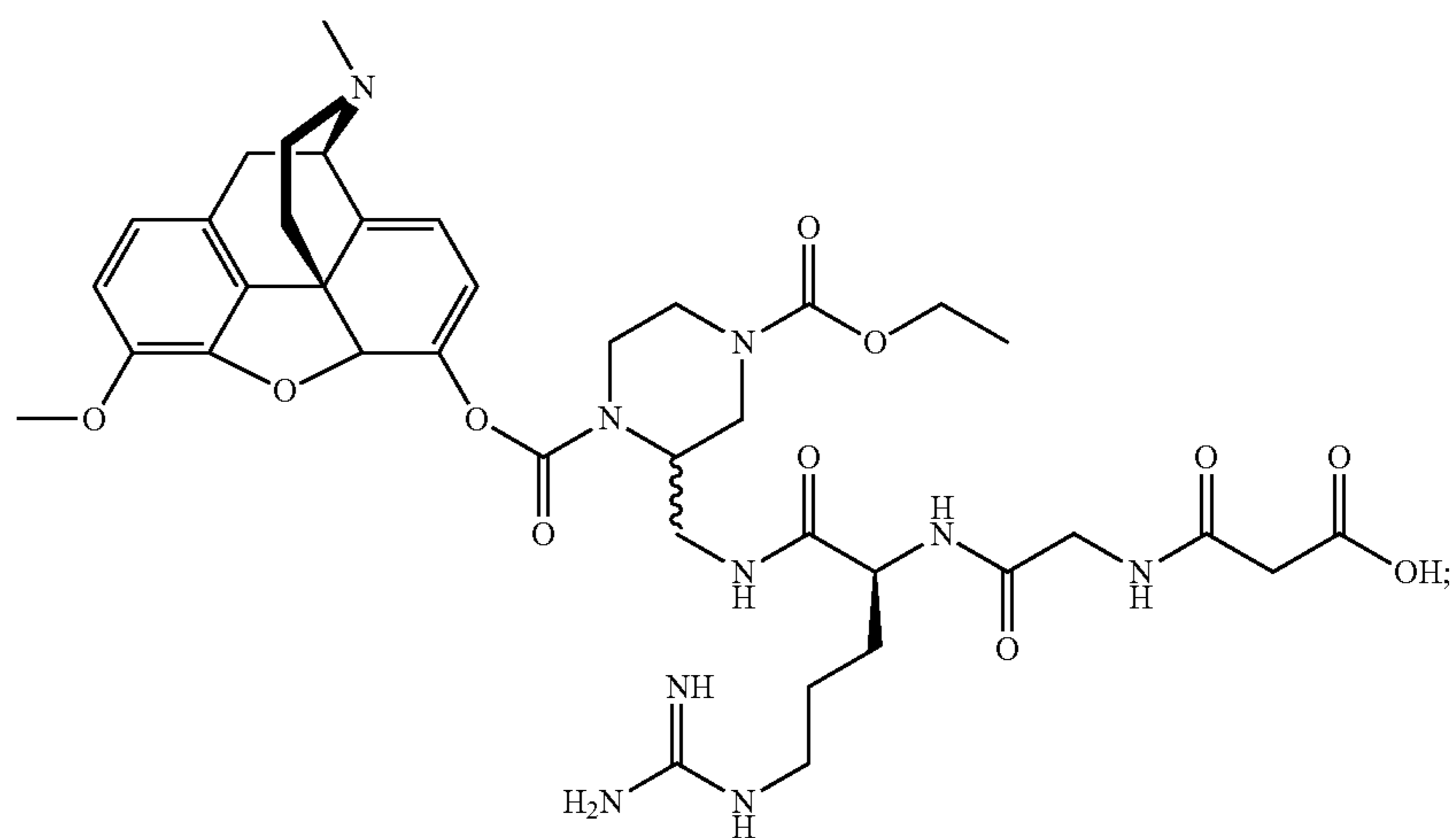
Compound KC-45:
