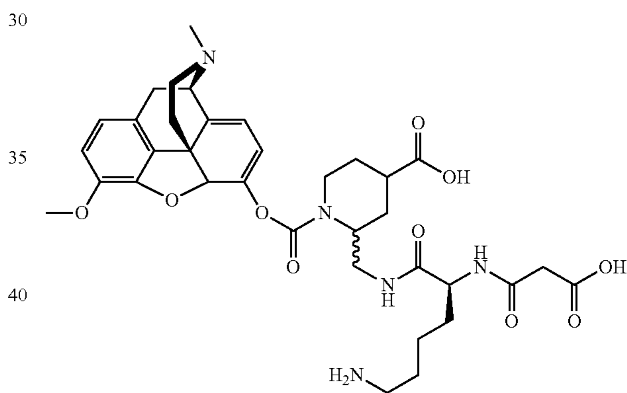
Compound KC-53:
