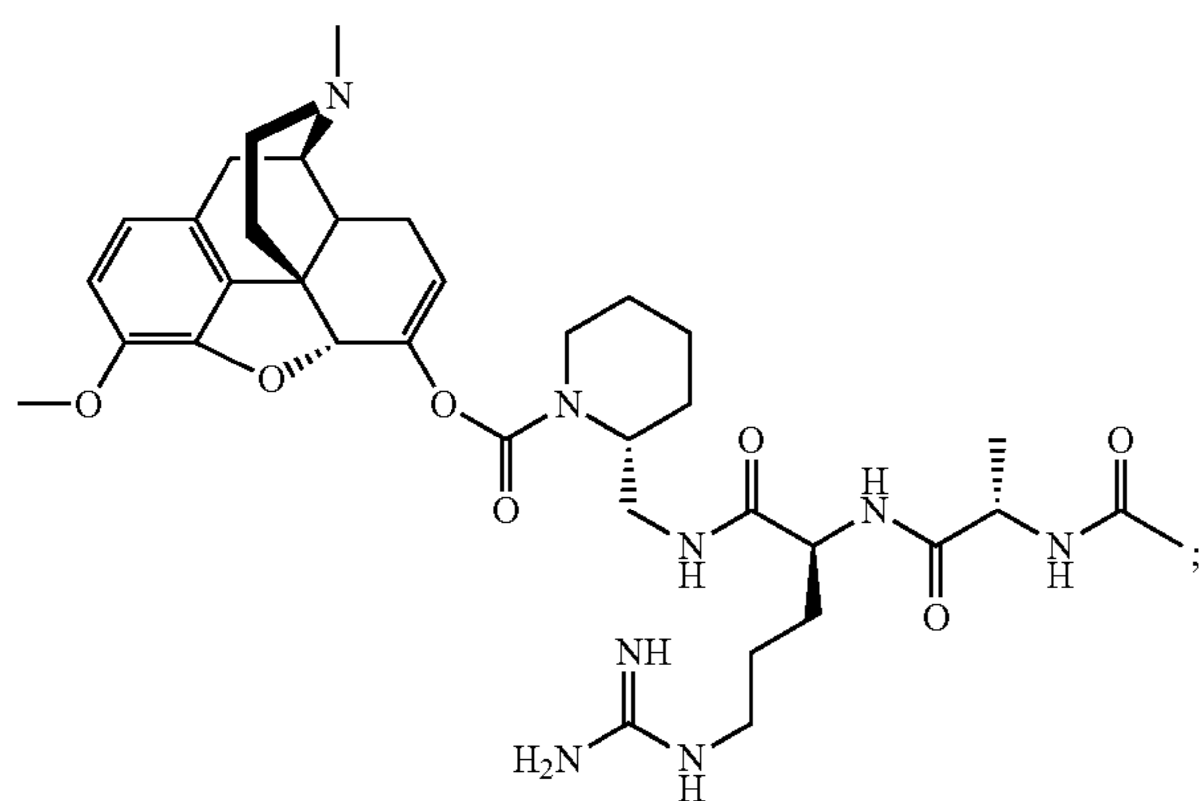
Compound KC-37:
