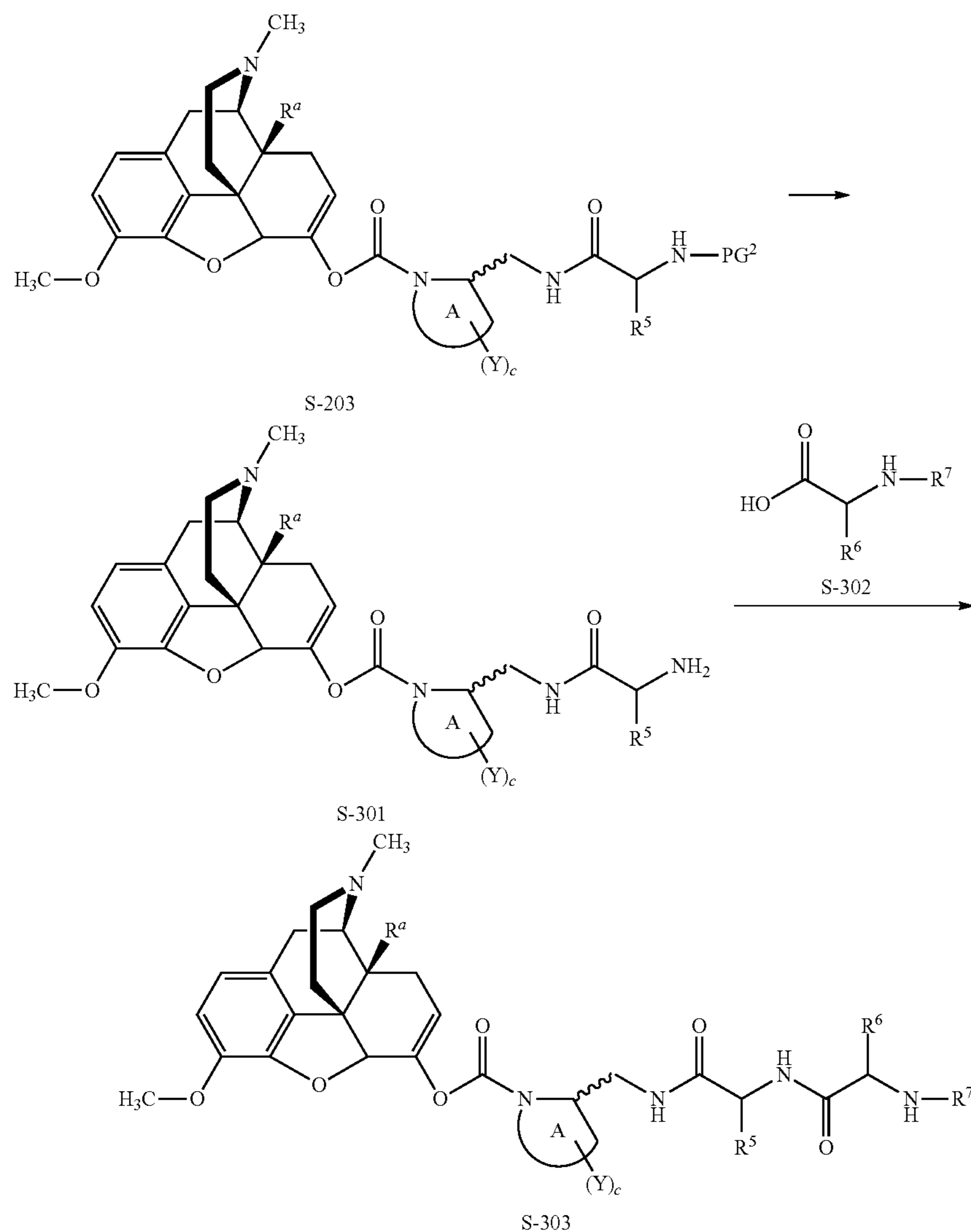
Scheme 3
