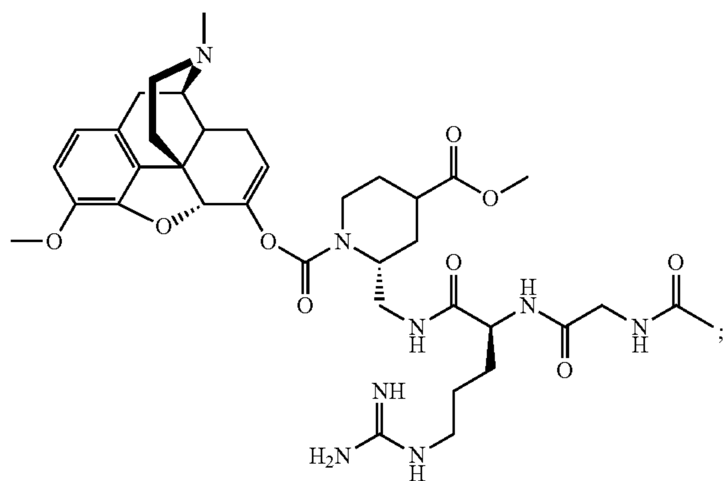
Compound KC-41:
