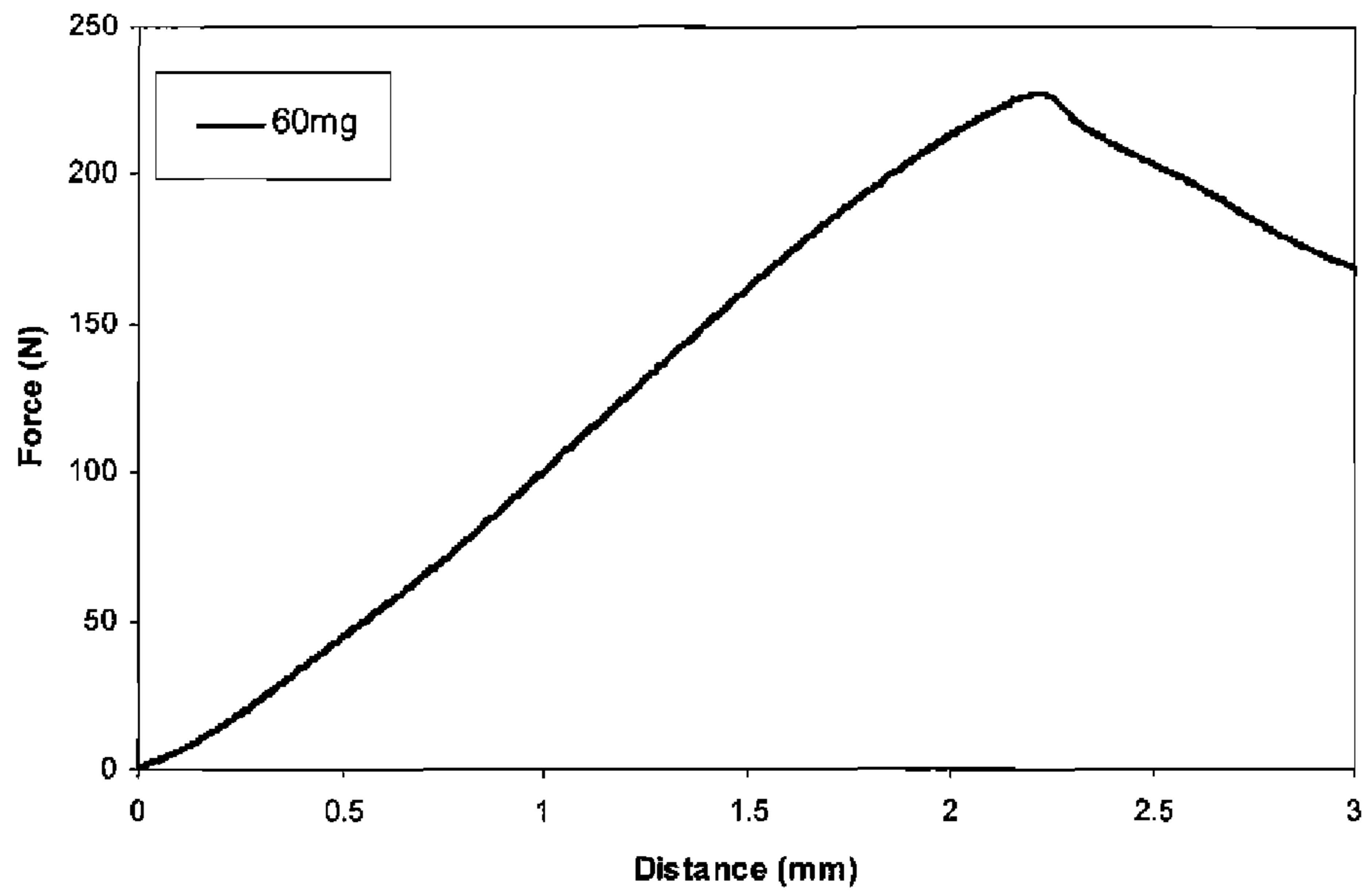
Example 20 Indentation Test of Example 16.1 tablet
