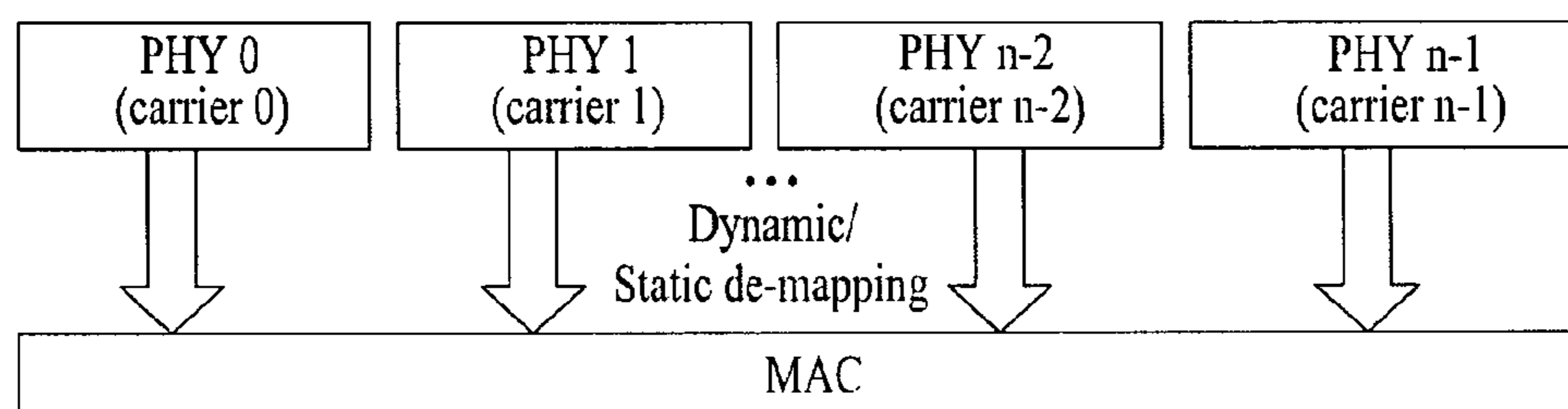
(b) Receiver
