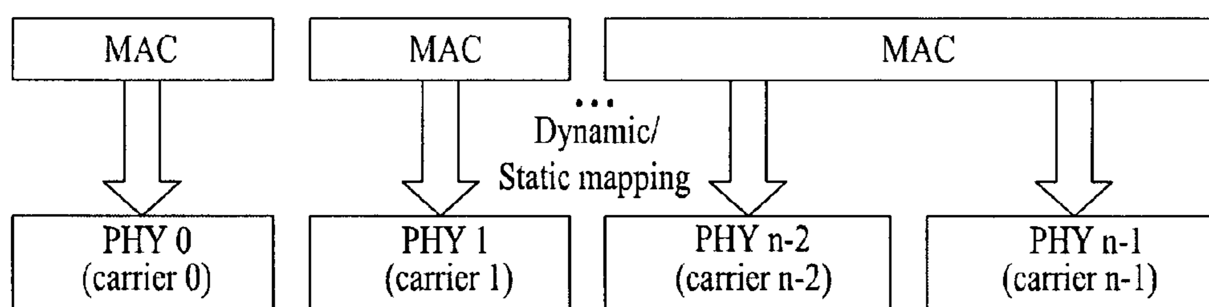
(a) Transmitter
