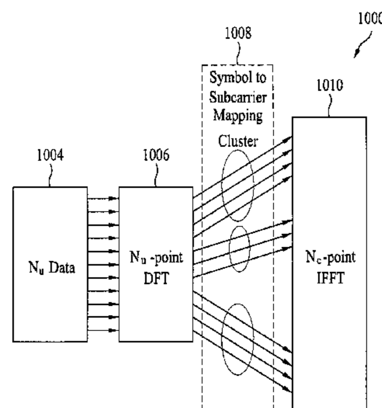
Clustered DFT-s-OFDMA
