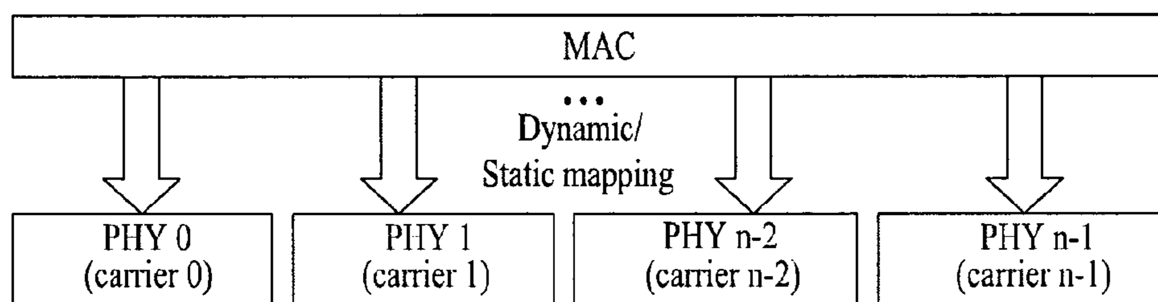
(a) Transmitter
