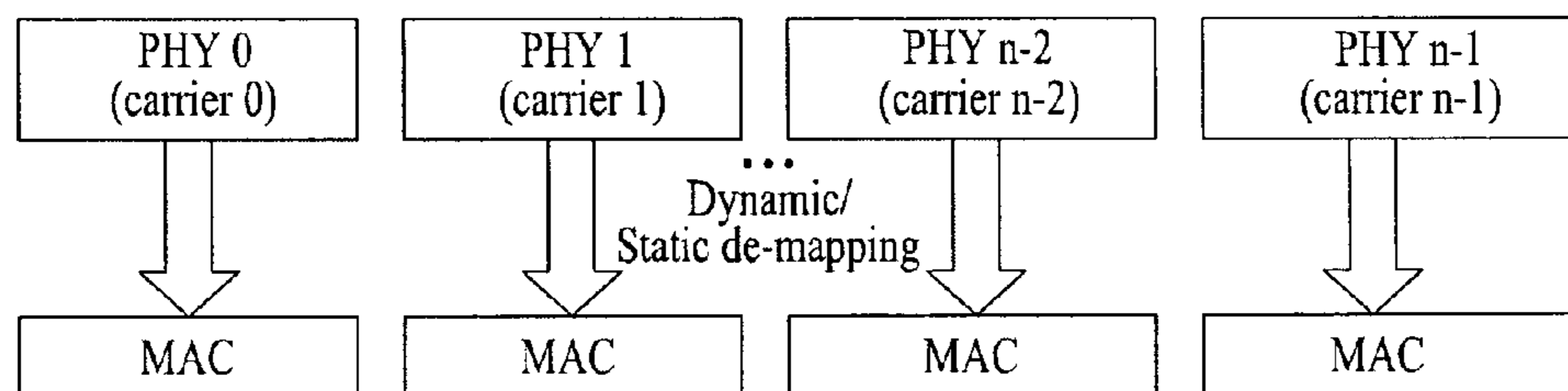
(b) Receiver
