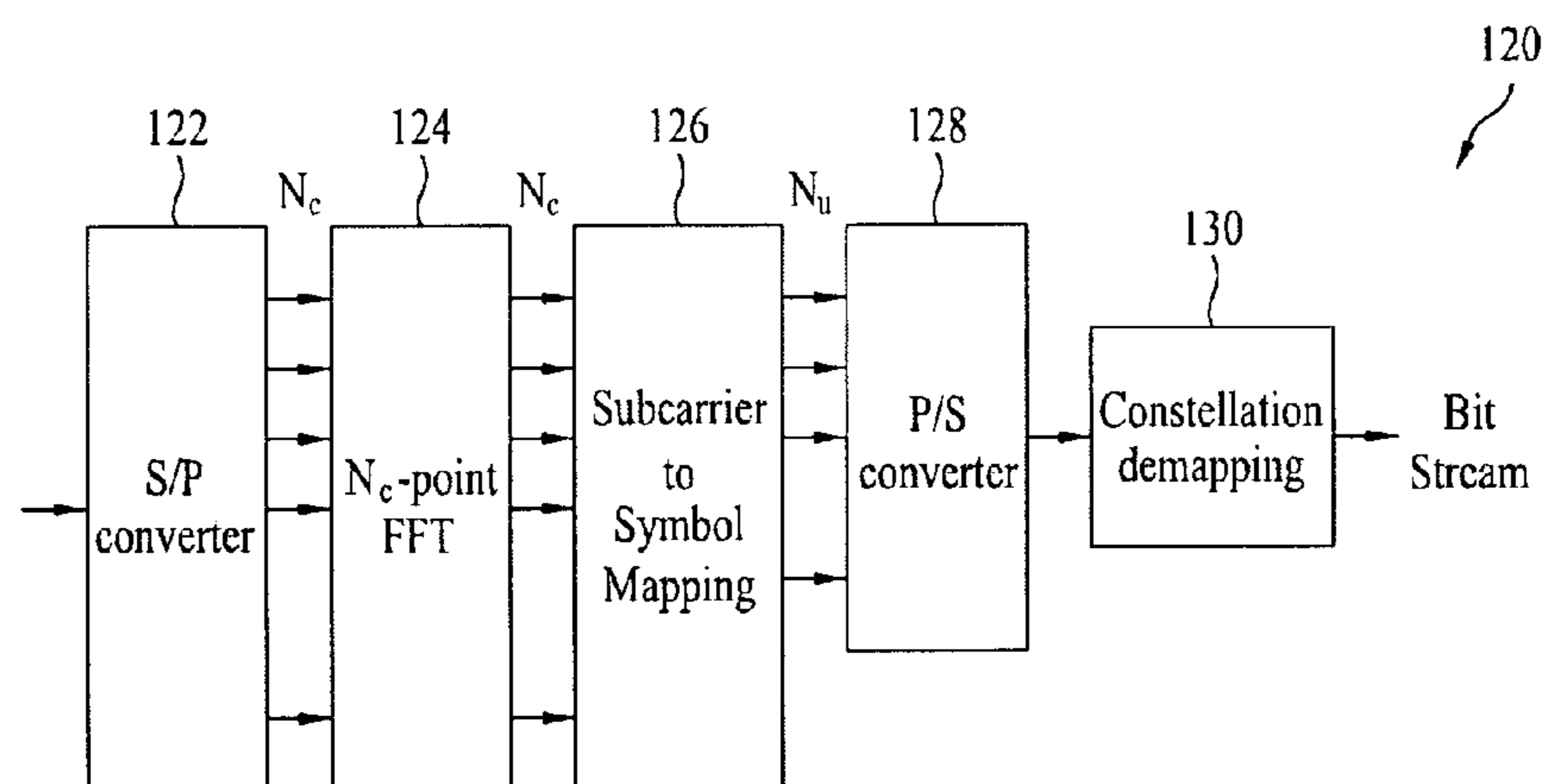
Conventional OFDMA receiver
