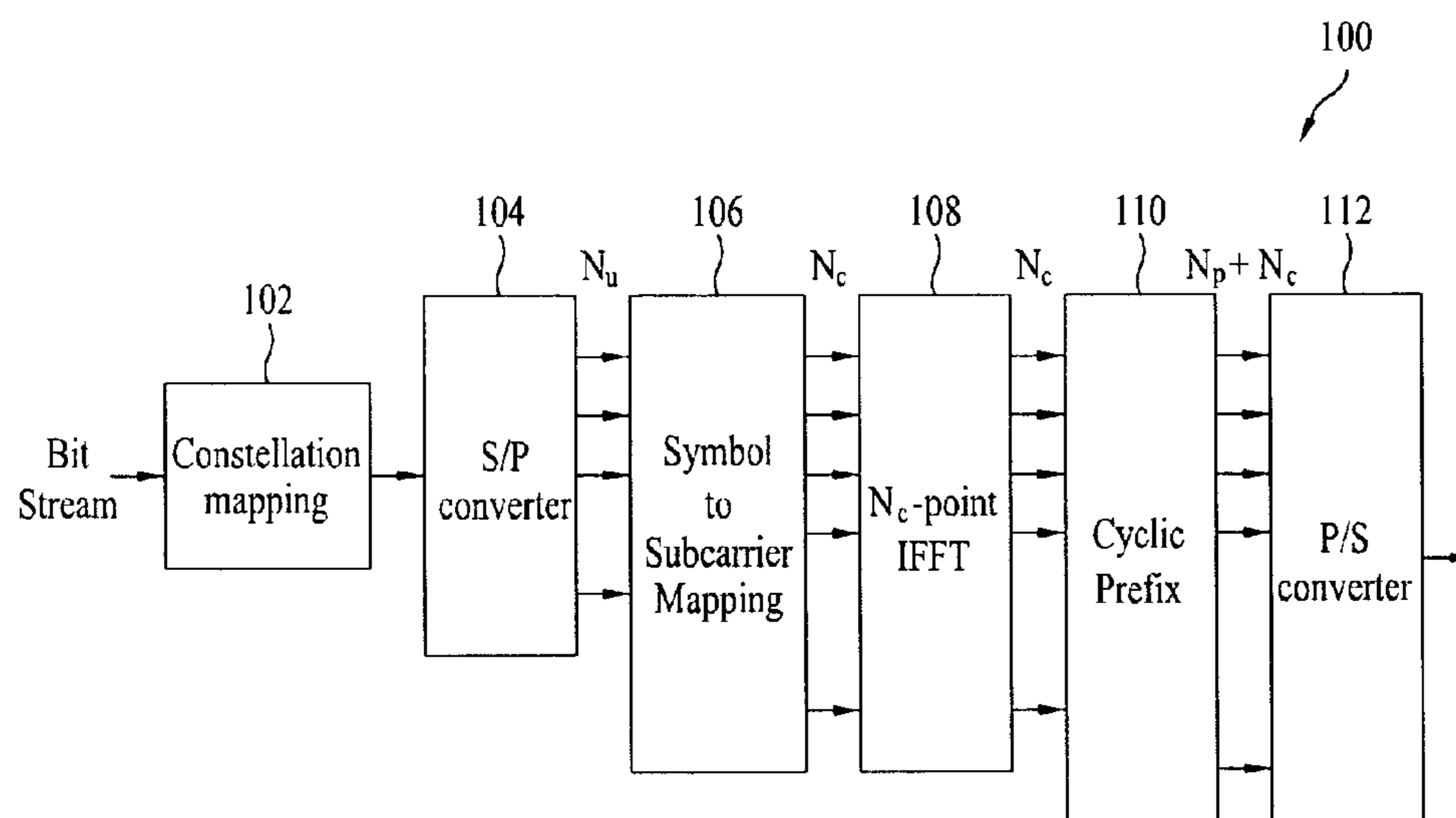
Conventional OFDMA transmitter
