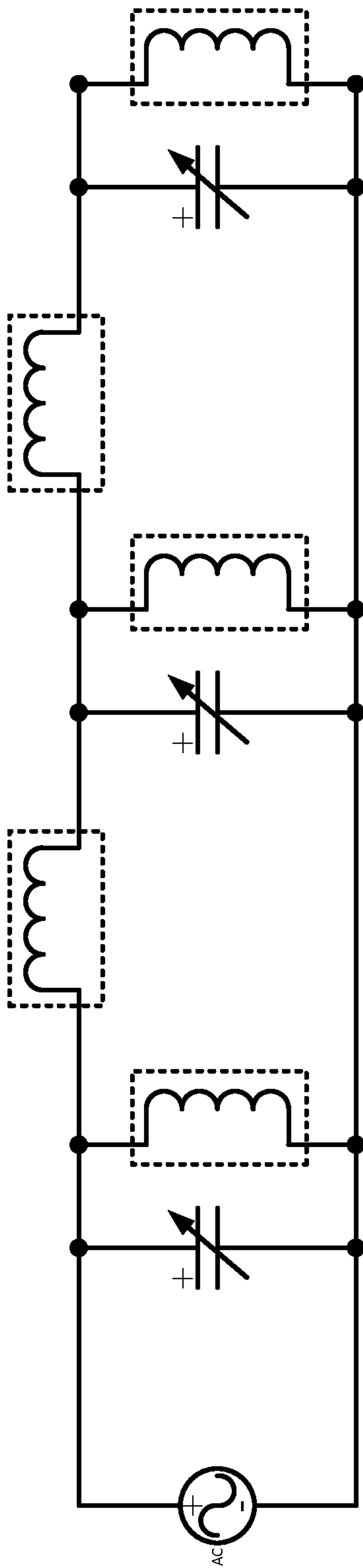
Pi-Type Band Pass Filter
