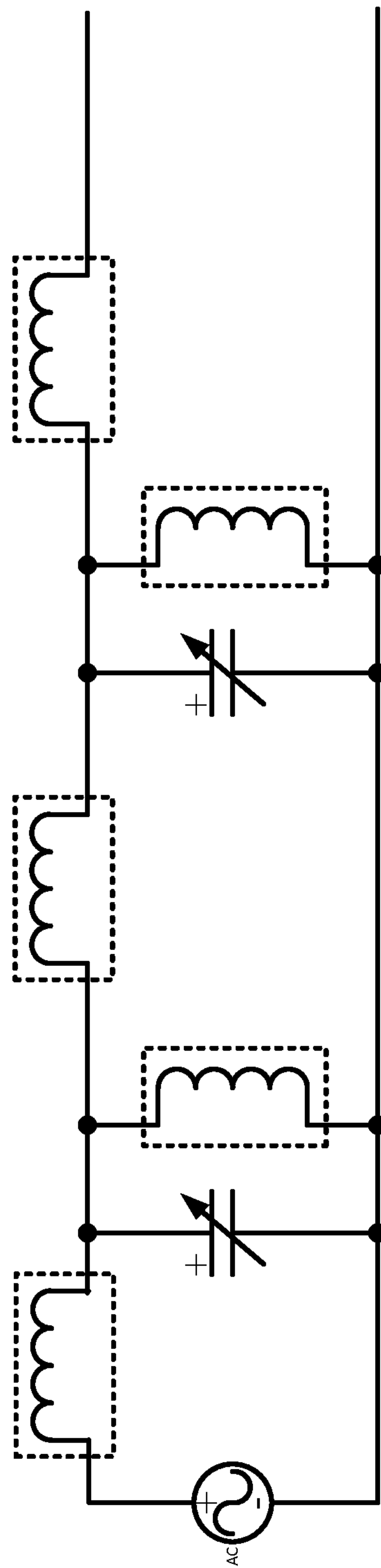
T-Type Band Pass Filter
