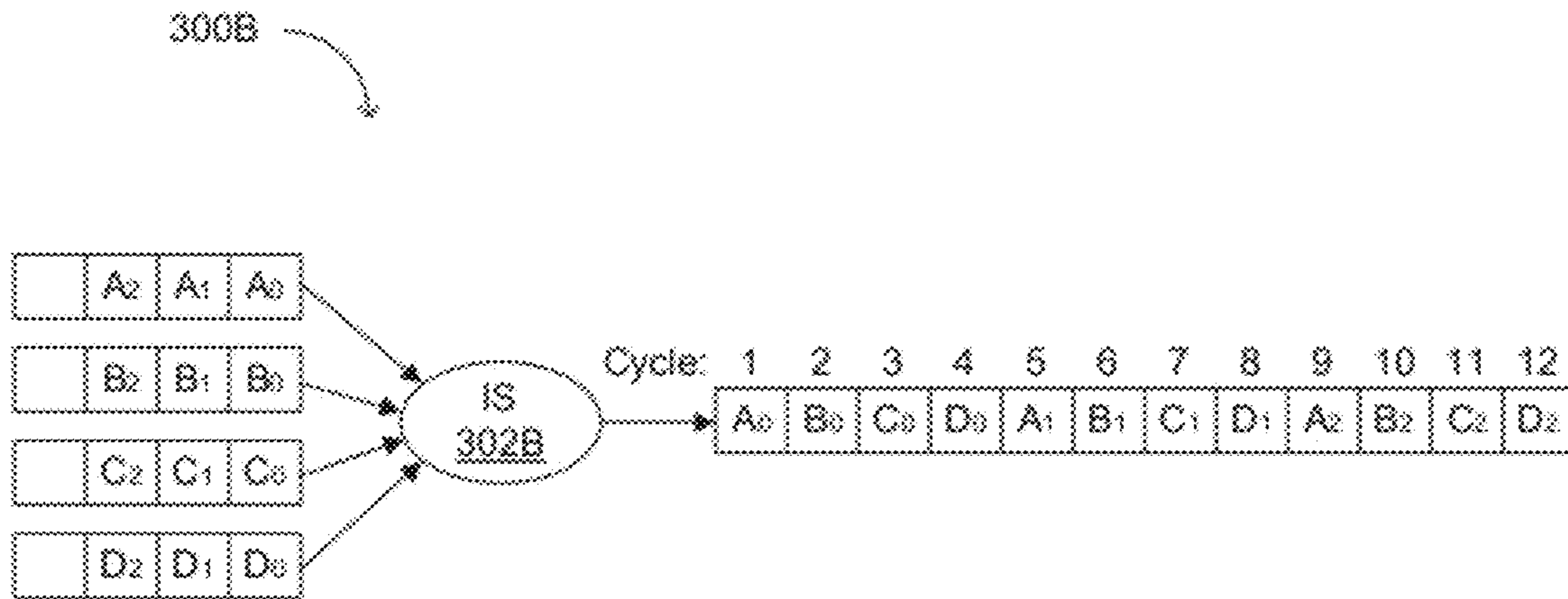
FIG. 3B (conventional)
