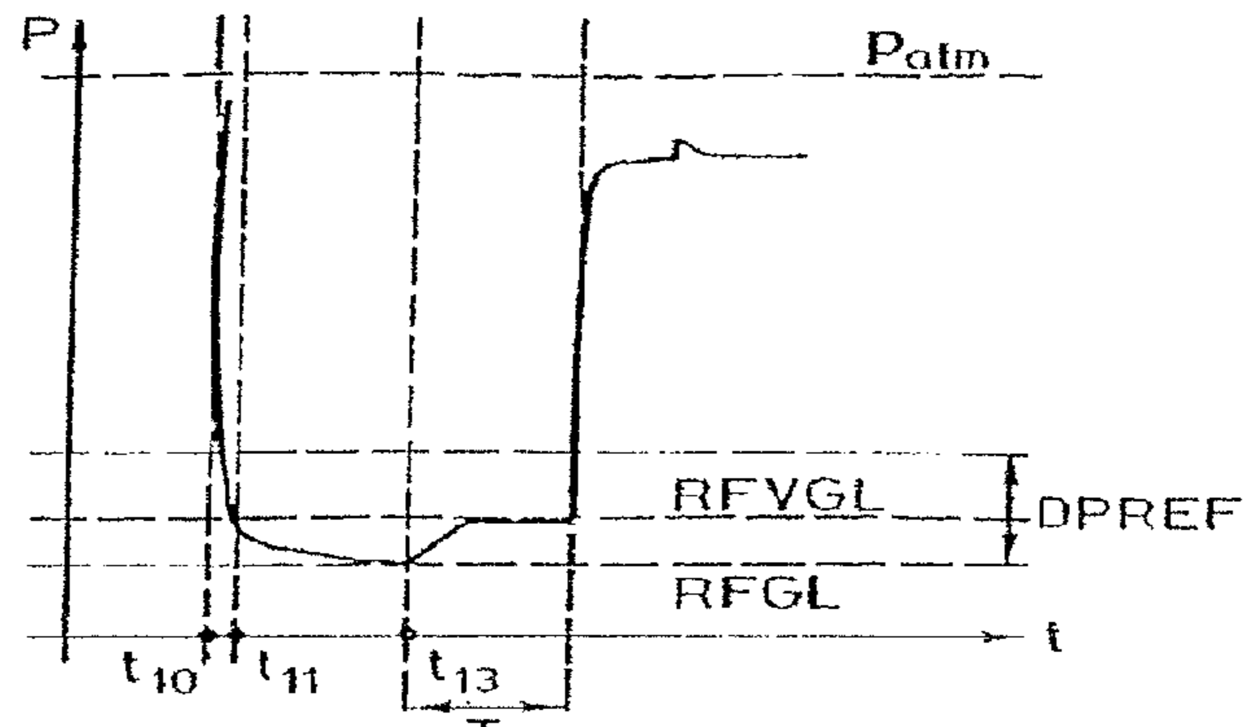
EVAC TEST VENT FIG.11c
