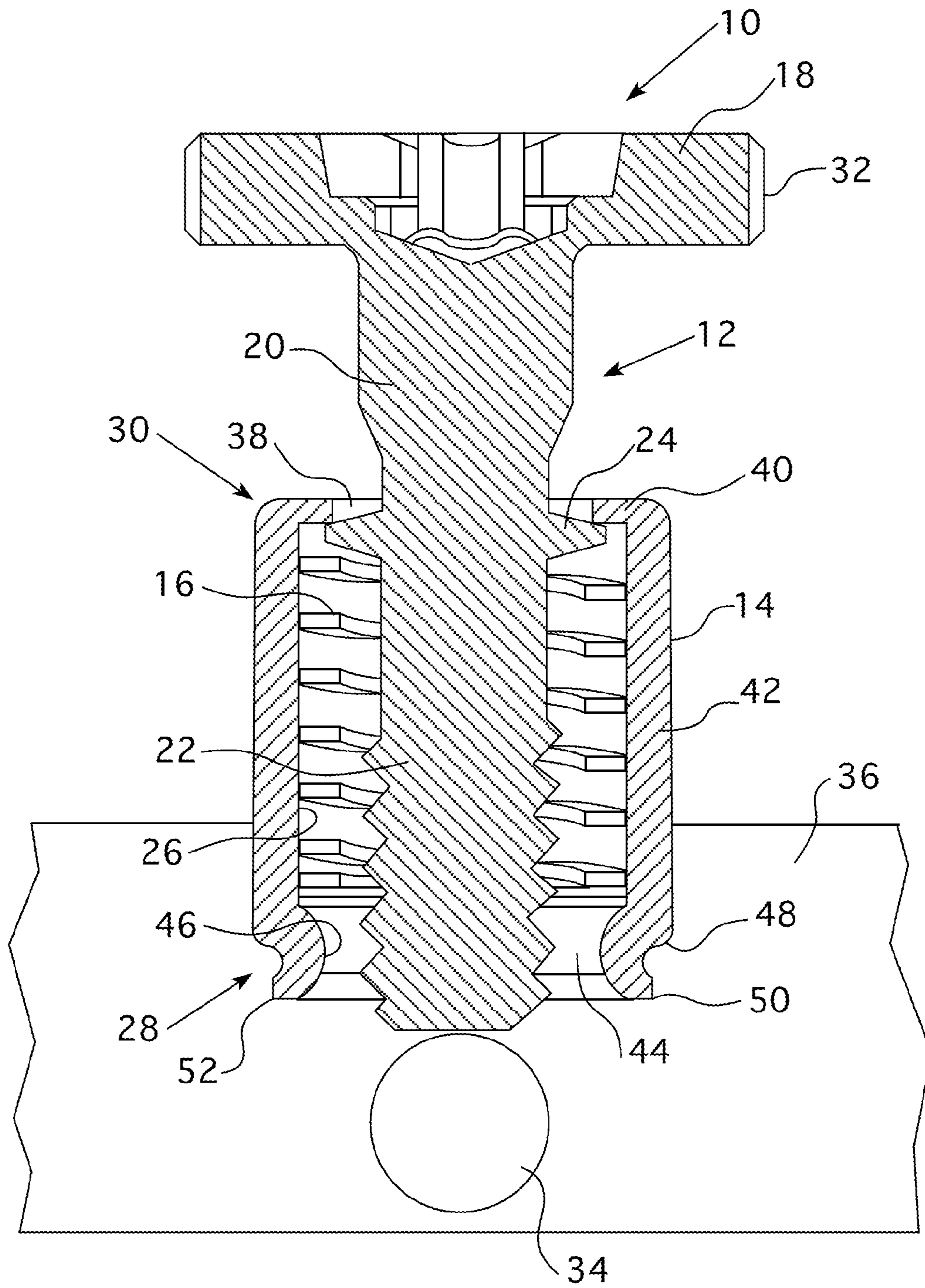
FIG. 1 (Prior Art)
