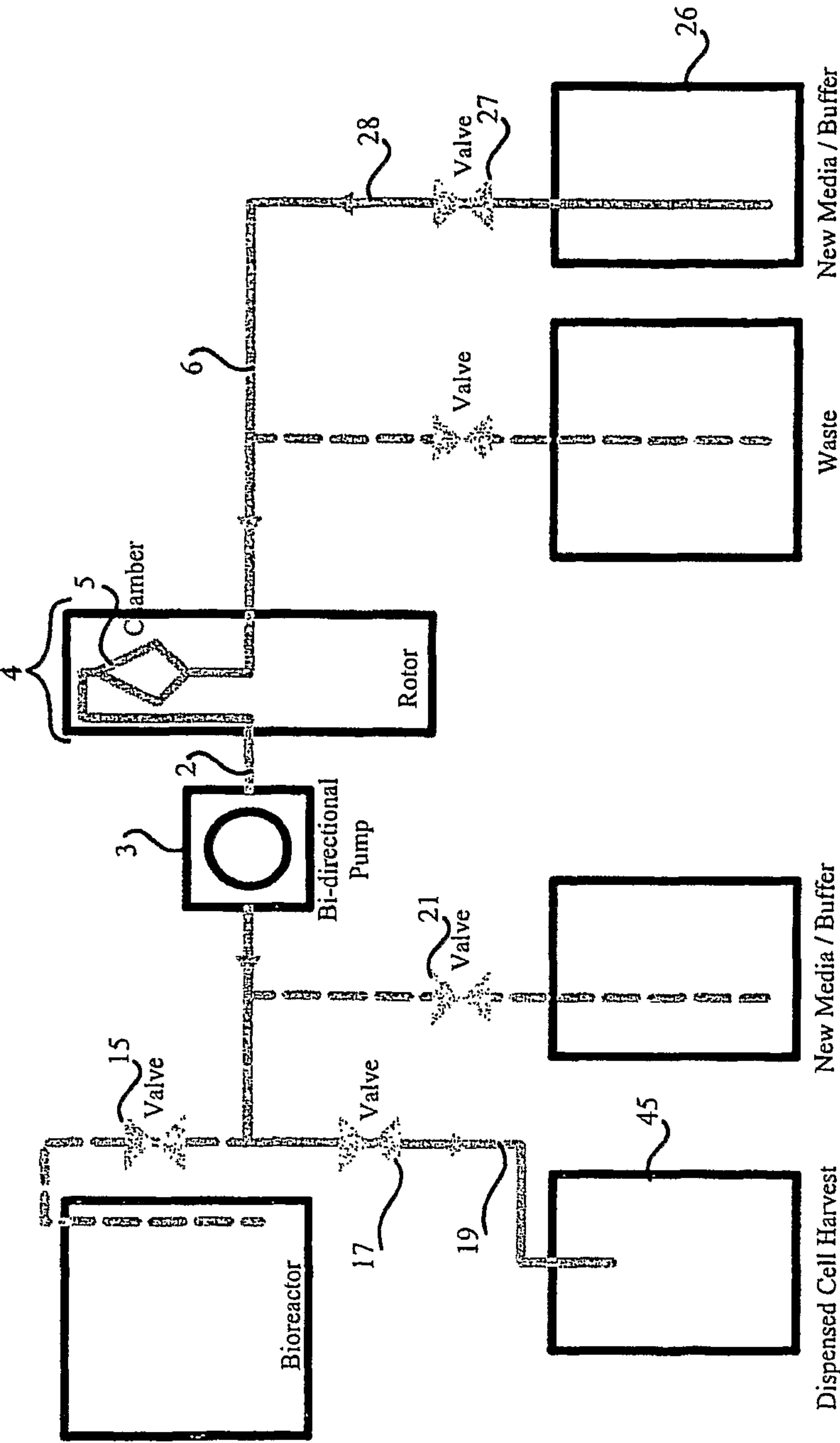
Figure 23 Cell Dispenser Flow Diagram Dispense Mode
