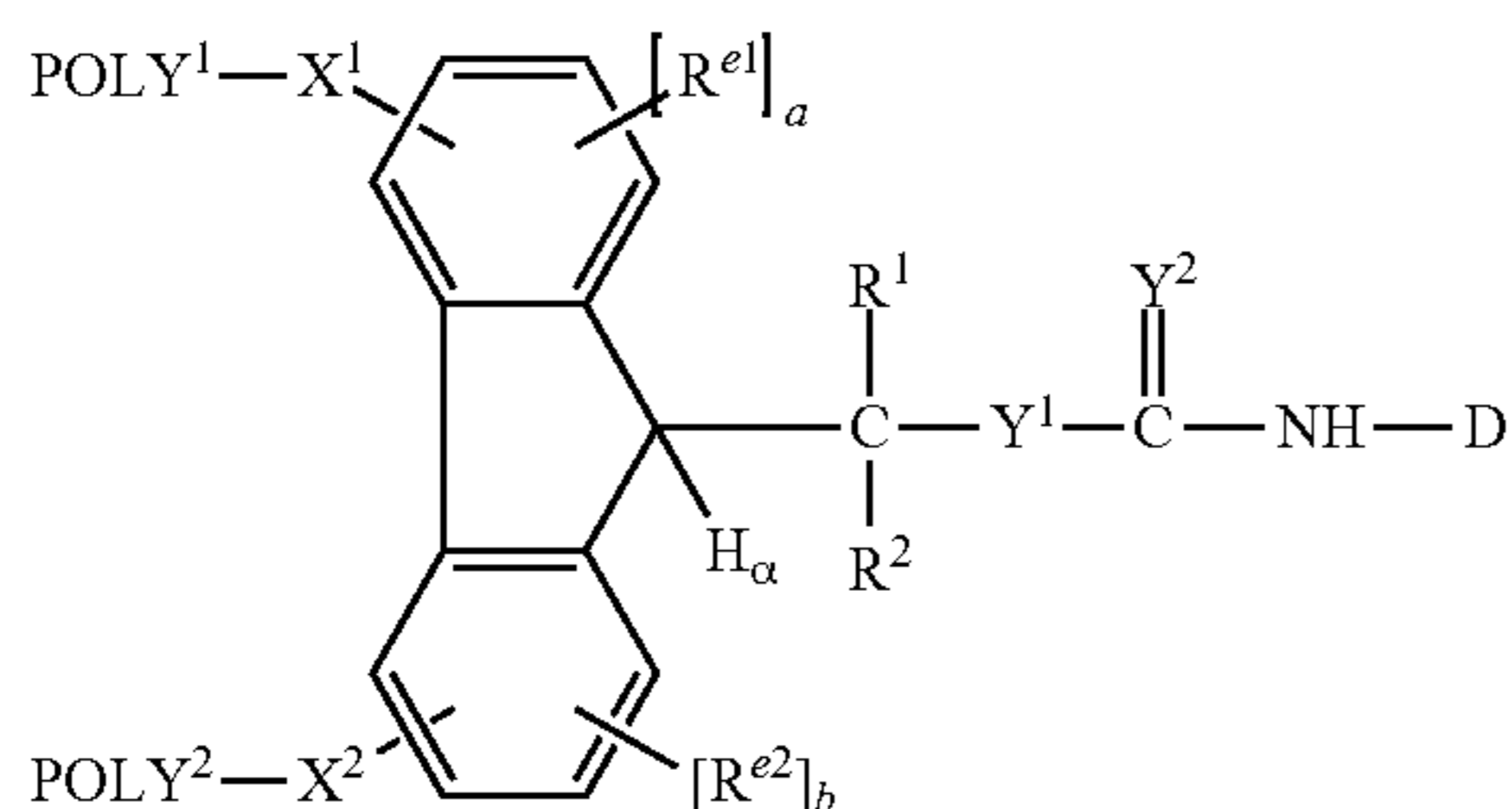
(Formula V-C)
