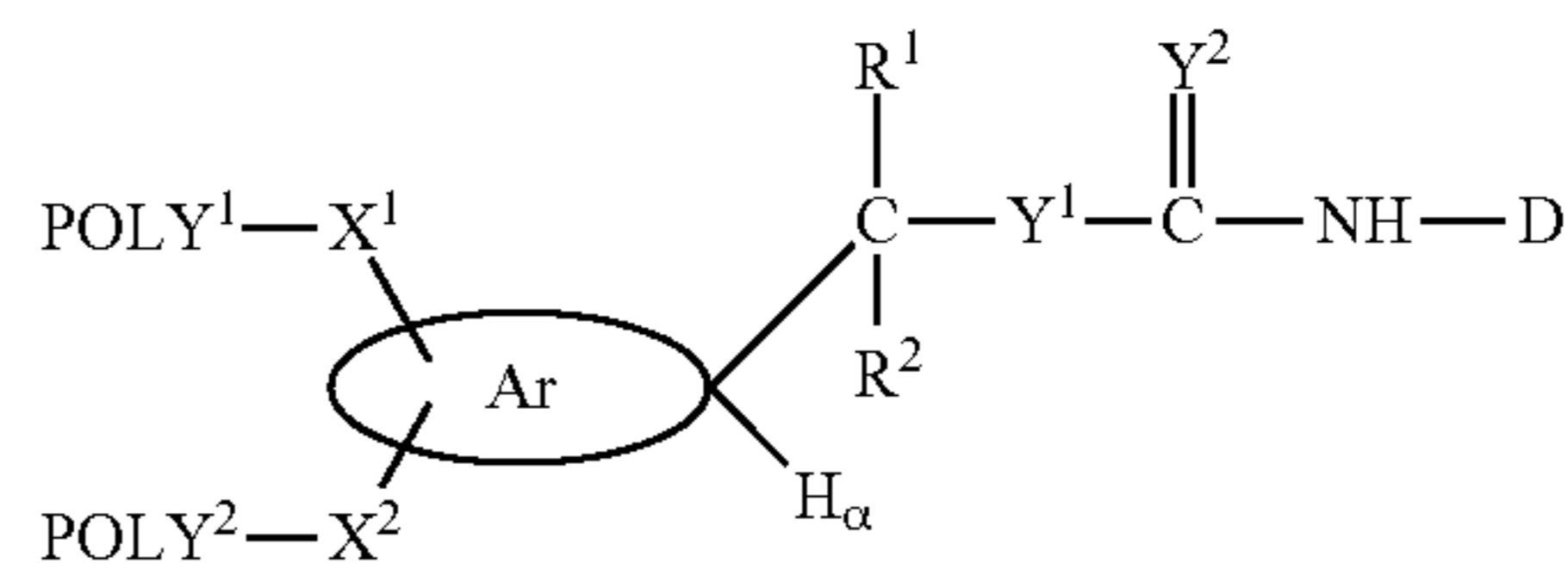
(Formula Ia-C)
