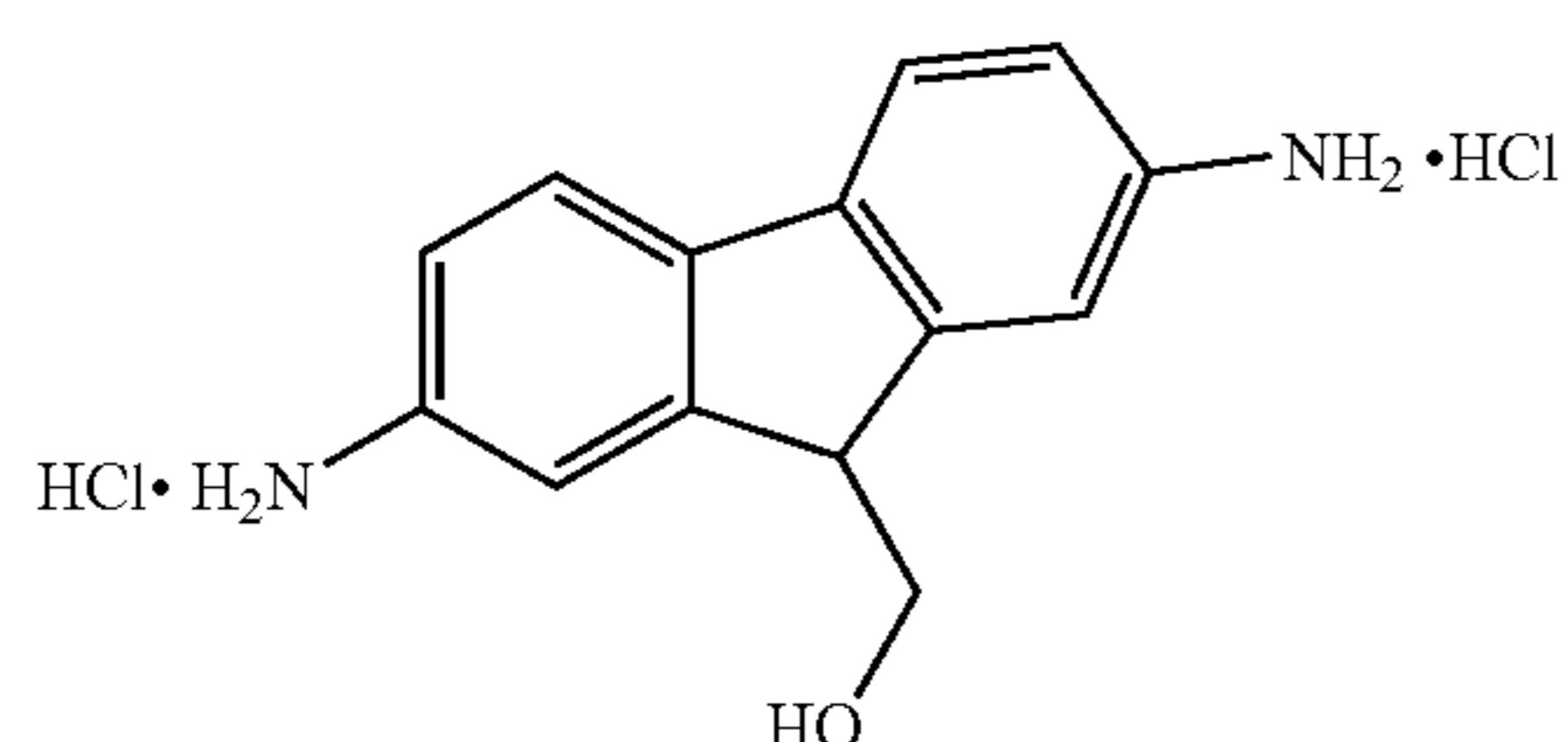
9-hydroxymethyl-2,7-diaminofluorene dihydrochloride
