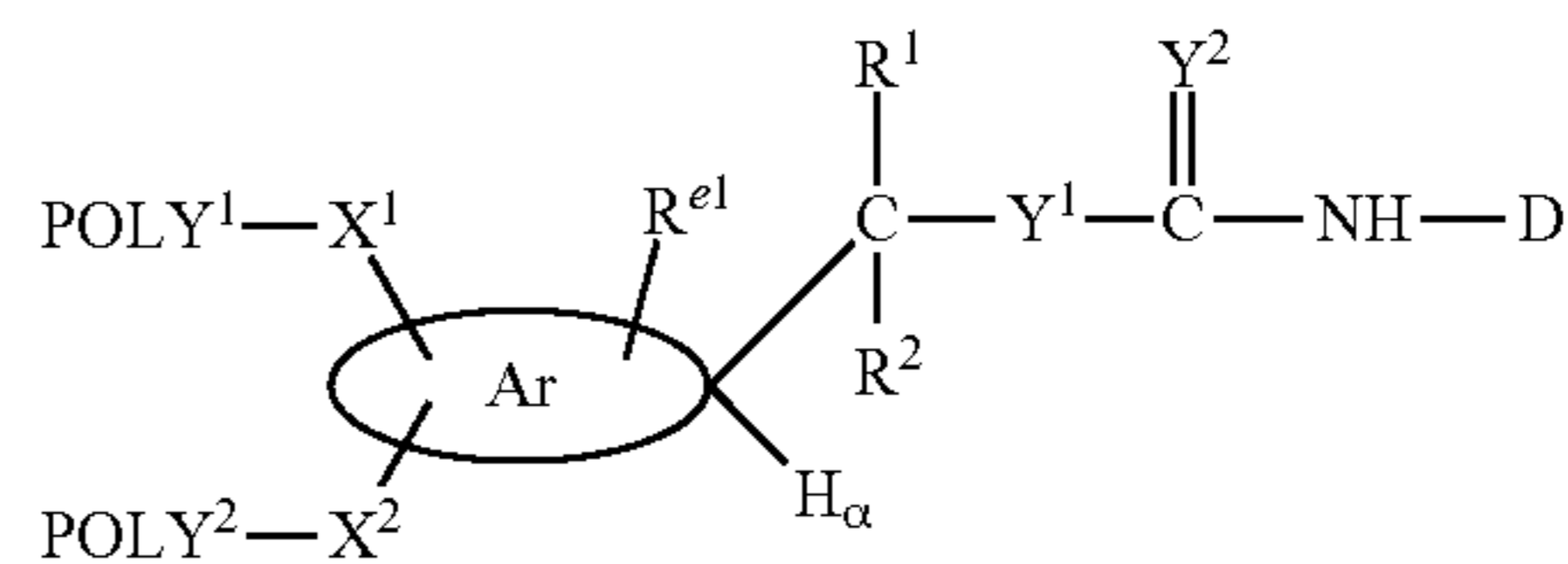
(Formula Ic-C)
