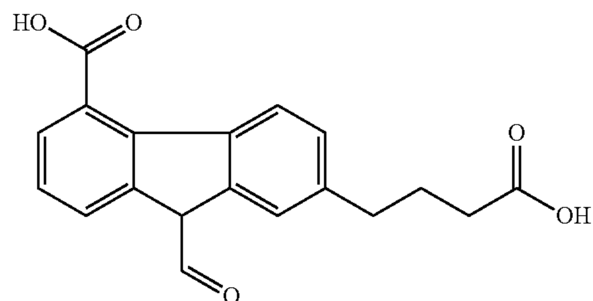
9-formyl-7-(3-carboxy-propyl)-4-fluorencarboxylic acid
