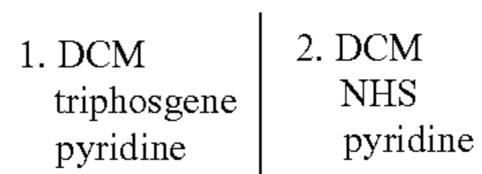
9-hydroxymethyl-4-(mPEG(10,000)-carboxamide)-7-(3-(mPEG(10,000))carbamoyl-propyl)fluorene
