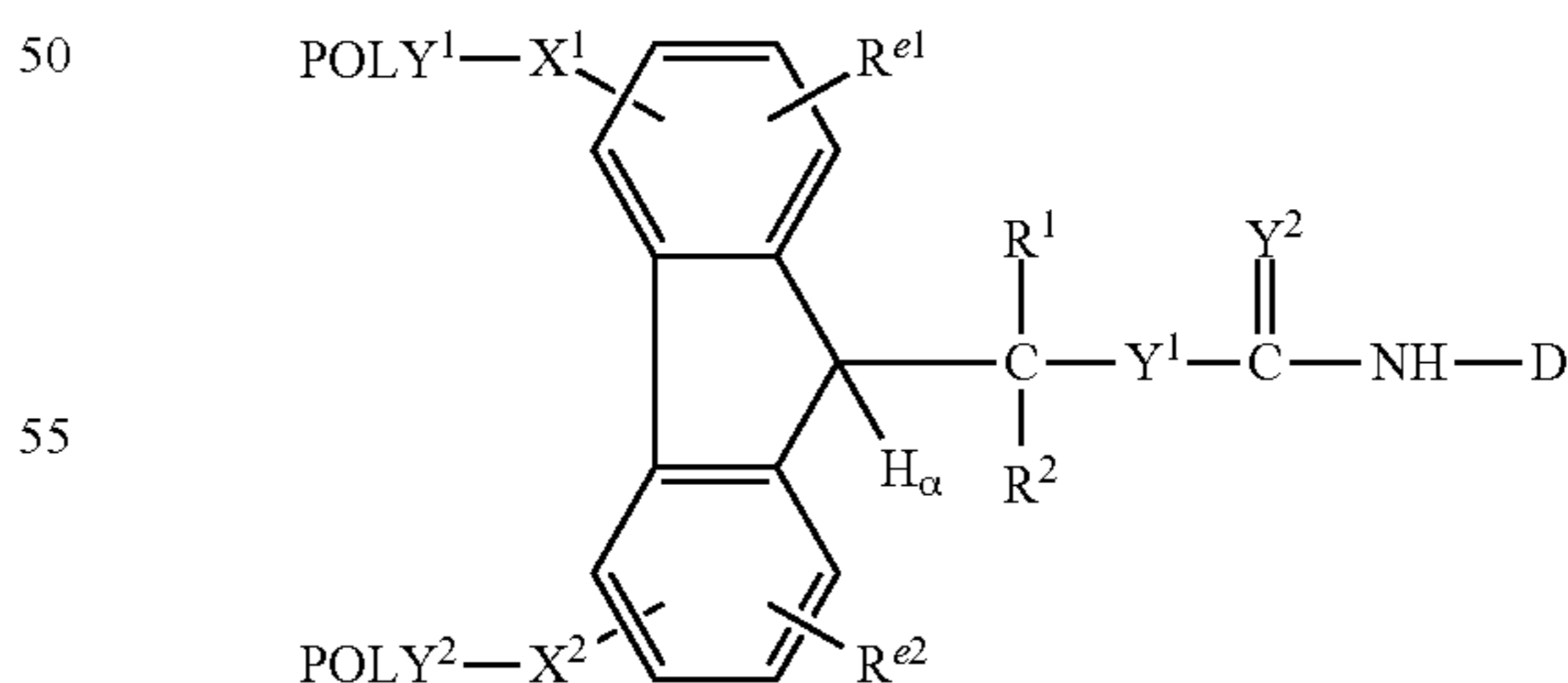
(Formula Vb-C)
