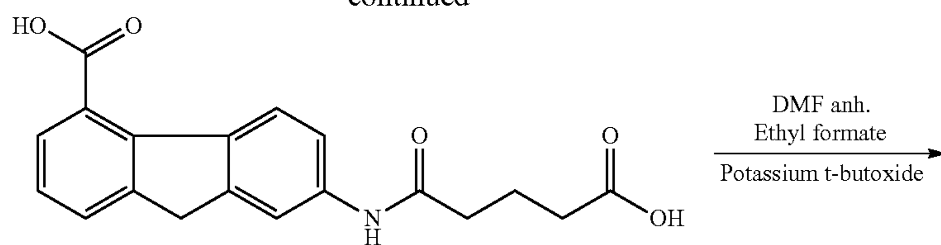
4-carboxylic acid-7-(amidoglutamic acid)fluorene
