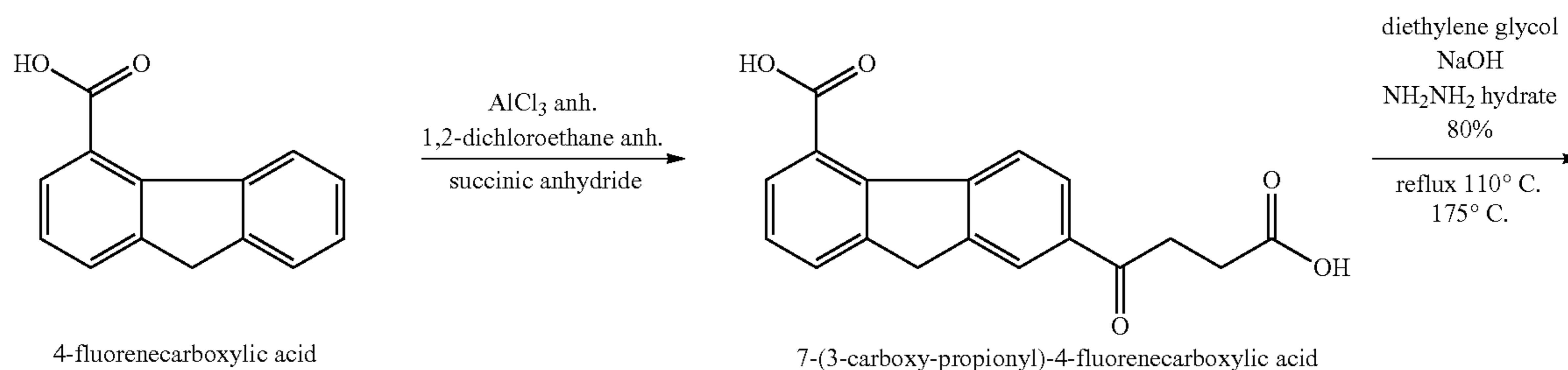
Scheme 4.
