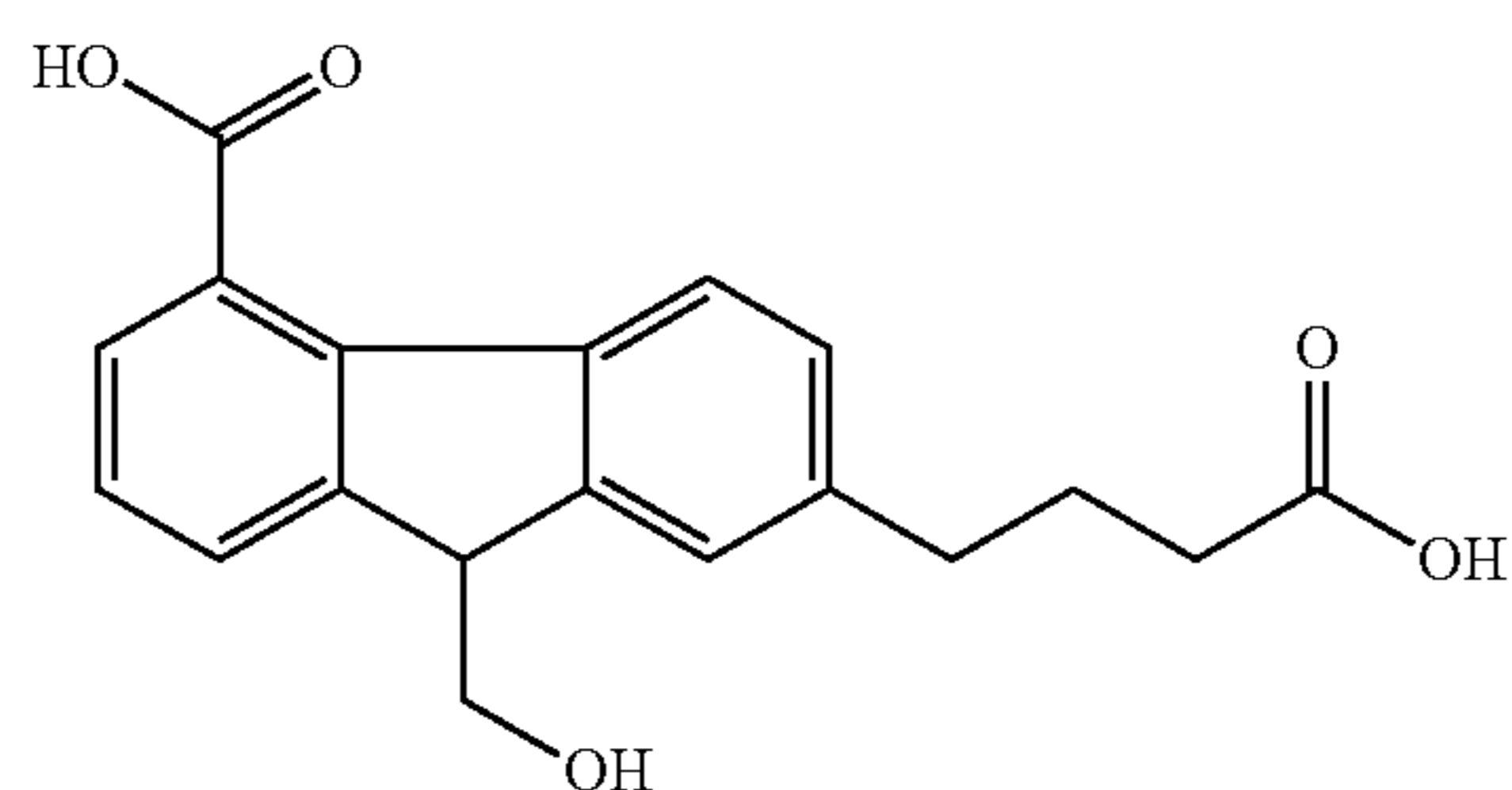
9-hydroxymethyl-7-(3-carboxy-propyl)-4-fluorencarboxylic acid
