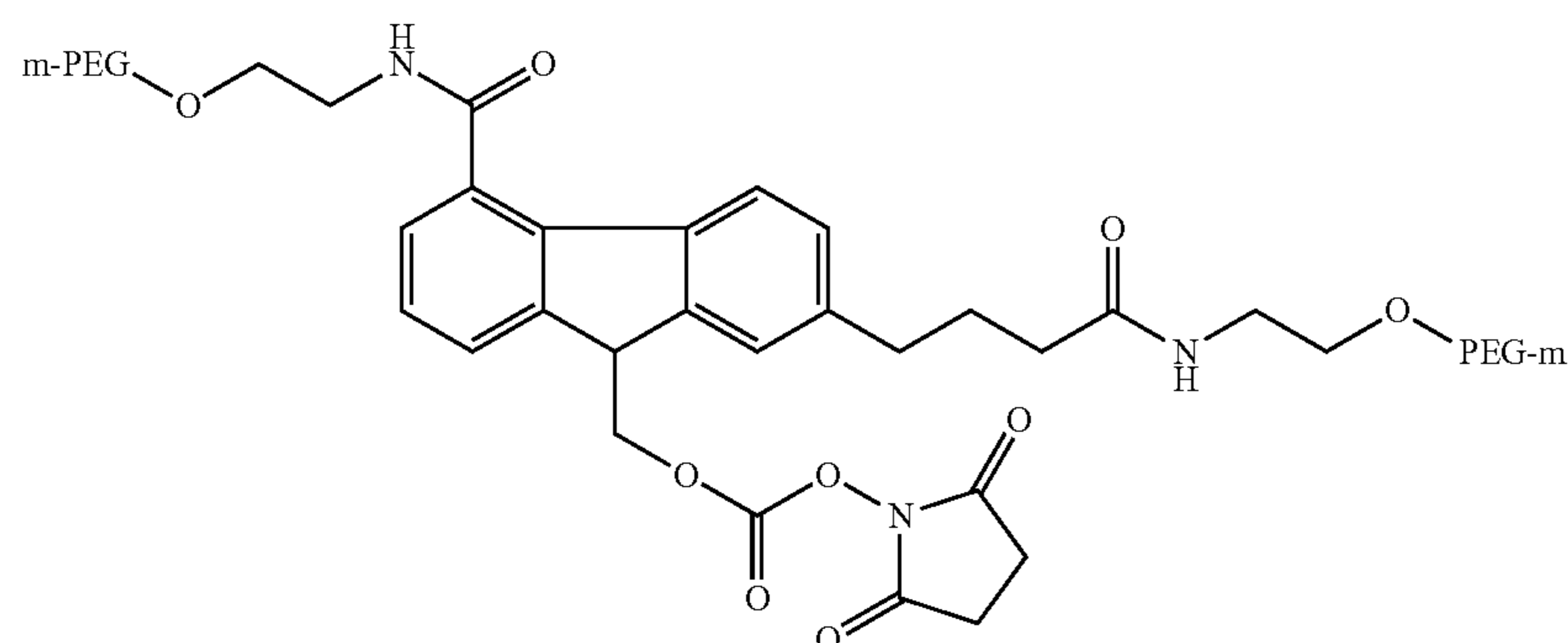
9-hydroxymethyl-4-(mPEG(10,000)-carboxamide)-7-(3-(mPEG(10,000))carbamoyl-propyl)fluorene-N-hydroxysuccinimide
