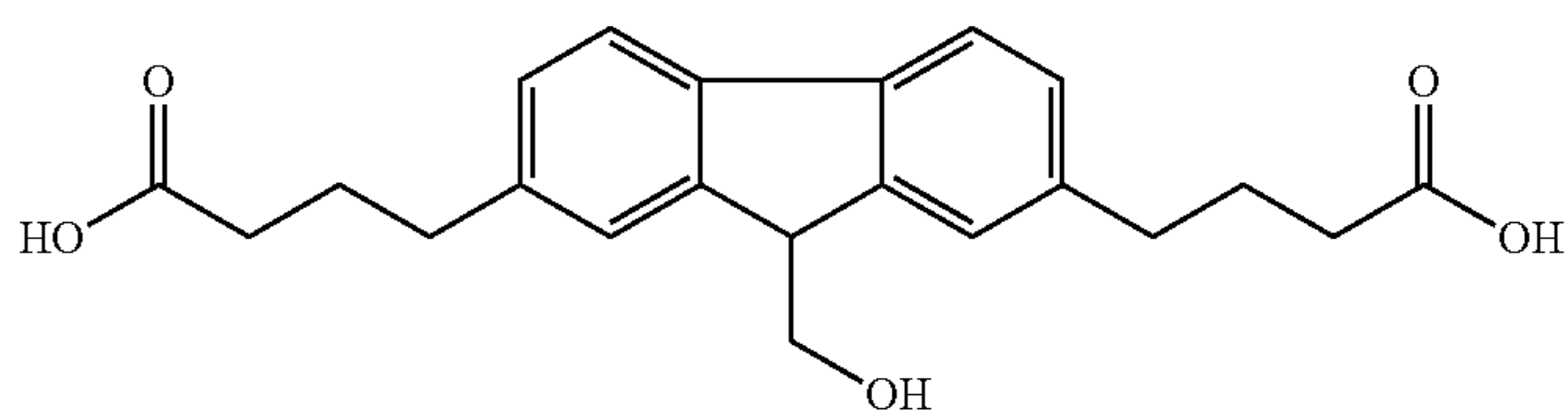
9-hydroxymethyl-2,7-di(3-carboxy-propyl)fluorene
