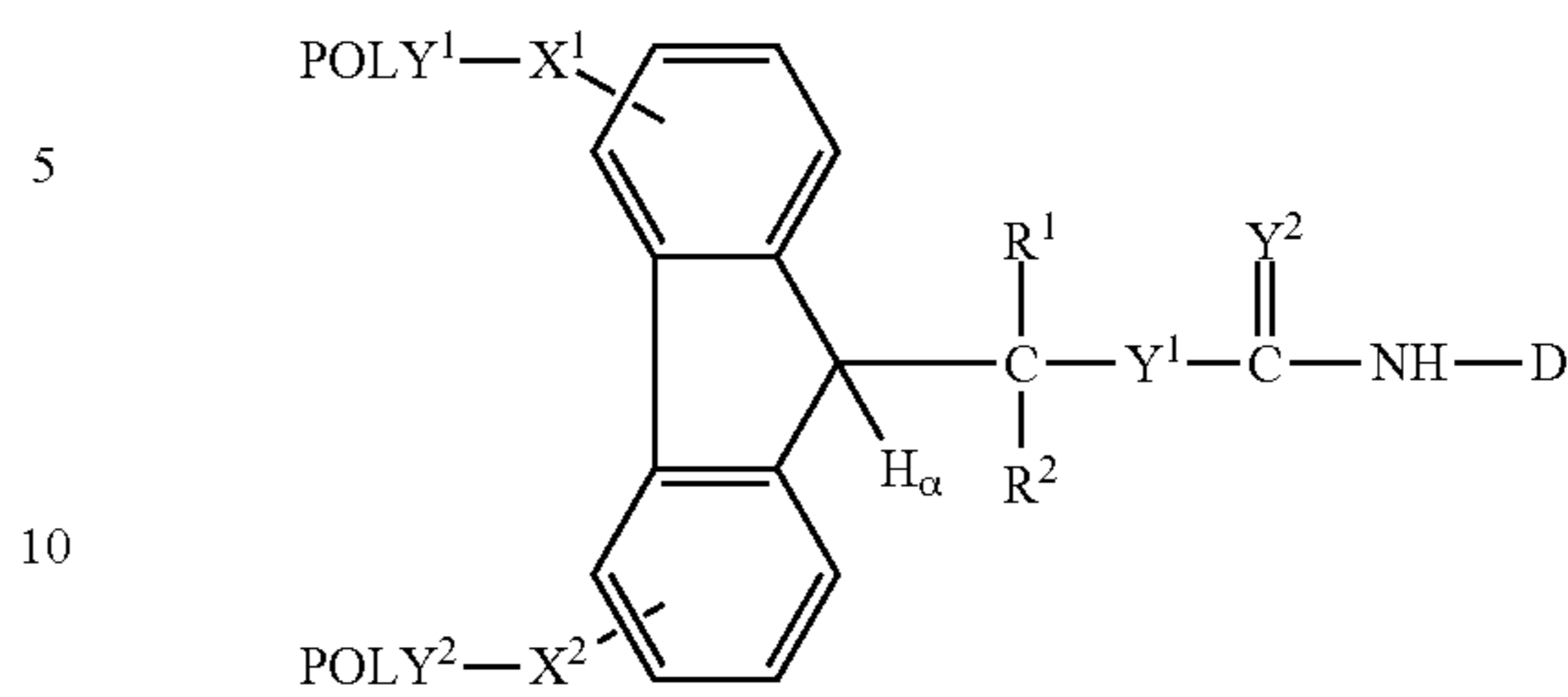
(Formula Va-C)
