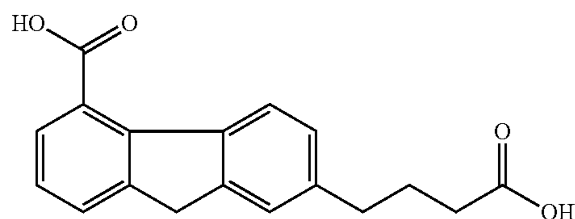
7-(3-carboxy-propyl)-4-fluorencarboxylic acid
