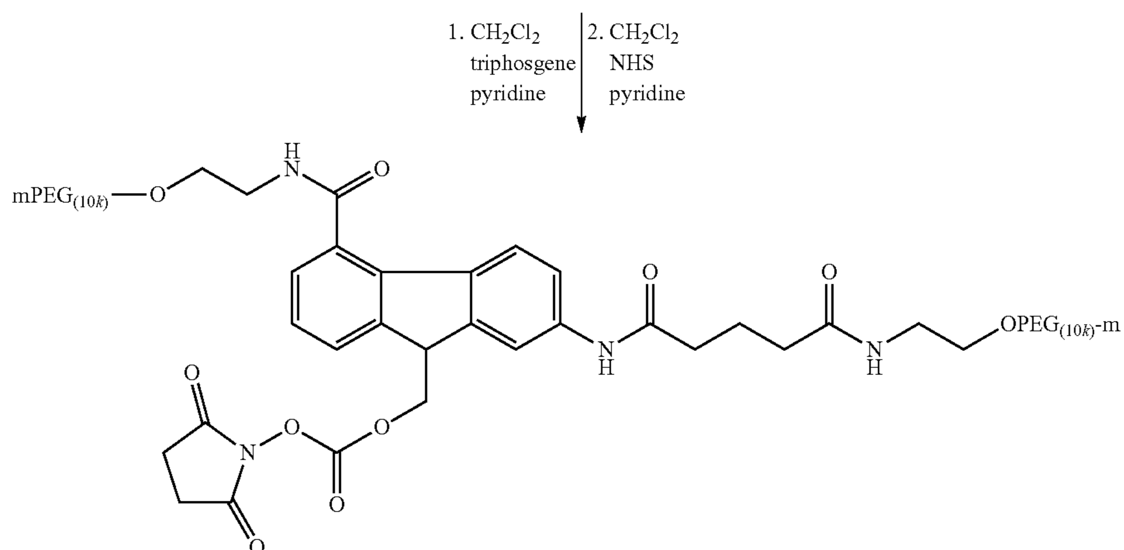
9-hydroxymethyl-4-(mPEG(10,000)-carboxyamide)-7-(mPEG(10,000)-amidoglutamic acid)fluorene-N-hydroxysuccinimide
