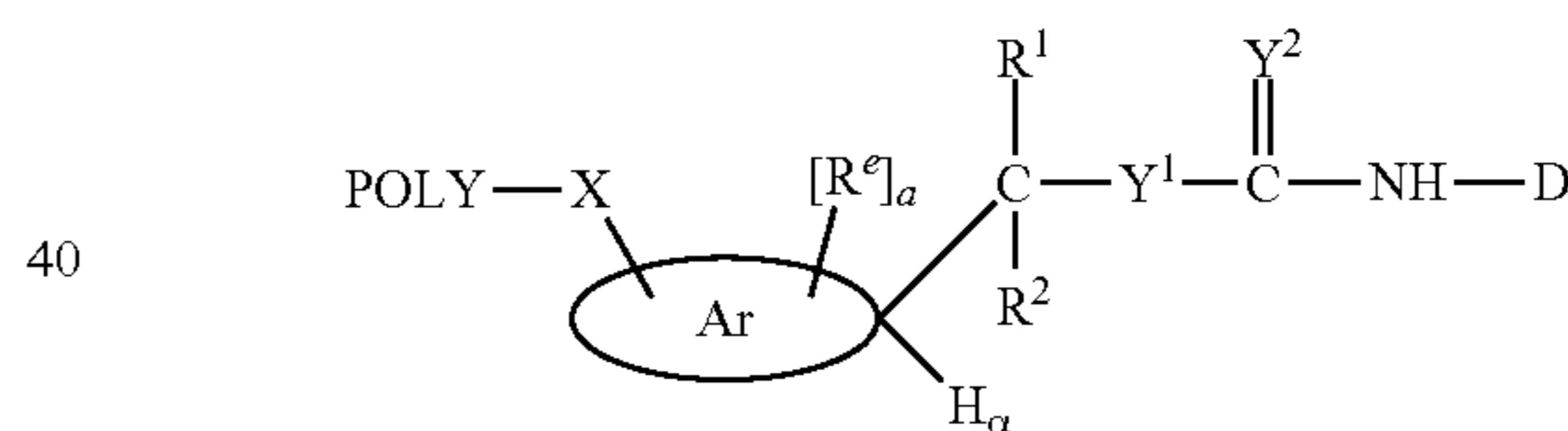
(Formula VI-C)
