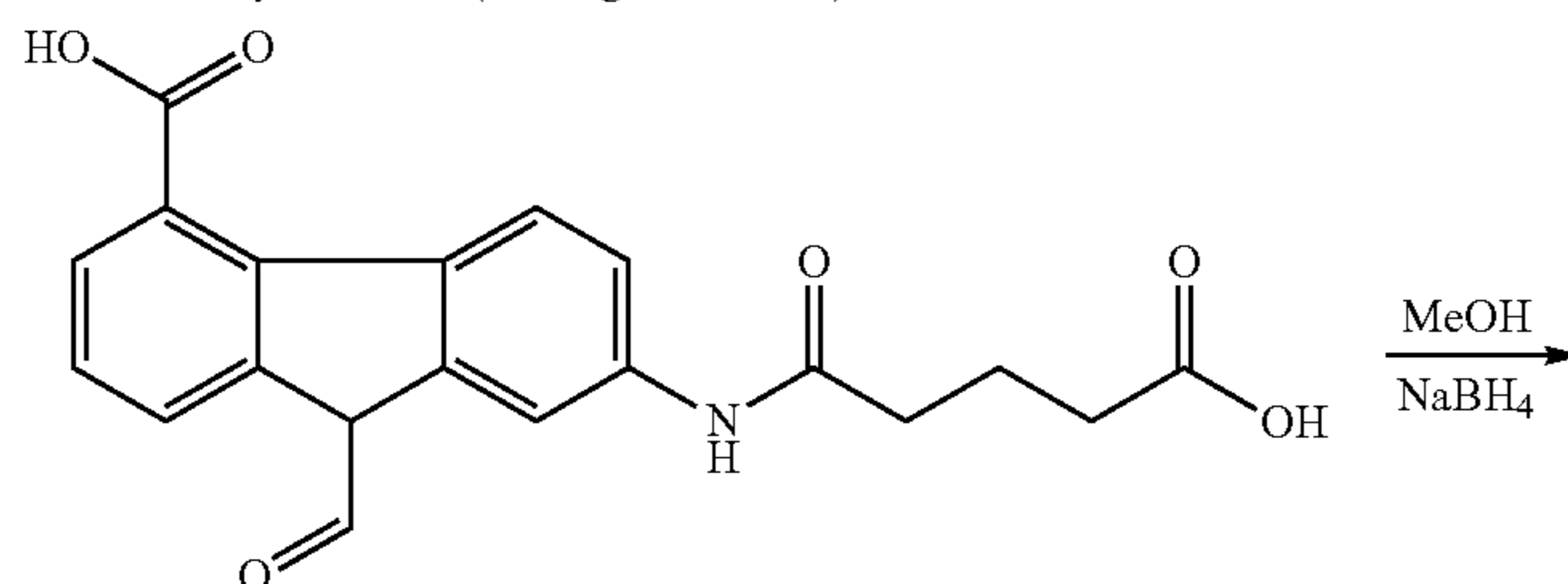
9-formyl-4-carboxylic acid-7-(amidoglutamic acid)fluorene
