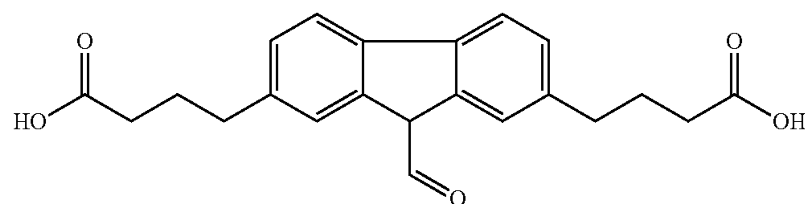
9-formyl-2,7-di(3-carboxy-propyl)fluorene
