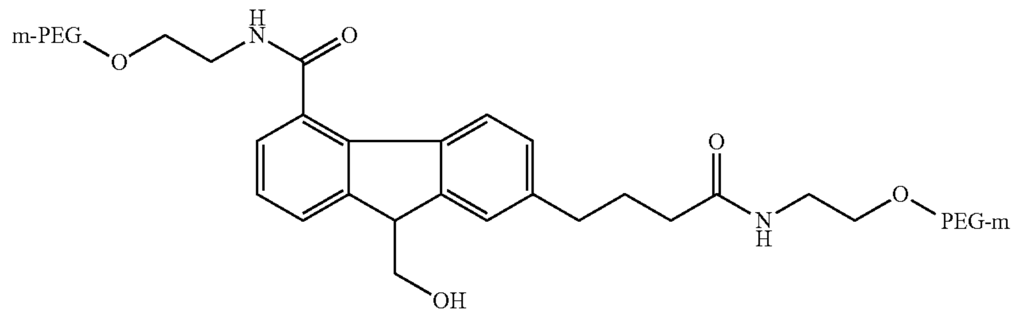
9-hydroxymethyl-4-(mPEG(10,000)-carboxamide)-7-(3-(mPEG(10,000))carbamoyl-propyl)fluorene
