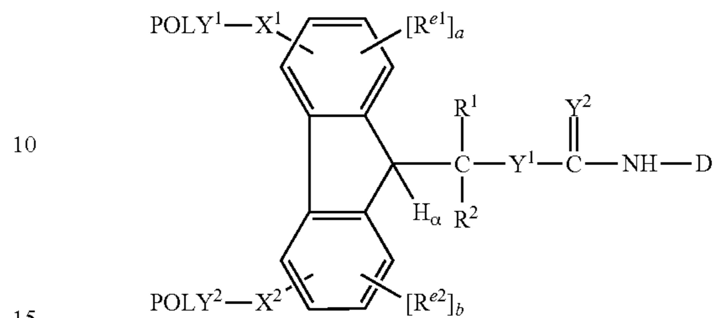
(Formula V-C)
