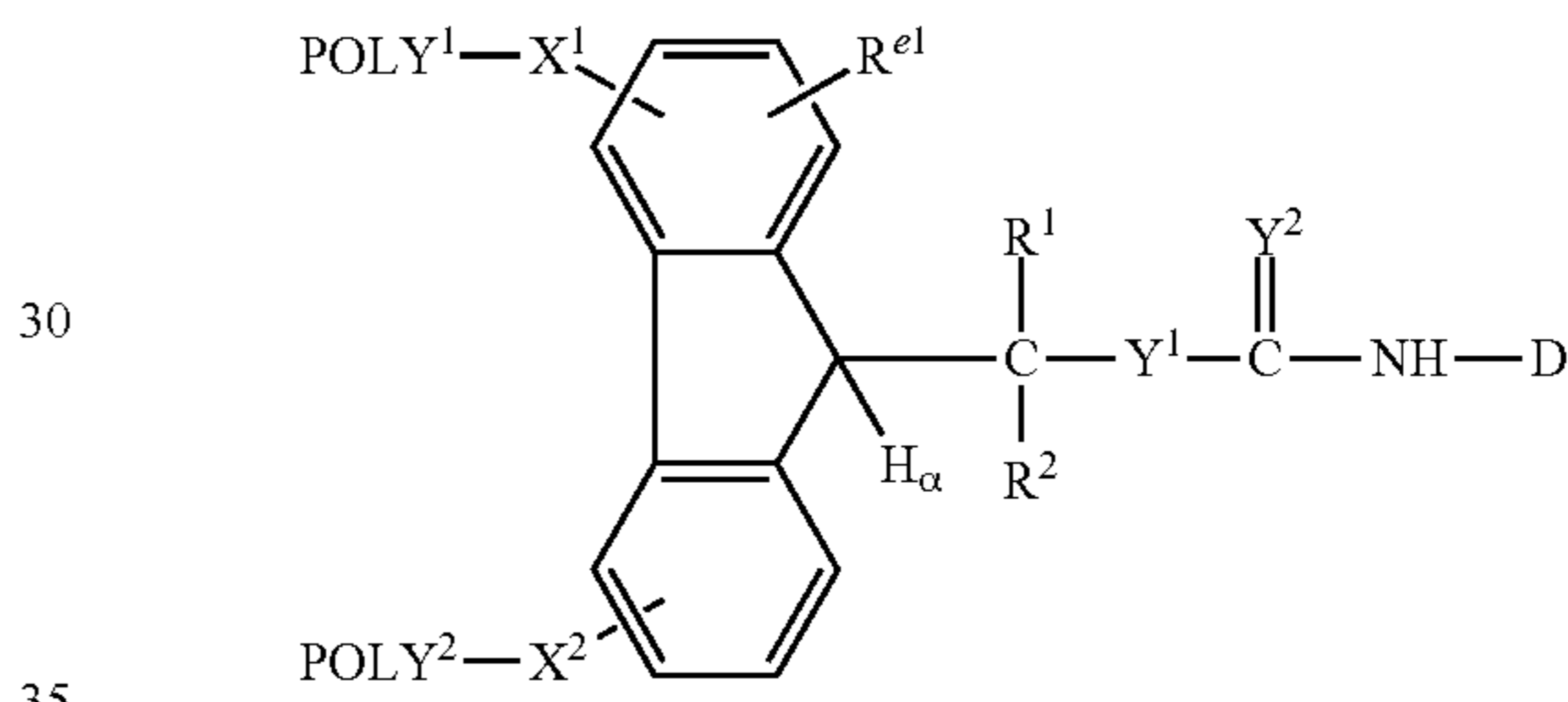
(Formula Vc-C)
