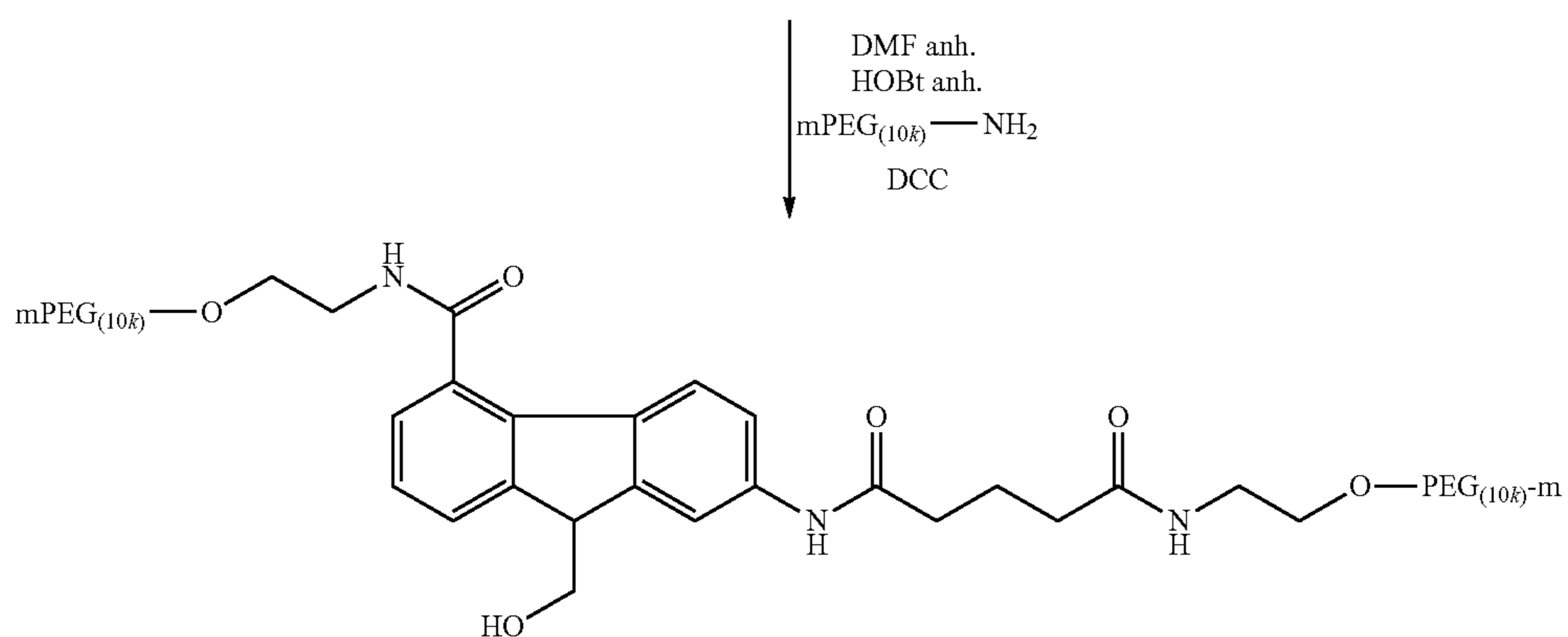
9-hydroxymethyl-4-(mPEG(10,000)-carboxyamide)-7-(mPEG(10,000)-amidoglutamic acid)fluorene
