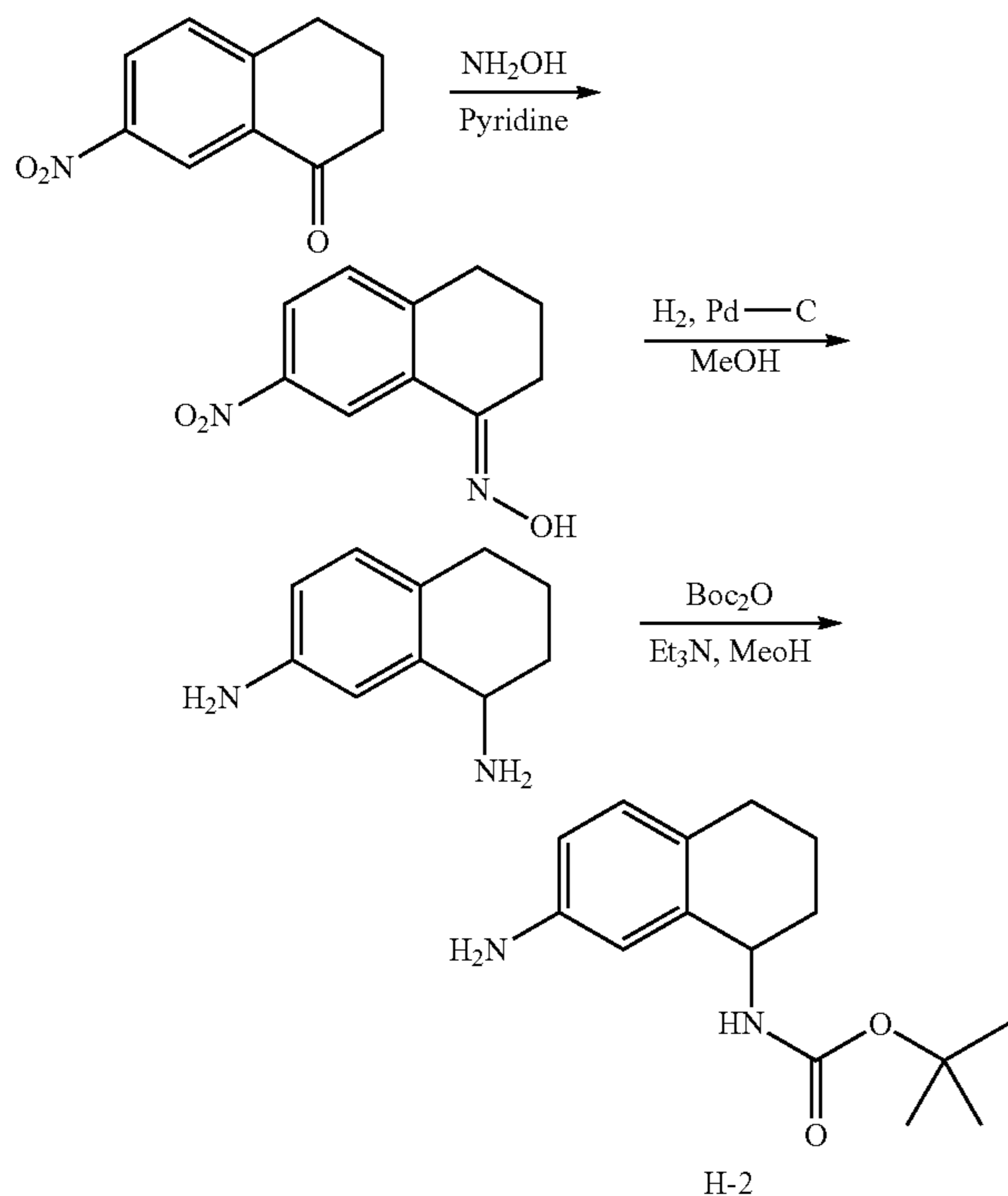
7-Nitro-3,4-dihydro-2H-naphthalen-1-one oxime
