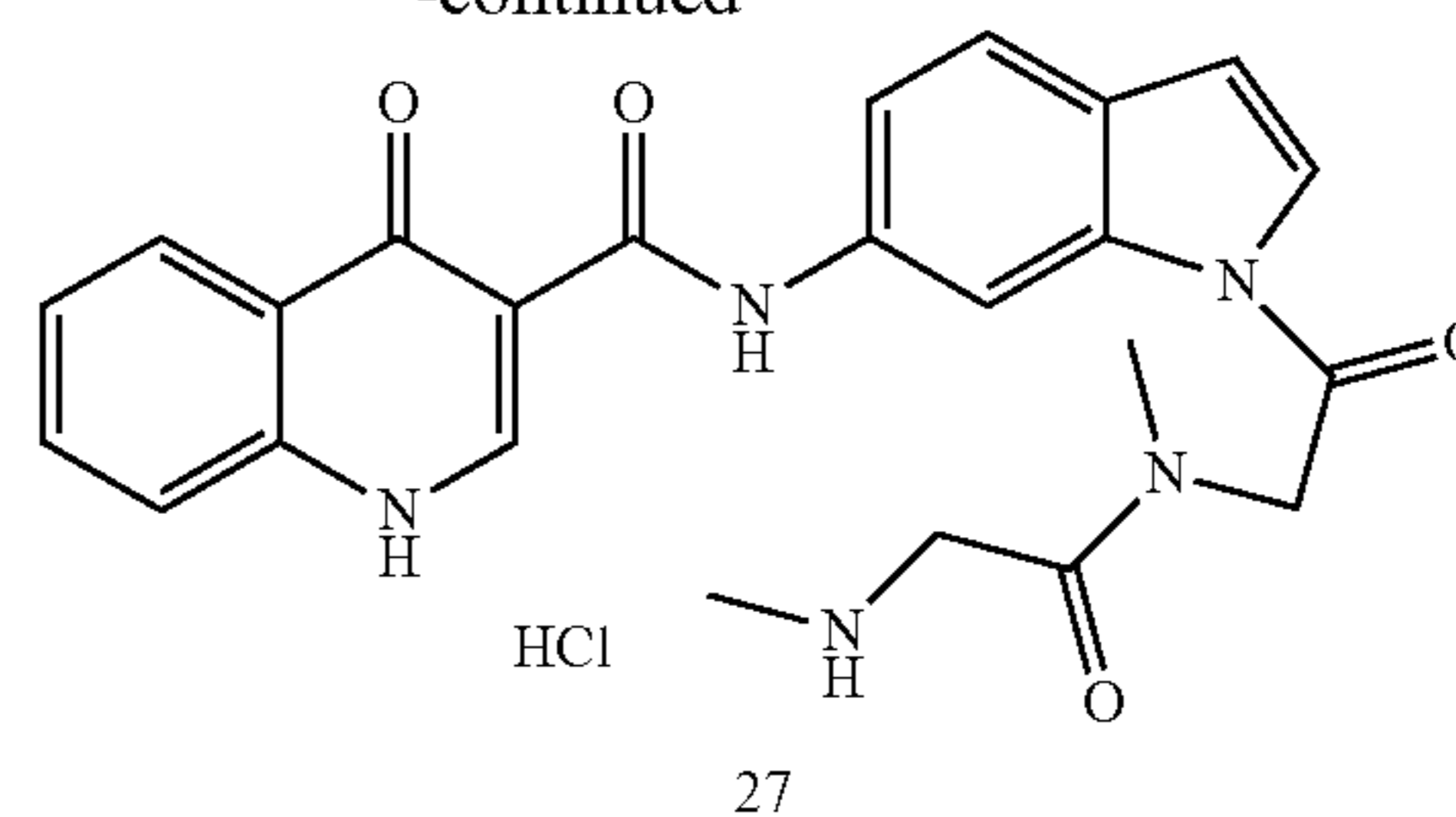
27; N-[1-[2-[Methyl-(2-methylaminoacetyl)-amino]acetyl]-1H-indol-6-yl]-4-oxo-1H-quinoline-3-carboxamide
