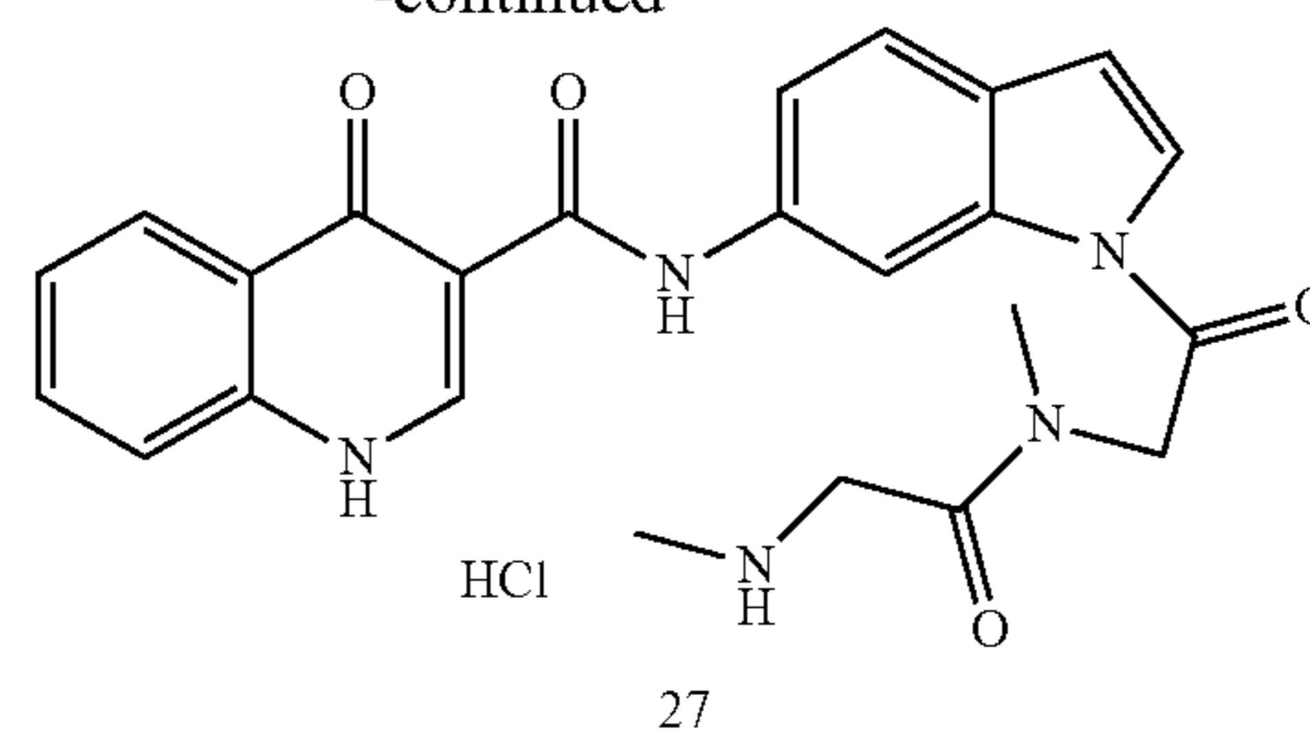
27; N-[1-[2-[Methyl-(2-methylaminoacetyl)-amino]acetyl]-1H-indol-6-yl]-4-oxo-1H-quinoline-3-carboxamide
