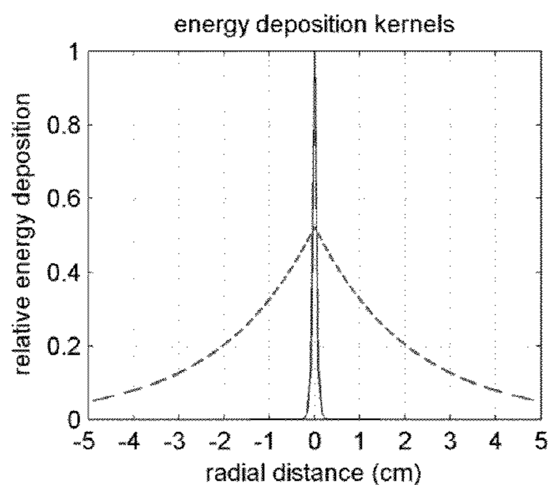
Diagram of energy deposition kernels.
