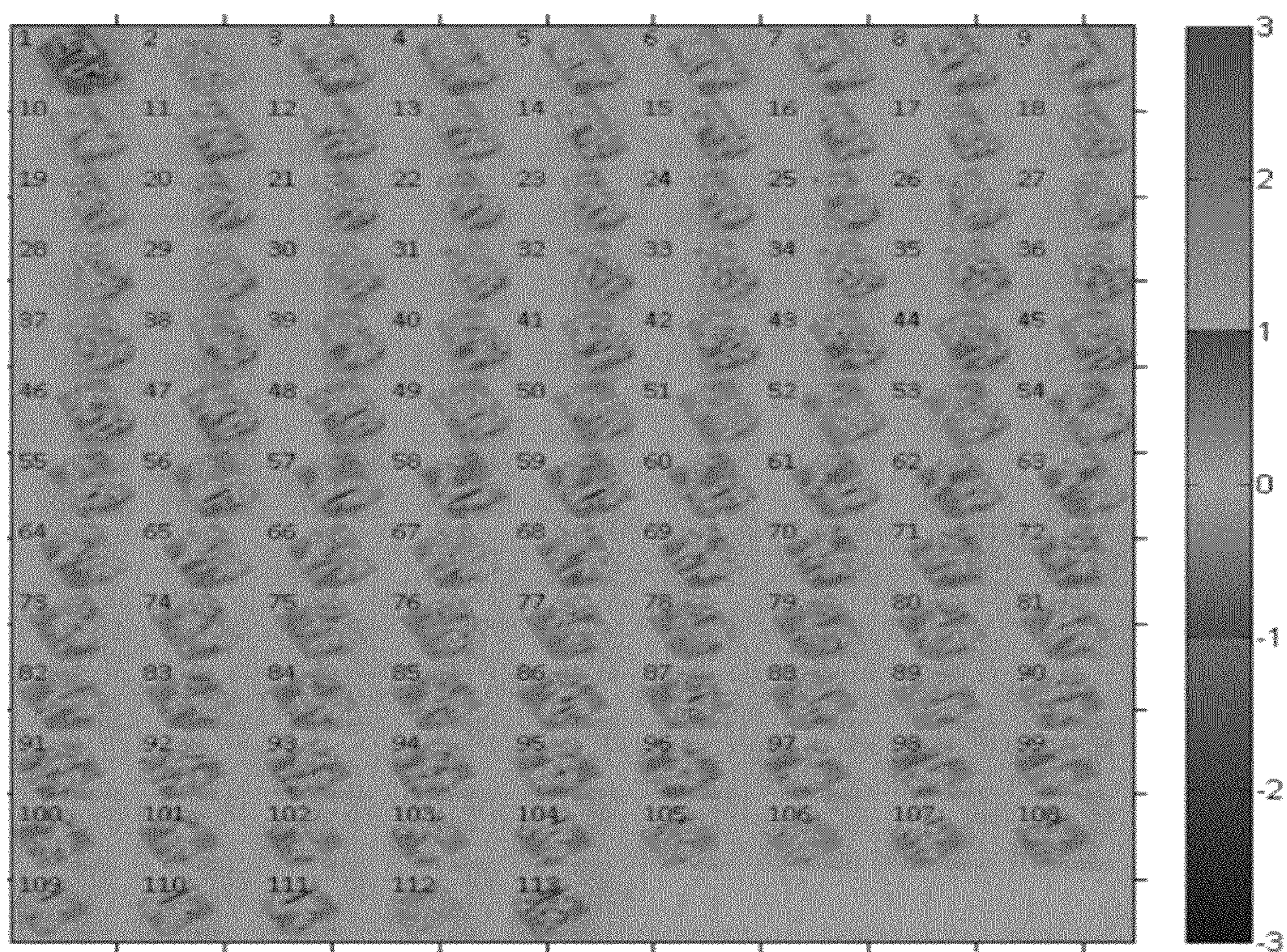
Gamma distributions (3%, 3mm, 3sec) between measurement and prediction of the differential (per CP) 2D portal dose images for a single 6MV FFF VMAT arc.
