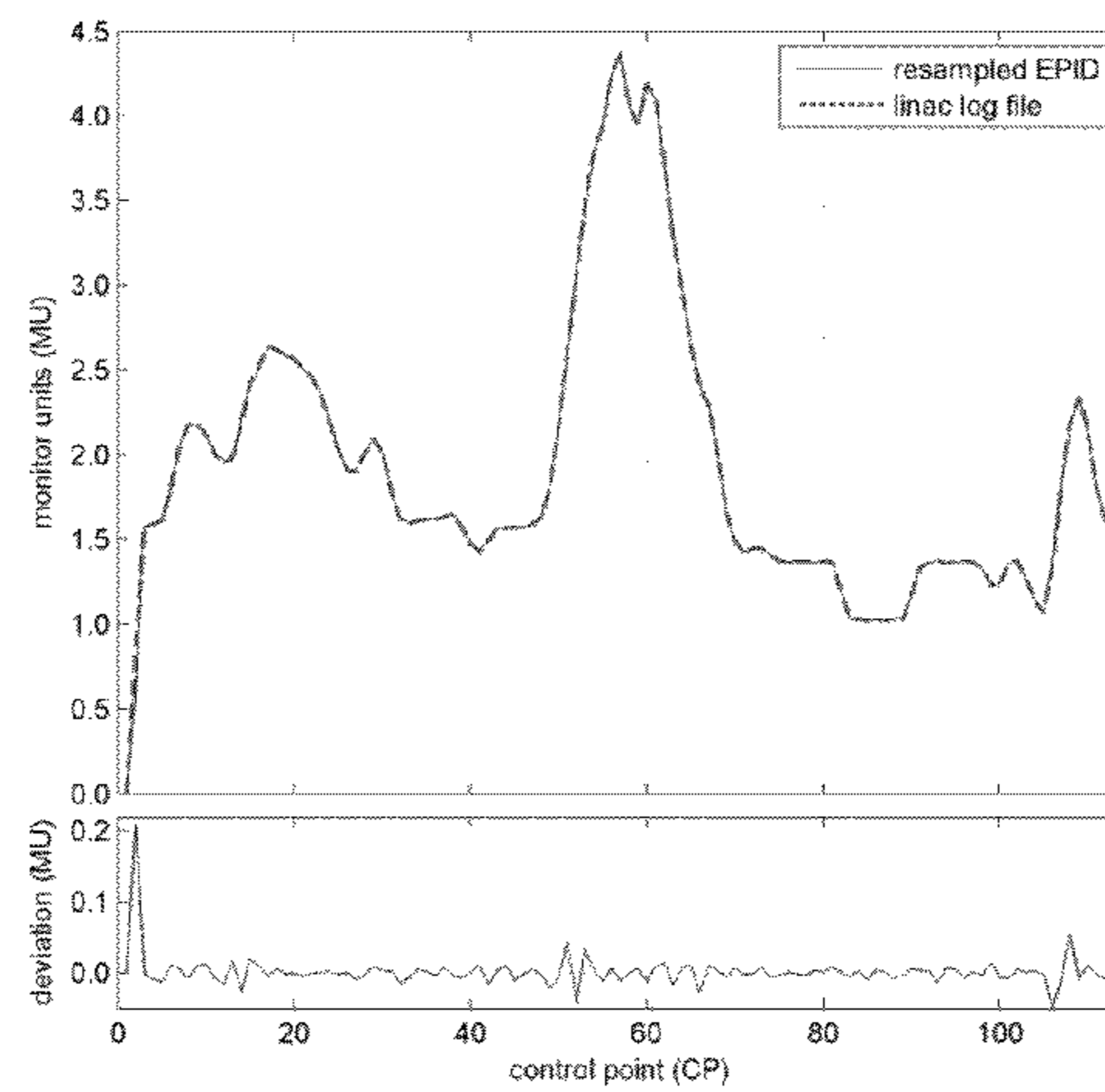
CP resampling MU check. The solid line is the resampled EPID header values. The dashed line is the linac log file values, the deviation from the log file is shown in the bottom panel.
