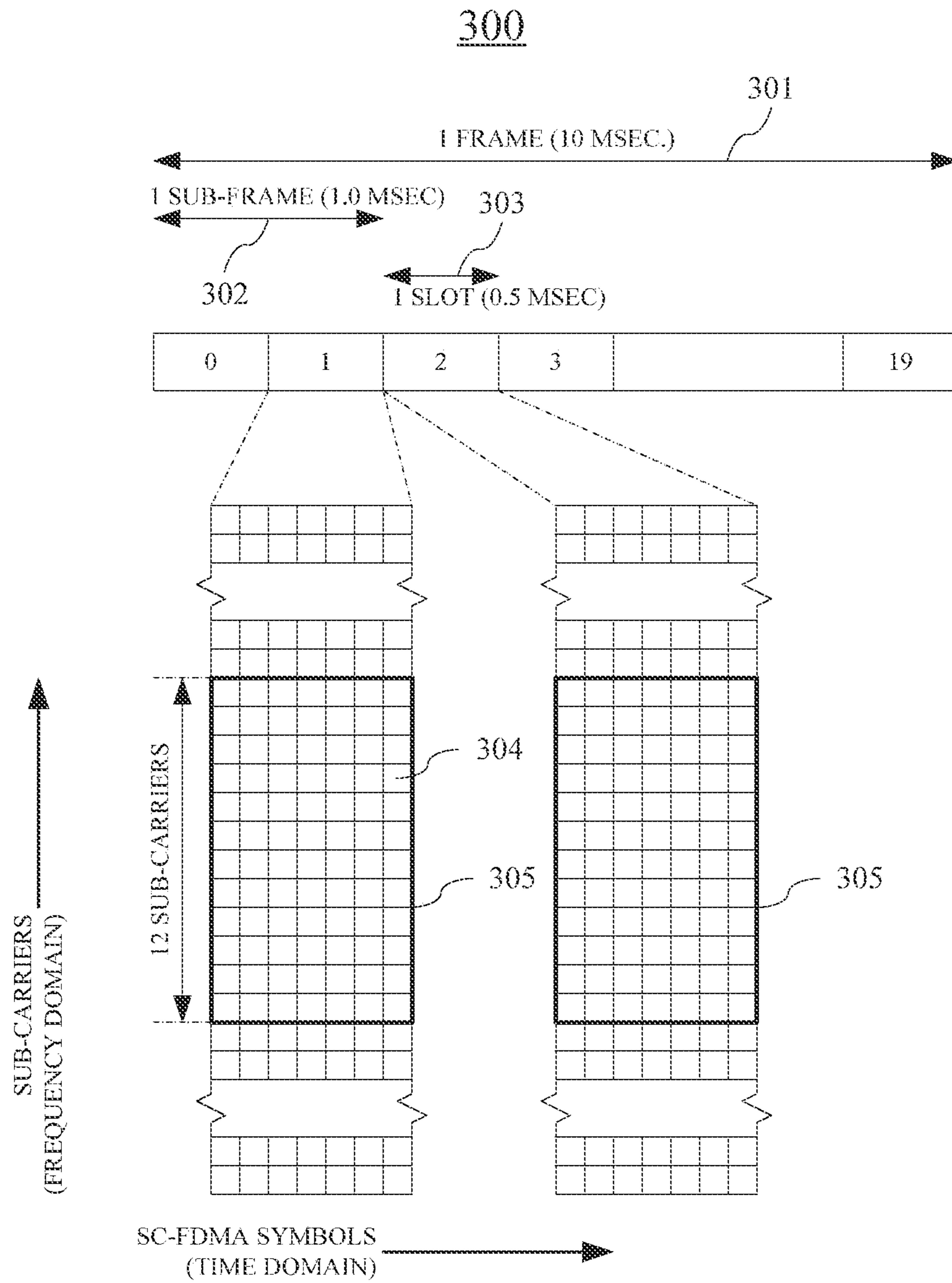
FIG. 3 (PRIOR ART)
