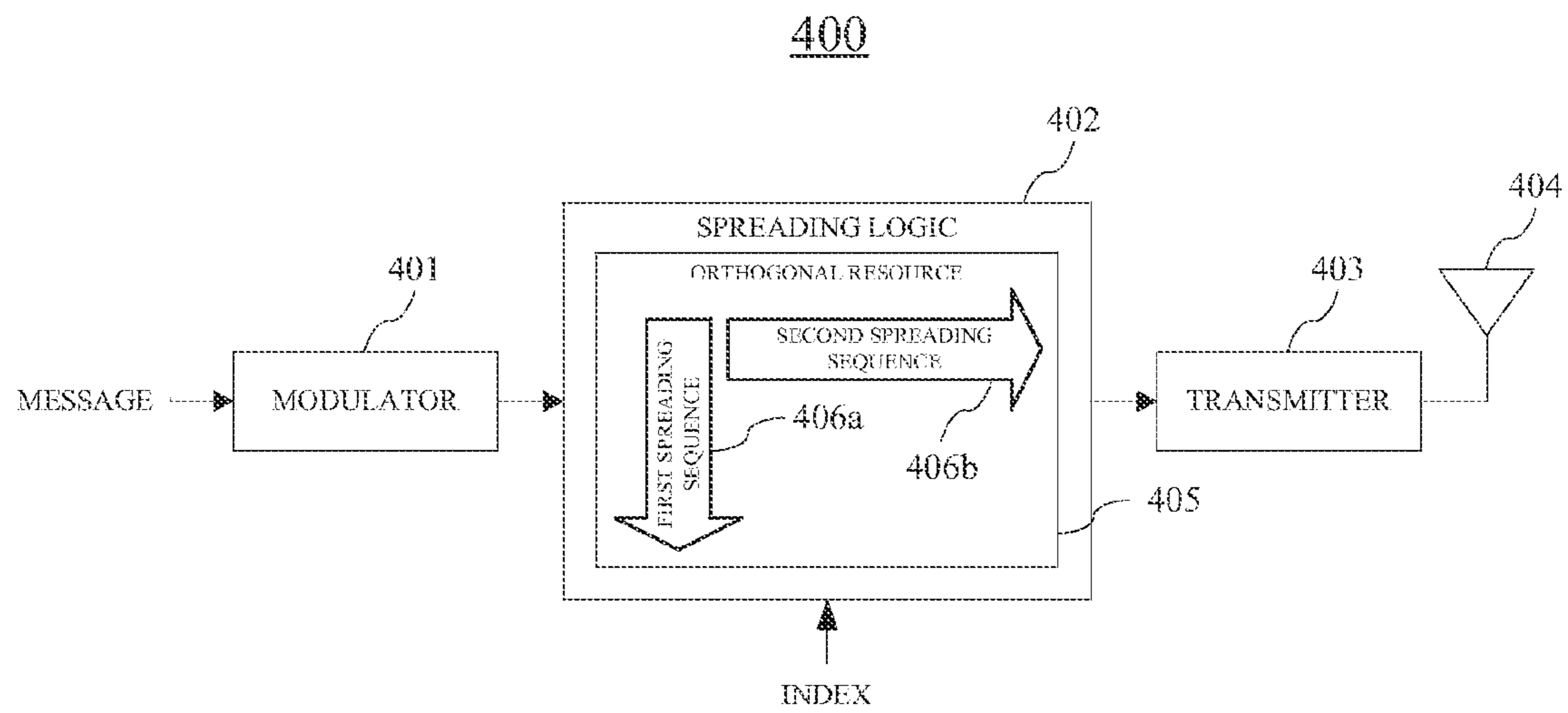
FIG. 4 (PRIOR ART)
