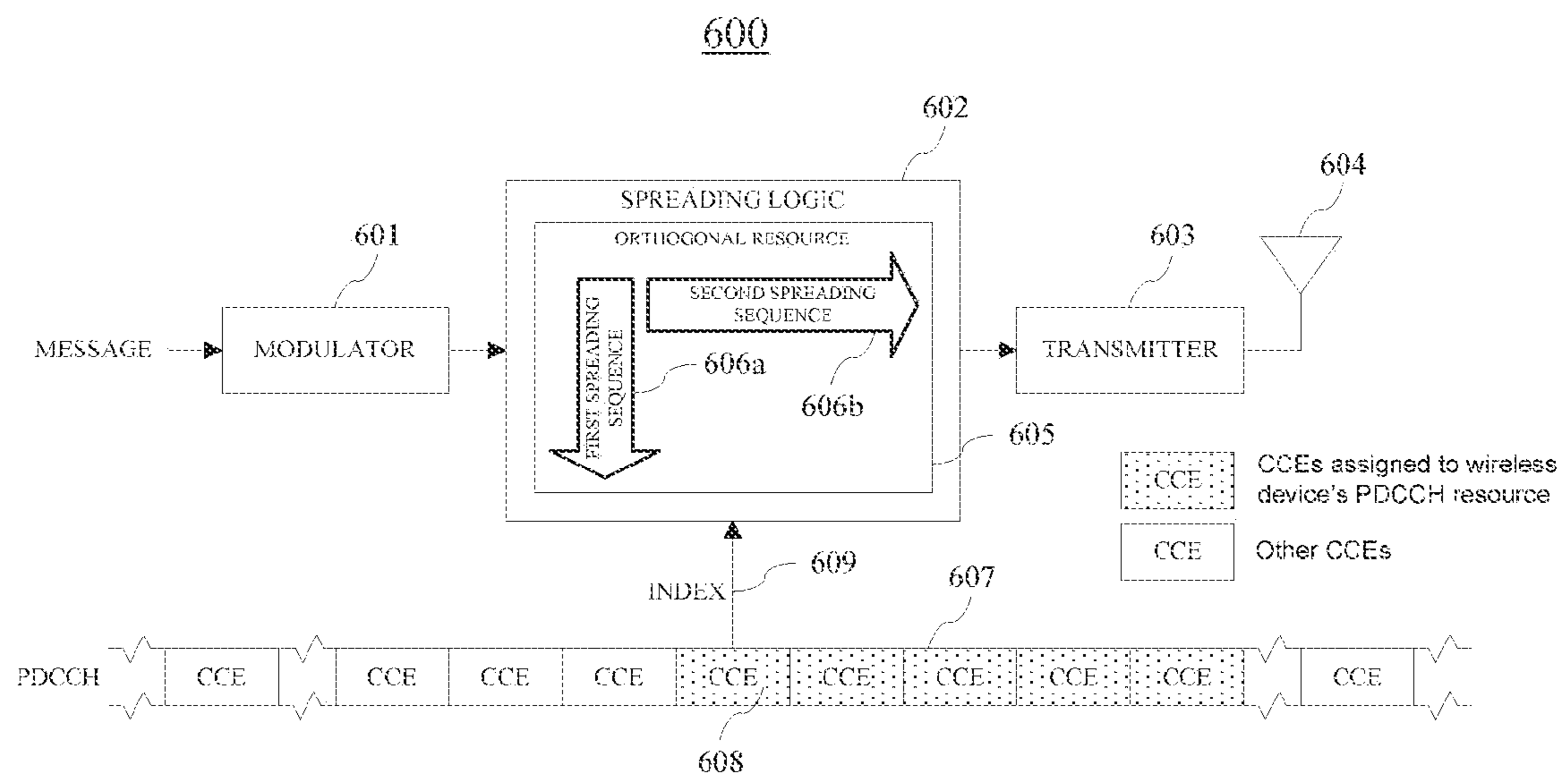
FIG. 6 (PRIOR ART)
