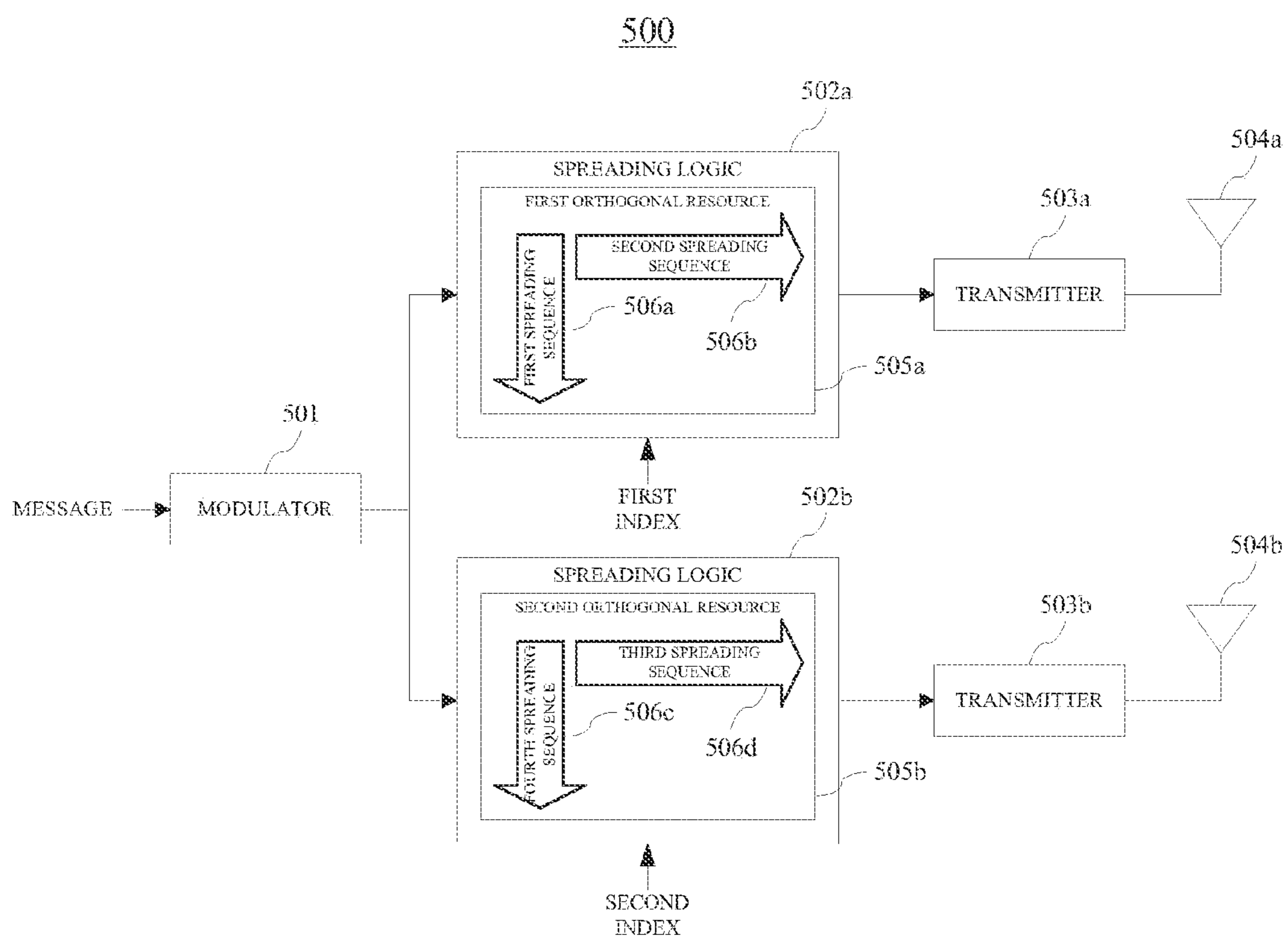
FIG. 5 (PRIOR ART)
