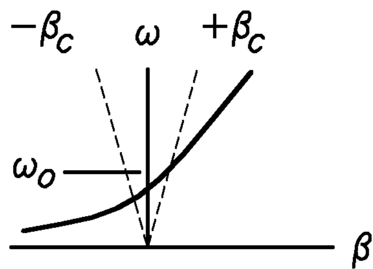
Composite (CRLH)
