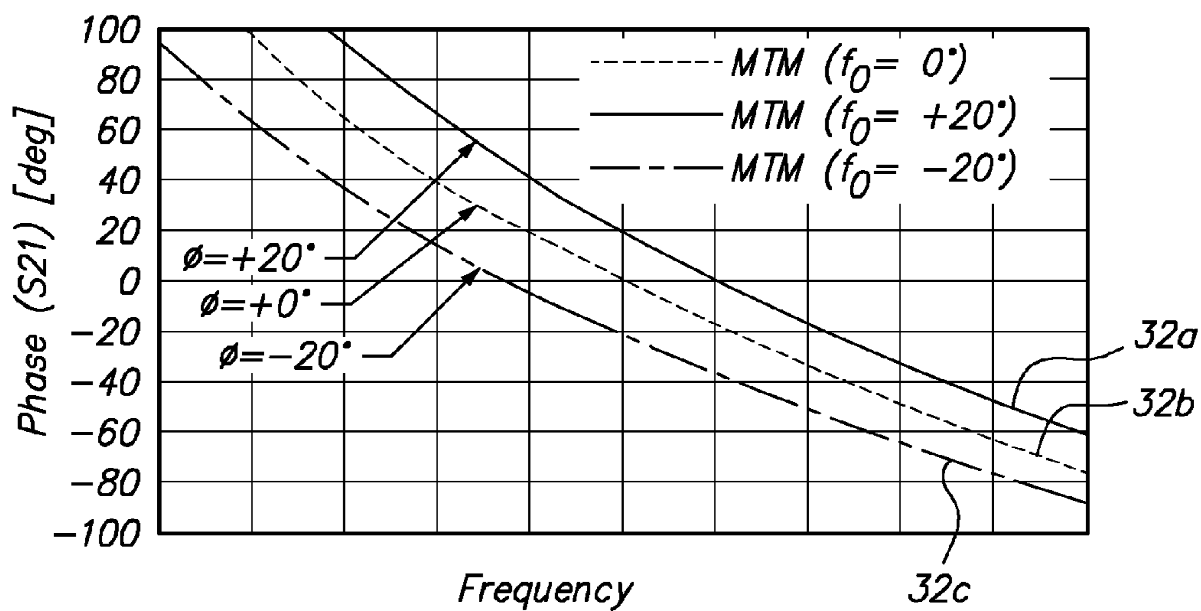
FIG. 3 (PRIOR ART)
