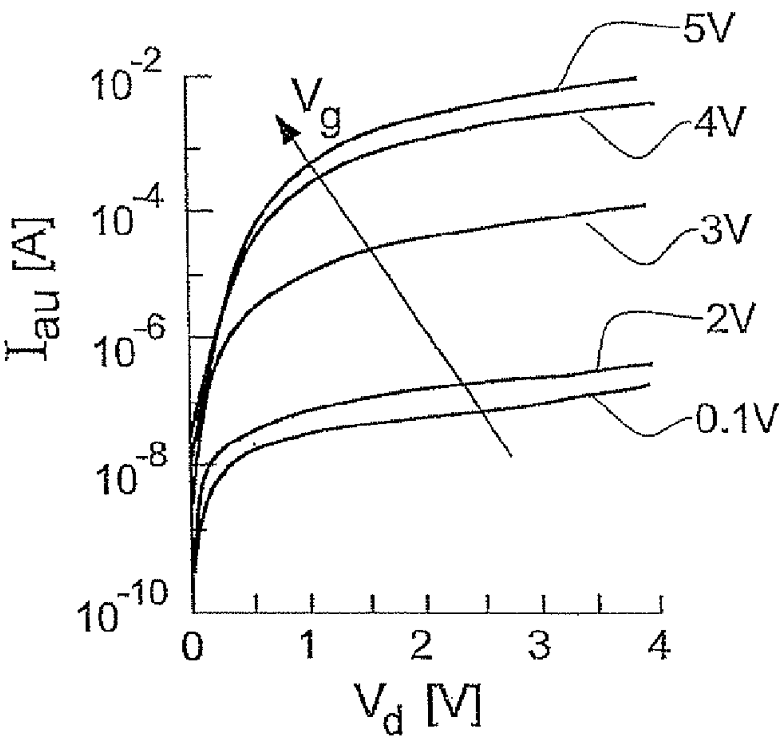
FIG. 1C (PRIOR ART)
