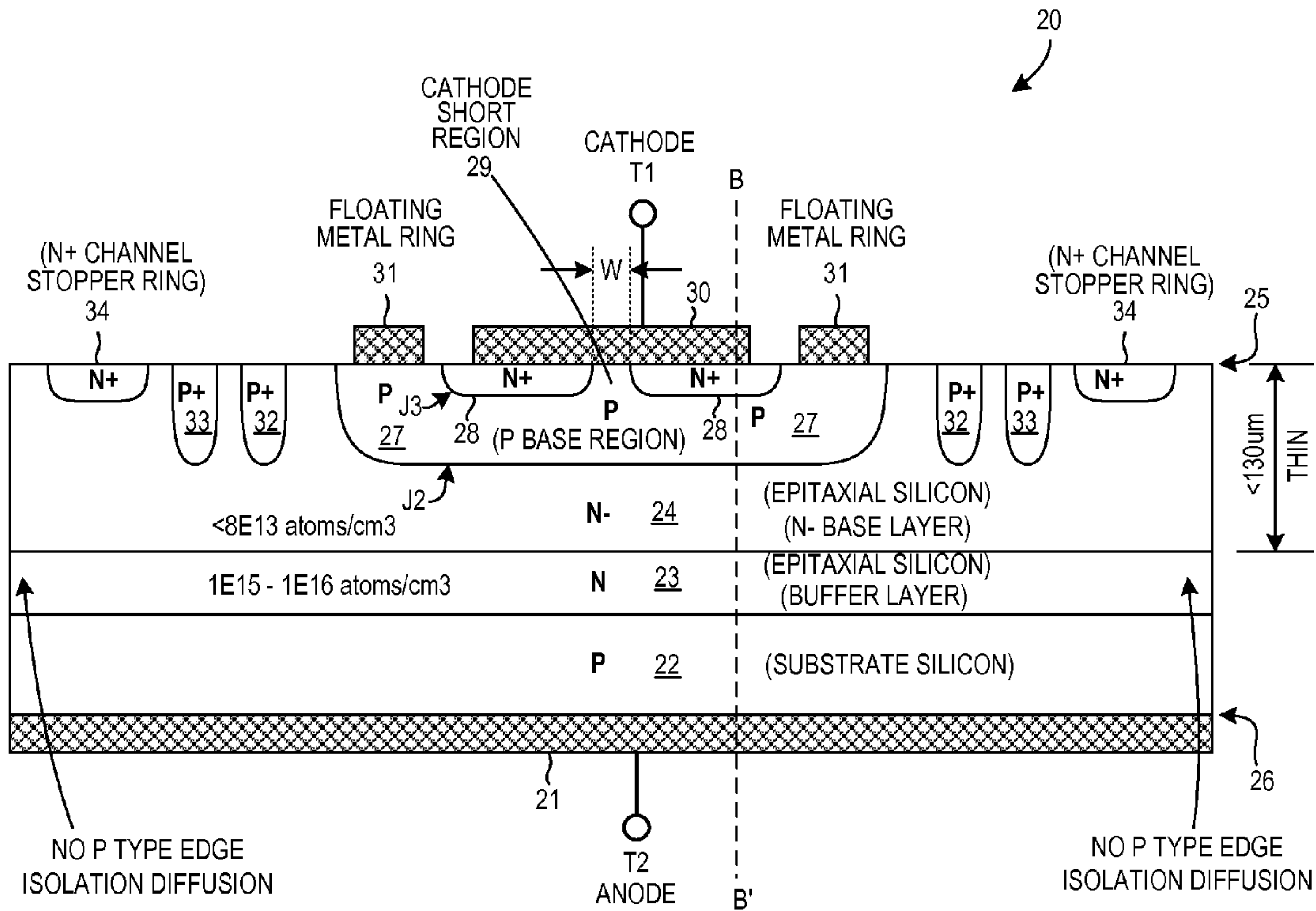
BREAKOVER DIODE DEVICE FIG. 7
