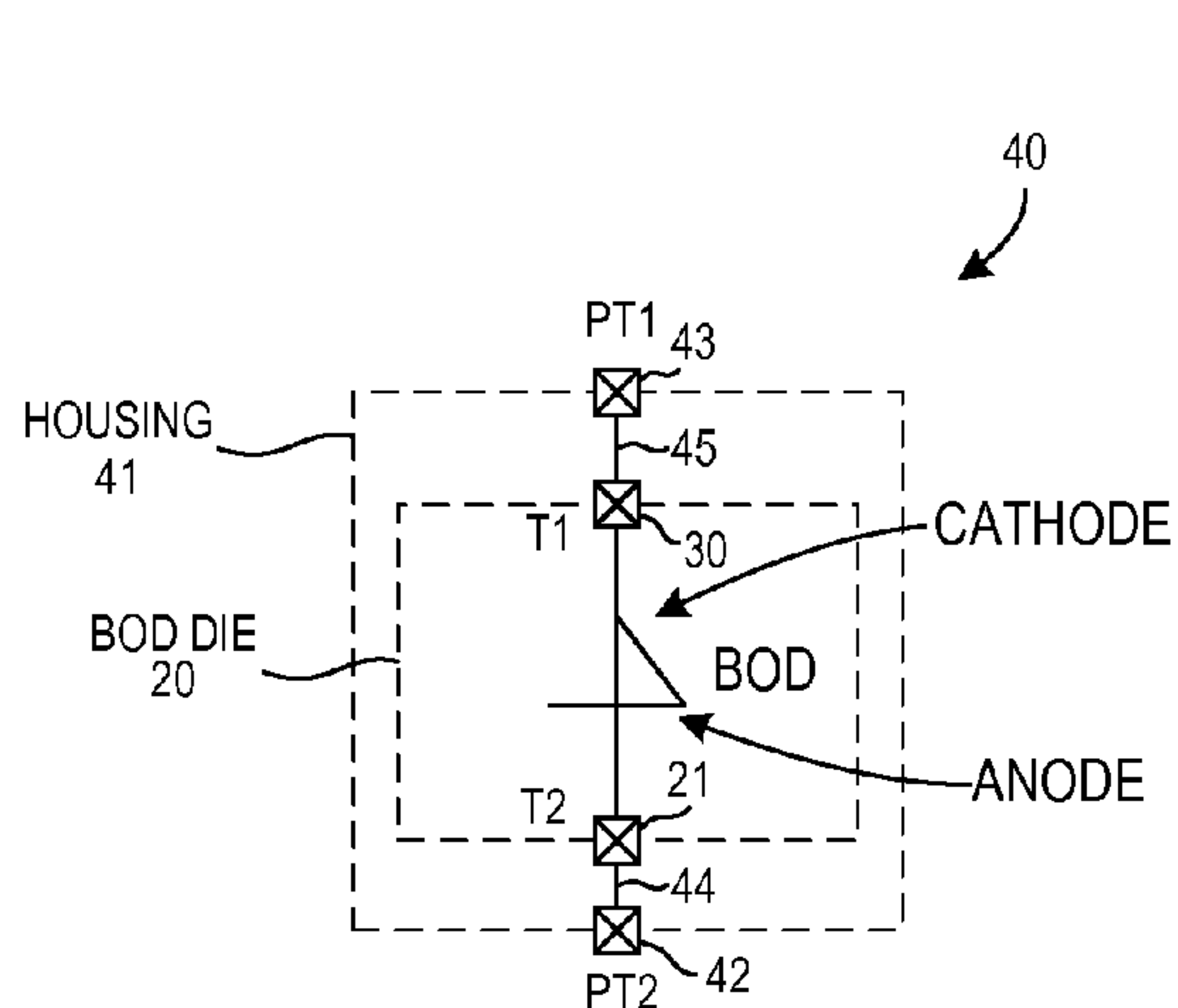
PACKAGED BOD DEVICE FIG. 9
