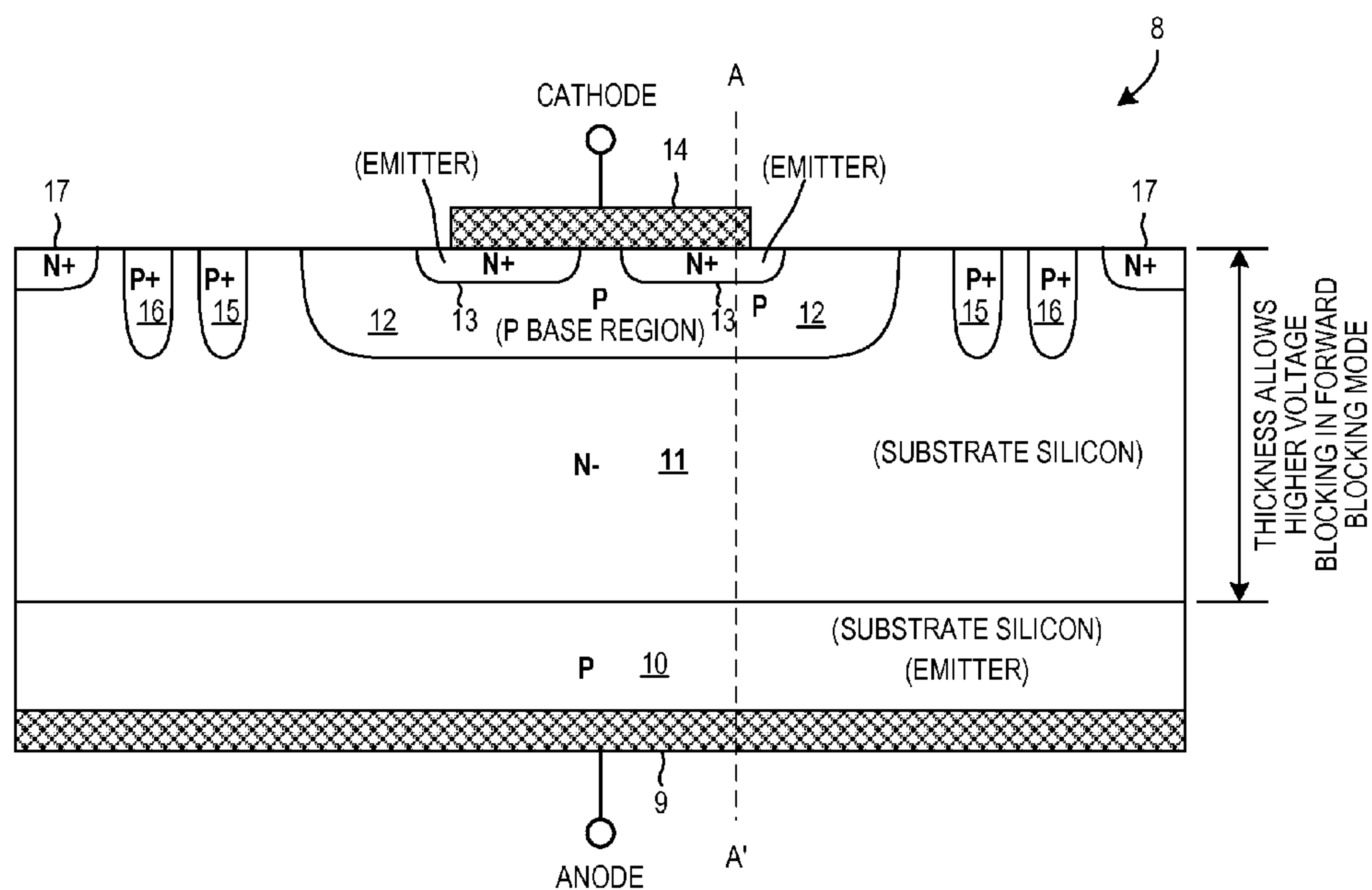
BULK BOD (PRIOR ART) FIG. 4
