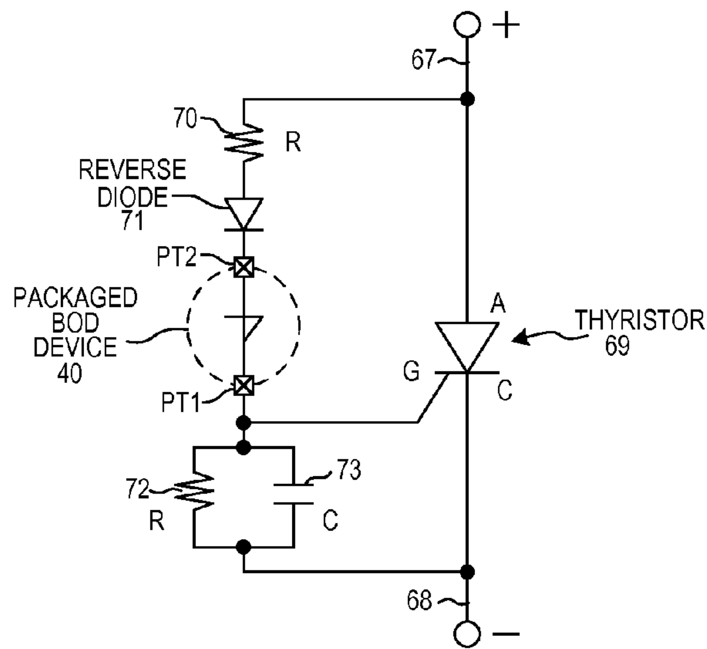
THYRISTOR PROTECTION CIRCUIT FIG. 19
