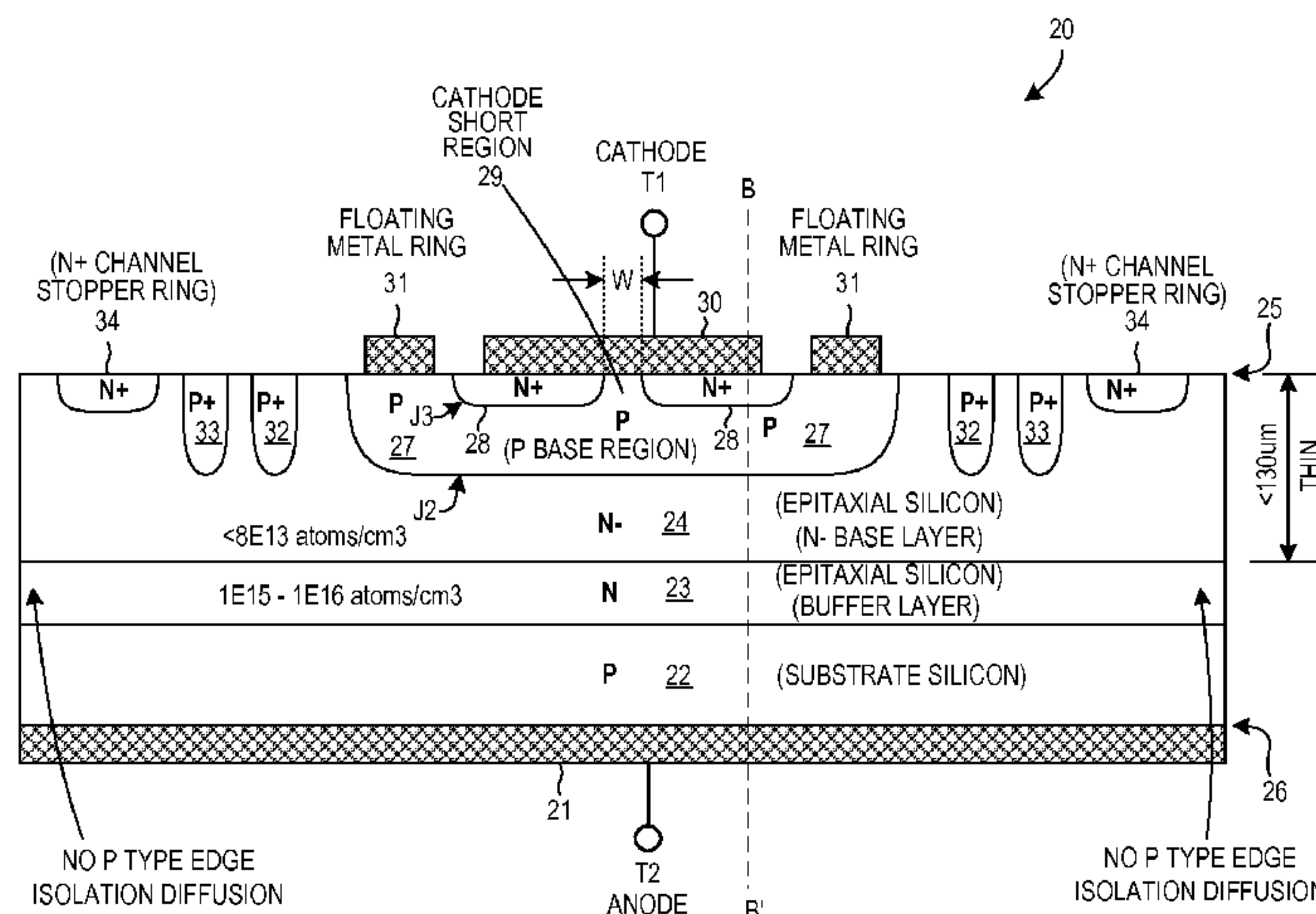
BREAKOVER DIODE DEVICE
