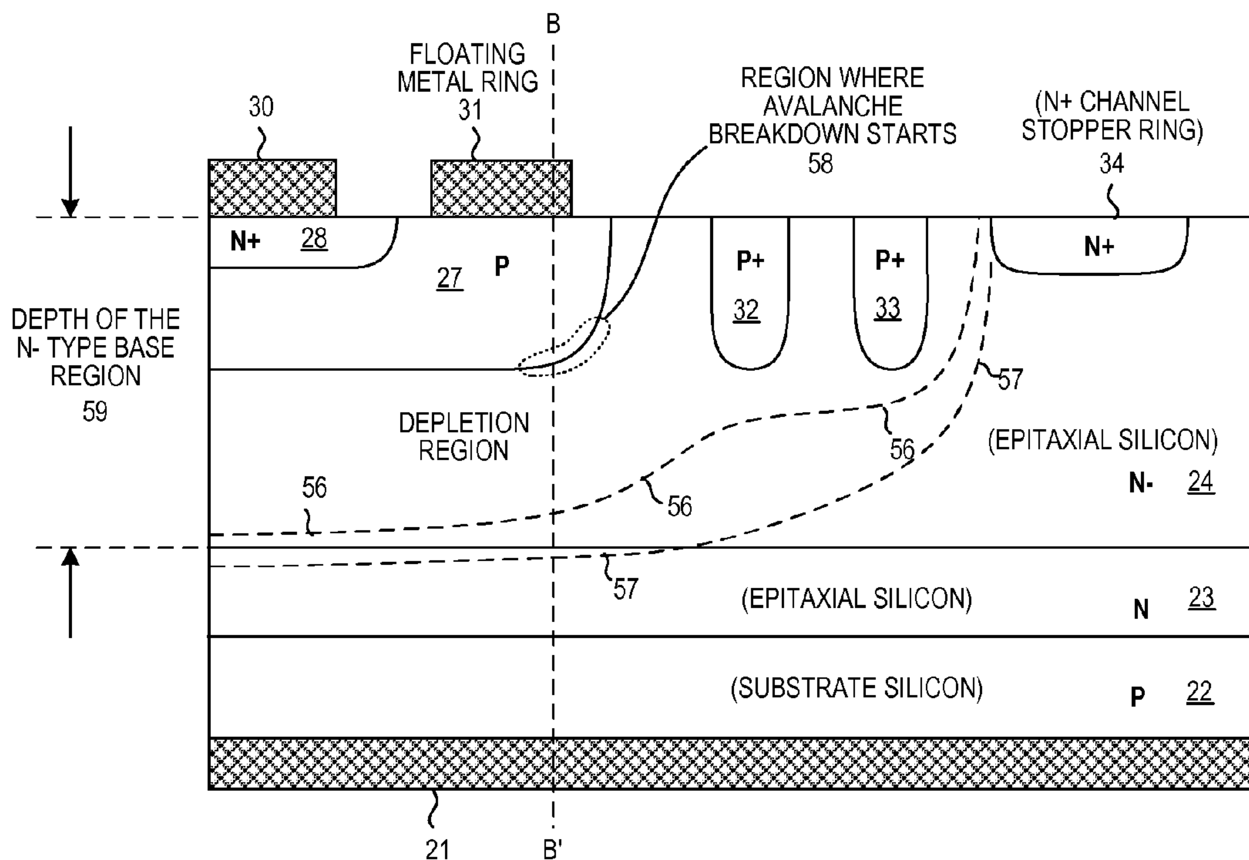
DEPLETION REGION JUST BEFORE AVALANCHE BREAKDOWN
