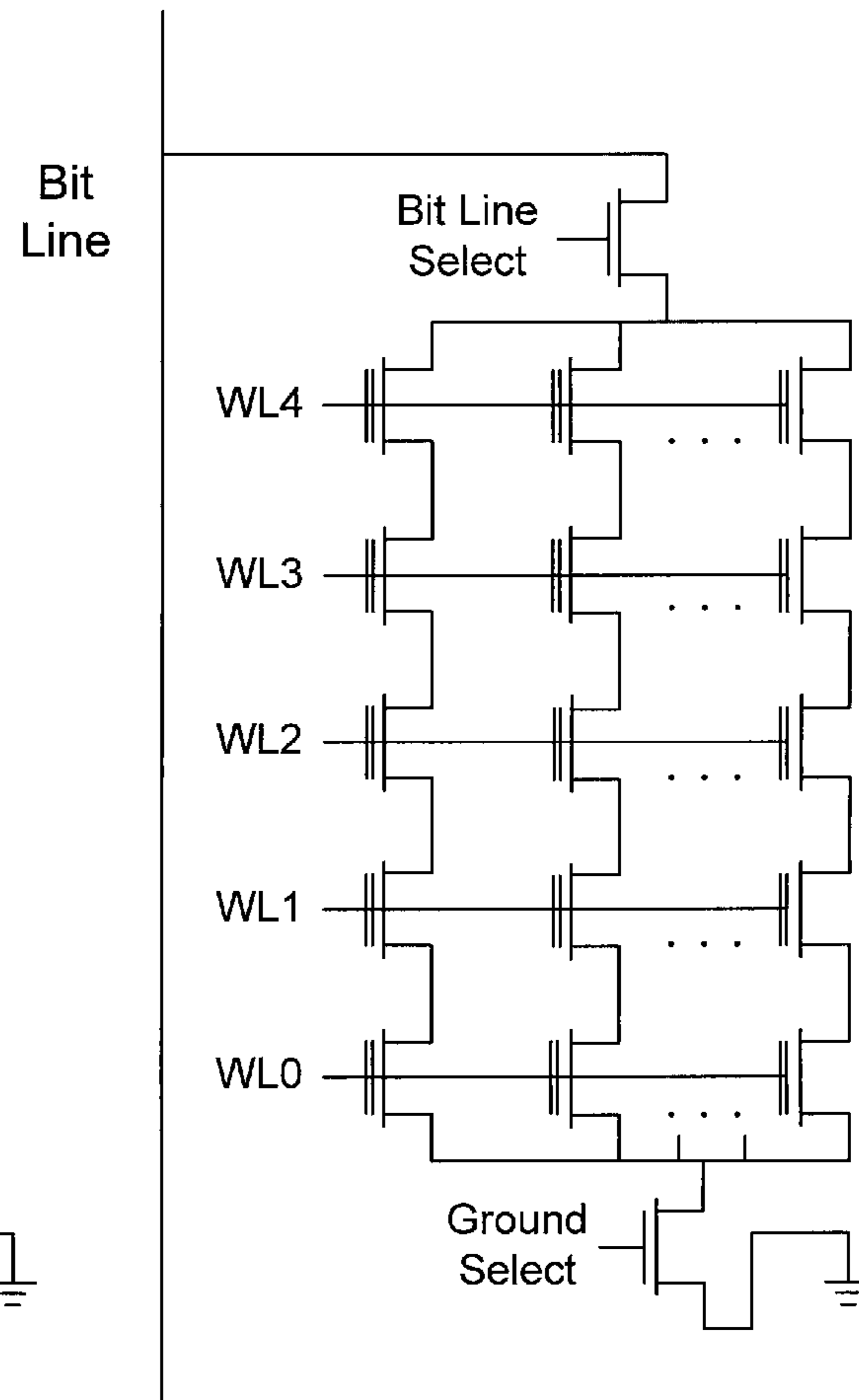
Multi-cell NAND flash structure
