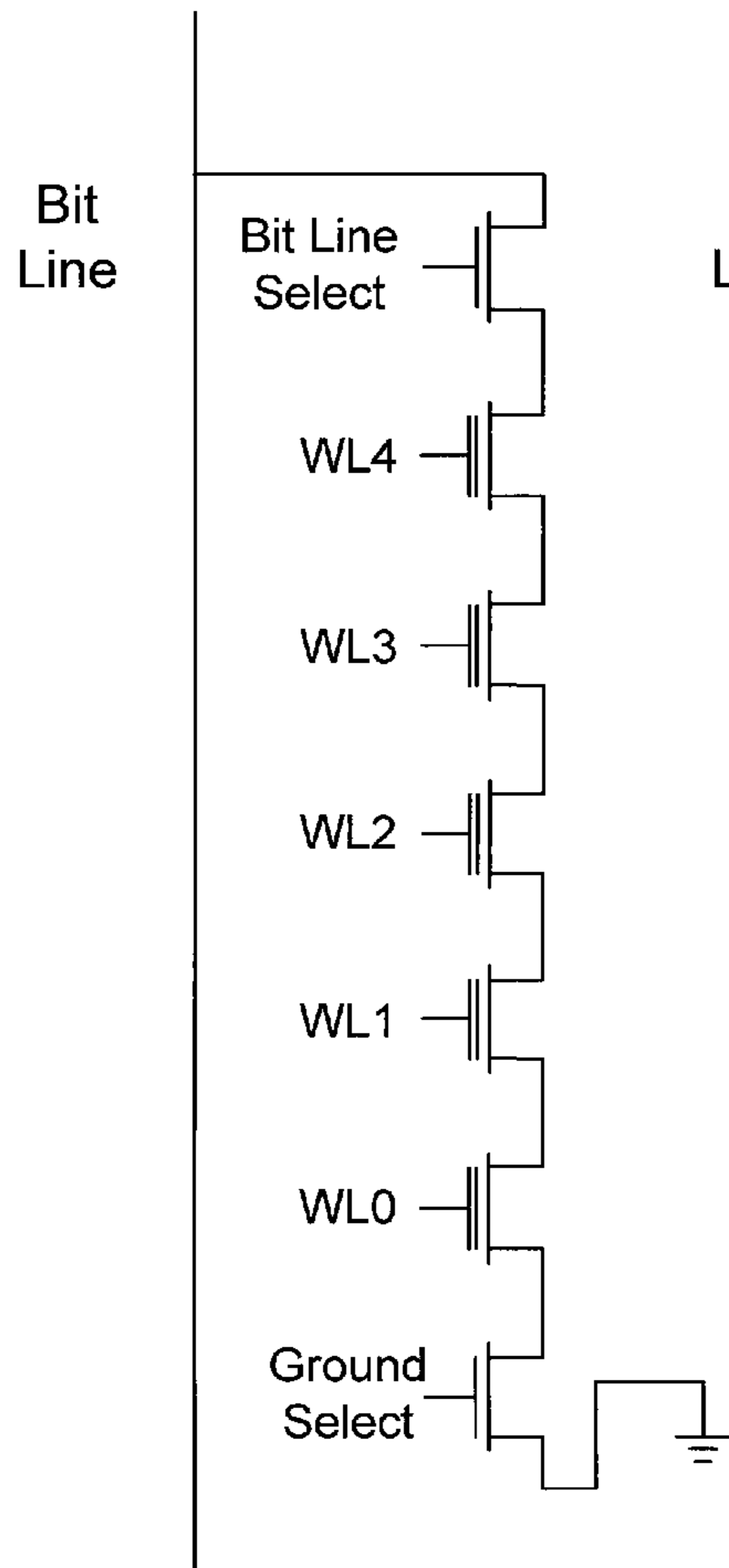
Traditional NAND flash structure
