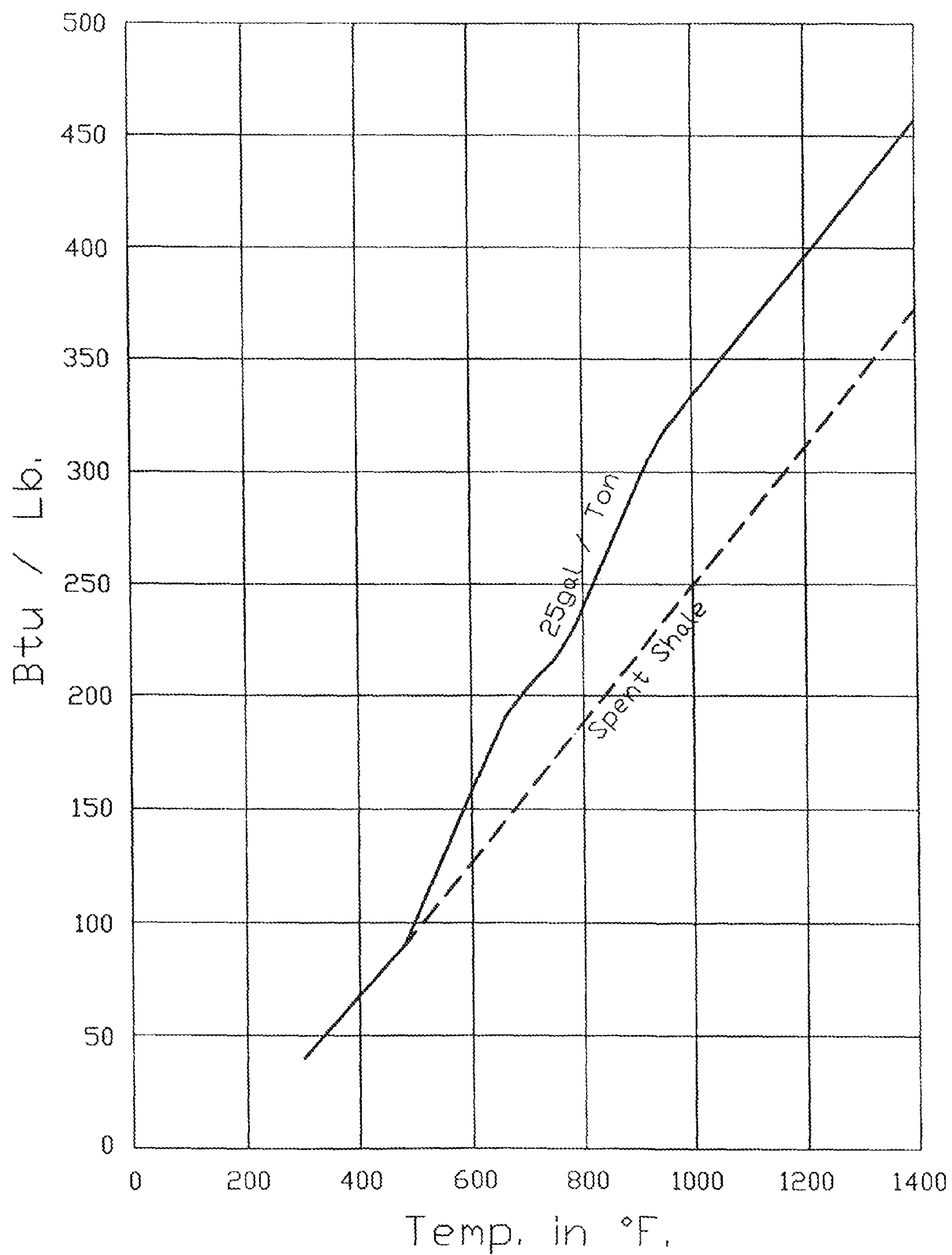
Figure 3: Thermal Energy Required For Retorting Oil Shale
