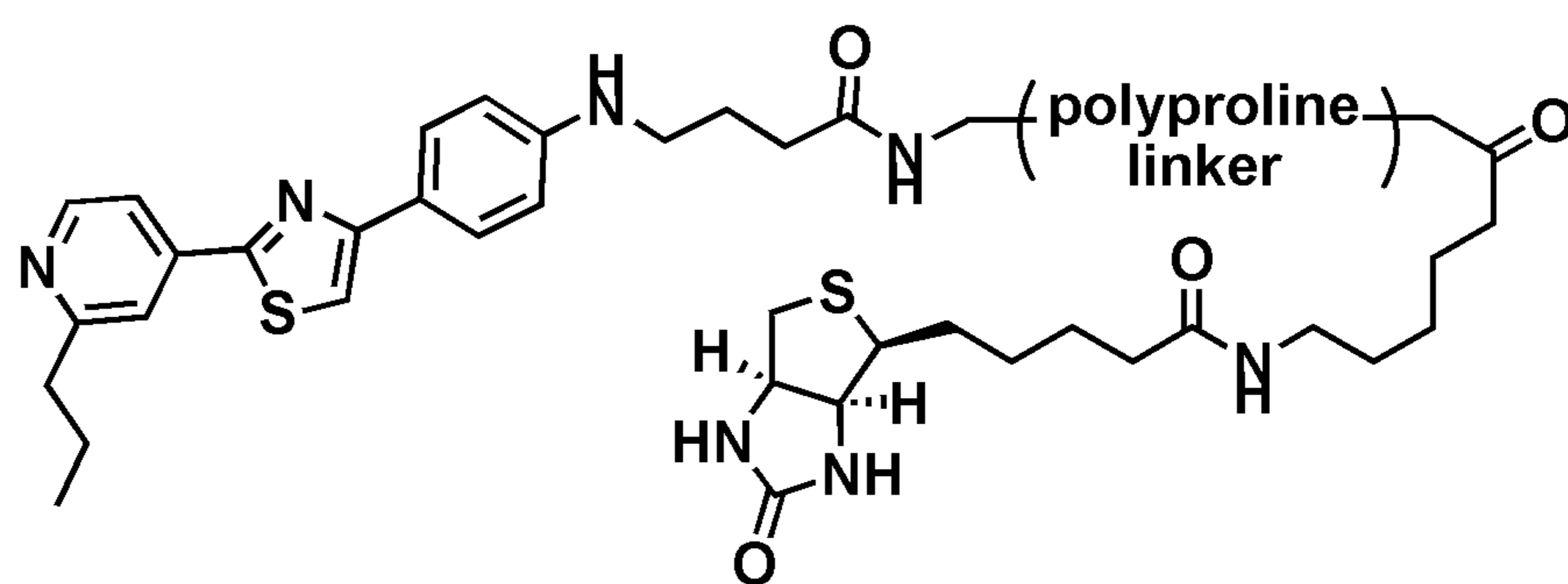
Fatostatin-polyproline linker-biotin conjugate
