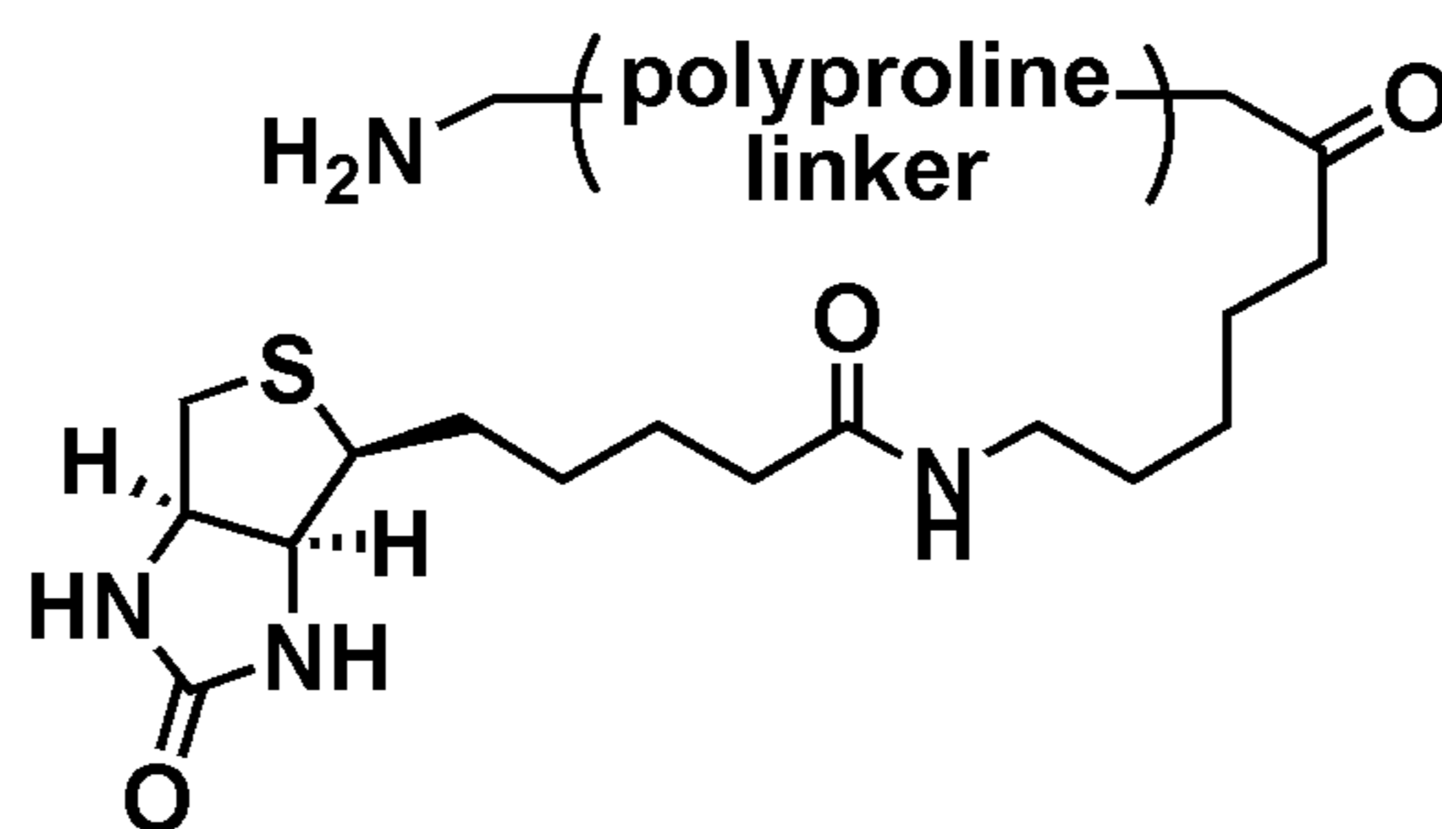
polyproline linker-biotin conjugate
