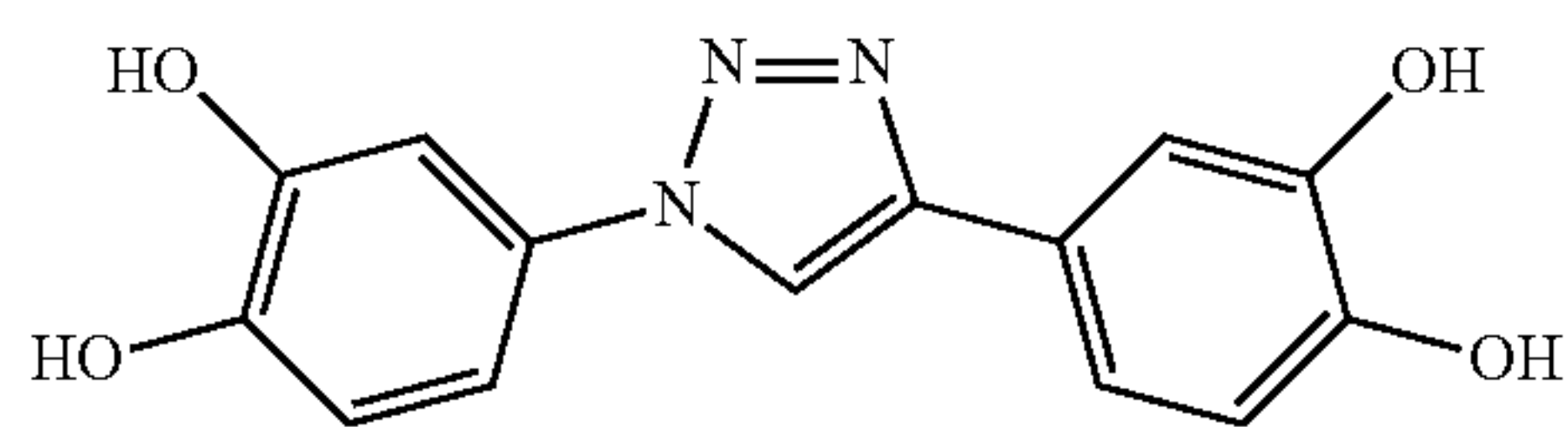
Compound SA-68
