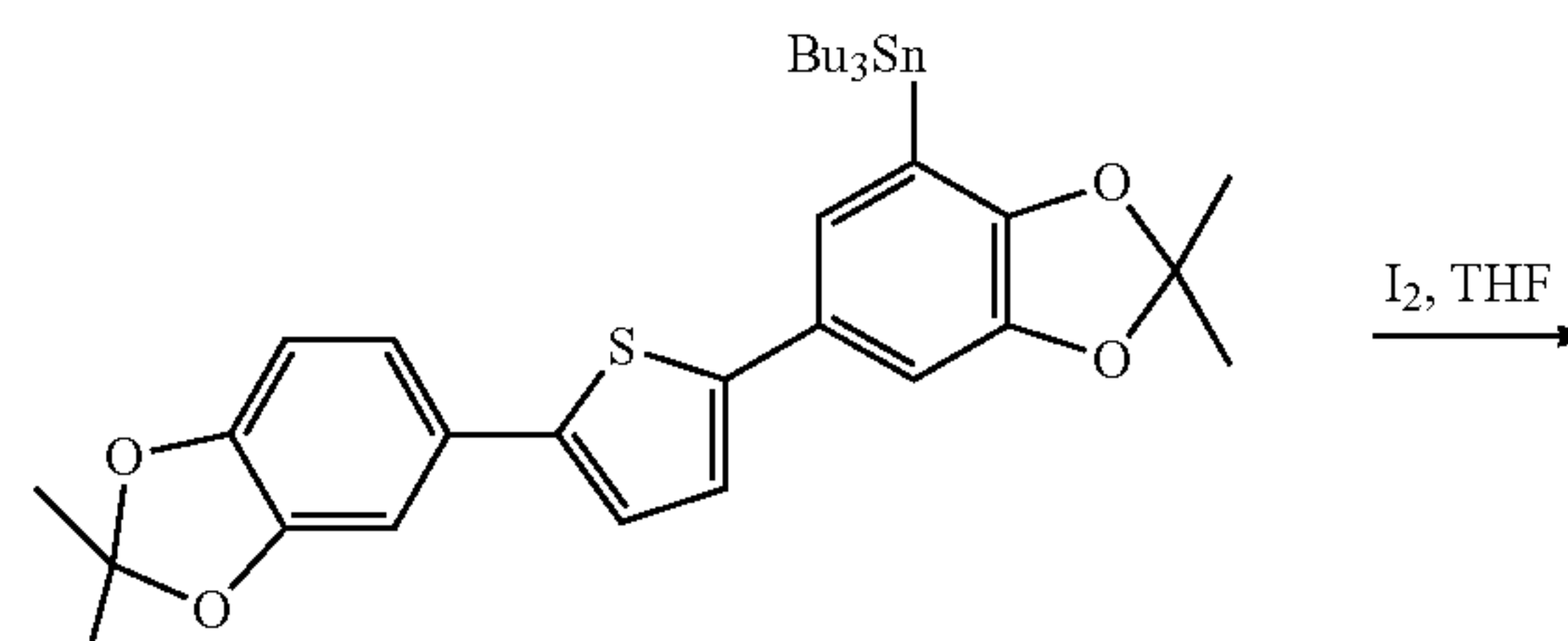
SA-77
