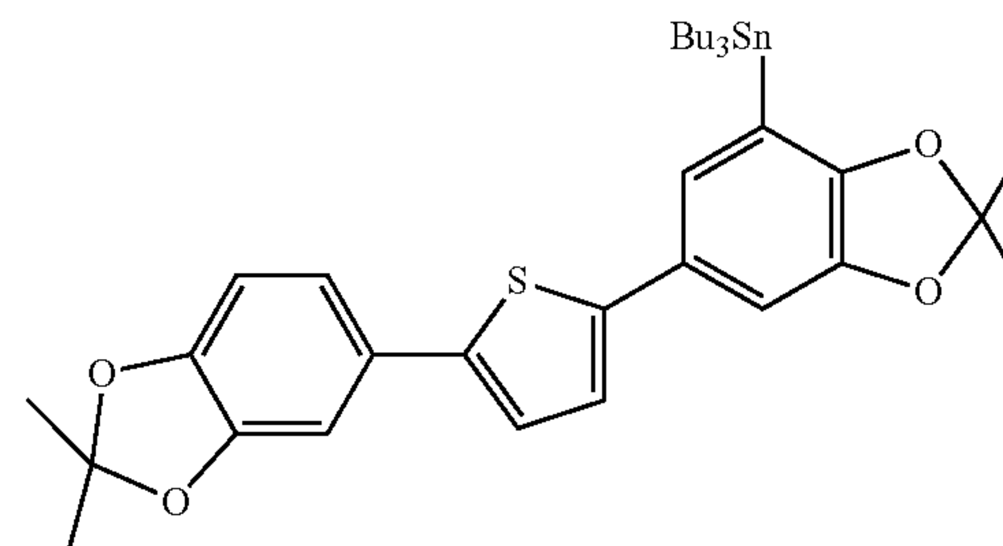
SA-77
