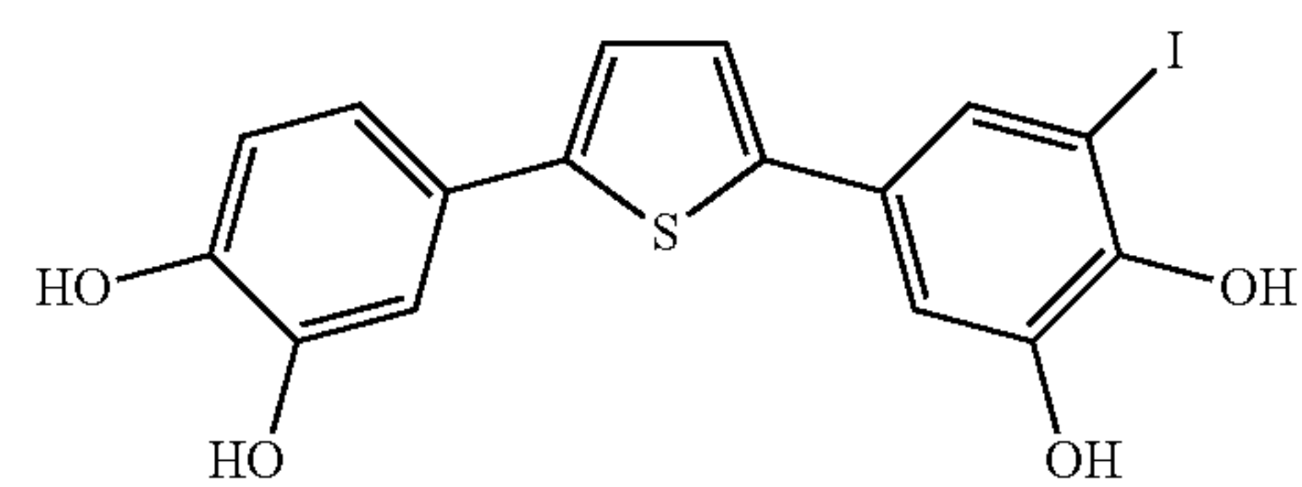
Compound SA-79
