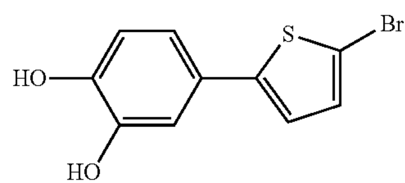
SA-62
