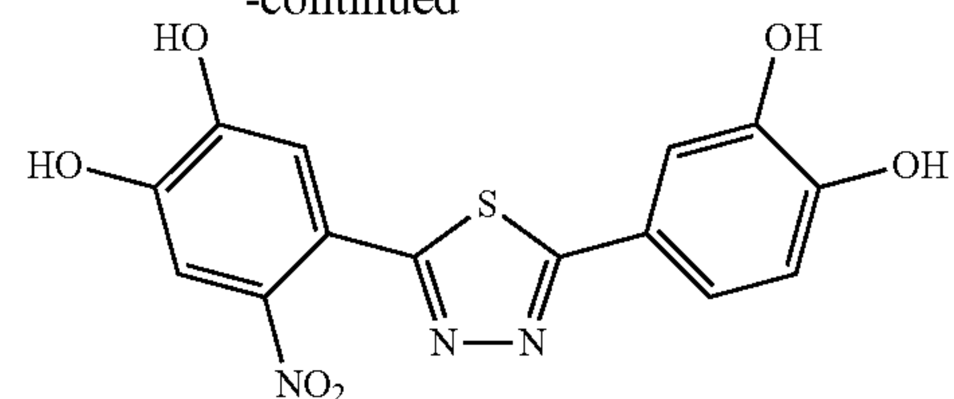
SA-108
