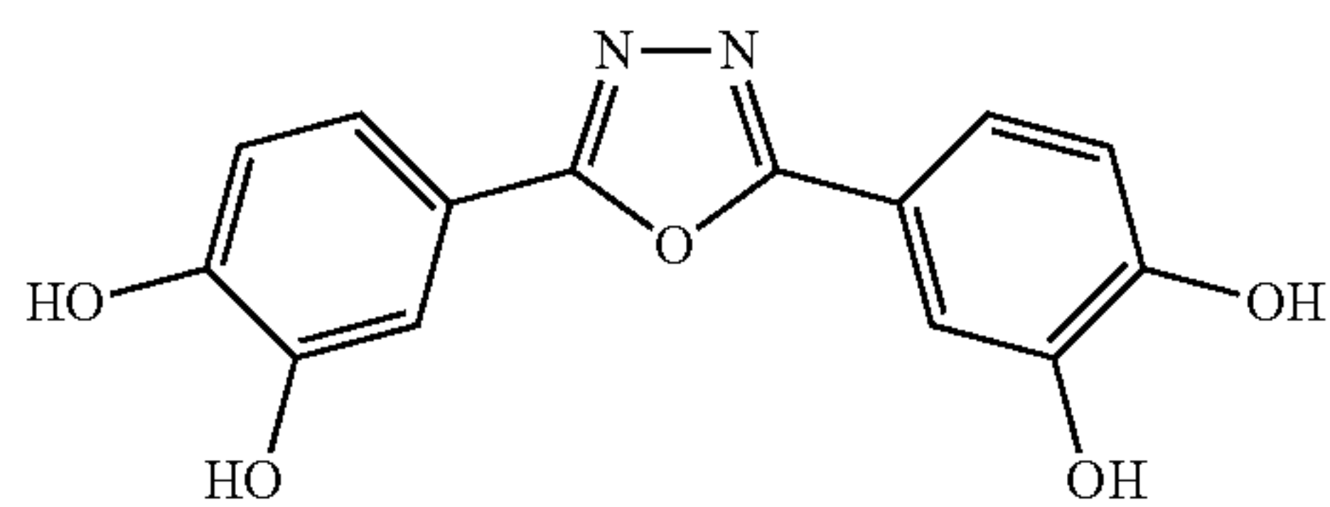
Compound SA-67
