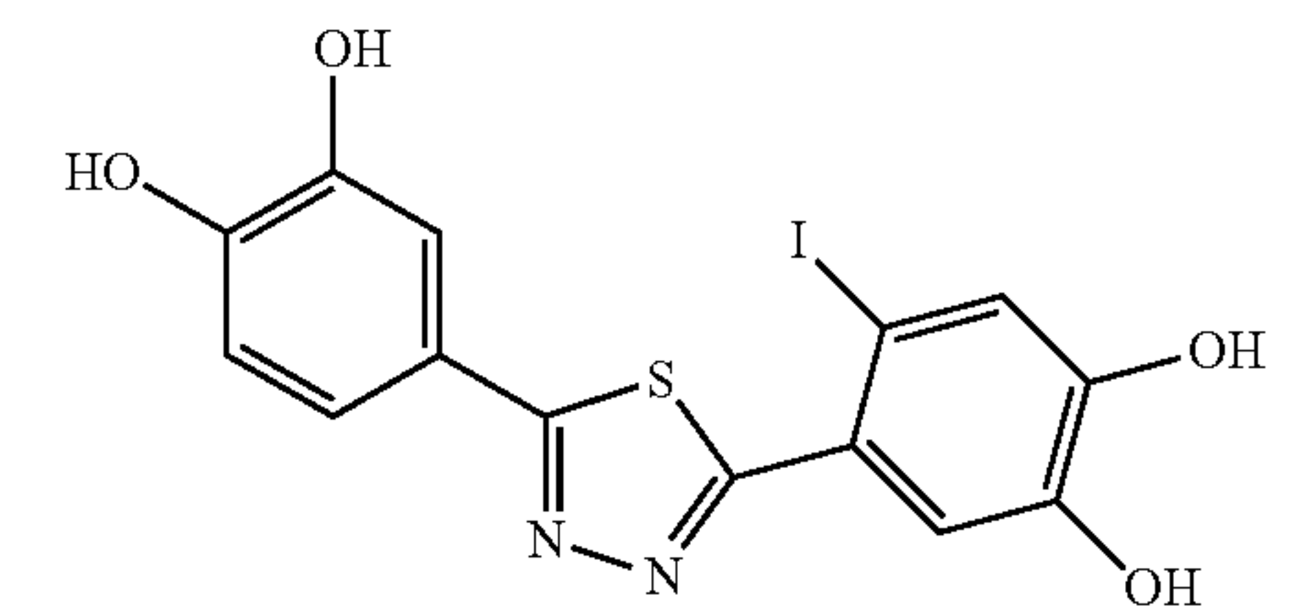
Compound SA-77
