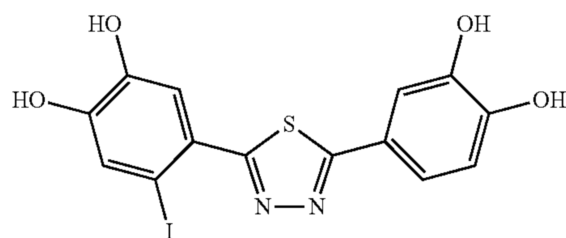
SA-76
