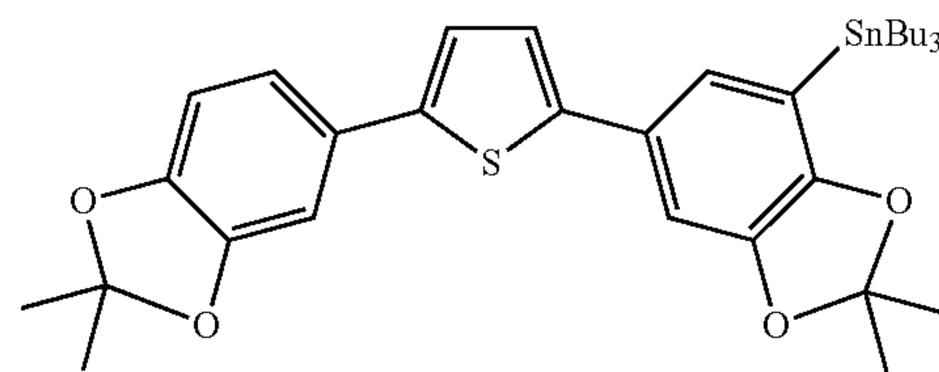
Compound SA-78
