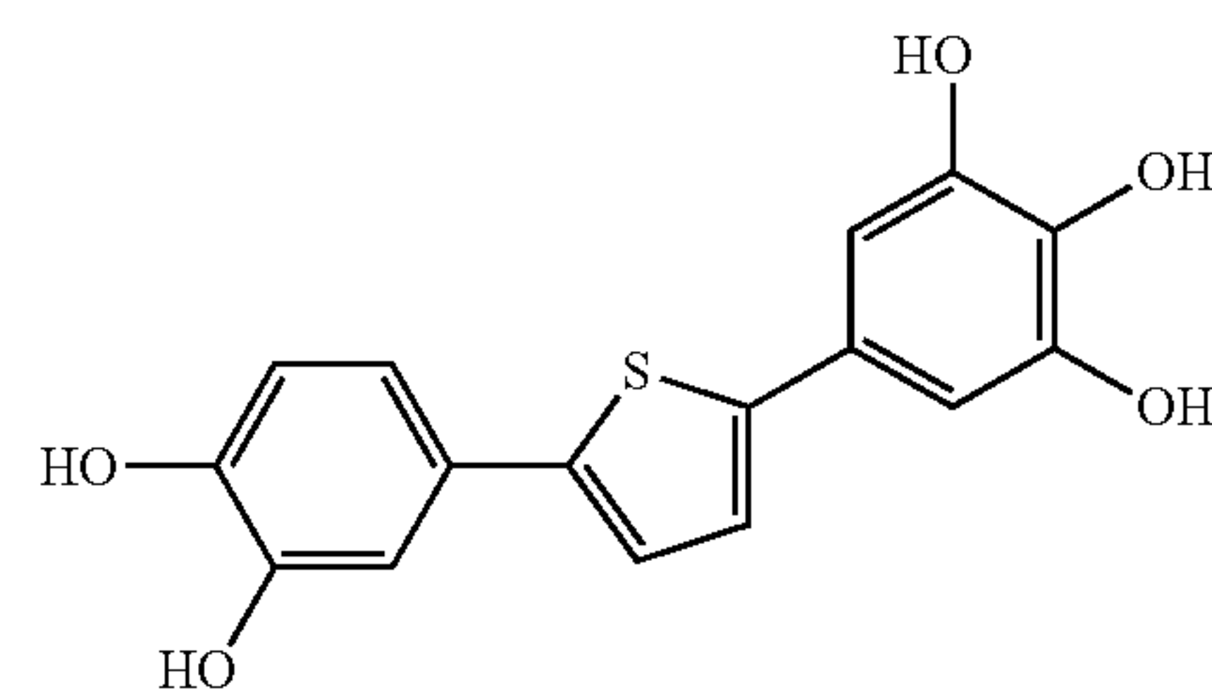
SA-63
