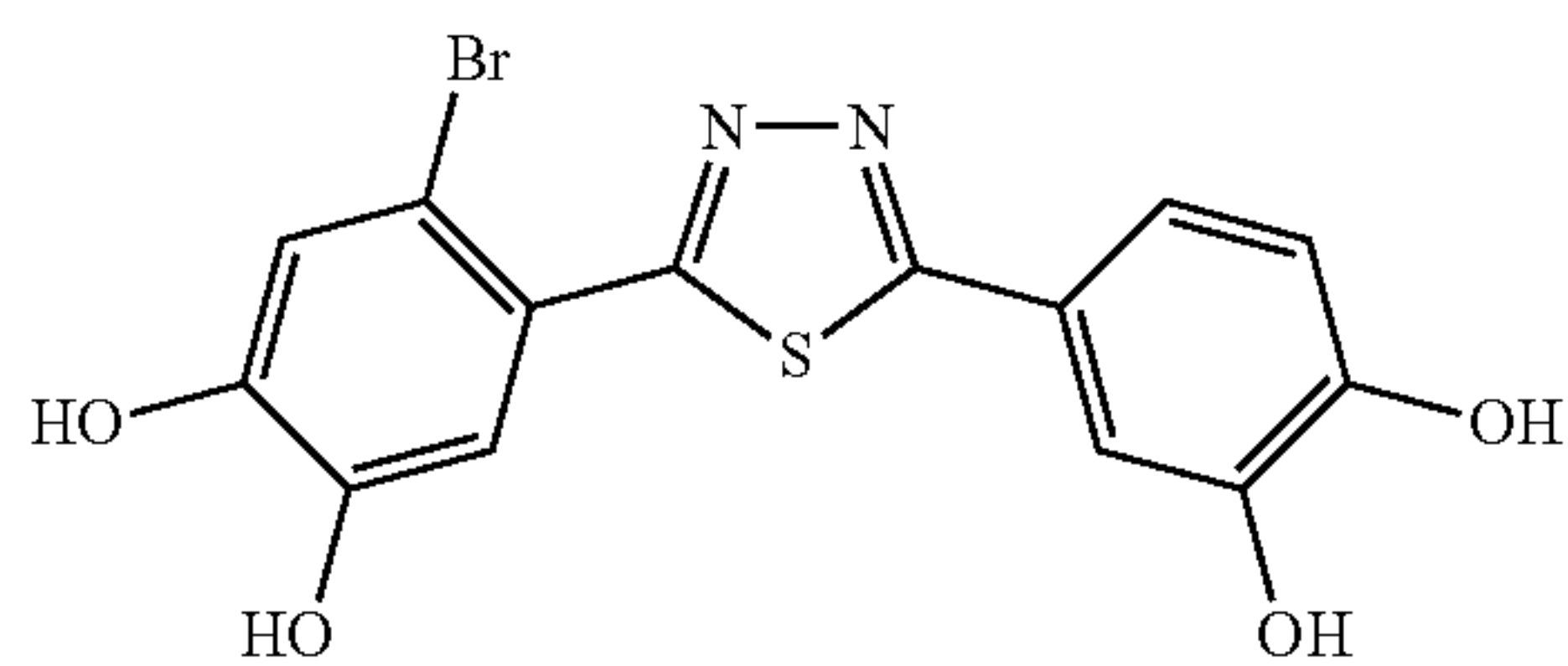
Compound SA-66
