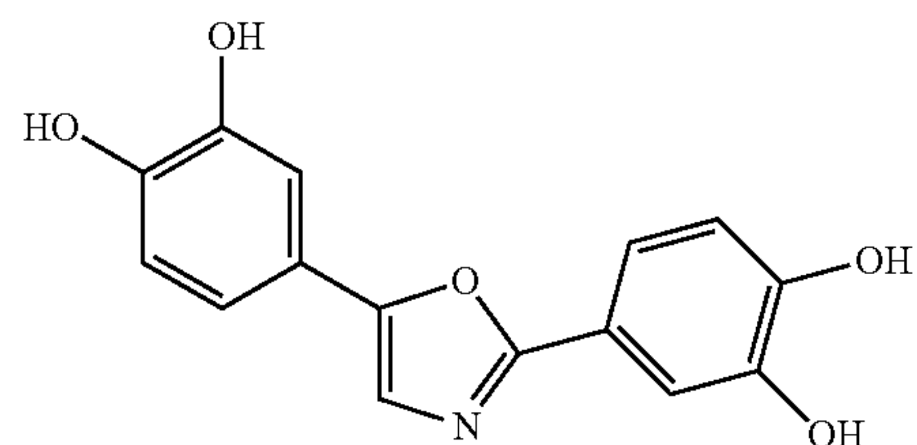
Compound SA-72
