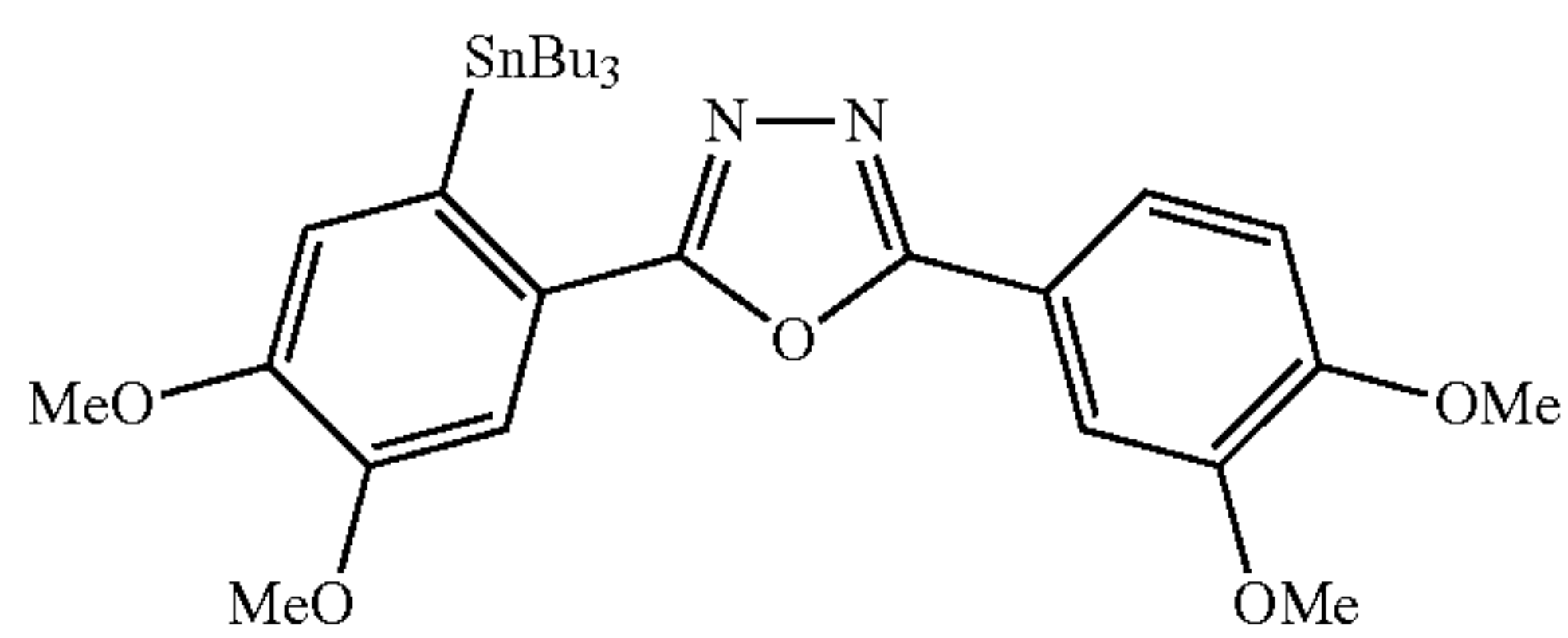
Compound SA-65
