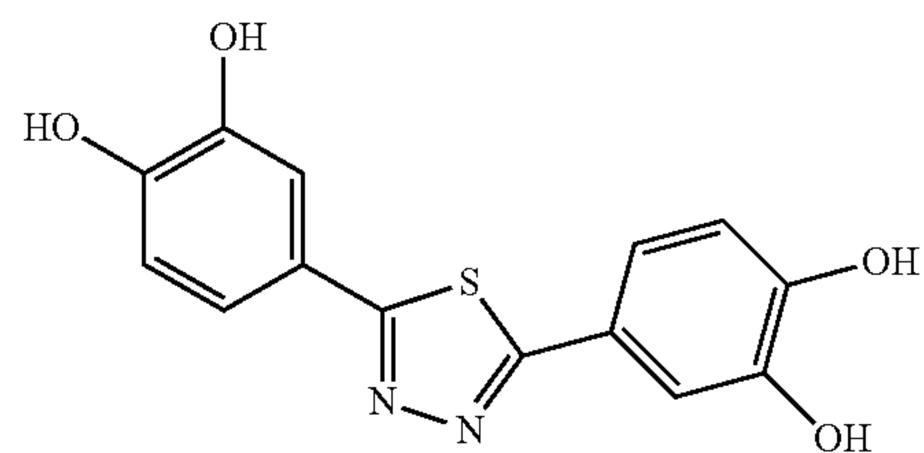
Compound SA-72
