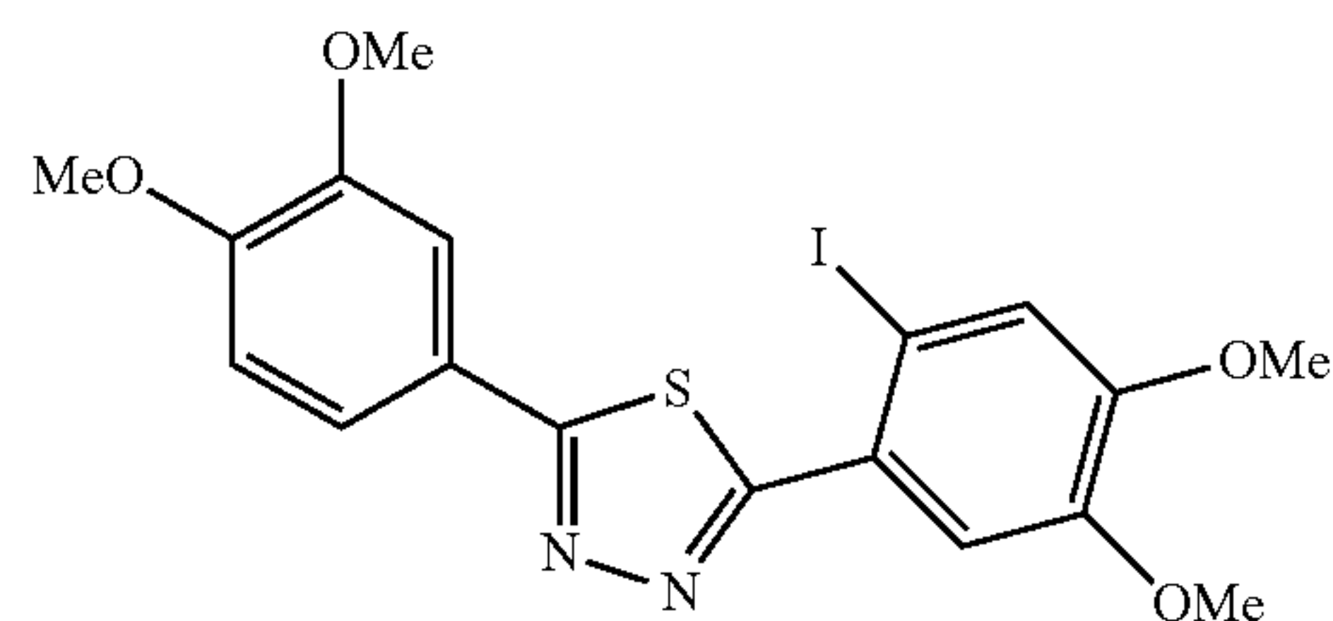
Compound SA-76
