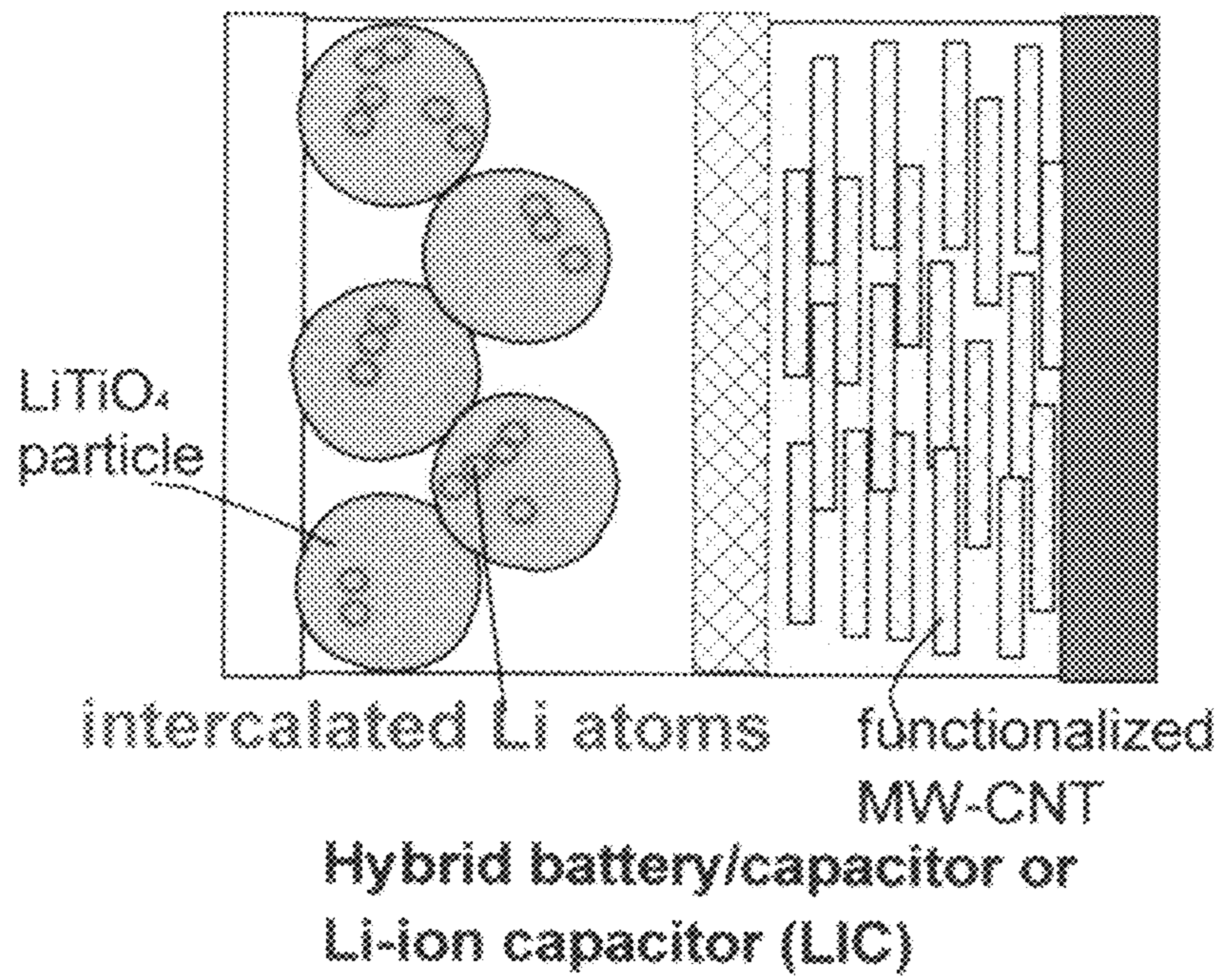
Hybrid battery/capacitor or Li-ion capacitor (LIC) FIG. 1(G) prior art
