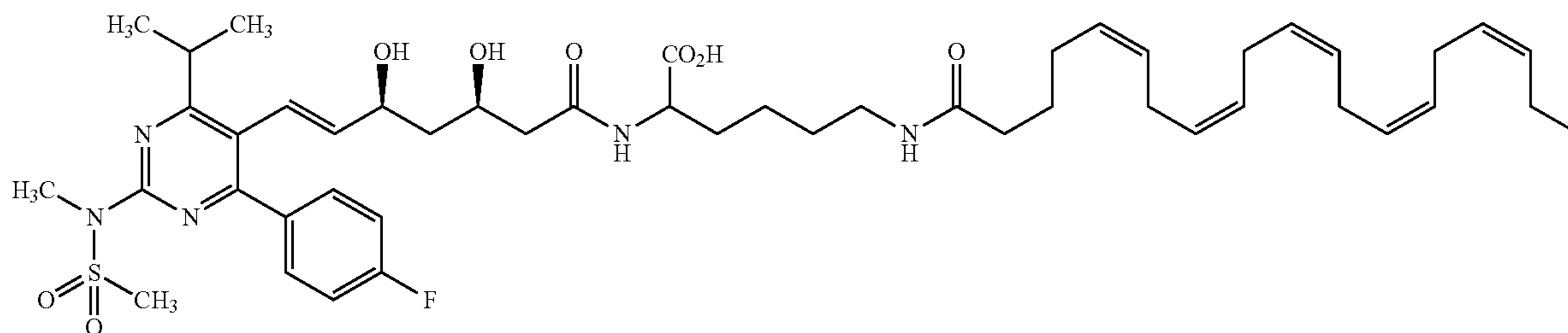
(5Z,8Z,11Z,14Z,17Z)-N-(2-(2-((3R,5S,E)-7-(4-(4-fluorophenyl)-6-isopropyl-2-(N-methylmethylsulfonamido)pyrimidin-5-yl)-3,5-dihydroxyhept-6-enamido)ethoxy)ethyl)icosa-5,8,11,14,17-pentaenamide (I-54)
