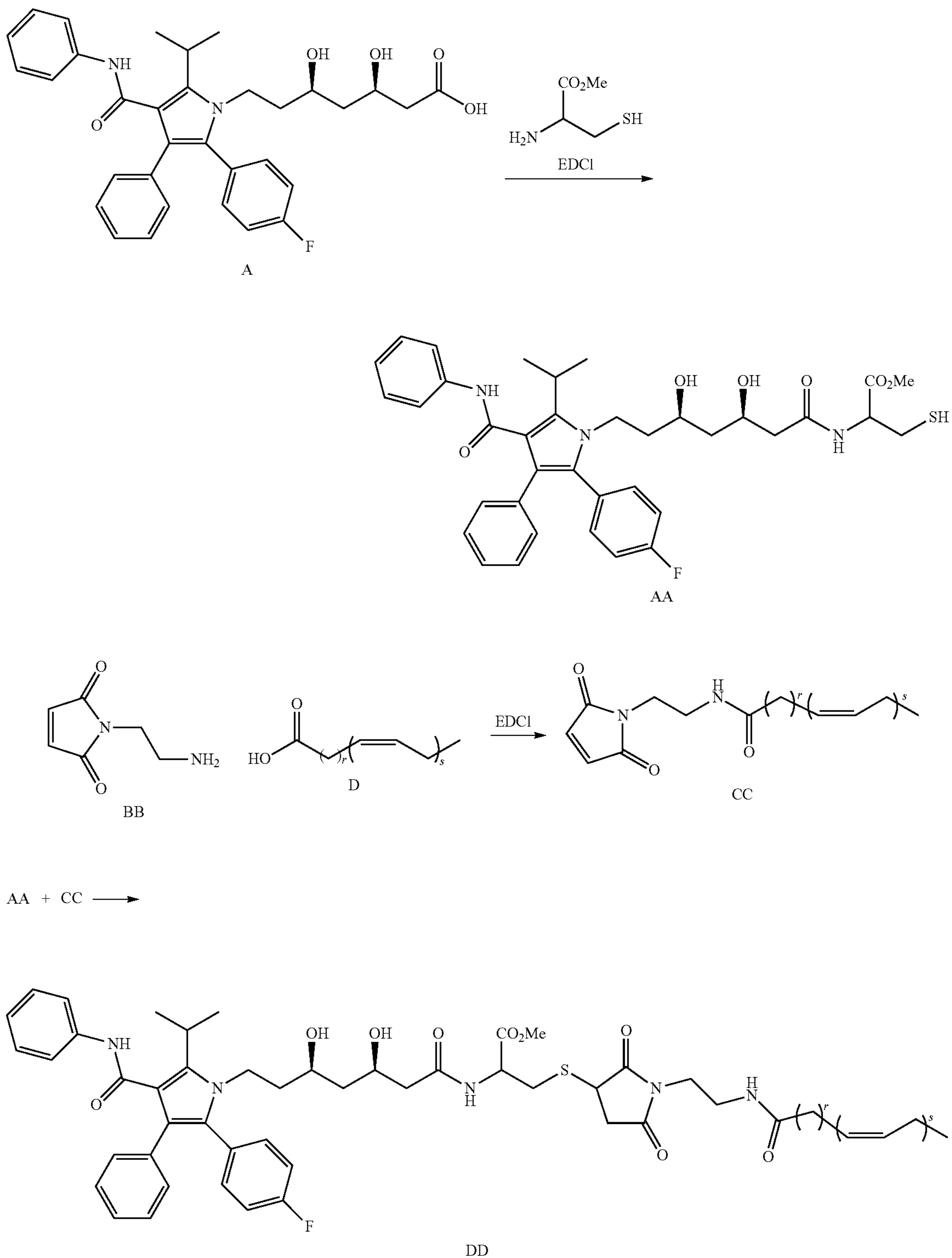
Scheme 8
