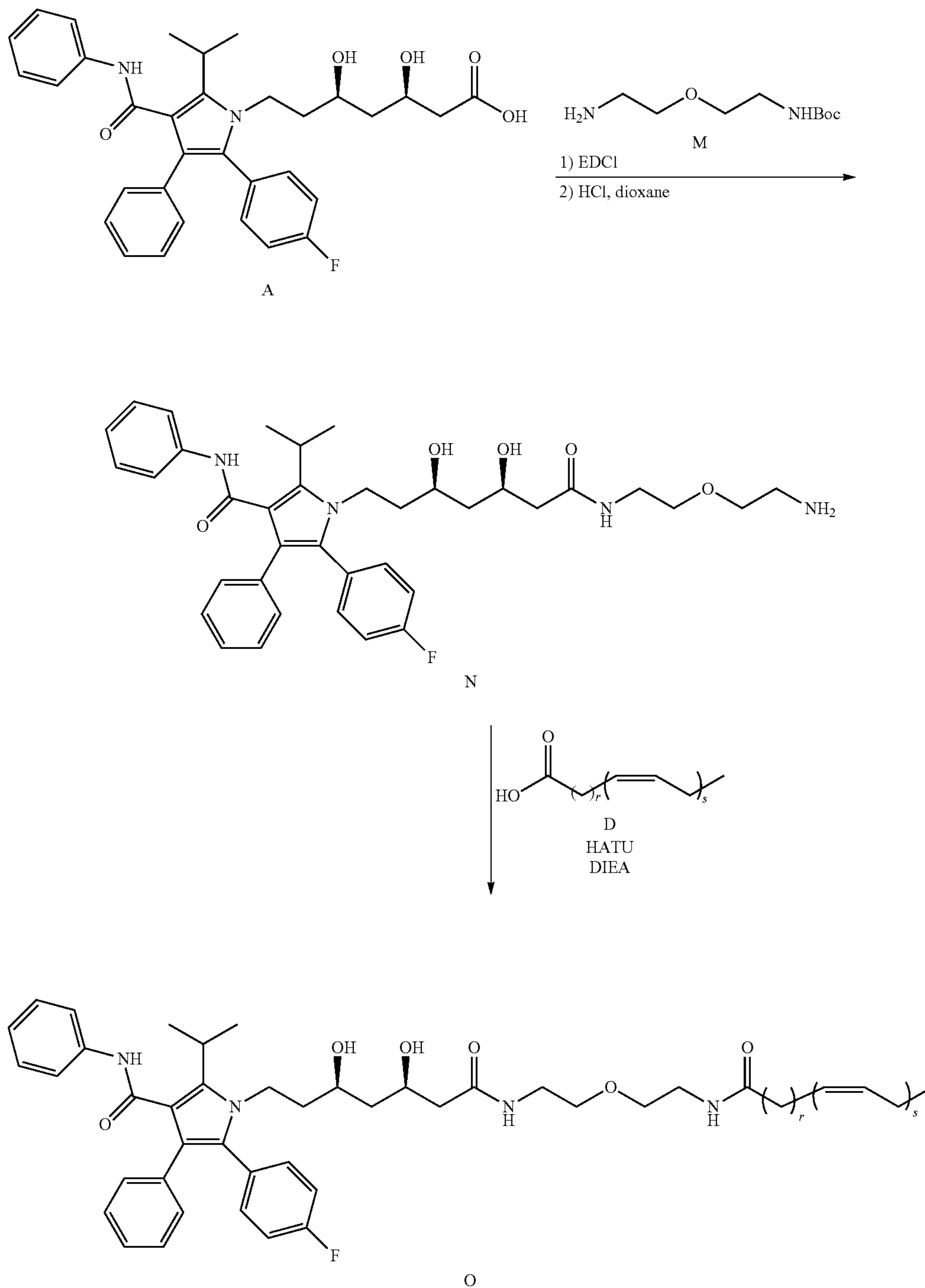
Scheme 4
