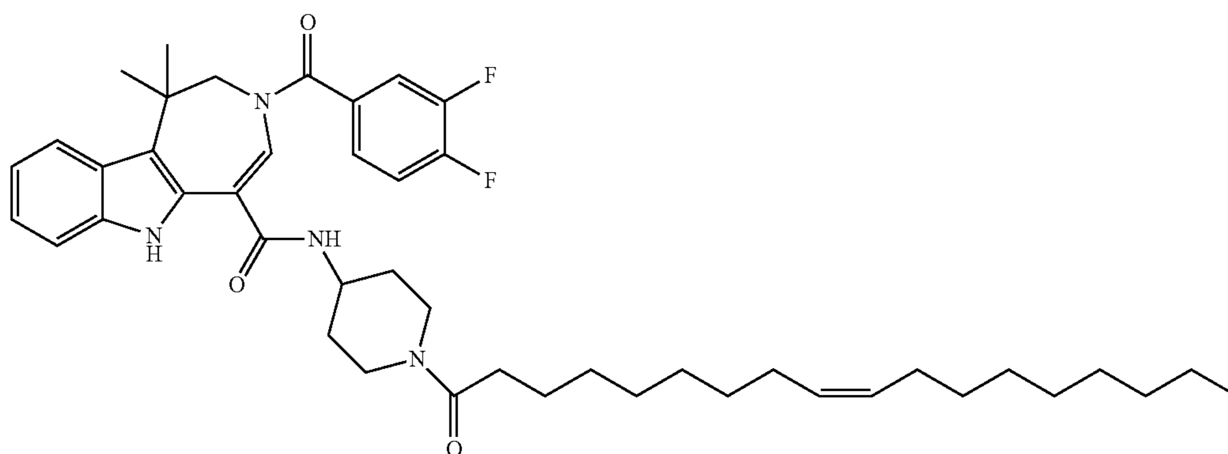
3-(3,4-difluorobenzoyl)-N-(1-((5Z,8Z,11Z,14Z,17Z)-icosa-5,8,11,14,17-pentaenoyl)piperidin-4-yl)-1,1-dimethyl-1,2,3,6-tetrahydroazepino[4,5-b]indole-5-carboxamide (II-71)
