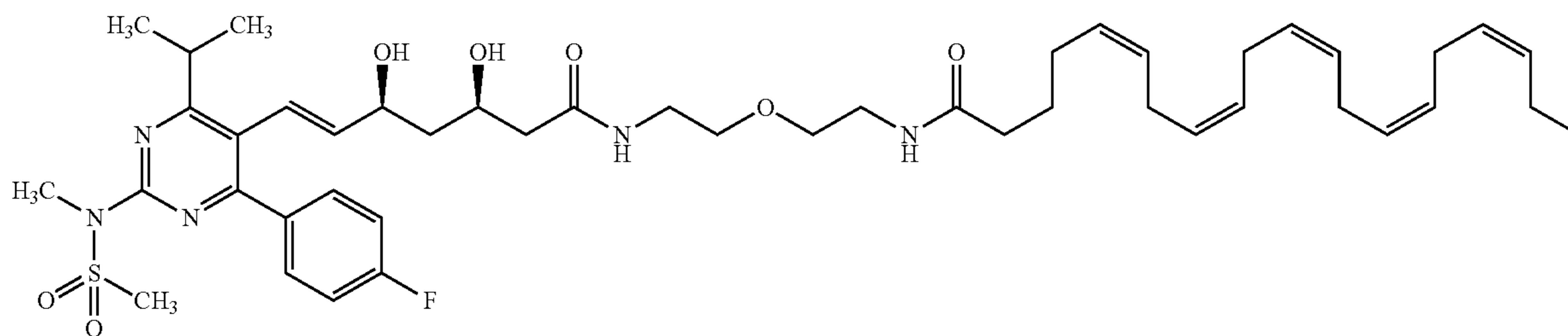
(4Z,7Z,10Z,13Z,16Z,19Z)-N-(2-(2-((3R,5S,E)-7-(4-(4-fluorophenyl)-6-isopropyl-2-(N-methylmethylsulfonamido)pyrimidin-5-yl)-3,5-dihydroxyhept-6-enamido)ethoxy)ethyl)docosa-4,7,10,13,16,19-hexaenamide (I-53)
