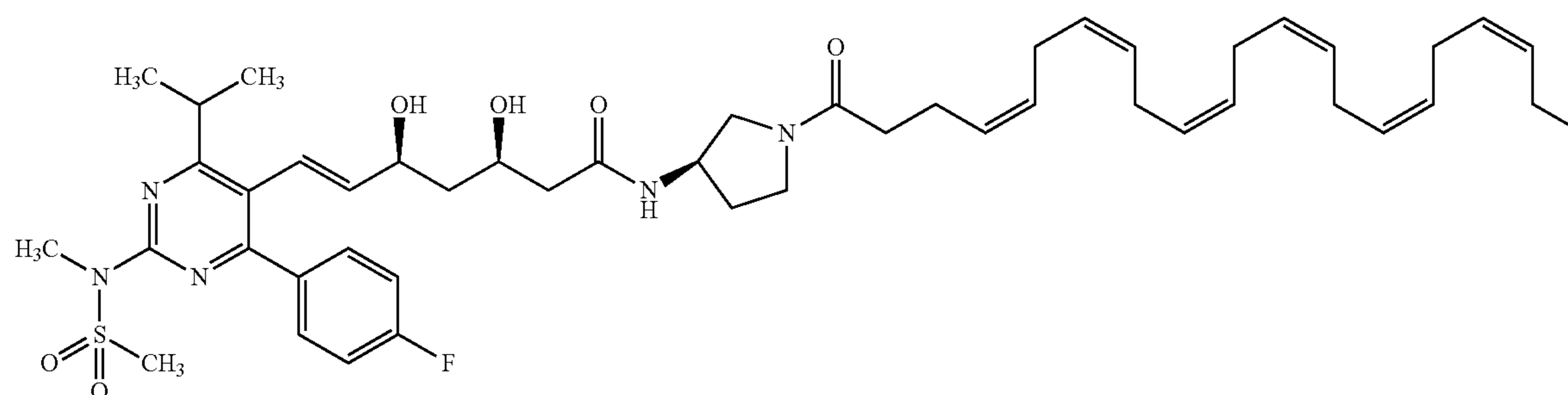
(3R,5S,E)-N-((R)-1-((4Z,7Z,10Z,13Z,16Z,19Z)-docosa-4,7,10,13,16,19-hexaenoyl)pyrrolidin-3-yl)-7-(4-(4-fluorophenyl)-6-isopropyl-2-(N-methylmethylsulfonamido)pyrimidin-5-yl)-3,5-dihydroxyhept-6-enamide (I-61)
