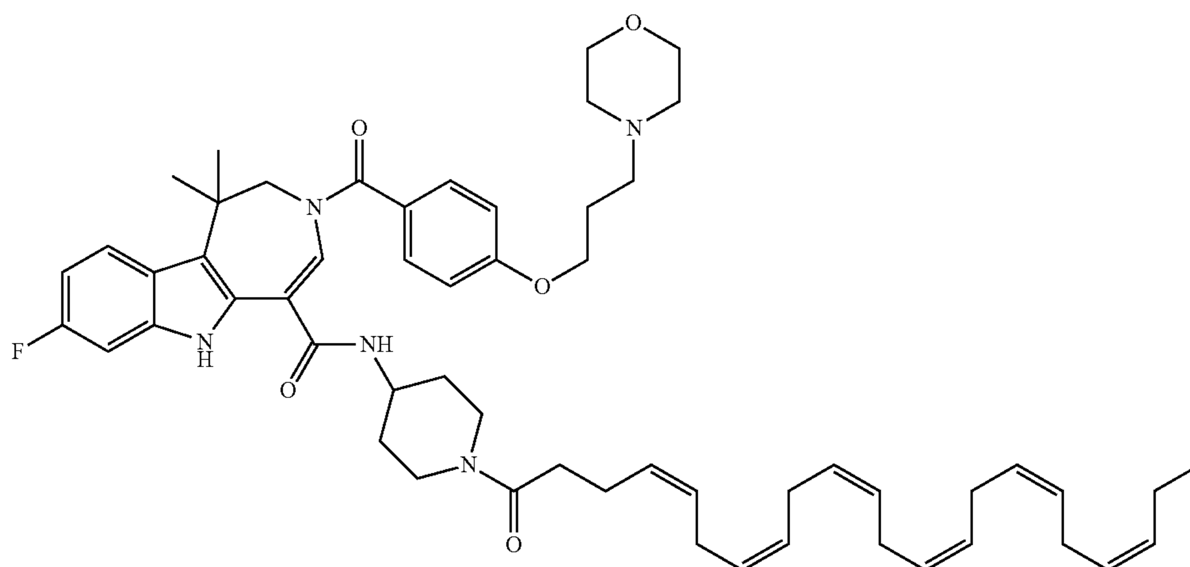
(Z)-8-fluoro-1,1-dimethyl-3-(4-(3-morpholinopropoxy)benzoyl)-N-(2-oleamidoethyl)-1,2,3,6-tetrahydroazepino[4,5-b]indole-5-carboxamide (II-60)
