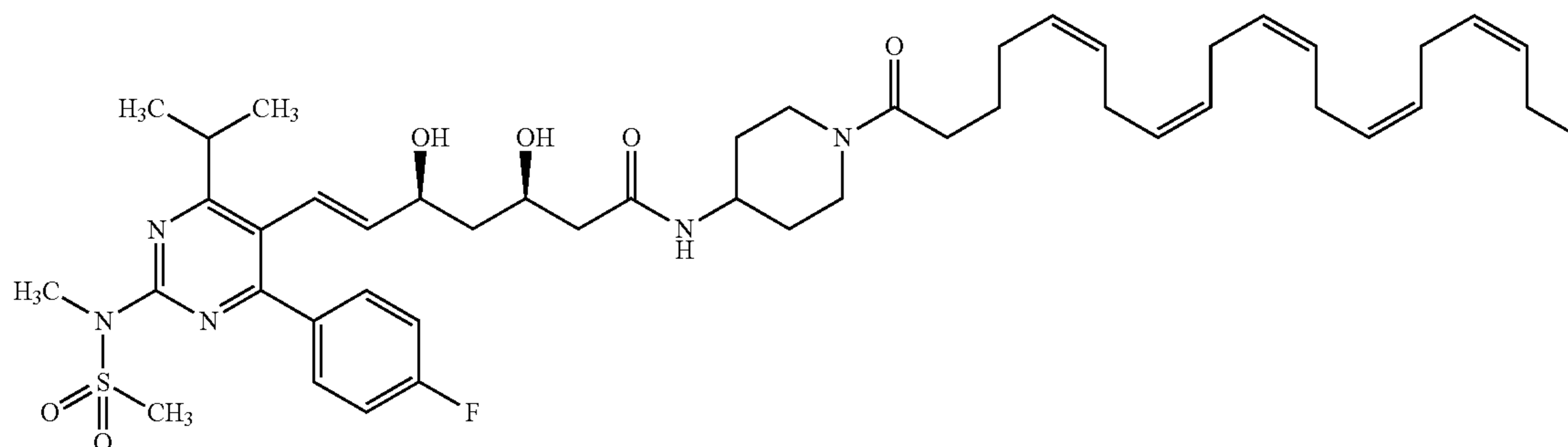
(3R,5S,E)-7-(4-(4-fluorophenyl)-6-isopropyl-2-(N-methylmethylsulfonamido)pyrimidin-5-yl)-3,5-dihydroxy-N-(1-((5Z,8Z,11Z,14Z,17Z)-icosa-5,8,11,14,17-pentaenoyl)piperidin-4-yl)hept-6-enamide (I-59)
