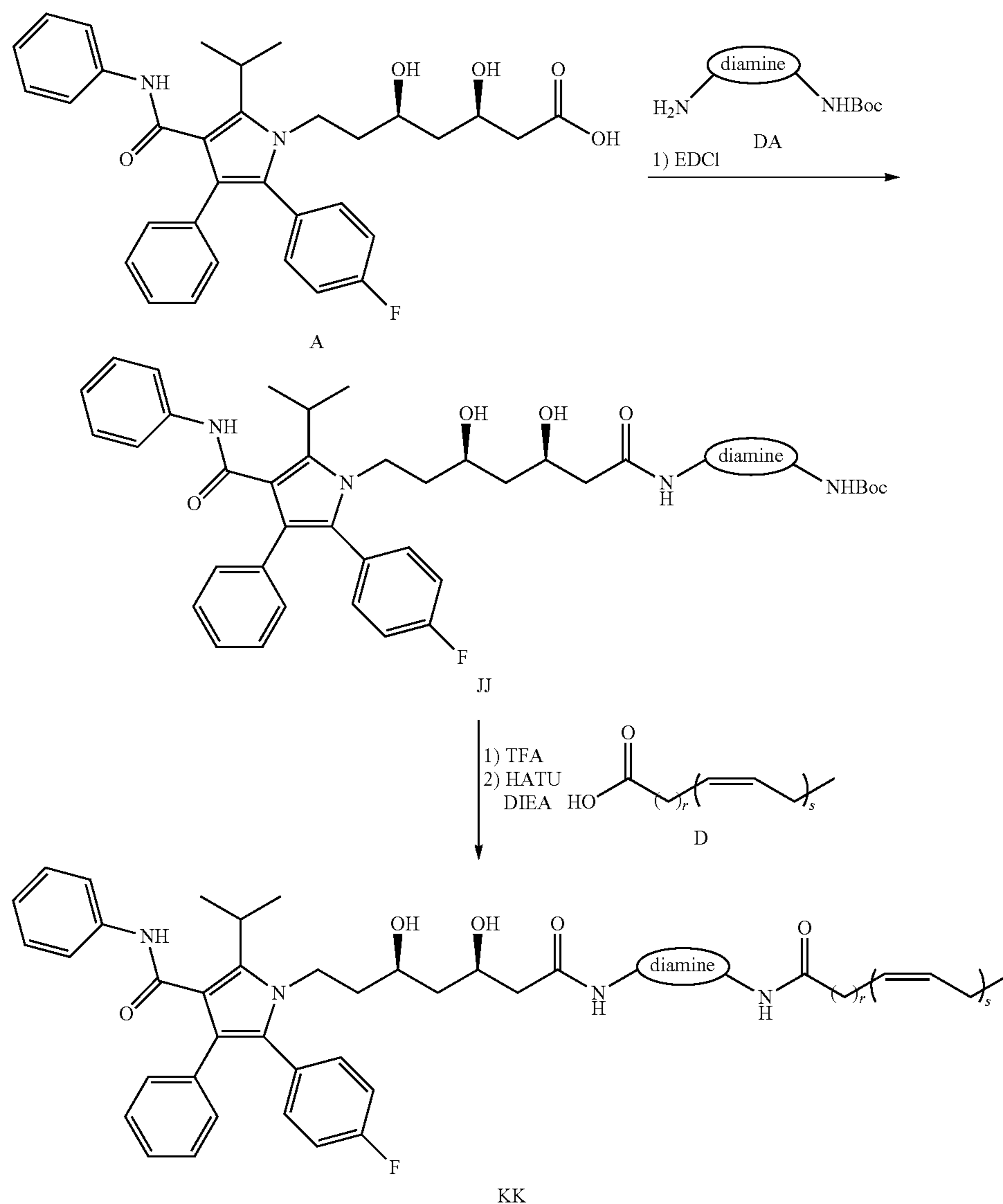
Scheme 10
