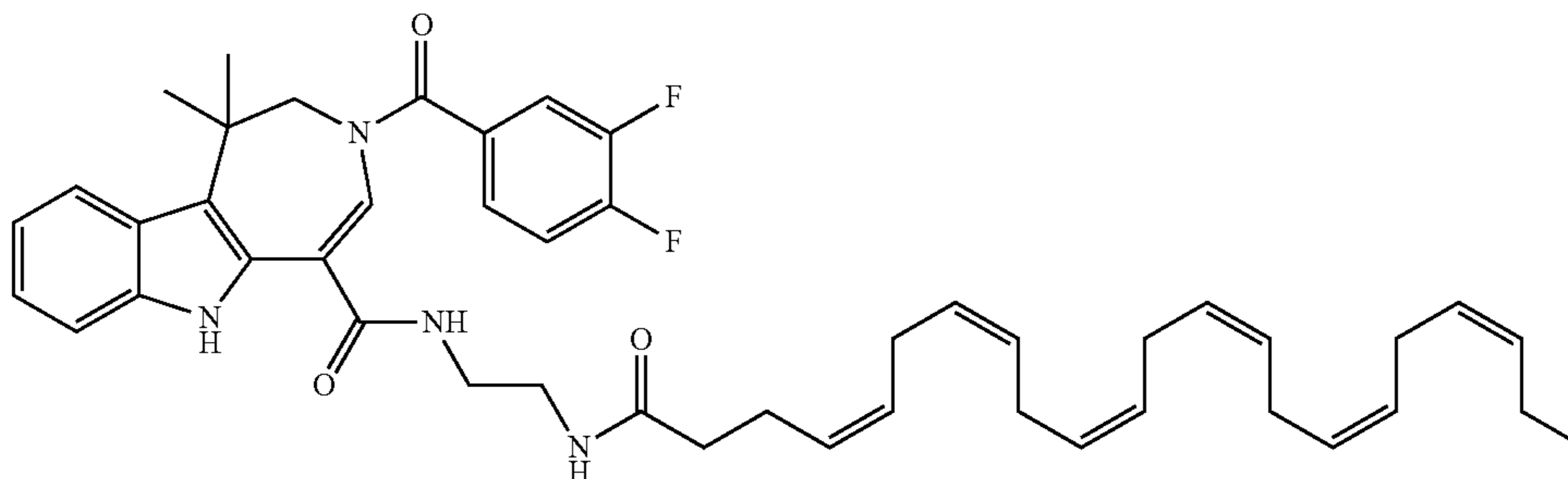
(R,Z)-8-fluoro-1,1-dimethyl-3-(4-(3-morpholinopropoxy)benzoyl)-N-(1-oleoylpyrrolidin-3-yl)-1,2,3,6-tetrahydroazepino[4,5-b]indole-5-carboxamide (II-66)
