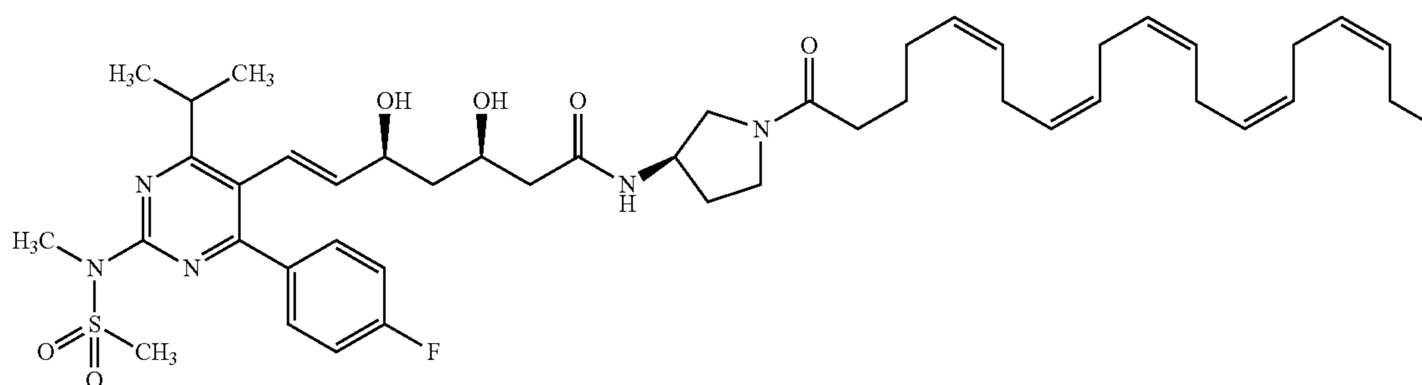
(3R,5S,E)-7-(4-(4-fluorophenyl)-6-isopropyl-2-(N-methylmethylsulfonamido)pyrimidin-5-yl)-3,5-dihydroxy-N-((R)-1-((5Z,8Z,11Z,14Z,17Z)-icosa-5,8,11,14,17-pentaenoyl)pyrrolidin-3-yl)hept-6-enamide (I-62)
