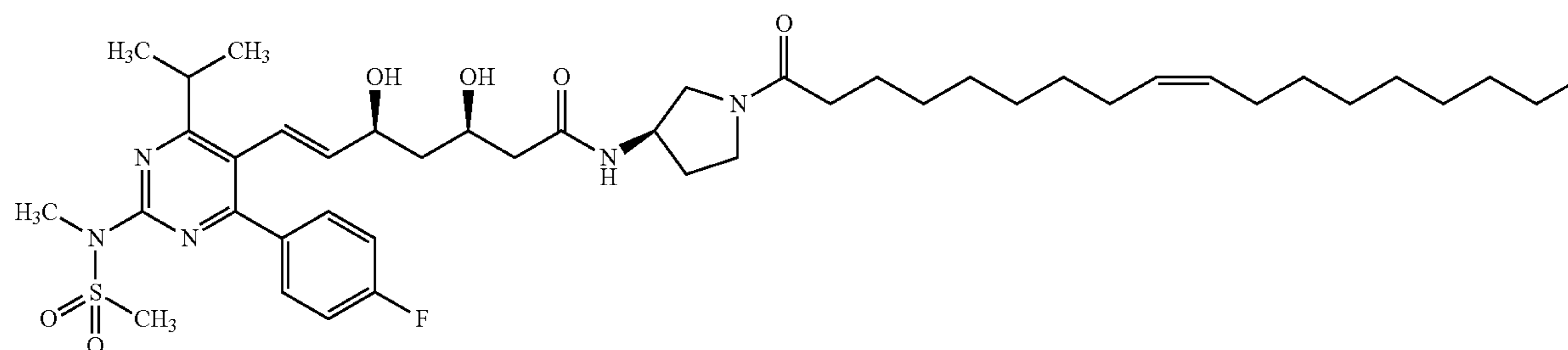
(3R,5S,E)-N-((R)-1-oleoylpyrrolidin-3-yl)-7-(4-(4-fluorophenyl)-6-isopropyl-2-(N-methylmethylsulfonamido)pyrimidin-5-yl)-3,5-dihydroxyhept-6-enamide (I-63)
