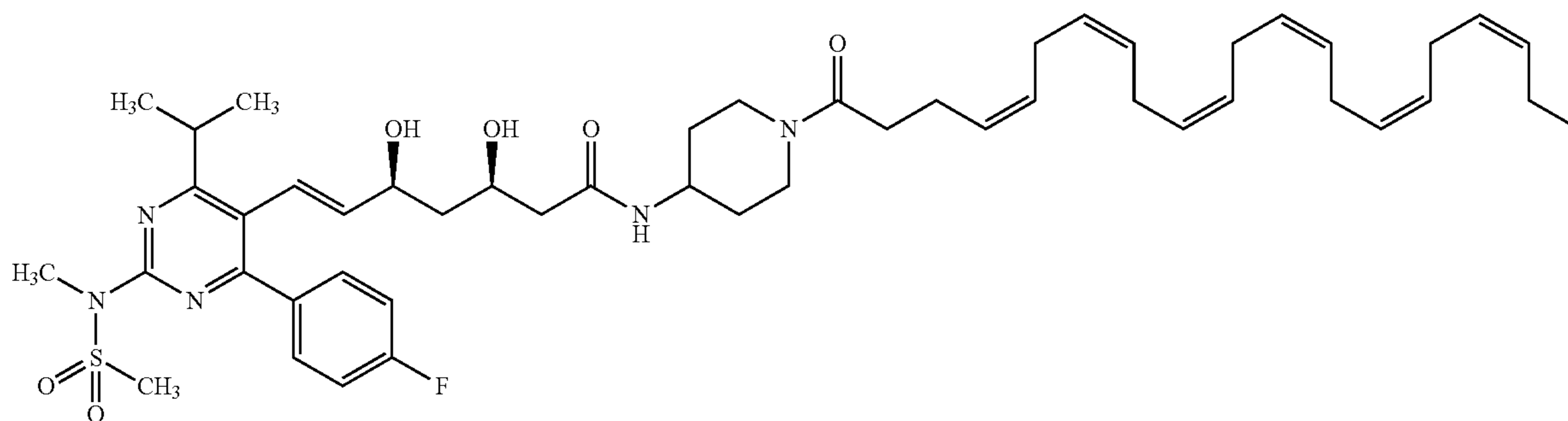
(3R,5S,E)-N-(1-((4Z,7Z,10Z,13Z,16Z,19Z)-docosa-4,7,10,13,16,19-hexaenoyl)piperidin-4-yl)-7-(4-(4-fluorophenyl)-6-isopropyl-2-(N-methylmethylsulfonamido)pyrimidin-5-yl)-3,5-dihydroxyhept-6-enamide (I-58)
