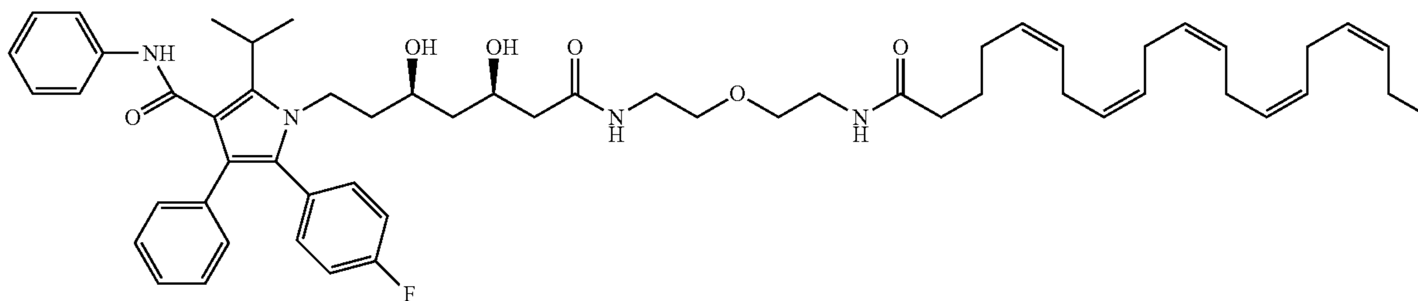
1-((3R,5R)-7((2-(2-((4Z,7Z,10Z,13Z,16Z,19Z)-docosa-4,7, 45 10,13,16,19-hexaenamido)ethoxy)ethyl)amino)-3,5-dihydroxy-7-oxoheptyl)-5-(4-fluorophenyl)-2-isopropyl-N,4-diphenyl-1H-pyrrole-3-carboxamide (I-32)
