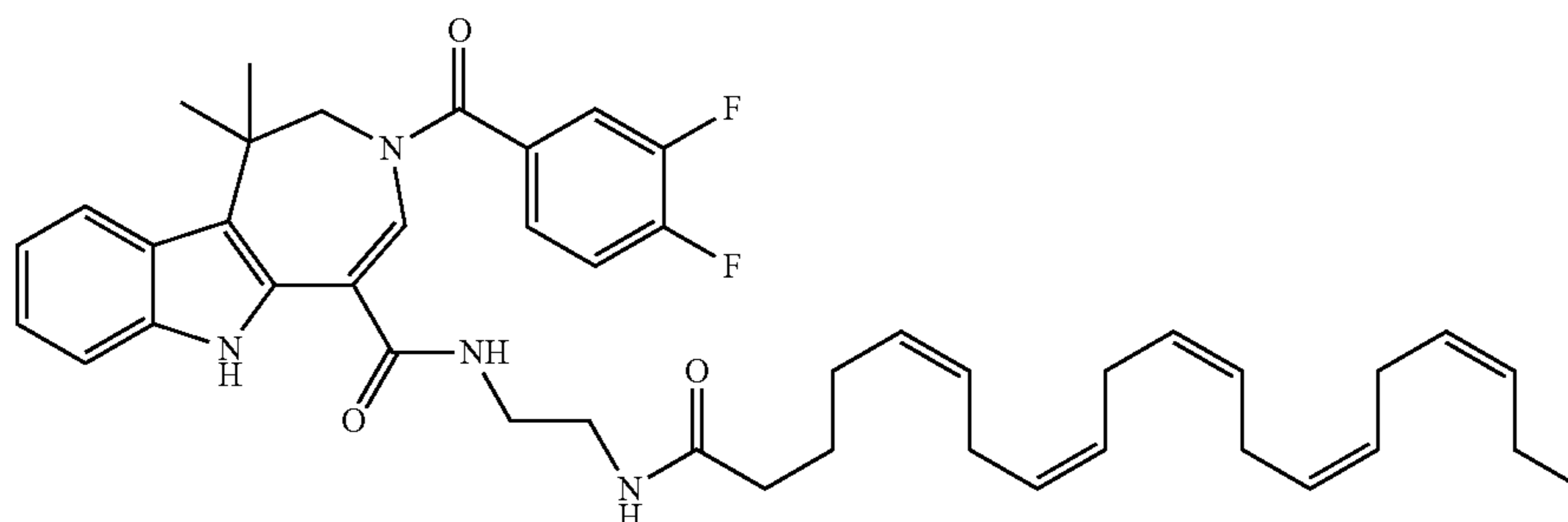
3-(3,4-difluorobenzoyl)-N-(2-((4Z,7Z,10Z,13Z,16Z,19Z)-docosa-4,7,10,13,16,19-hexaenamido)ethyl)-1,1-dimethyl-1,2,3,6-tetrahydroazepino[4,5-b]indole-5-carboxamide (II-67)
