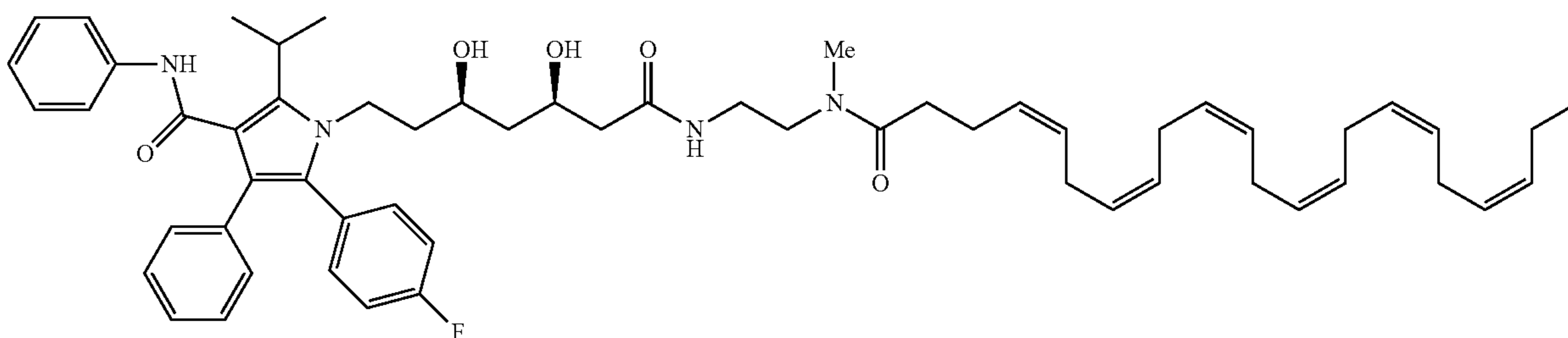
1-((3R,5R)-3,5-dihydroxy-7-((2-oleamidoethyl)amino)-7-oxoheptyl)-5-(4-fluorophenyl)-2-isopropyl-N,4-diphenyl-1H-pyrrole-3-carboxamide (I-24)
