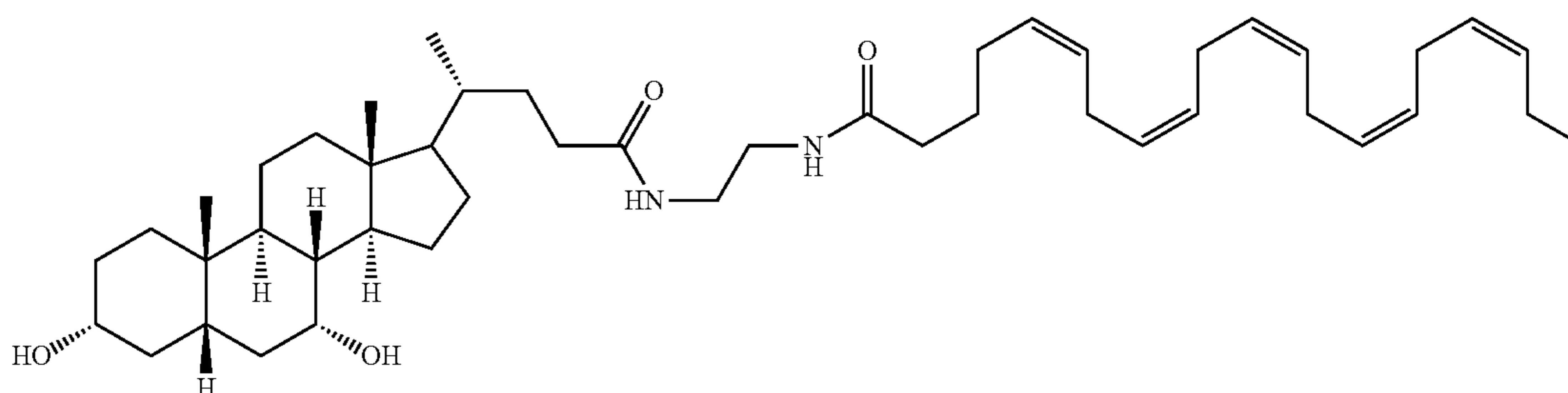
(4Z,7Z,10Z,13Z,16Z,19Z)—N-(2-((4R)-4-((3R,5S,7R,8R,9S,10S,13R,14S)-3,7-dihydroxy-10,13-dimethylhexadecahydro-1H-cyclopenta[a]phenanthren-17-yl)pentanamido)ethyl)docosa-4,7,10,13,16,19-hexaenamide (II-22) 15
