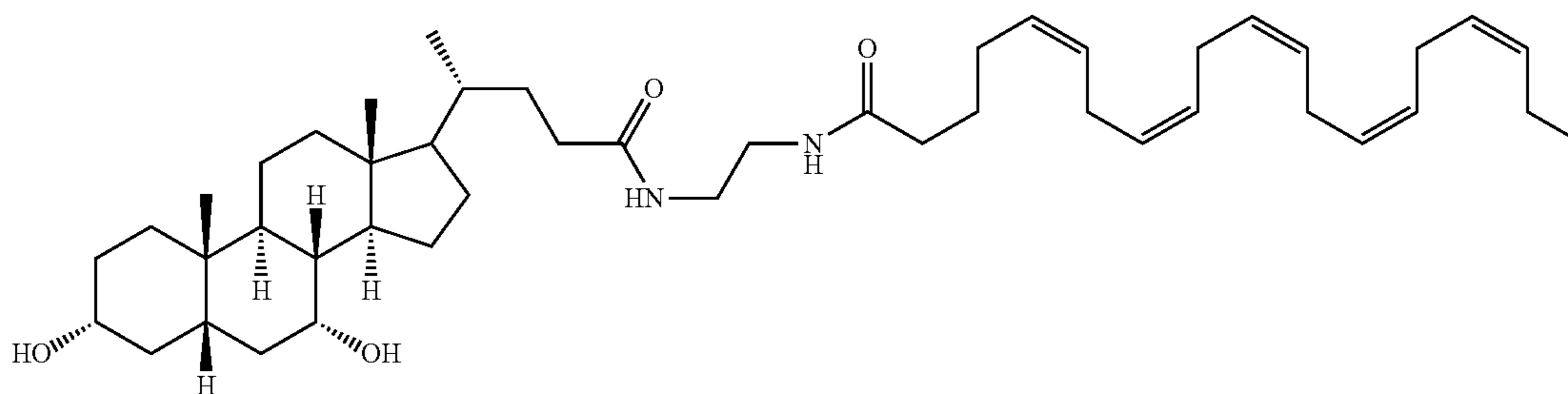
(4Z,7Z,10Z,13Z,16Z,19Z)—N-(2-((4R)-4-((3R,5S,7R,8R,9S,10S,13R,14S)-3,7-dihydroxy-10,13-dimethylhexadecahydro-1H-cyclopenta[a]phenanthren-17-yl)pentanamido)ethyl)docosa-4,7,10,13,16,19-hexaenamide (II-22) 15
