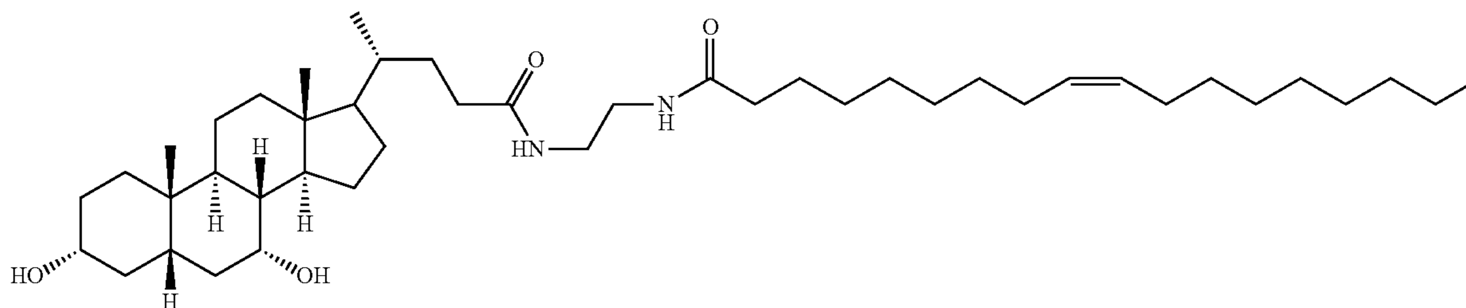
(5Z,8Z,11Z,14Z,17Z)—N-(2-((4R)-4-((3R,5S,7R,8R,9S,10S,13R,14S)-3,7-dihydroxy-10,13-dimethylhexadecahydro-1H-cyclopenta[a]phenanthren-17-yl)pentanamido)ethyl)icosa-5,8,11,14,17-pentaenamide (II-23) 30
