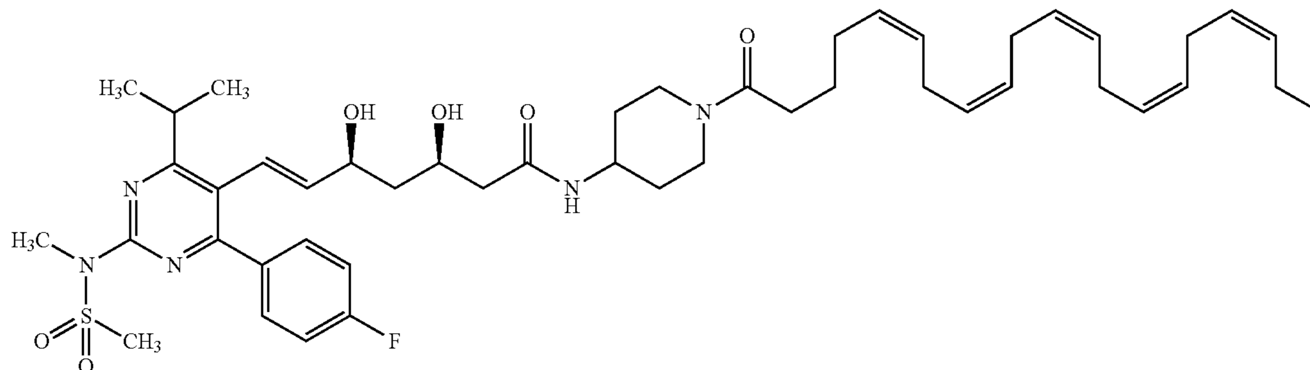
(3R,5S,E)-7-(4-(4-fluorophenyl)-6-isopropyl-2-(N-methylmethylsulfonamido)pyrimidin-5-yl)-3,5-dihydroxy-N-(1-((5Z,8Z,11Z,14Z,17Z)-icosa-5,8,11,14,17-pentaenoyl)piperidin-4-yl)hept-6-enamide (I-59)
