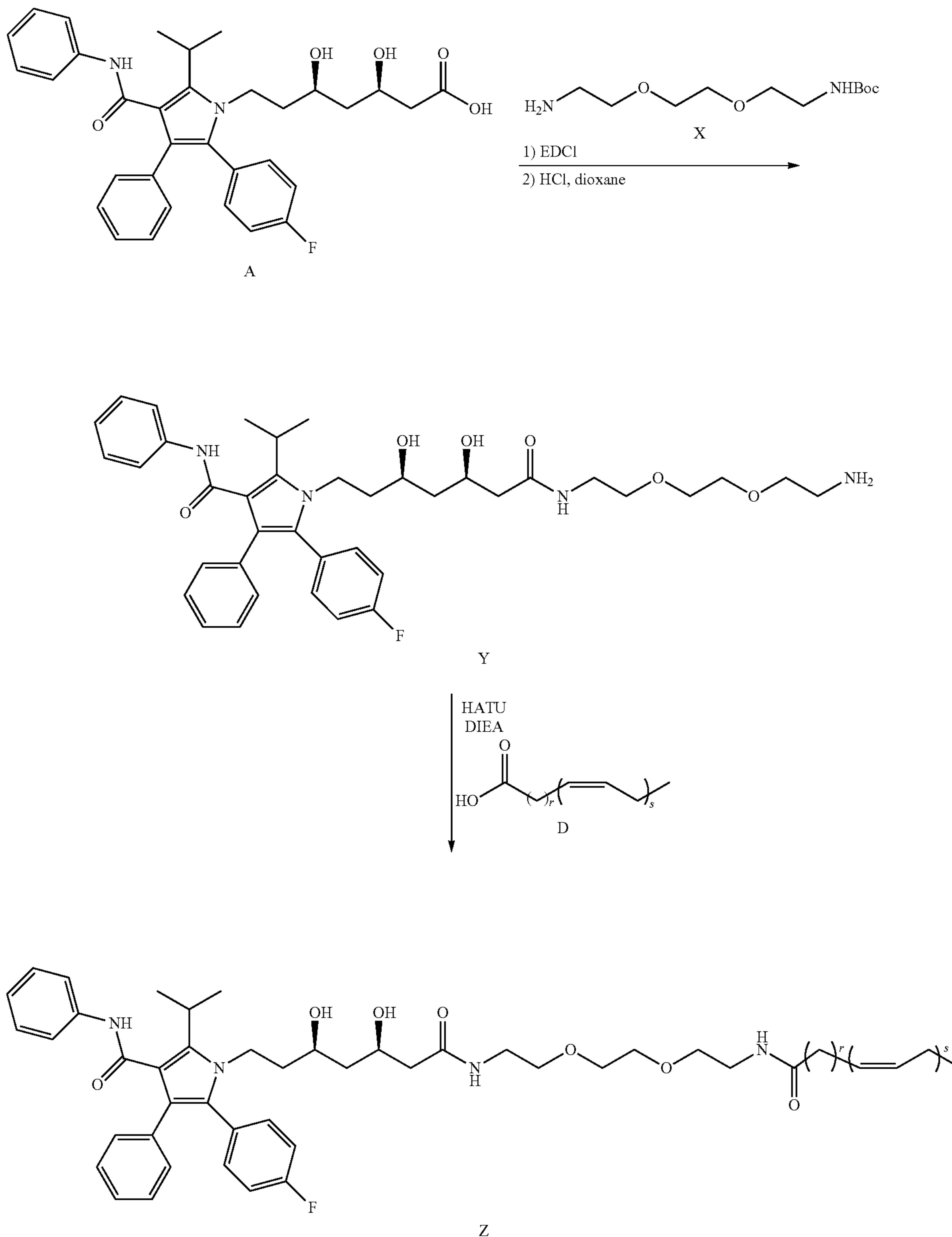
Scheme 7
