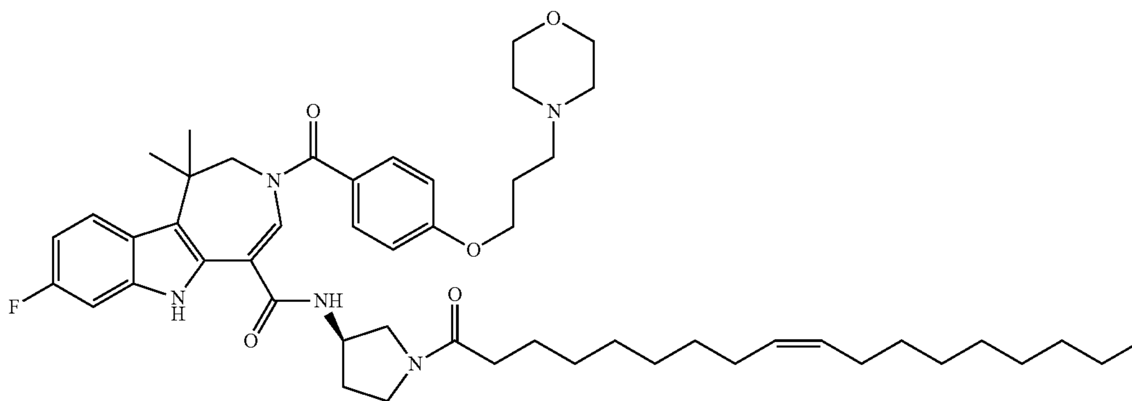
(R,Z)-8-fluoro-1,1-dimethyl-3-(4-(3-morpholinopropoxy)benzoyl)-N-(1-oleoylpyrrolidin-3-yl)-1,2,3,6-tetrahydroazepino[4,5-b]indole-5-carboxamide (II-66)
