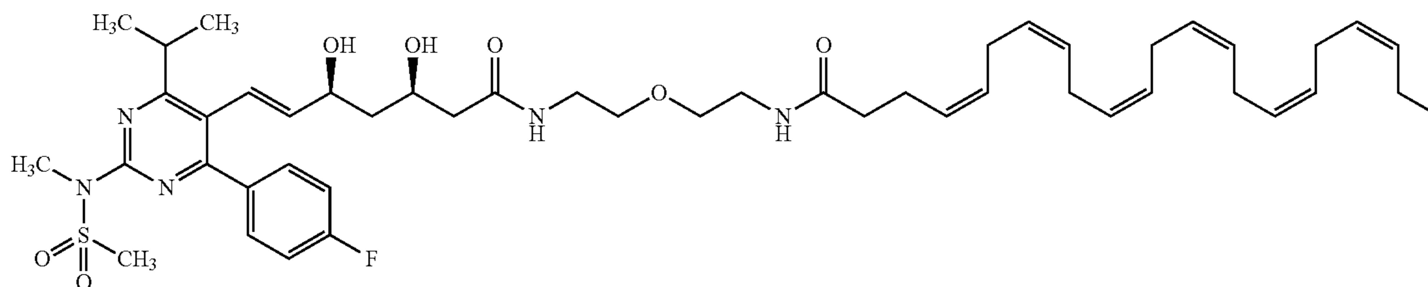
N-(2-(2-((3R,5S,E)-7-(4-(4-fluorophenyl)-6-isopropyl-2-(N-methylmethylsulfonamido)pyrimidin-5-yl)-3,5-dihydroxyhept-6-enamido)ethoxy)ethyl)oleamide (I-52)
