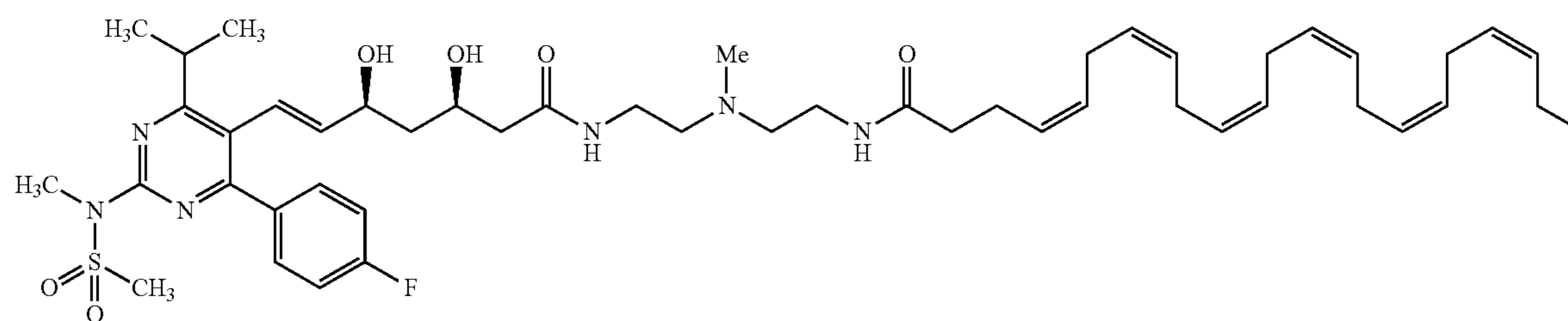
(4Z,7Z,10Z,13Z,16Z,19Z)—N-(2-((2-((3R,5S,E)-7-(4-(4-fluorophenyl)-6-isopropyl-2-(N-methylmethylsulfonamido)pyrimidin-5-yl)-3,5-dihydroxyhept-6-enamido)ethyl)(methylamino)ethyl)docosa-4,7,10,13,16,19-hexaenamide (I-49) 30
