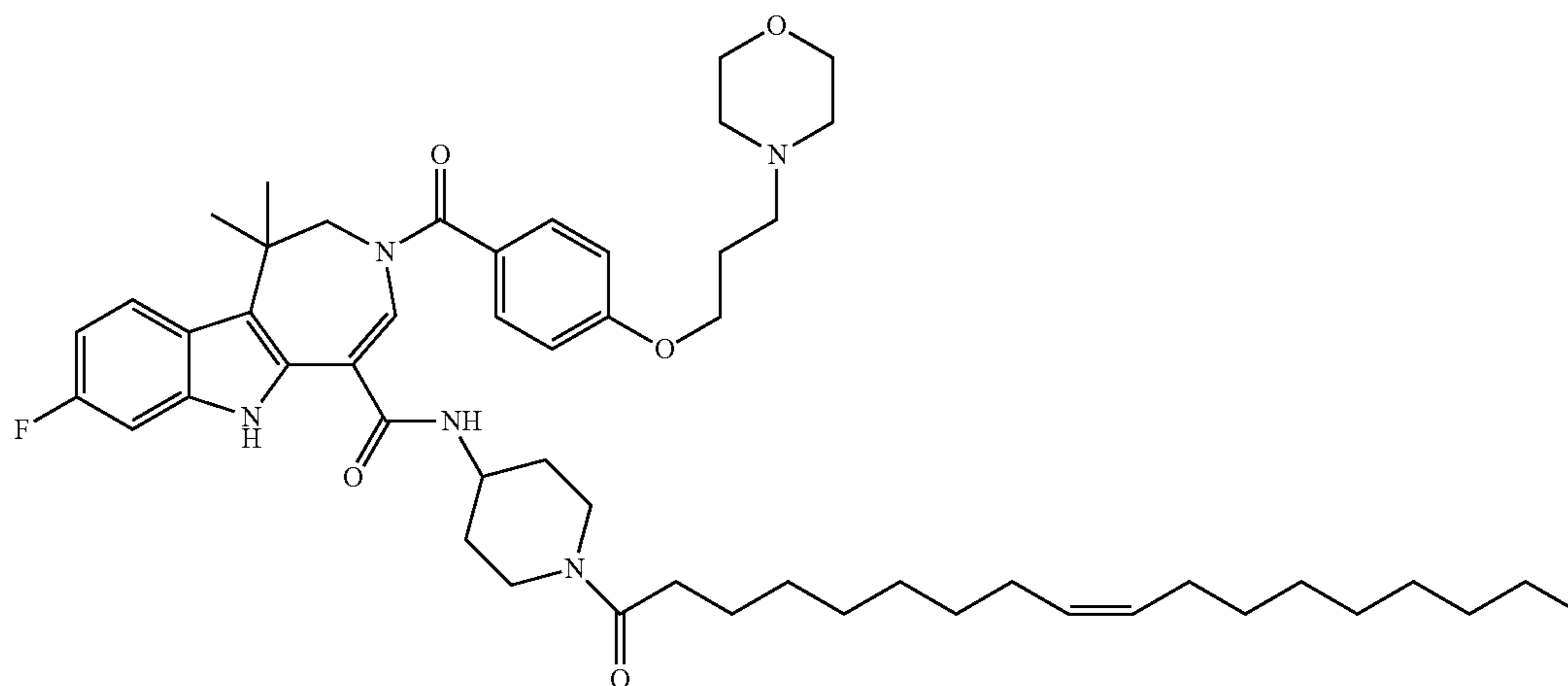
(Z)-8-fluoro-1,1-dimethyl-3-(4-(3-morpholinopropoxy)benzoyl)-N-(1-oleoylpiperidin-4-yl)-1,2,3,6-tetrahydroazepino[4,5-b]indole-5-carboxamide (II-63)
