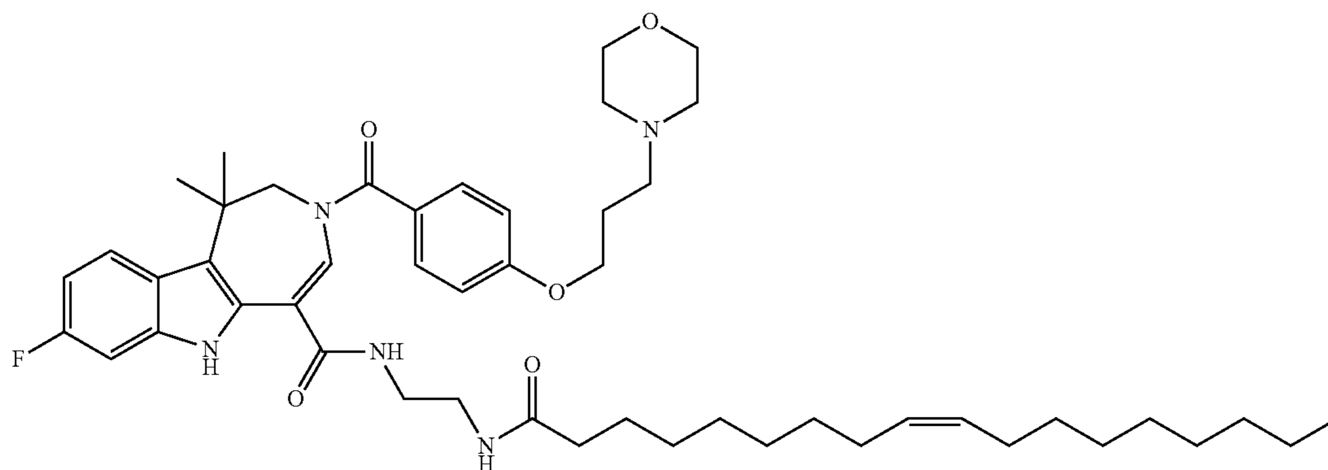
(Z)-8-fluoro-1,1-dimethyl-3-(4-(3-morpholinopropoxy)benzoyl)-N-(2-oleamidoethyl)-1,2,3,6-tetrahydroazepino[4,5-b]indole-5-carboxamide (II-60)
