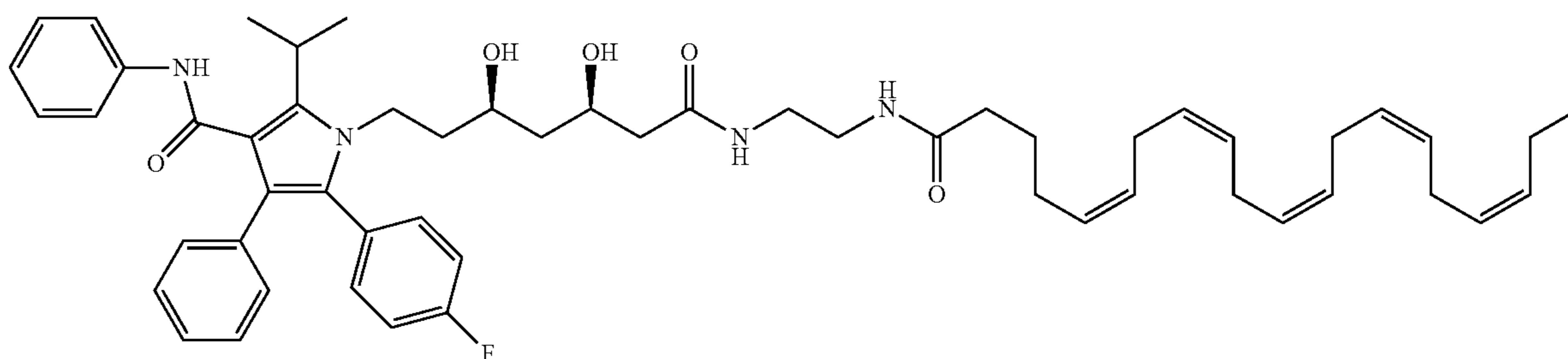
1-((3R,5R)-7-((2-((4Z,7Z,10Z,13Z,16Z,19Z)-docosa-4,7,10,13,16,19-hexaenamido)ethyl)amino)-3,5-dihydroxy-7-oxoheptyl)-5-(4-fluorophenyl)-2-isopropyl-N,4-diphenyl-1H-pyrrole-3-carboxamide (I-22) 15
