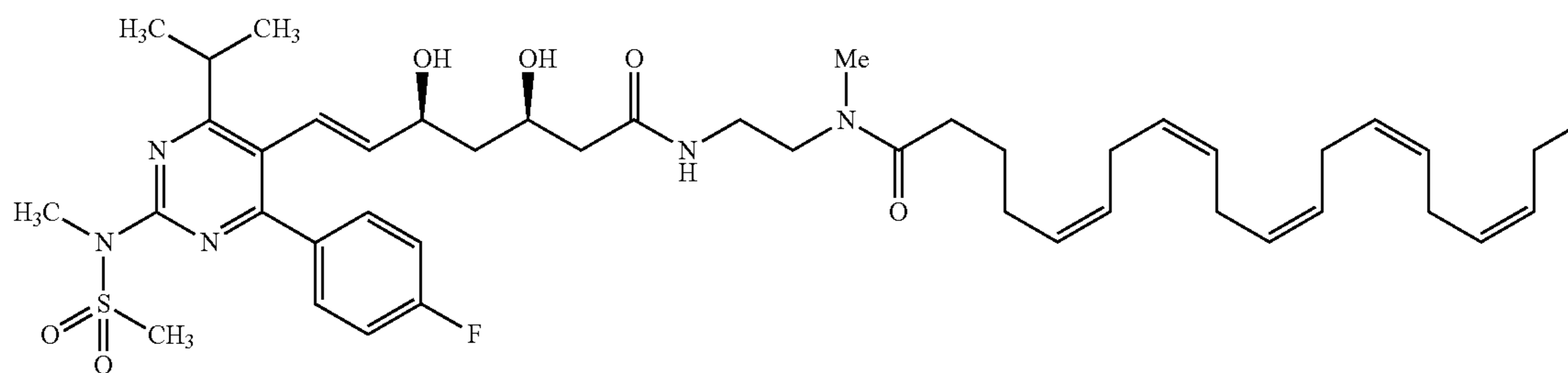
(5Z,8Z,11Z,14Z,17Z)—N-(2-((3R,5S,E)-7-(4-(4-fluorophenyl)-6-isopropyl-2-(N-methylmethylsulfonamido)pyrimidin-5-yl)-3,5-dihydroxyhept-6-enamido)ethyl)-N-methyl-icos-5,8,11,14,17-pentaenamide (I-48) 15
