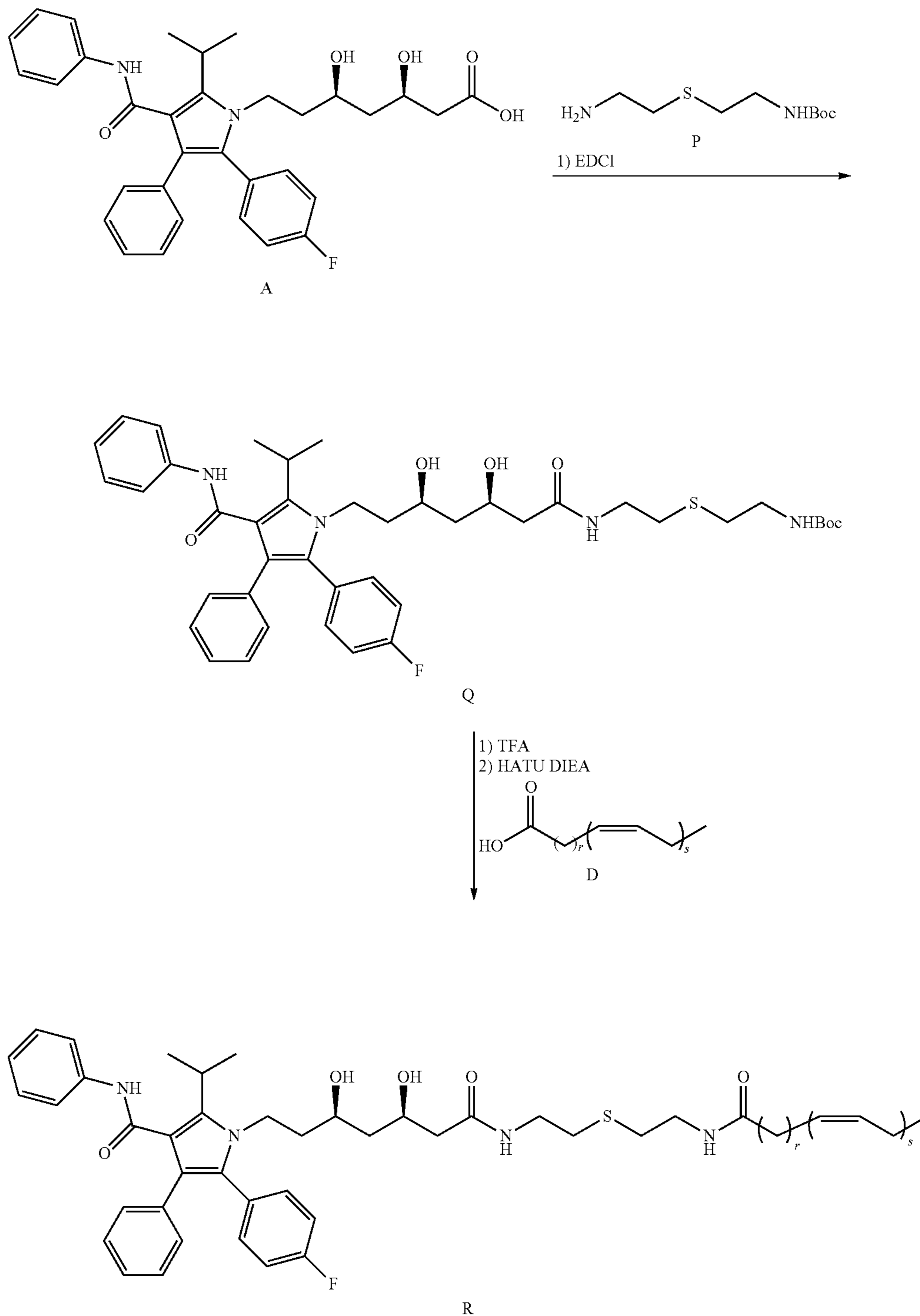
Scheme 5
