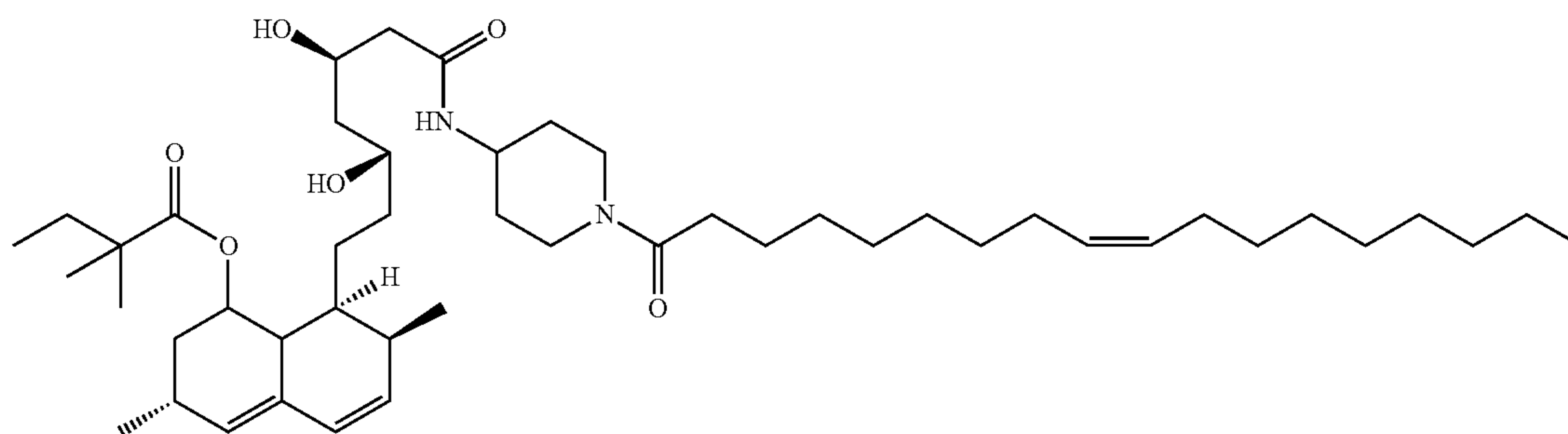
(3R,7S,8S)-8-((3S,5R)-3,5-dihydroxy-7-((1-((5Z,8Z,11Z,14Z,17Z)-icoso-5,8,11,14,17-pentaenoyl)piperidin-4-yl)amino)-7-oxoheptyl)-3,7-dimethyl-1,2,3,7,8,8a-hexahydronaphthalen-1-yl 2,2-dimethylbutanoate (I-17)
