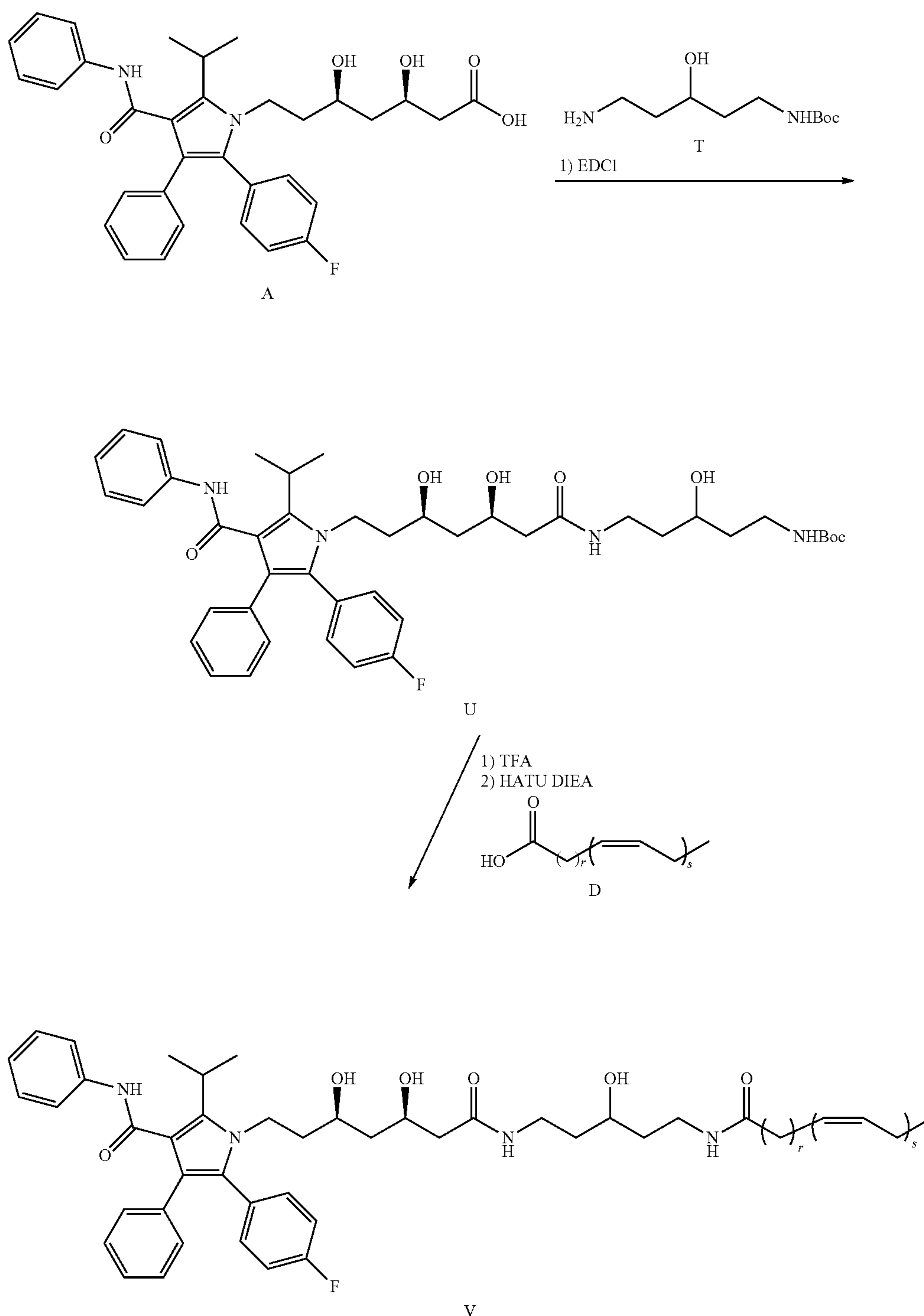
Scheme 6
