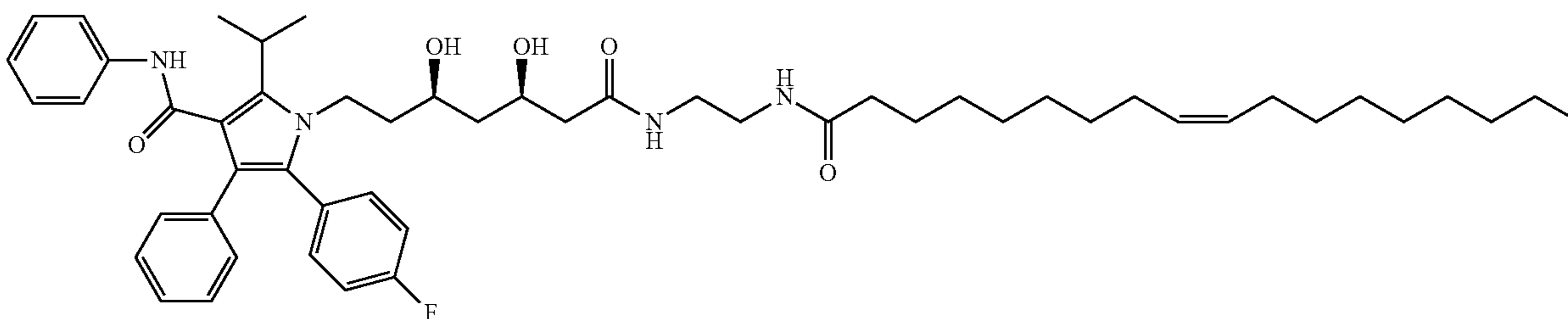
1-((3R,5R)-3,5-dihydroxy-7-((2-((5Z,8Z,11Z,14Z,17Z)-icosa-5,8,11,14,17-pentaenamido)ethyl)amino)-7-oxoheptyl)-5-(4-fluorophenyl)-2-isopropyl-N,4-diphenyl-1H-pyrrole-3-carboxamide (I-23) 30
