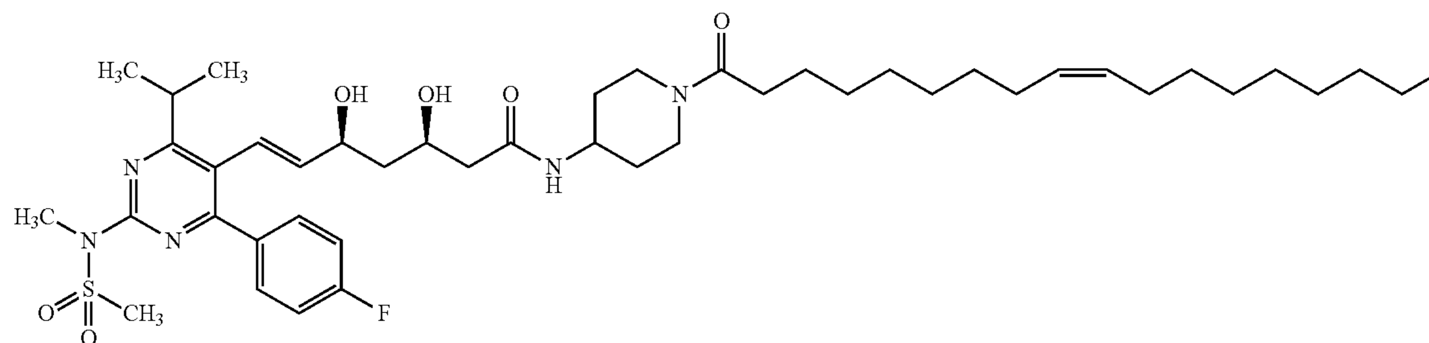
(3R,5S,E)-7-(4-(4-fluorophenyl)-6-isopropyl-2-(N-methylmethylsulfonamido)pyrimidin-5-yl)-3,5-dihydroxy-N-(1-oleoylpiperidin-4-yl)hept-6-enamide (I-60)
