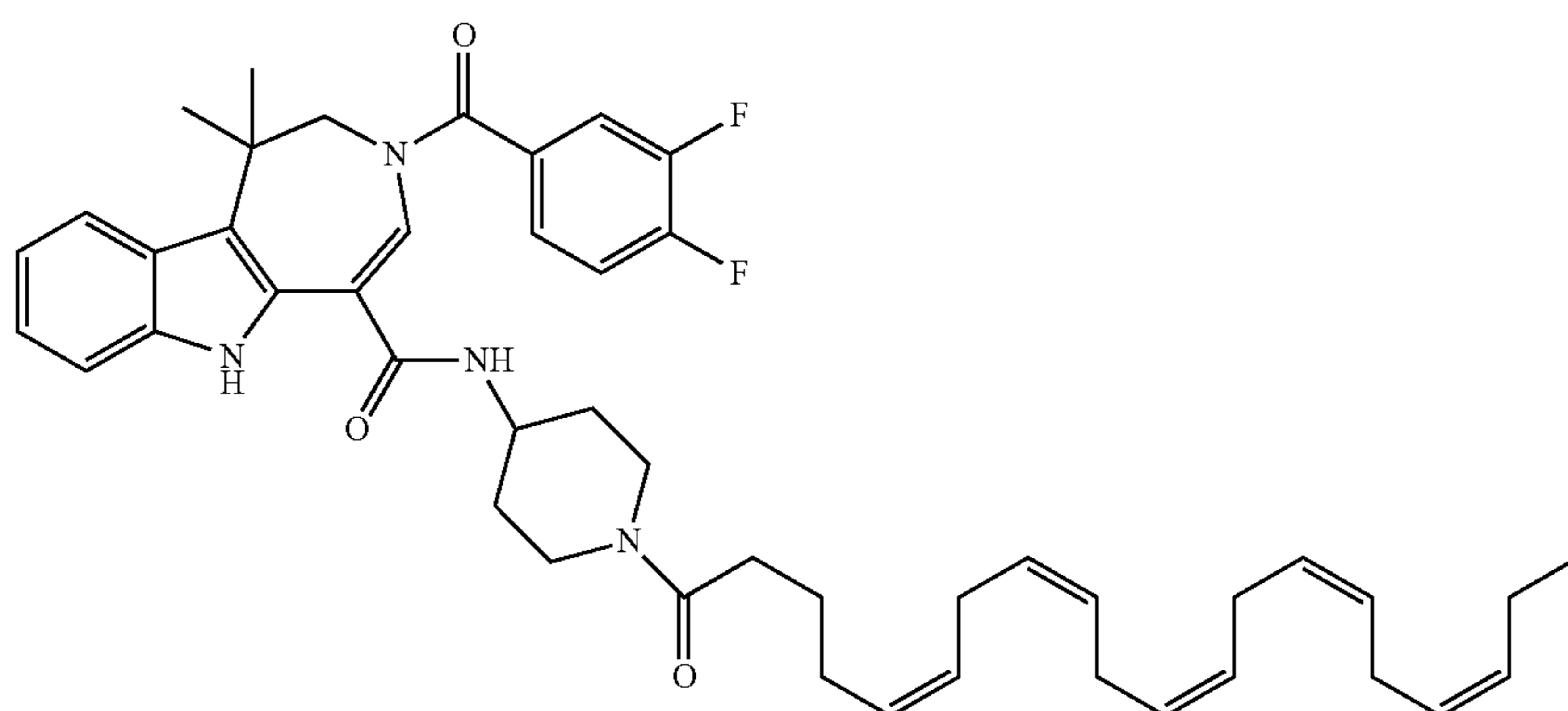
3-(3,4-difluorobenzoyl)-N-(1-((4Z,7Z,10Z,13Z,16Z,19Z)-docosa-4,7,10,13,16,19-hexaenoyl)piperidin-4-yl)-1,1-dimethyl-1,2,3,6-tetrahydroazepino[4,5-b]indole-5-carboxamide (II-70) 20
