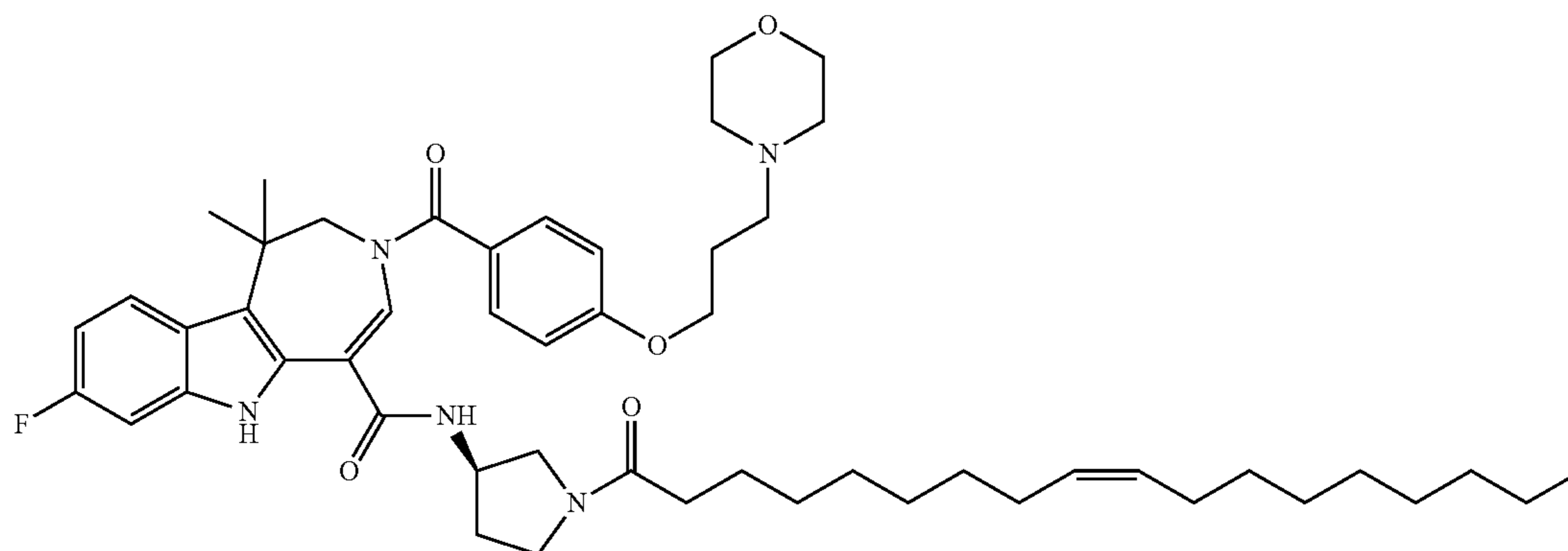
(R,Z)-8-fluoro-1,1-dimethyl-3-(4-(3-morpholinopropoxy)benzoyl)-N-(1-oleoylpyrrolidin-3-yl)-1,2,3,6-tetrahydroazepino[4,5-b]indole-5-carboxamide (II-66)
