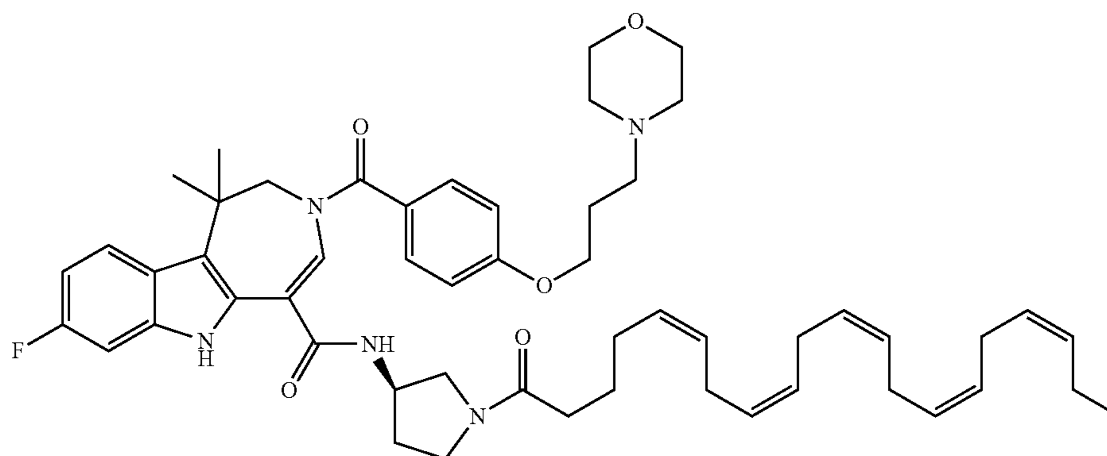
N-((R)-1-((4Z,7Z,10Z,13Z,16Z,19Z)-docosa-4,7,10,13,16,19-hexaenoyl)pyrrolidin-3-yl)-8-fluoro-1,1-dimethyl-3-(4-(3-morpholinopropoxy)benzoyl)-1,2,3,6-tetrahydroazepino[4,5-b]indole-5-carboxamide (II-64)
