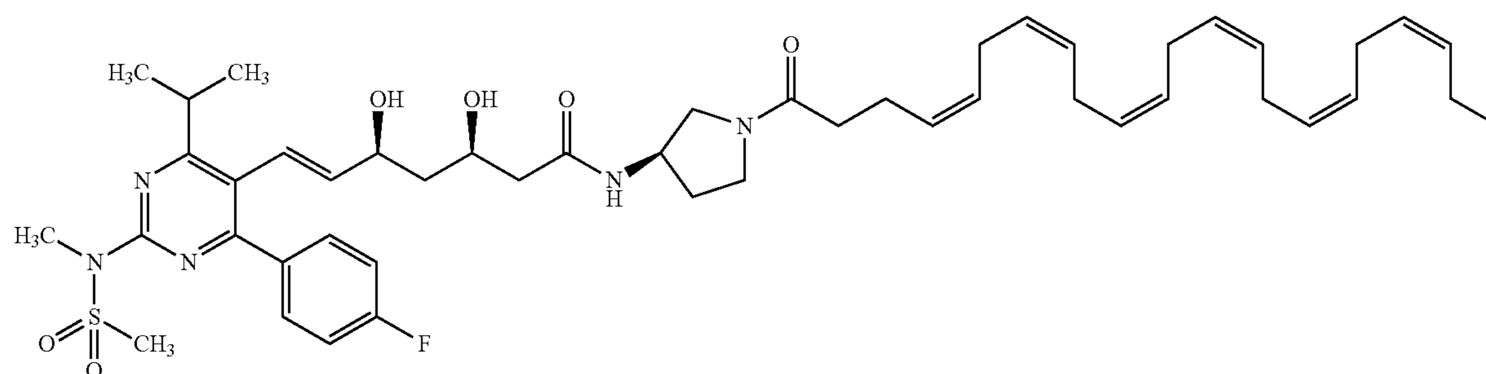
(3R,5S,E)-N-((R)-1-((4Z,7Z,10Z,13Z,16Z,19Z)-docosa-4,7,10,13,16,19-hexaenoyl)pyrrolidin-3-yl)-7-(4-(4-fluorophenyl)-6-isopropyl-2-(N-methylmethylsulfonamido)pyrimidin-5-yl)-3,5-dihydroxyhept-6-enamide (I-61)
