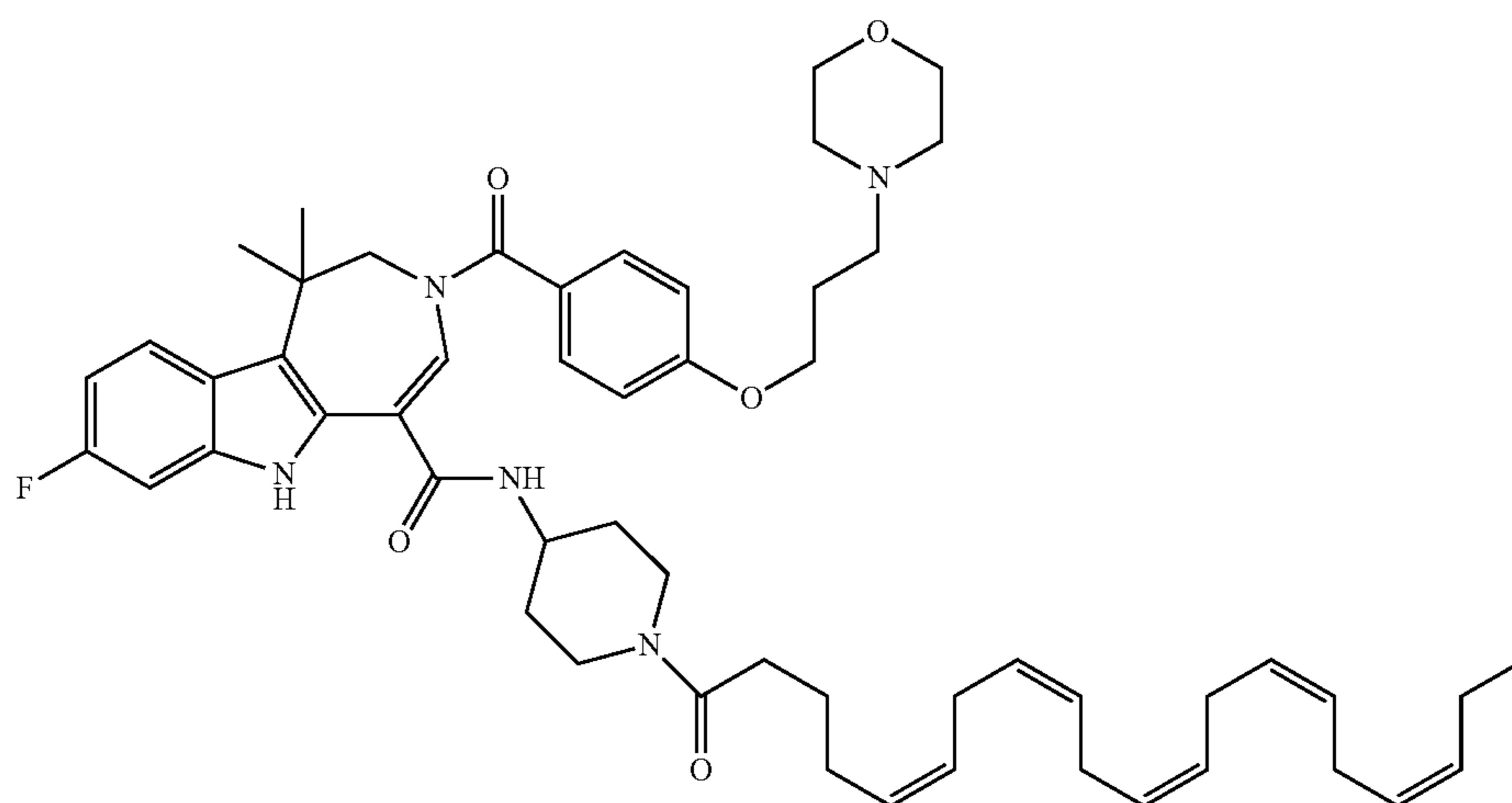
8-fluoro-N-(1-((5Z,8Z,11Z,14Z,17Z)-icosa-5,8,11,14,17-pentaenoyl)piperidin-4-yl)-1,1-dimethyl-3-(4-(3-morpholinopropoxy)benzoyl)-1,2,3,6-tetrahydroazepino[4,5-b]indole-5-carboxamide (II-62)
