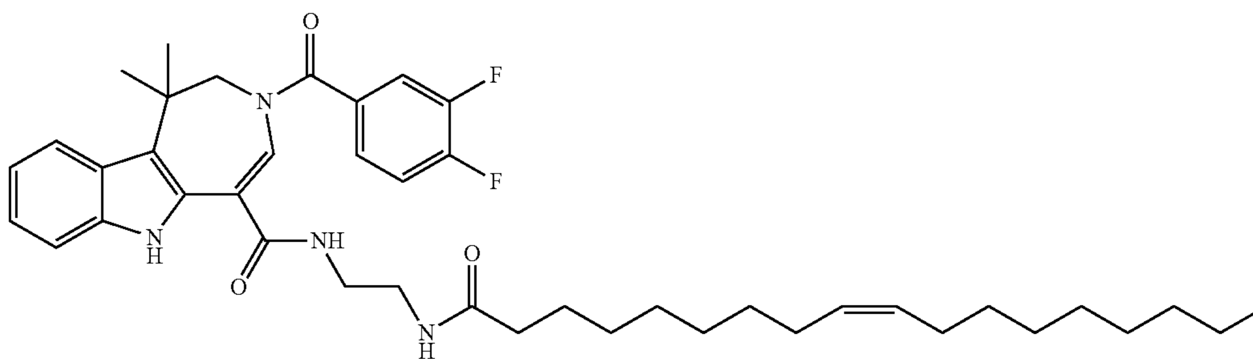
3-(3,4-difluorobenzoyl)-N-(2-((5Z,8Z,11Z,14Z,17Z)-icosa-5,8,11,14,17-pentaenamido)ethyl)-1,1-dimethyl-1,2,3,6-tetrahydroazepino[4,5-b]indole-5-carboxamide (II-68)
