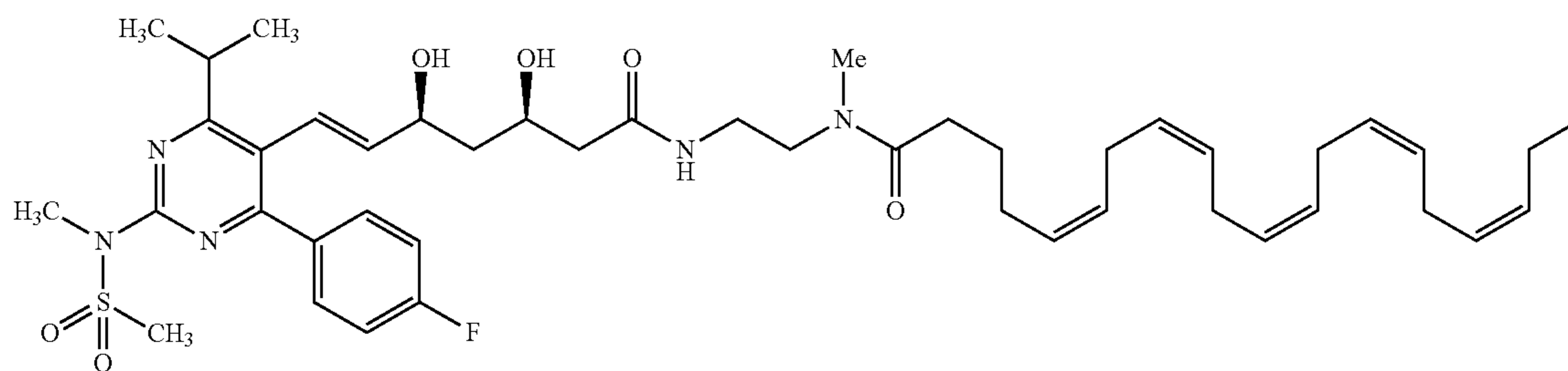
(5Z,8Z,11Z,14Z,17Z)—N-(2-((3R,5S,E)-7-(4-(4-fluorophenyl)-6-isopropyl-2-(N-methylmethylsulfonamido)pyrimidin-5-yl)-3,5-dihydroxyhept-6-enamido)ethyl)-N-methyl-icos-5,8,11,14,17-pentaenamide (I-48) 15
