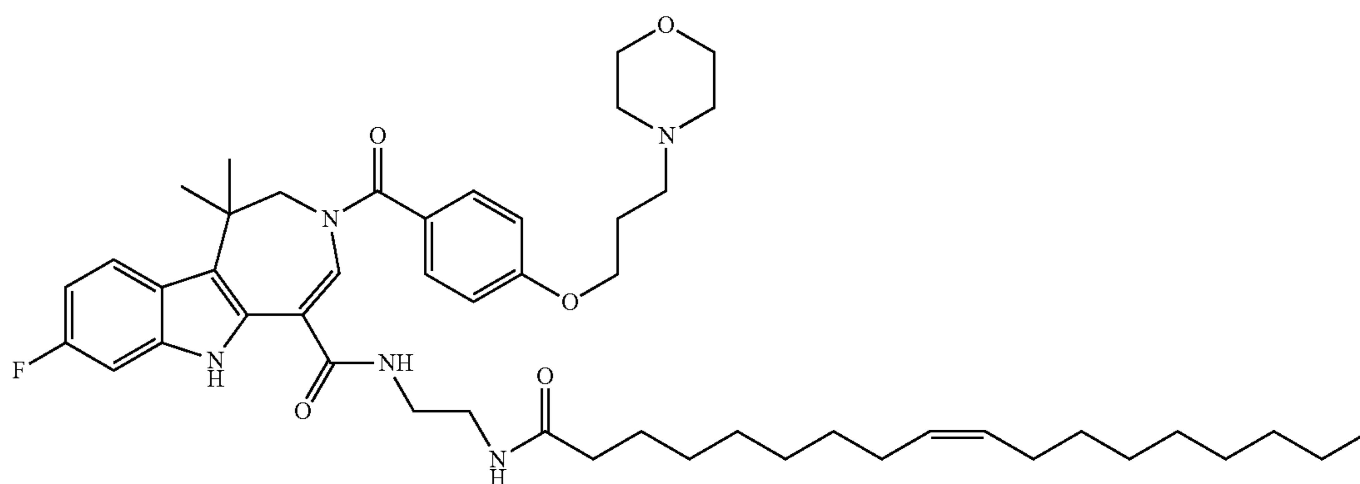
(Z)-8-fluoro-1,1-dimethyl-3-(4-(3-morpholinopropoxy)benzoyl)-N-(2-oleamidoethyl)-1,2,3,6-tetrahydroazepino[4,5-b]indole-5-carboxamide (II-60)
