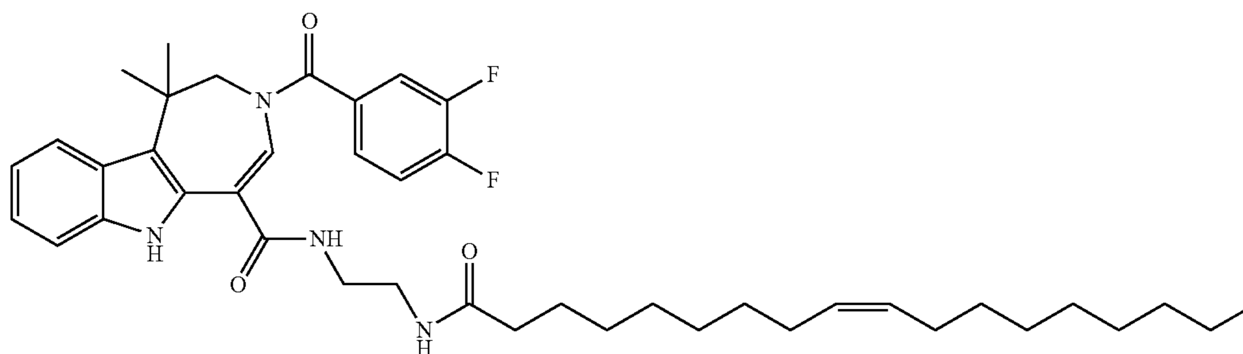
3-(3,4-difluorobenzoyl)-N-(2-((5Z,8Z,11Z,14Z,17Z)-icosa-5,8,11,14,17-pentaenamido)ethyl)-1,1-dimethyl-1,2,3,6-tetrahydroazepino[4,5-b]indole-5-carboxamide (II-68)
