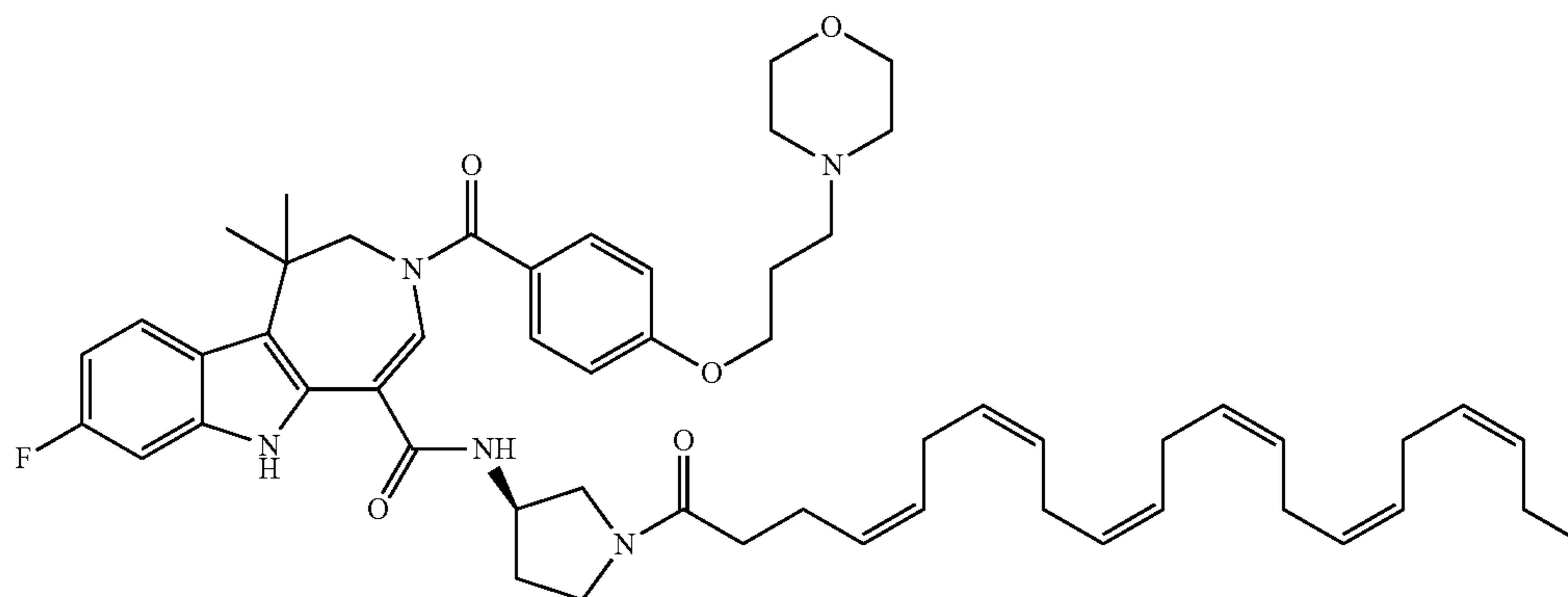
(Z)-8-fluoro-1,1-dimethyl-3-(4-(3-morpholinopropoxy)benzoyl)-N-(1-oleoylpiperidin-4-yl)-1,2,3,6-tetrahydroazepino[4,5-b]indole-5-carboxamide (II-63)
