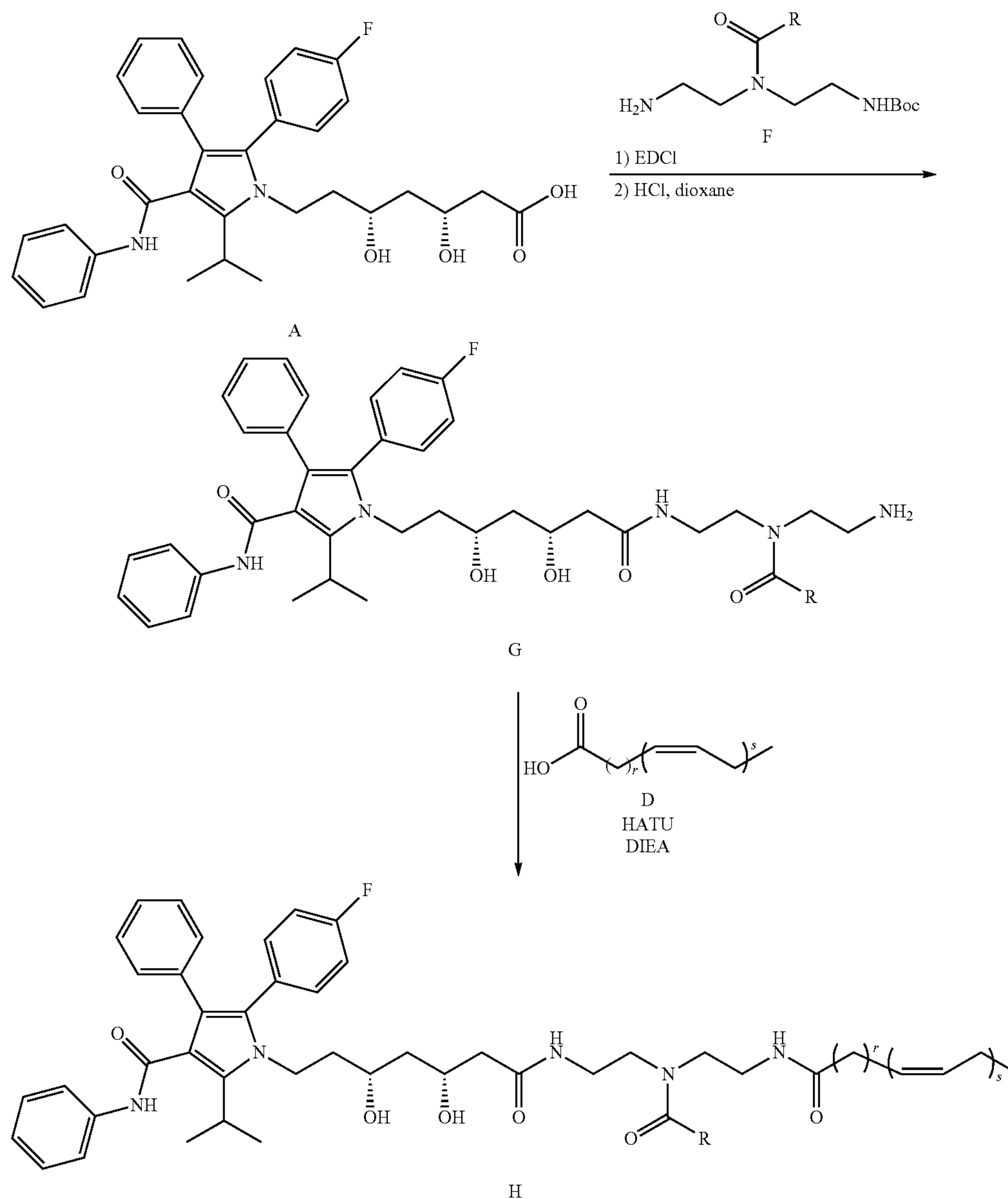
Scheme 2
