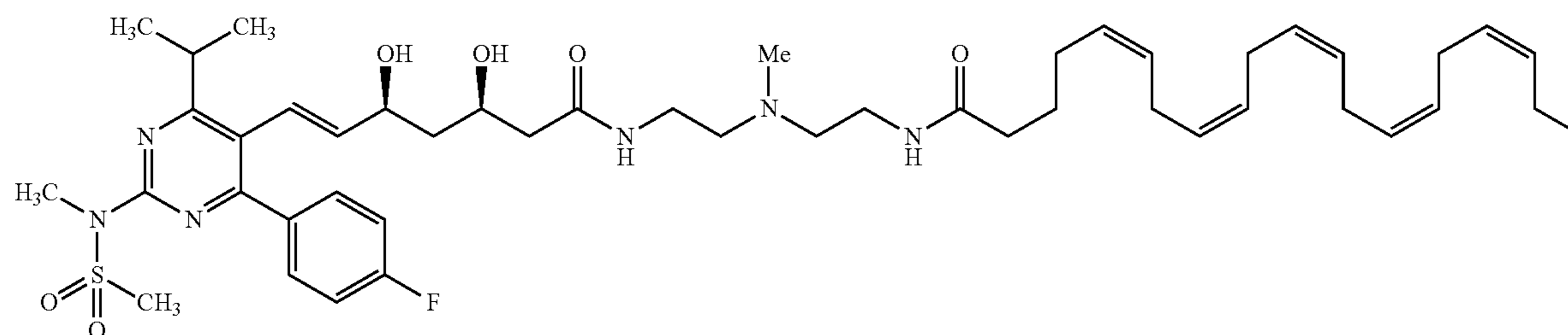
(4Z,7Z,10Z,13Z,16Z,19Z)—N-(2-((2-((3R,5S,E)-7-(4-(4-fluorophenyl)-6-isopropyl-2-(N-methylmethylsulfonamido)pyrimidin-5-yl)-3,5-dihydroxyhept-6-enamido)ethyl)(methylamino)ethyl)docosa-4,7,10,13,16,19-hexaenamide (I-49) 30
