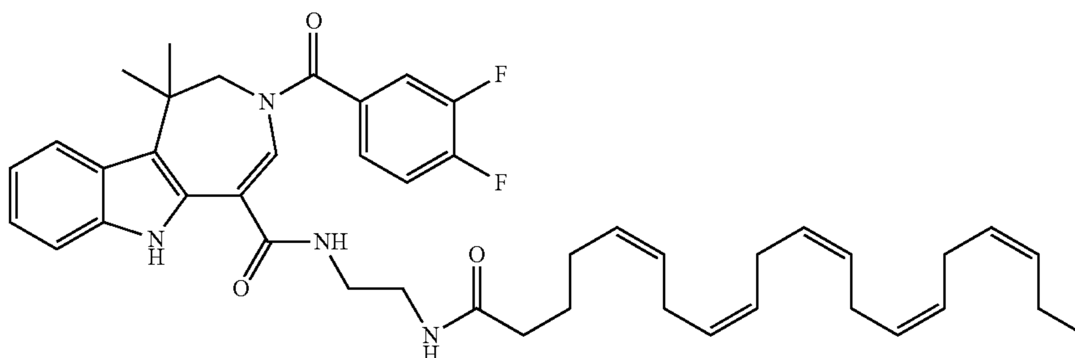
3-(3,4-difluorobenzoyl)-N-(2-((4Z,7Z,10Z,13Z,16Z,19Z)-docosa-4,7,10,13,16,19-hexaenamido)ethyl)-1,1-dimethyl-1,2,3,6-tetrahydroazepino[4,5-b]indole-5-carboxamide (II-67)
