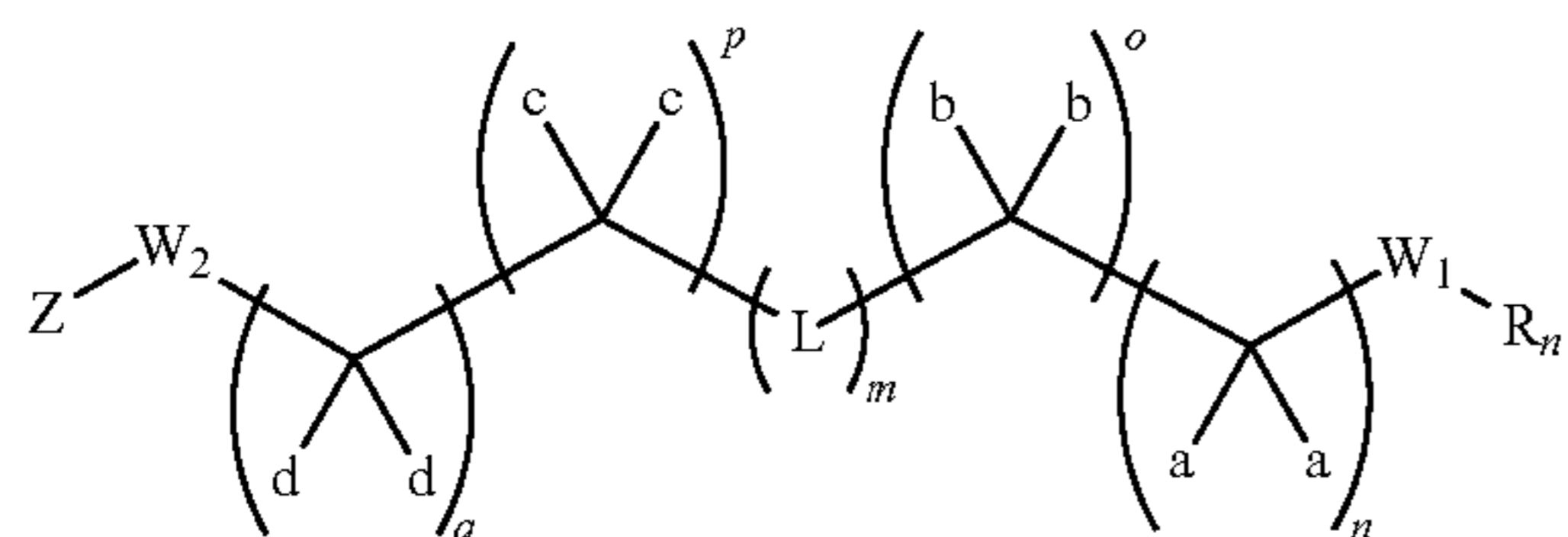
Formula I
