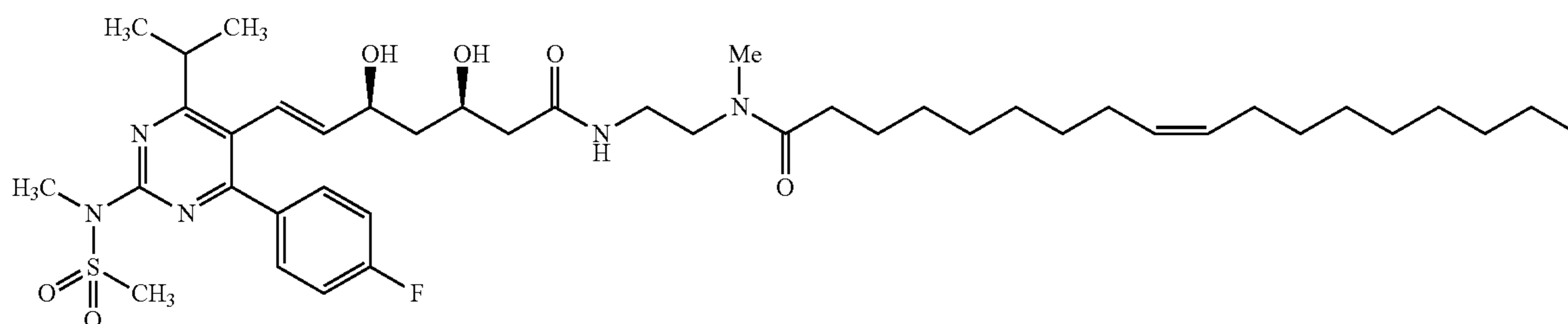
N-(2-((3R,5S,E)-7-(4-(4-fluorophenyl)-6-isopropyl-2-(N-methylmethylsulfonamido)pyrimidin-5-yl)-3,5-dihydroxyhept-6-enamido)ethyl)oleamide (I-45) 30
