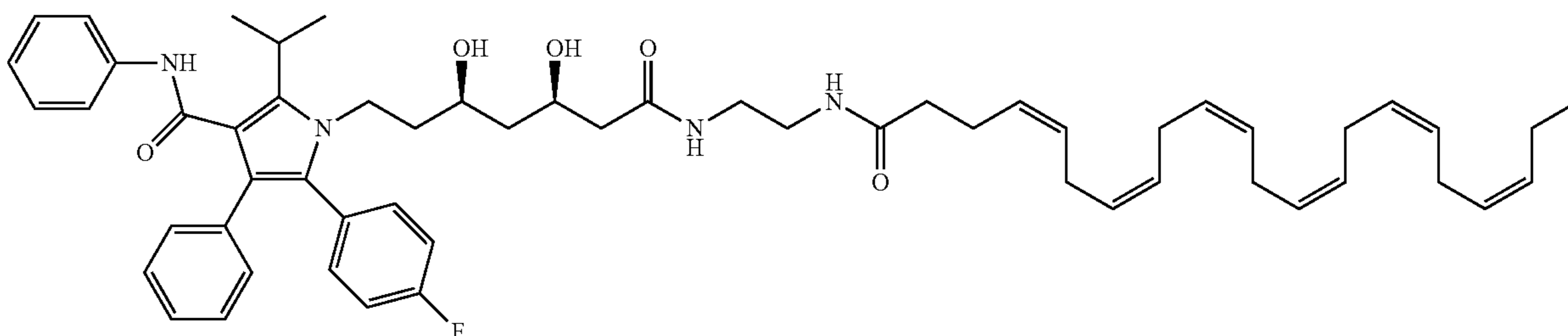
1-((3R,5R)-7-((2-((4Z,7Z,10Z,13Z,16Z,19Z)-docosa-4,7,10,13,16,19-hexaenamido)ethyl)amino)-3,5-dihydroxy-7-oxoheptyl)-5-(4-fluorophenyl)-2-isopropyl-N,4-diphenyl-1H-pyrrole-3-carboxamide (I-22) 15
