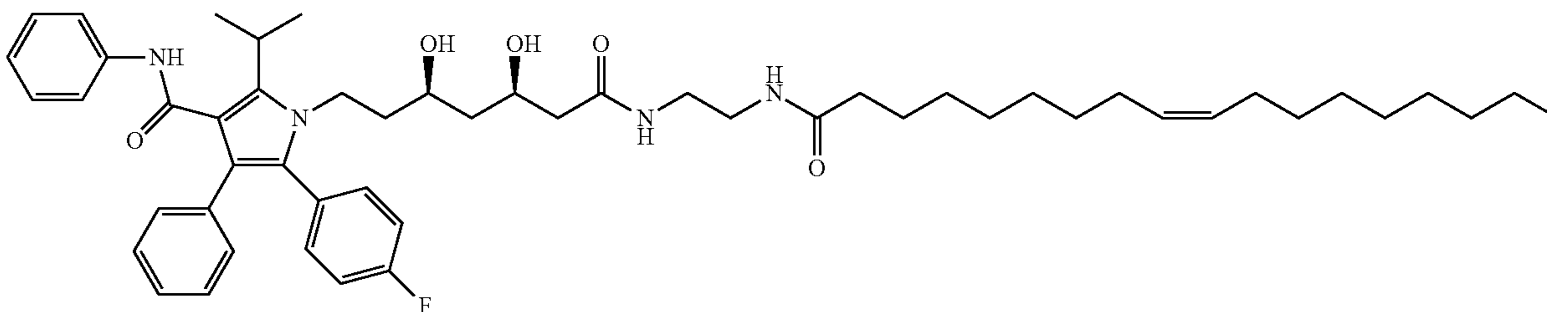
1-((3R,5R)-3,5-dihydroxy-7-((2-((5Z,8Z,11Z,14Z,17Z)-icosa-5,8,11,14,17-pentaenamido)ethyl)amino)-7-oxoheptyl)-5-(4-fluorophenyl)-2-isopropyl-N,4-diphenyl-1H-pyrrole-3-carboxamide (I-23) 30
