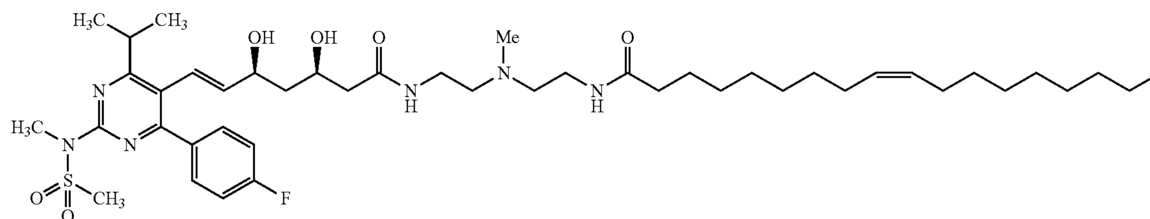
(5Z,8Z,11Z,14Z,17Z)—N-(2-((2-((3R,5S,E)-7-(4-(4-fluorophenyl)-6-isopropyl-2-(N-methylmethylsulfonamido)pyrimidin-5-yl)-3,5-dihydroxyhept-6-enamido)ethyl)(methylamino)ethyl)icosa-5,8,11,14,17-pentaenamide (I-50)
