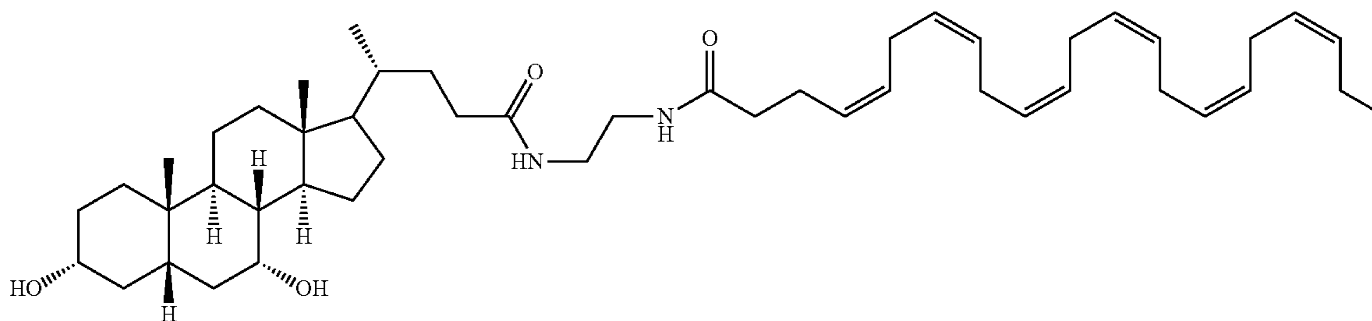
(4Z,7Z,10Z,13Z,16Z,19Z)—N-(2-((4R)-4-((3R,5S,7R,8R,9S,10S,13R,14S)-3,7-dihydroxy-10,13-dimethylhexadecahydro-1H-cyclopenta[a]phenanthren-17-yl)pentanamido)ethyl)docosa-4,7,10,13,16,19-hexaenamide (II-22) 15
