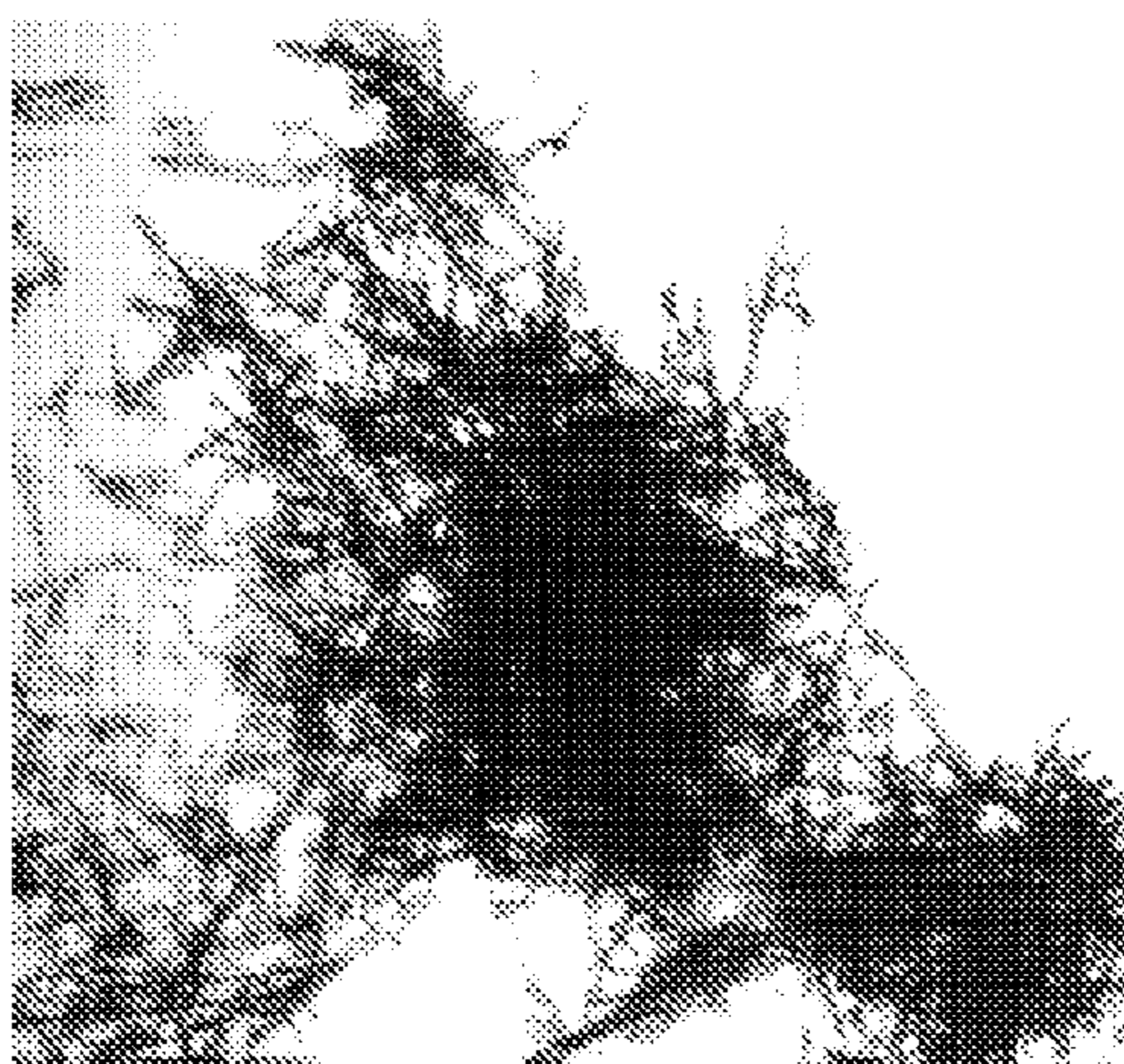
Crystal Form 1
