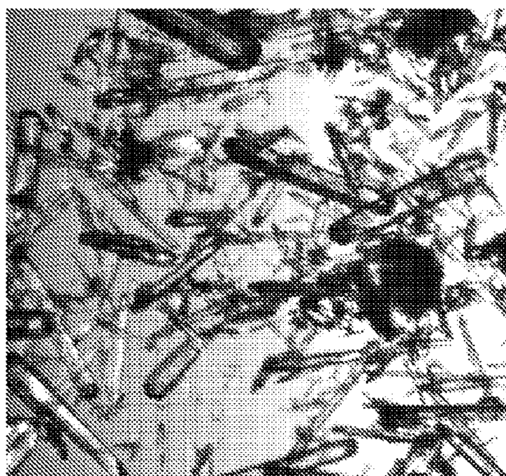
Crystal Form 3
