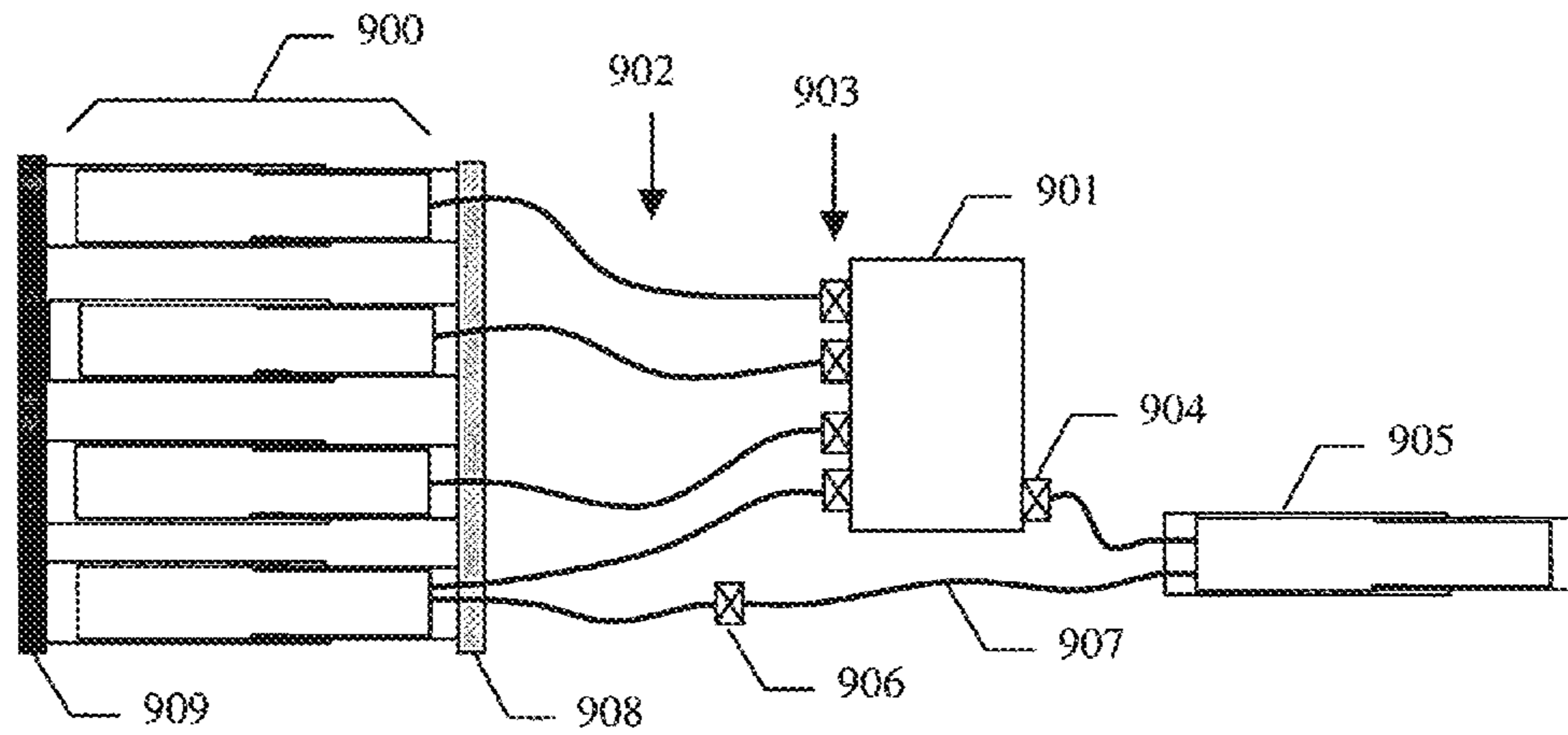
Variable-Spring-Rate Multiple-Pneumatic-Chamber and Energy Transfer System.
