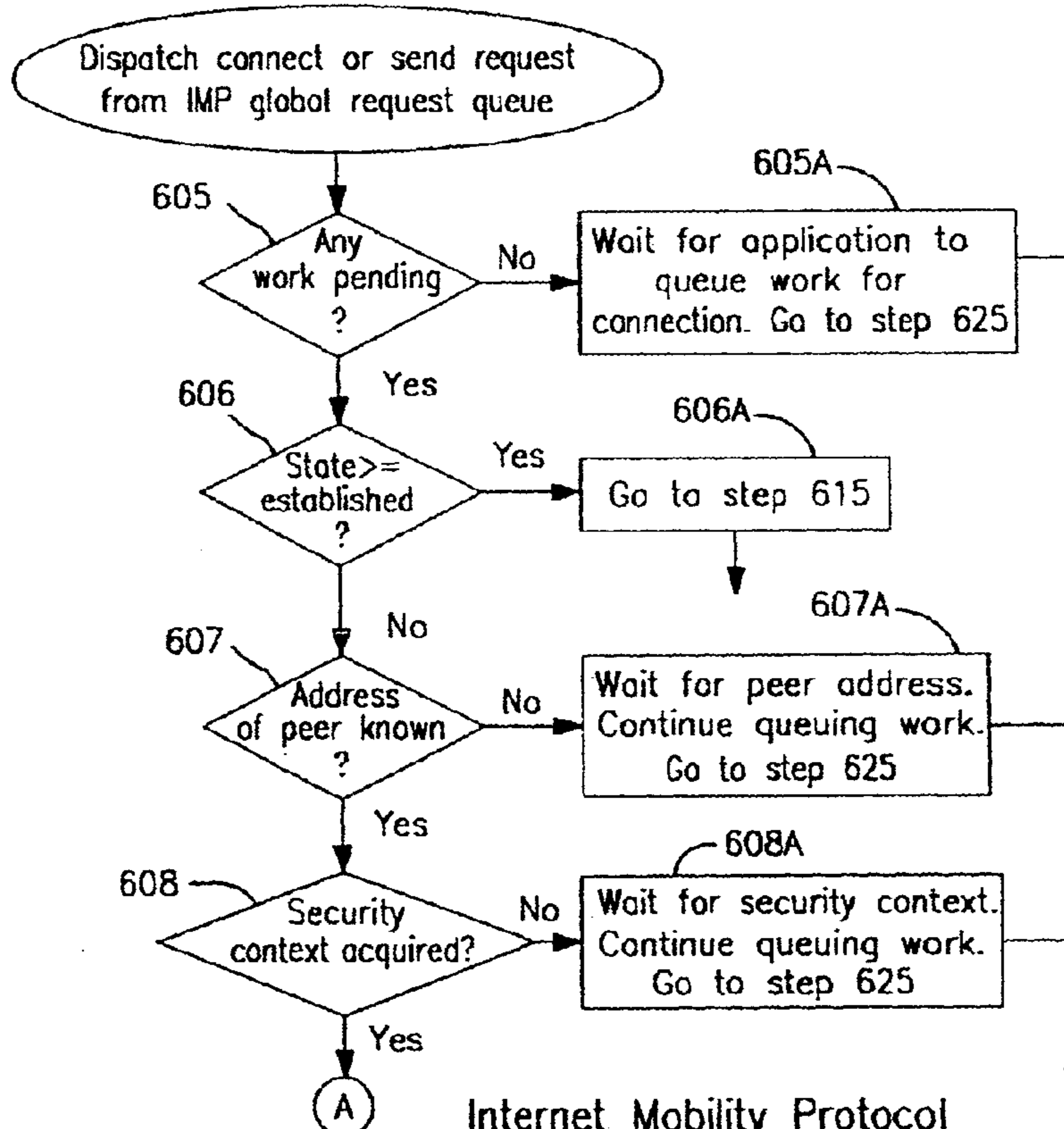
FIG. 10A Internet Mobility Protocol Connection Decision Tree. Connect and Send request logic
