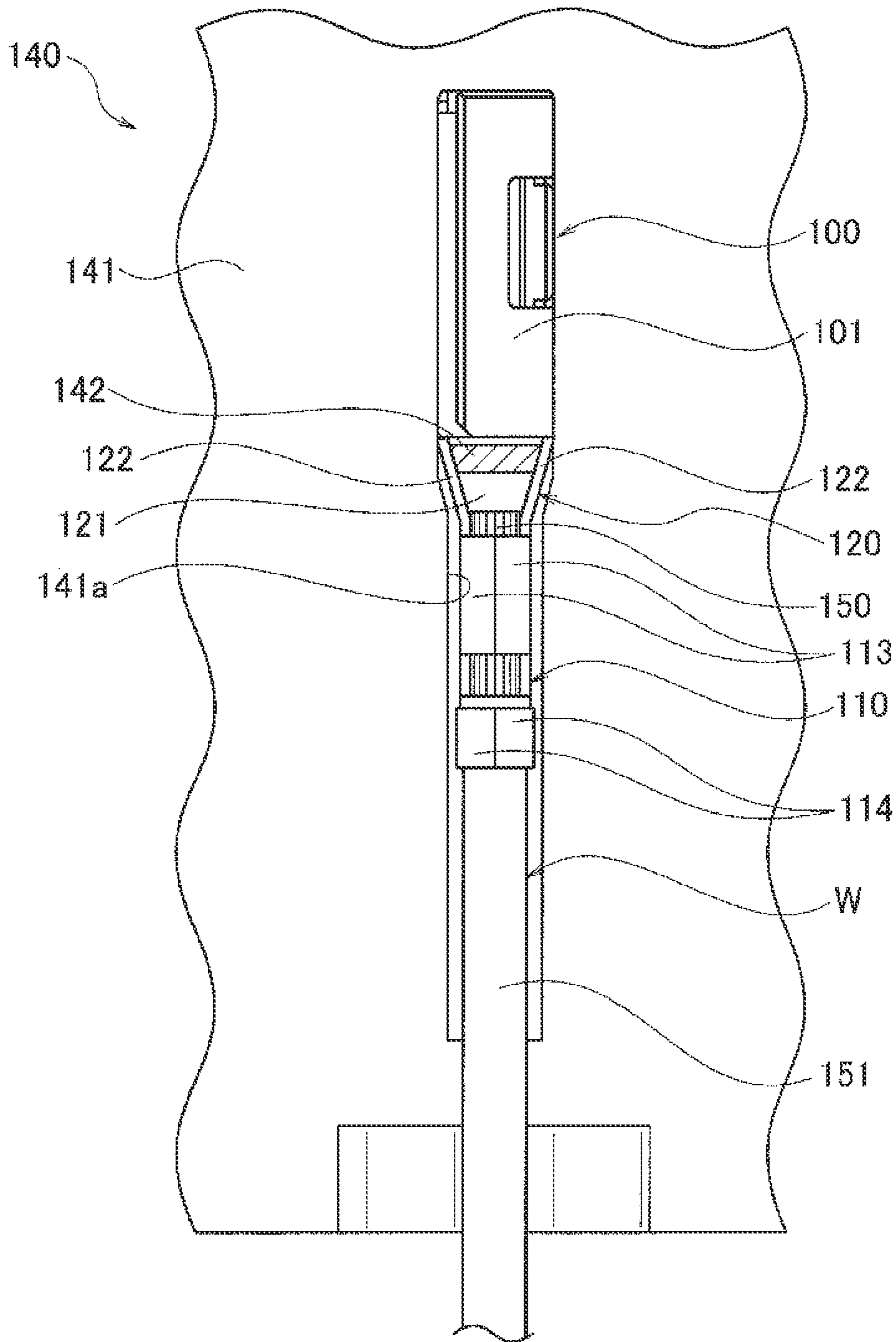
FIG. 3 RELATED ART
