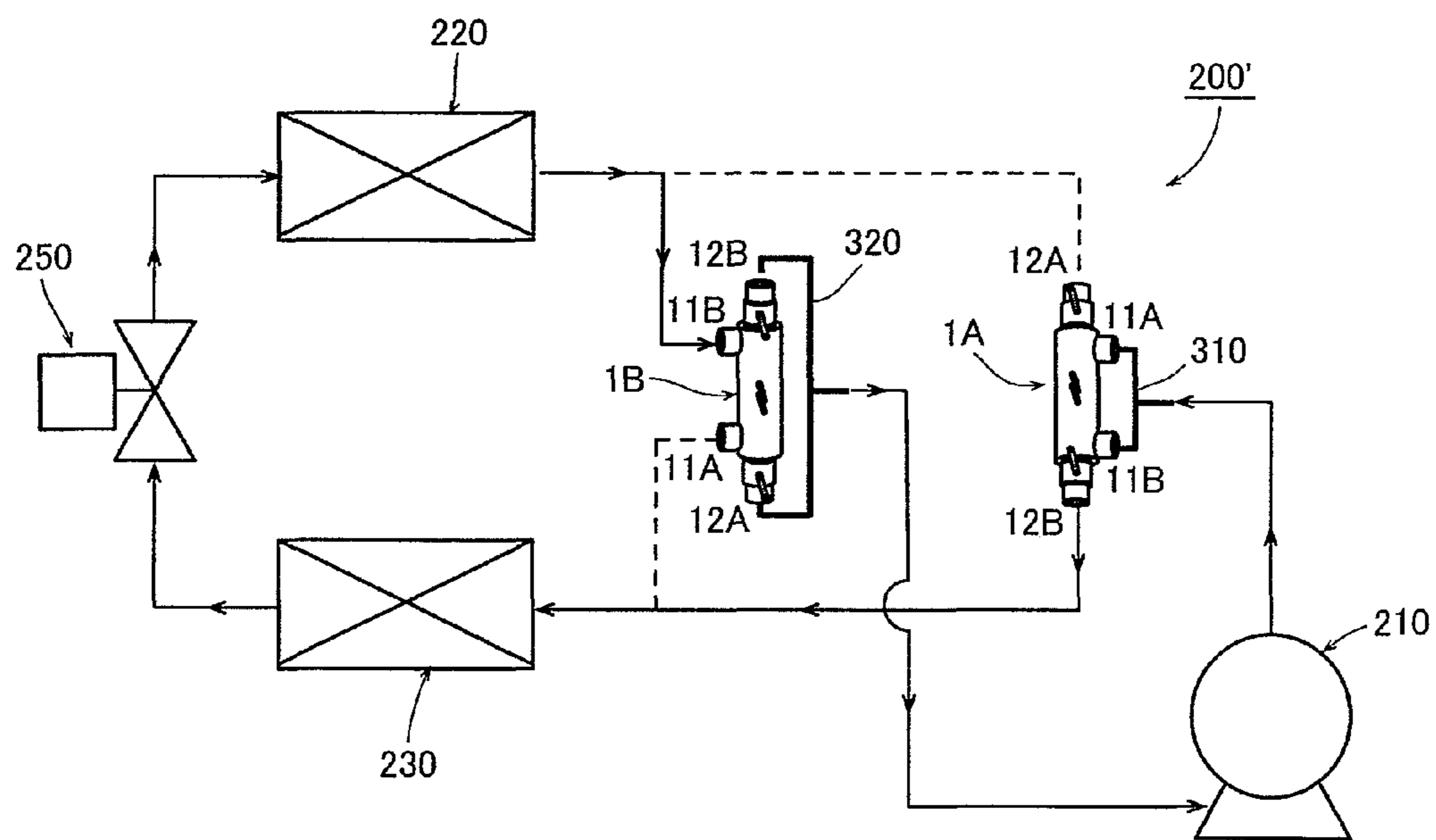
FIG. 4B < During heating operation >
