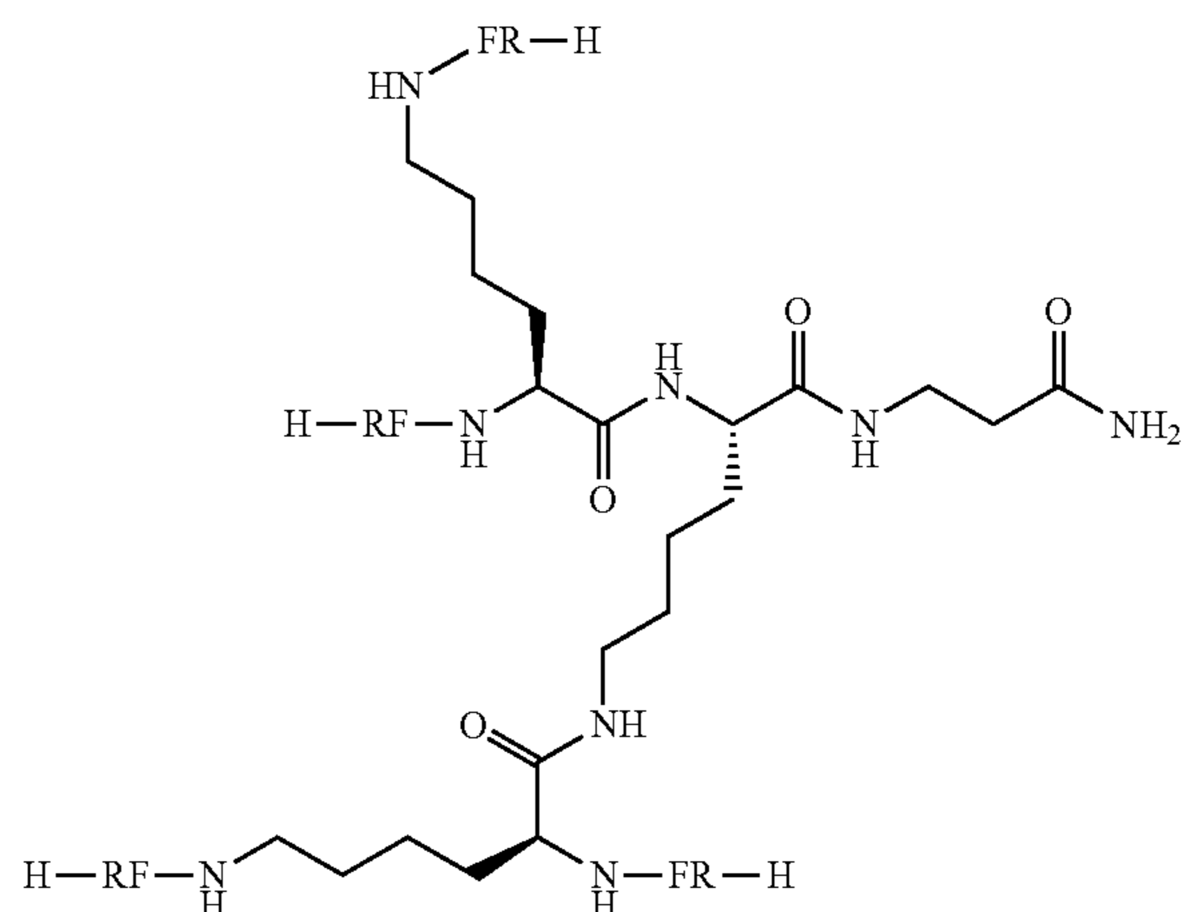
Compound 2 [Den(RF) 4D ]
