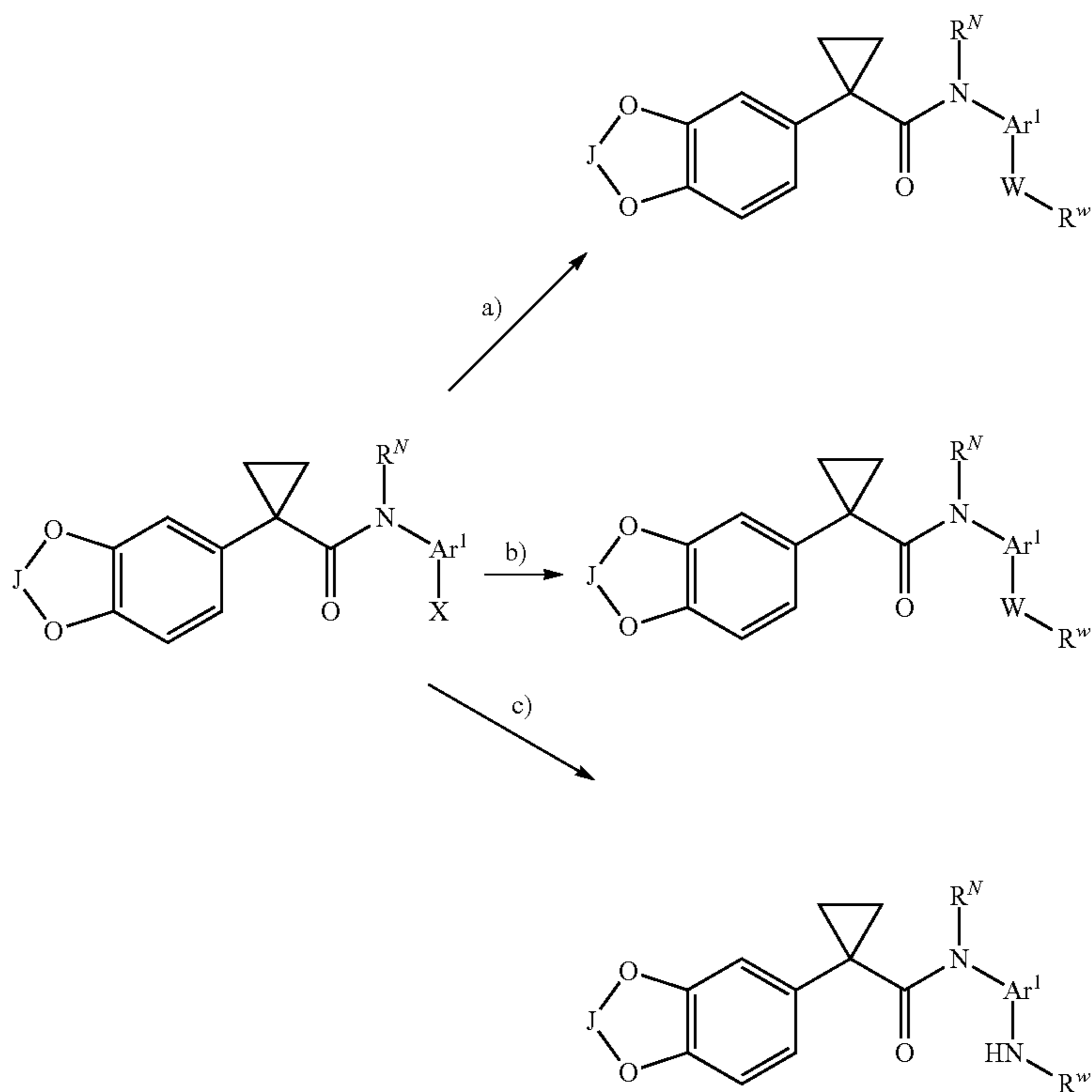
Scheme III-Derivatization of heteroarylhalides
