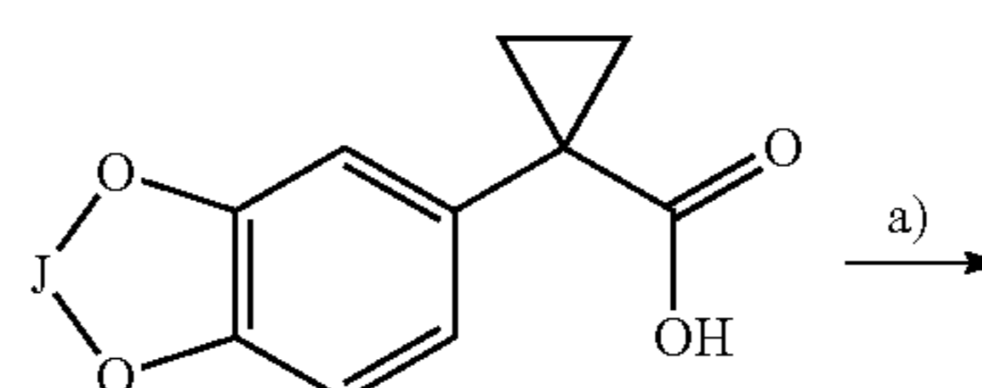
Scheme II-Amid coupling
