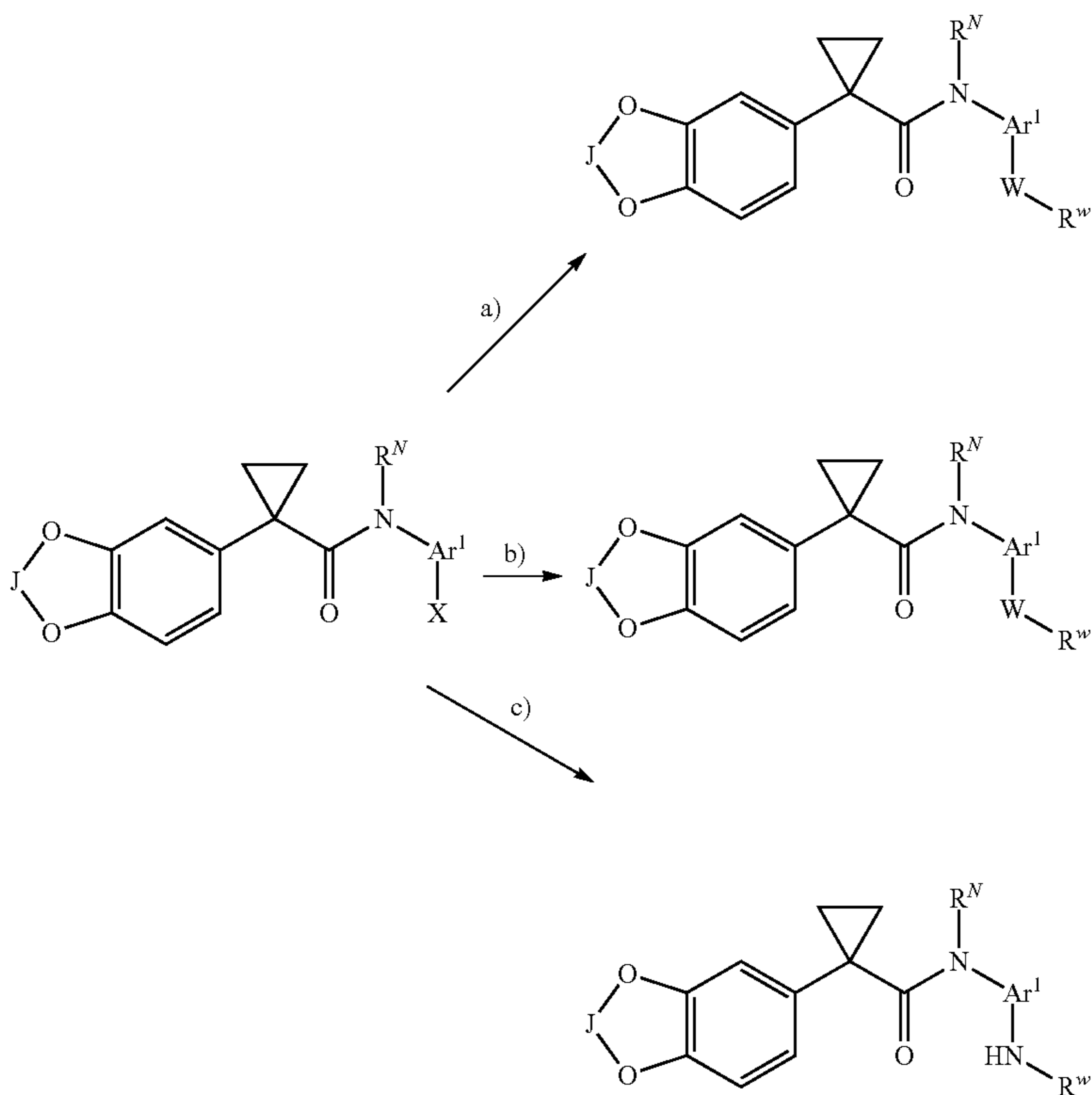
Scheme III-Derivatization of heteroarylhalides
