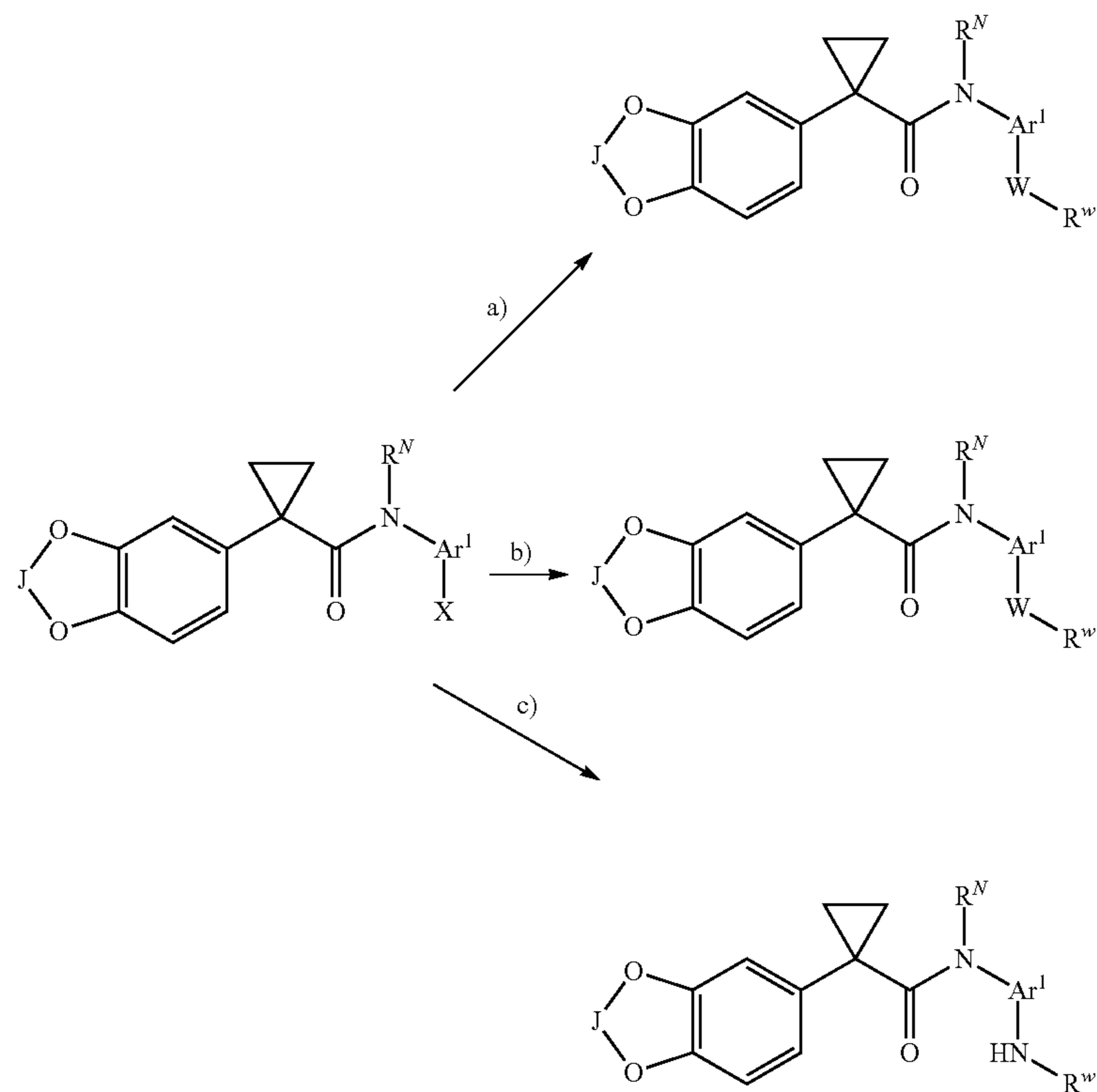
Scheme III-Derivatization of heteroarylhalides
