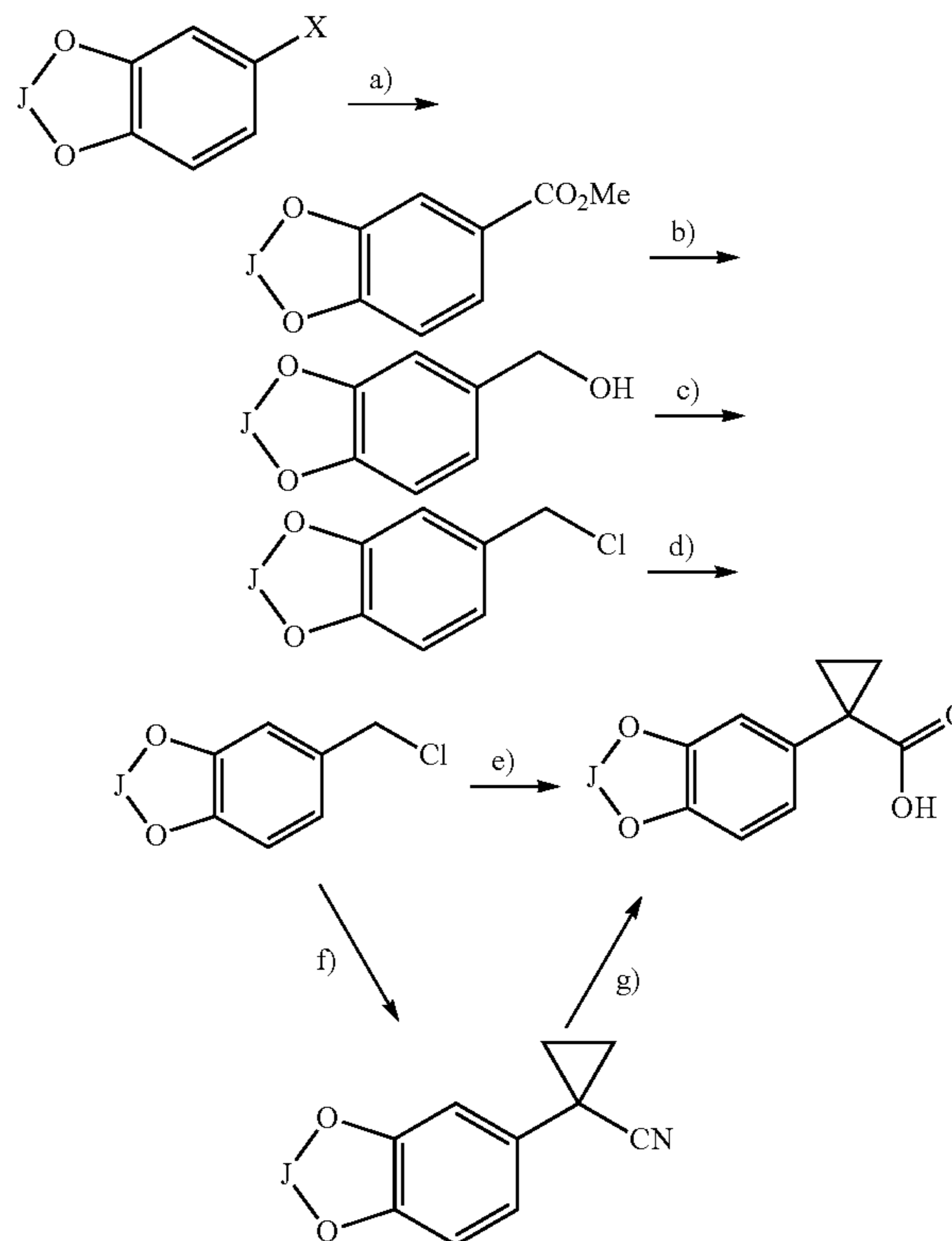
Scheme I-Preparation of cycloalkyl acids.
