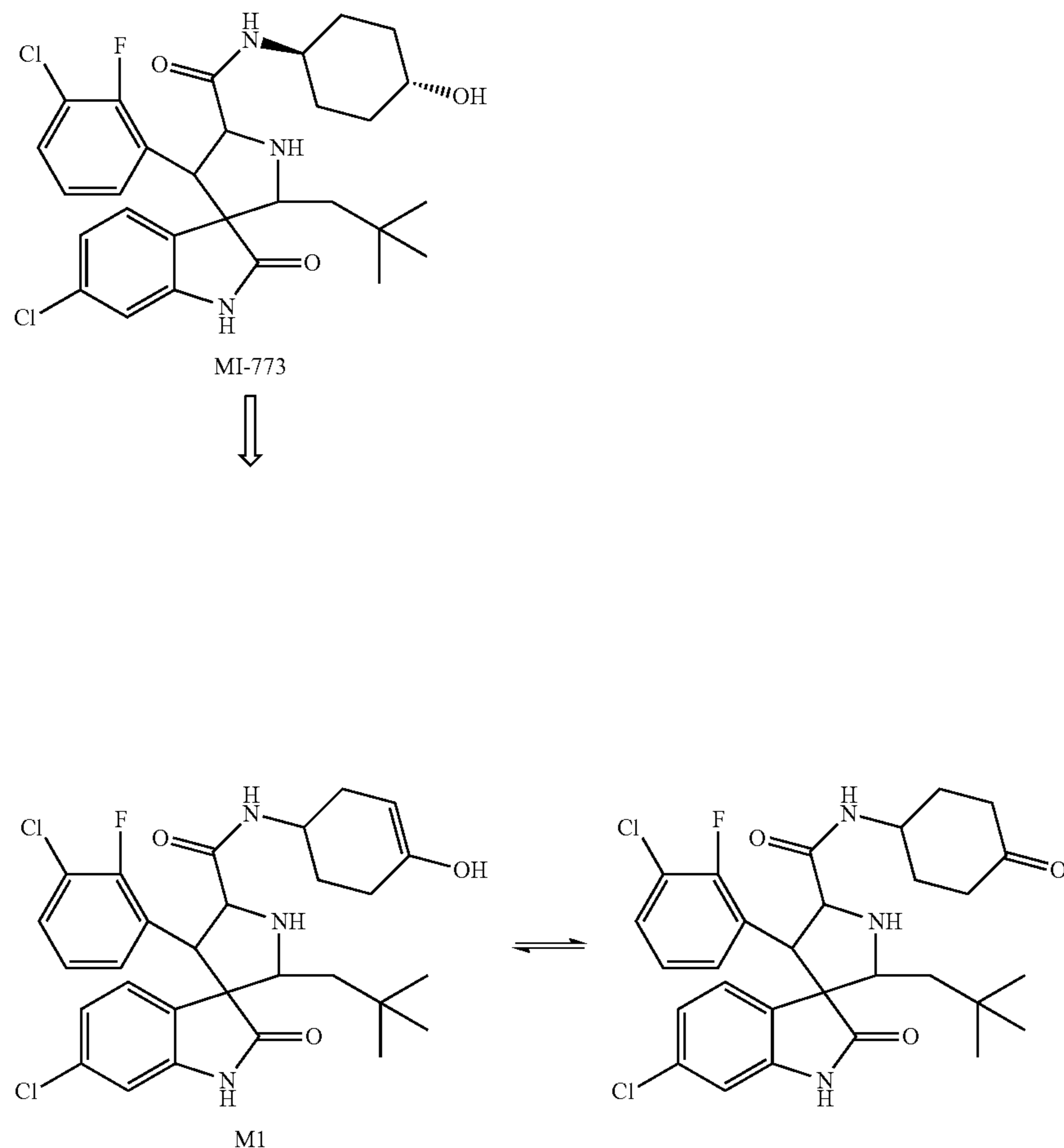
Chart 4. Proposed chemical structure of M1.
