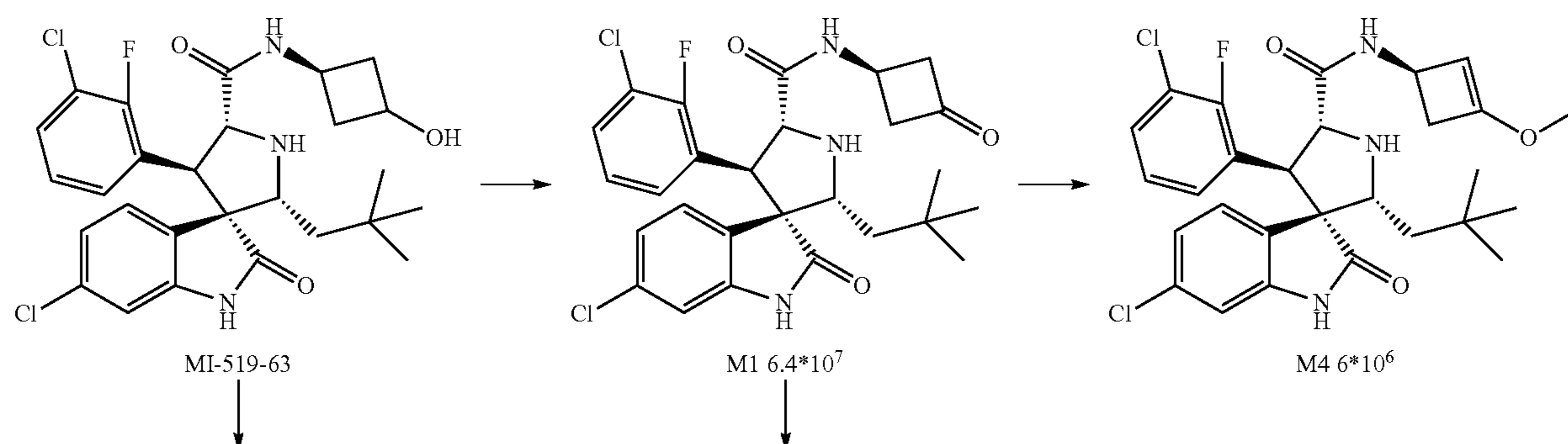
Chart 5. Biotransformation pathways of MI-519-63 in human liver microsomes incubation.
