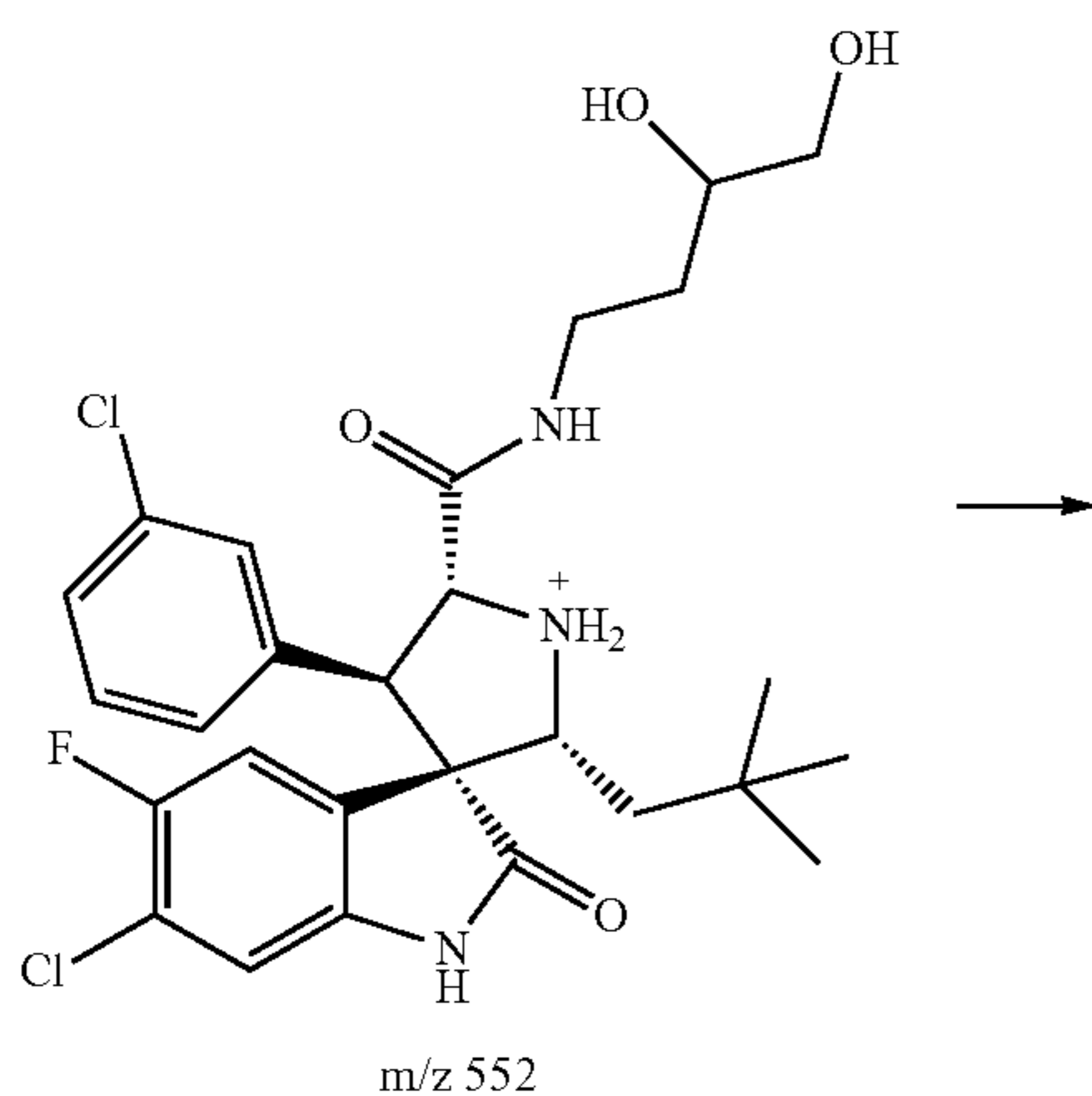
Scheme 5. Proposed fragmentation pathways of protonated MI-219.
