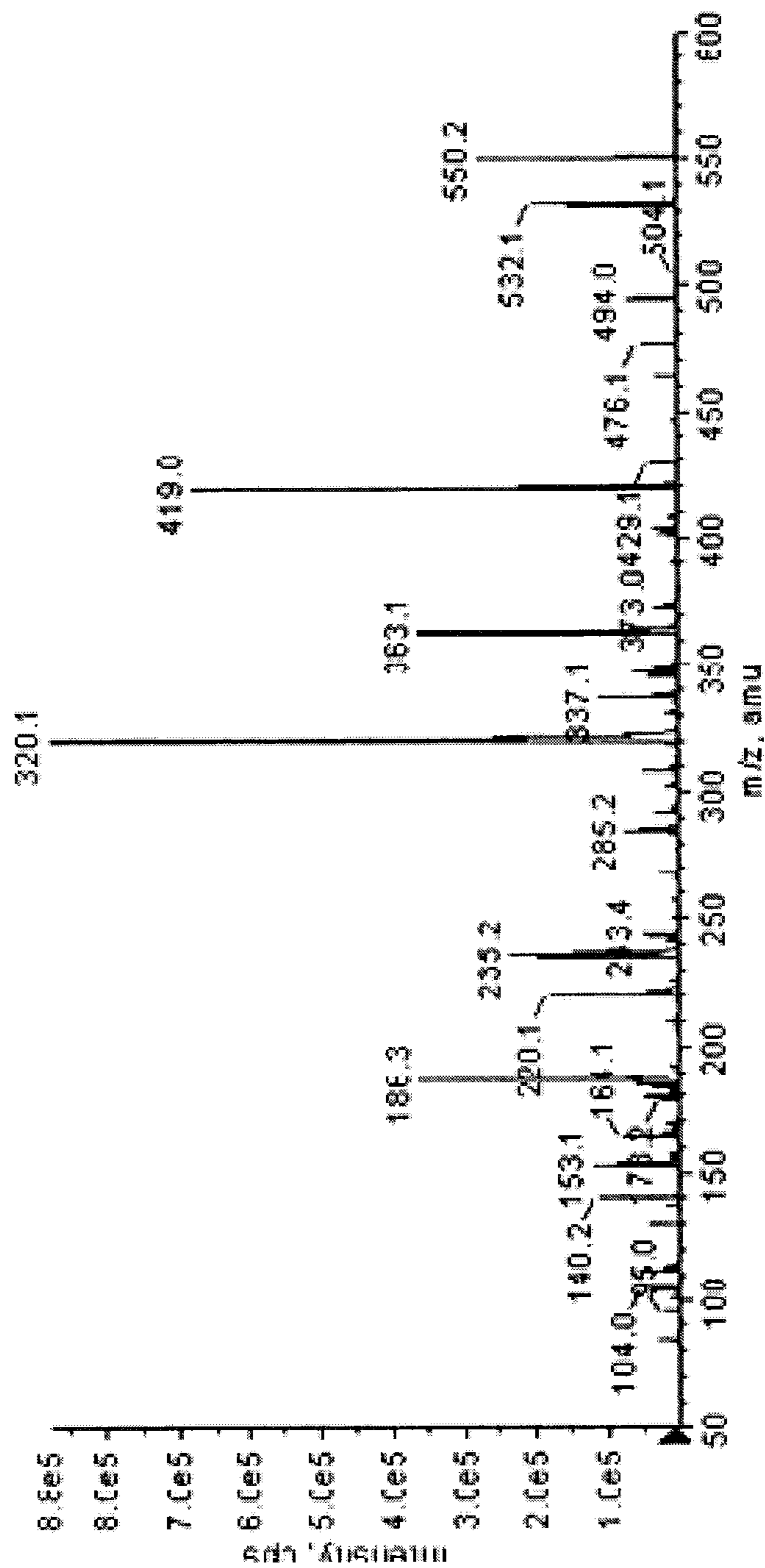
MS/MS spectrum of synthesized M1
