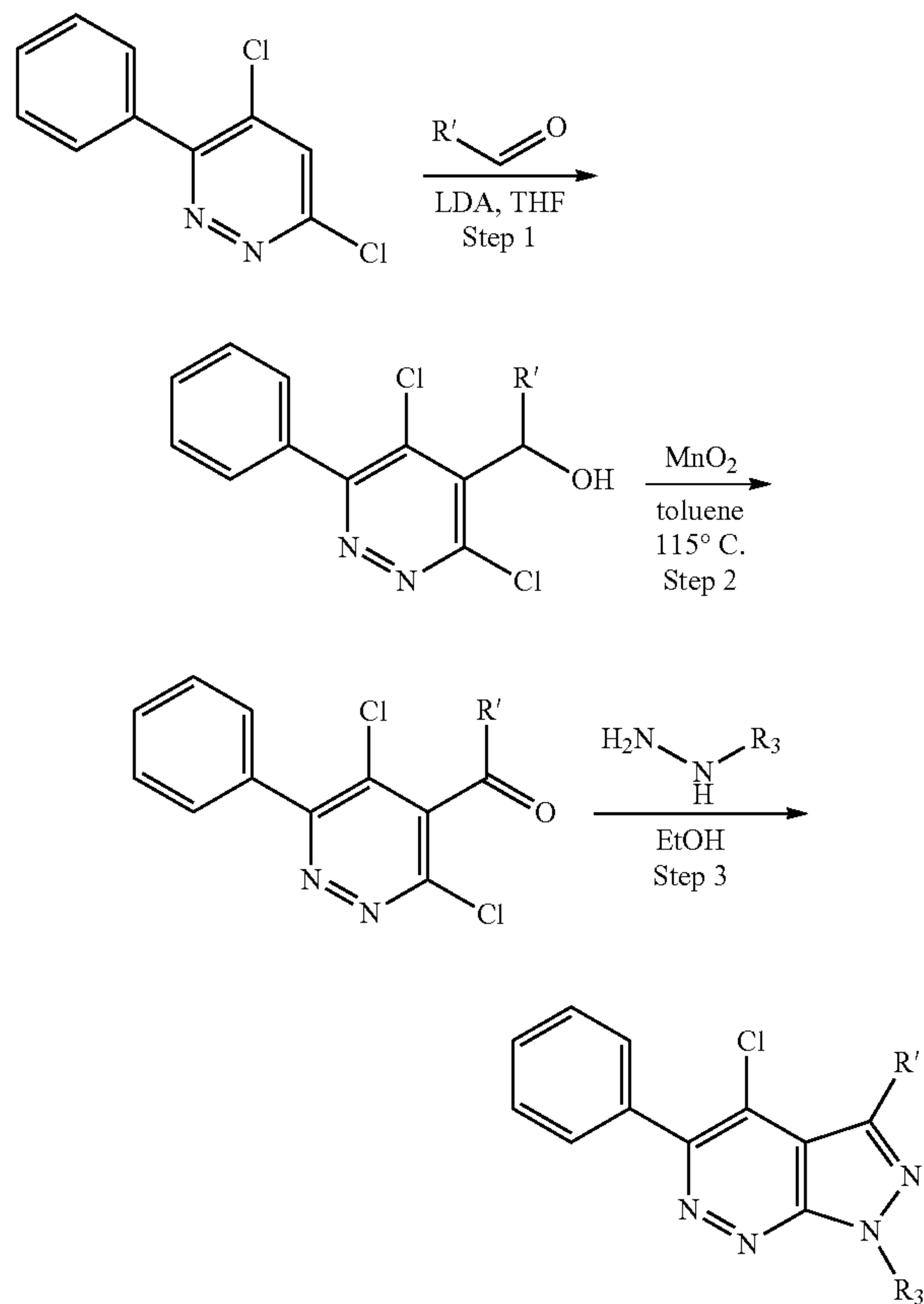
Scheme 2
