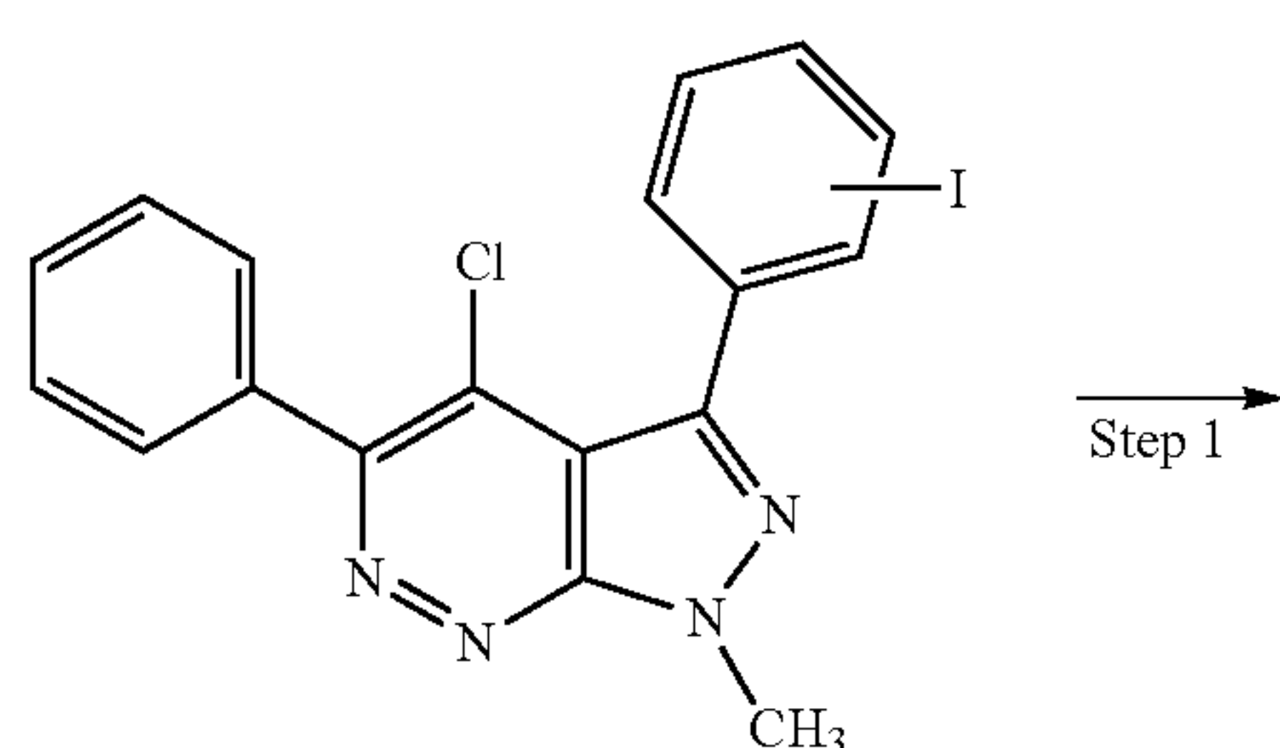
Scheme 3
