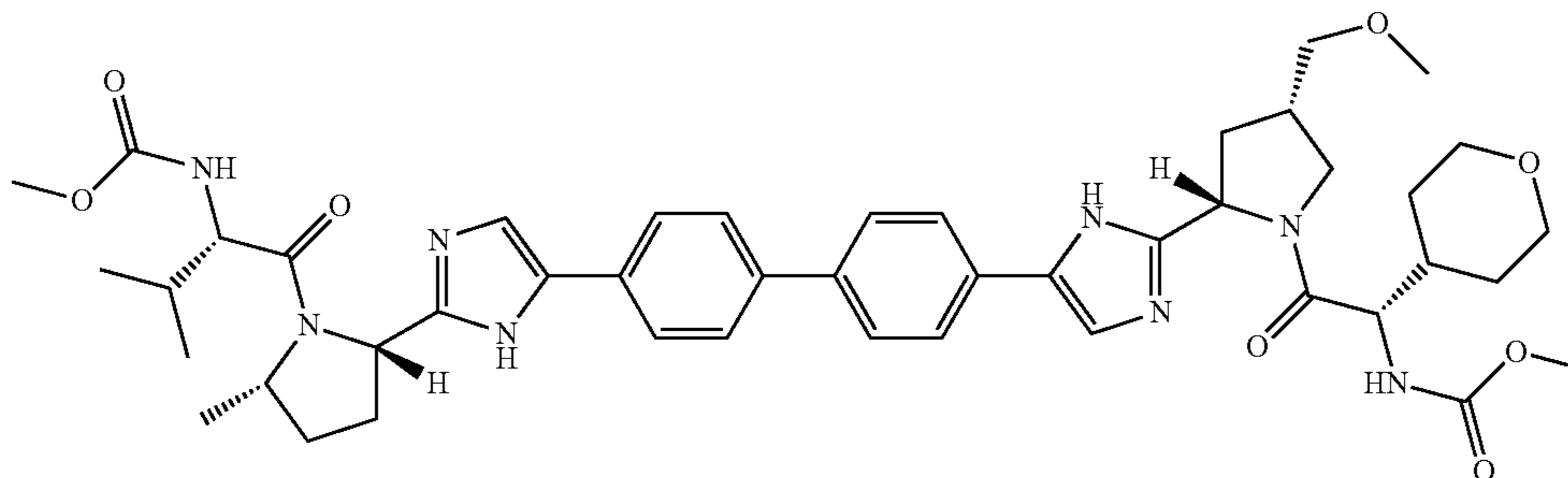
methyl [(1S)-2-[(2S,4S)-2-[5-(4'-{2-[(2S,5S)-1-[(2S)-2-[(methoxycarbonyl)amino]-3-methylbutanoyl]-5-methylpyrrolidin-2-yl]-1H-imidazol-5-yl}biphenyl-4-yl)-1H-imidazol-2-yl]-4-(methoxymethyl)pyrrolidin-1-yl]-2-oxo-1-(tetrahydro-2H-pyran-4-yl)ethyl]carbamate
