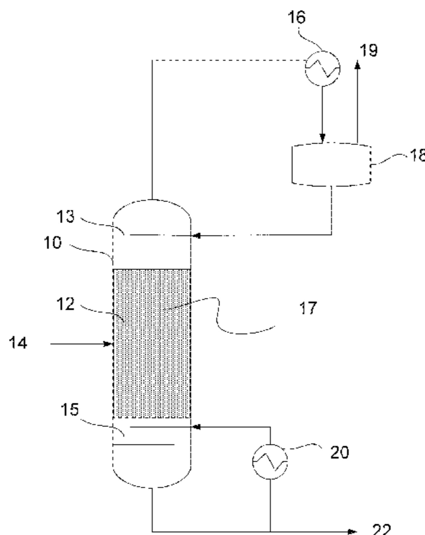
Single feed reactive distillation column schematic.
