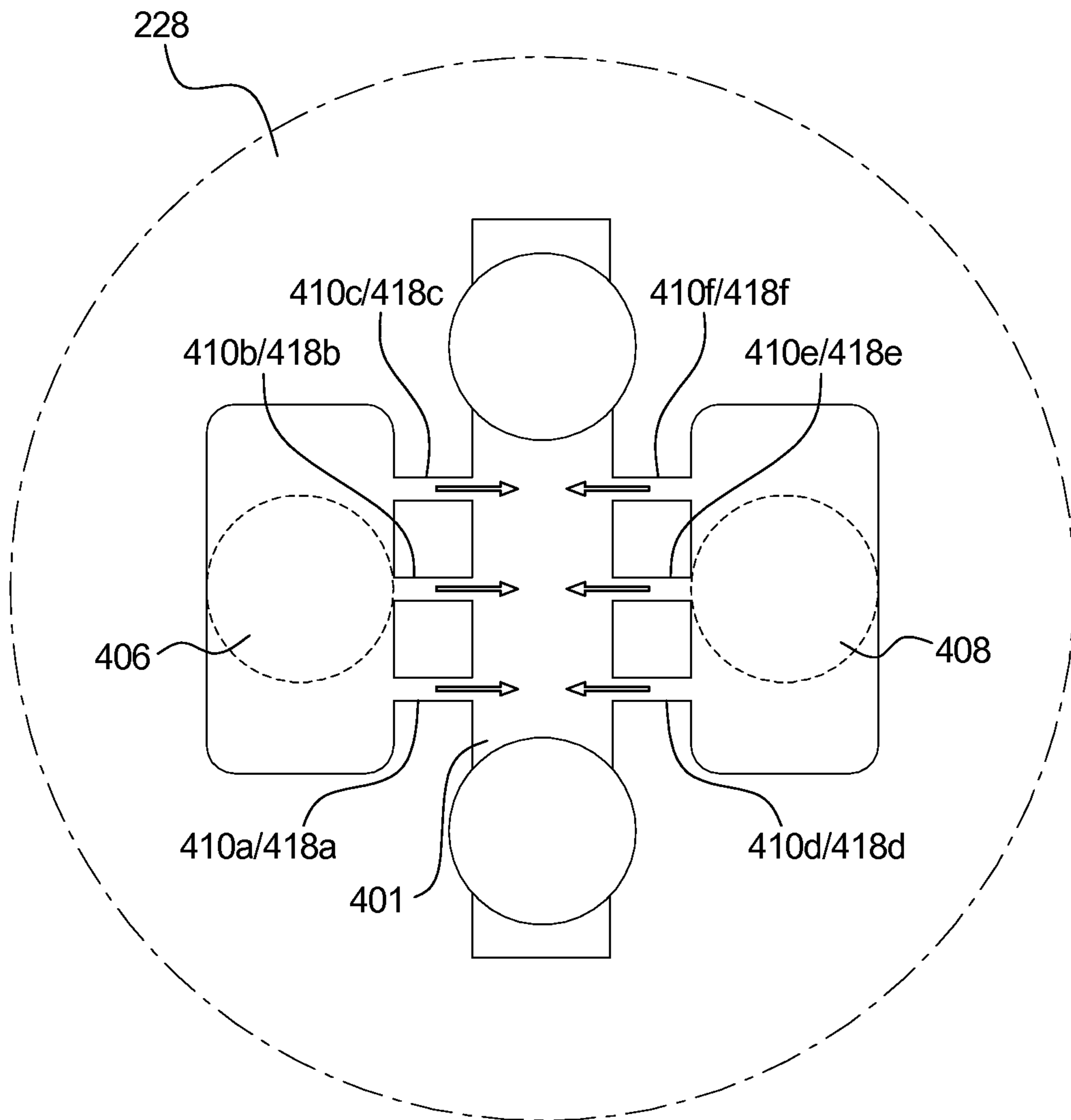
FIG. 9 (PRIOR ART)
