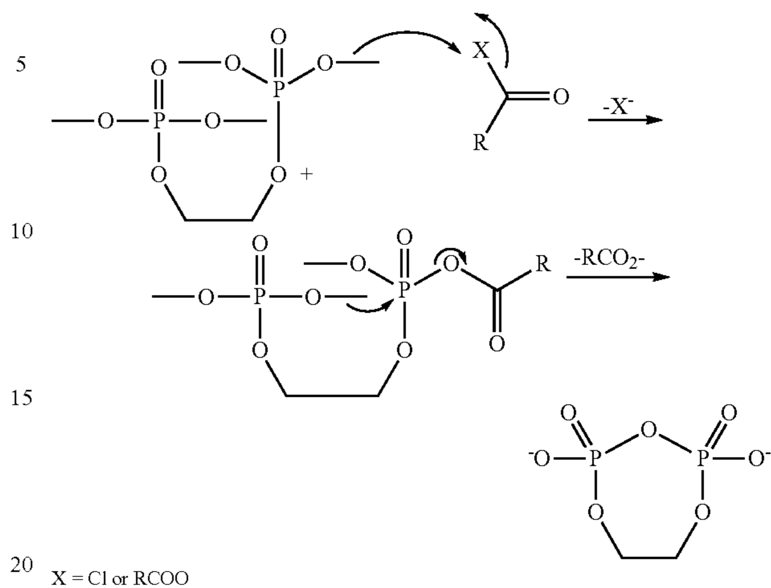
Scheme 2. Mechanism of internal pyrophosphate formation.
