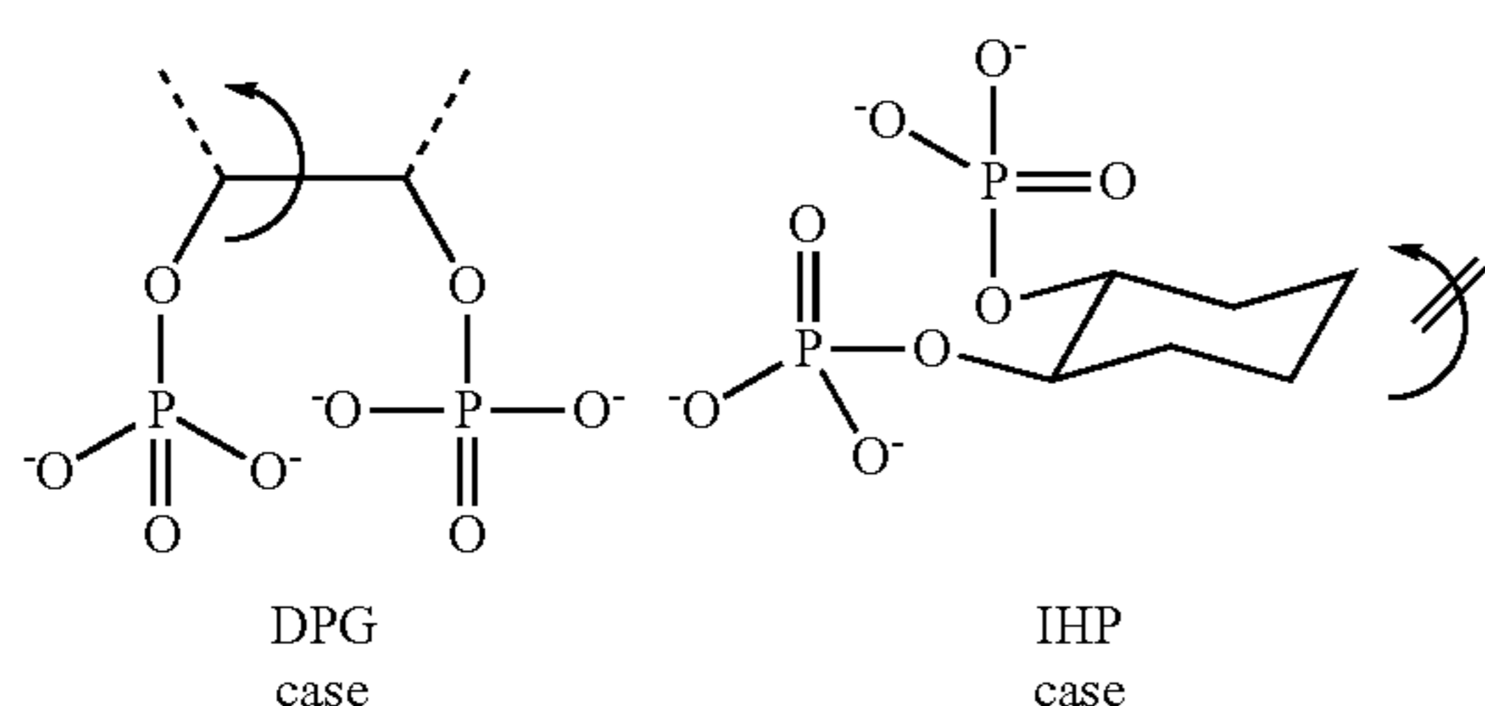
Scheme 5. Explanation of the behaviour of DPG and IHP toward acyl anhydrides.
