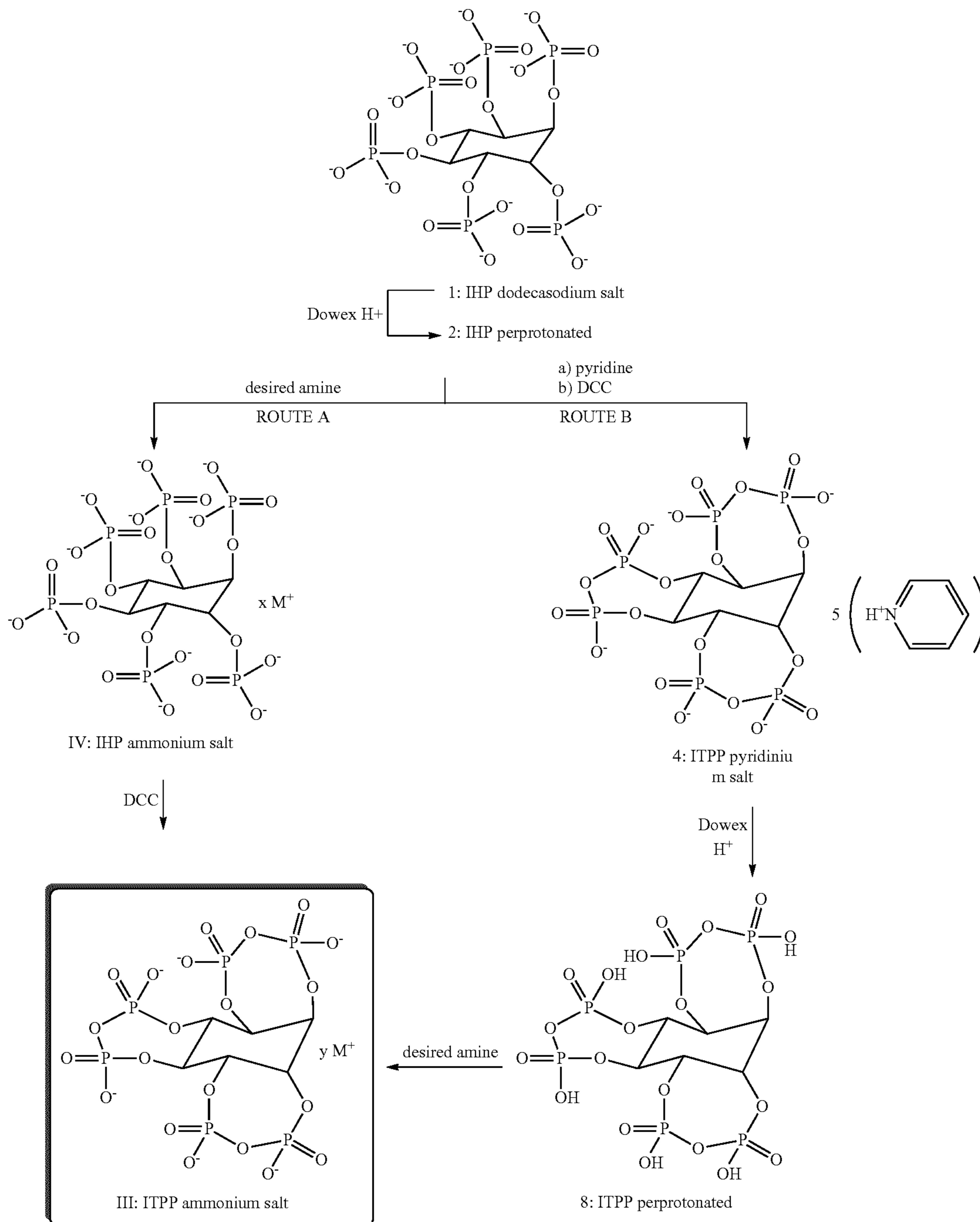
Scheme 6. General routes for the synthesis of ITPP ammonium salts.
