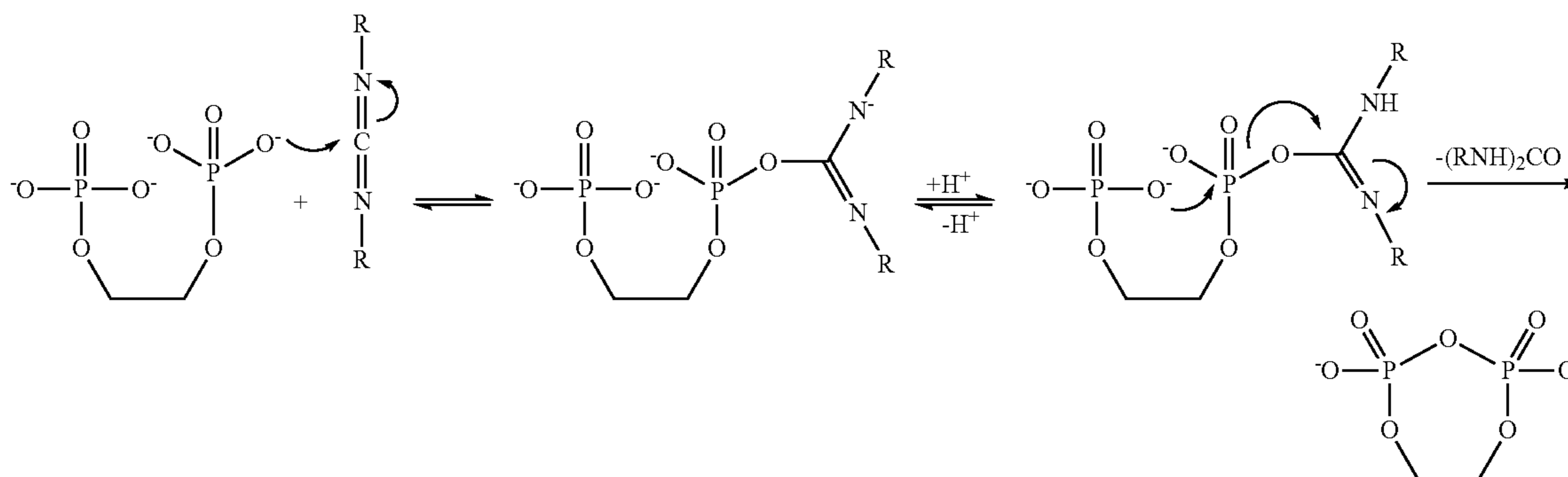
Scheme 4. Mechanistic pathways of the formation of pyrophosphates through a reaction with DCC.
