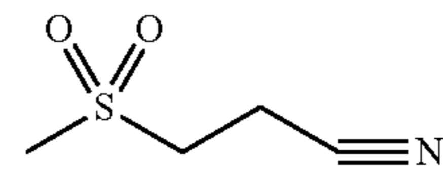
3-methanesulfonylpropionitrile
