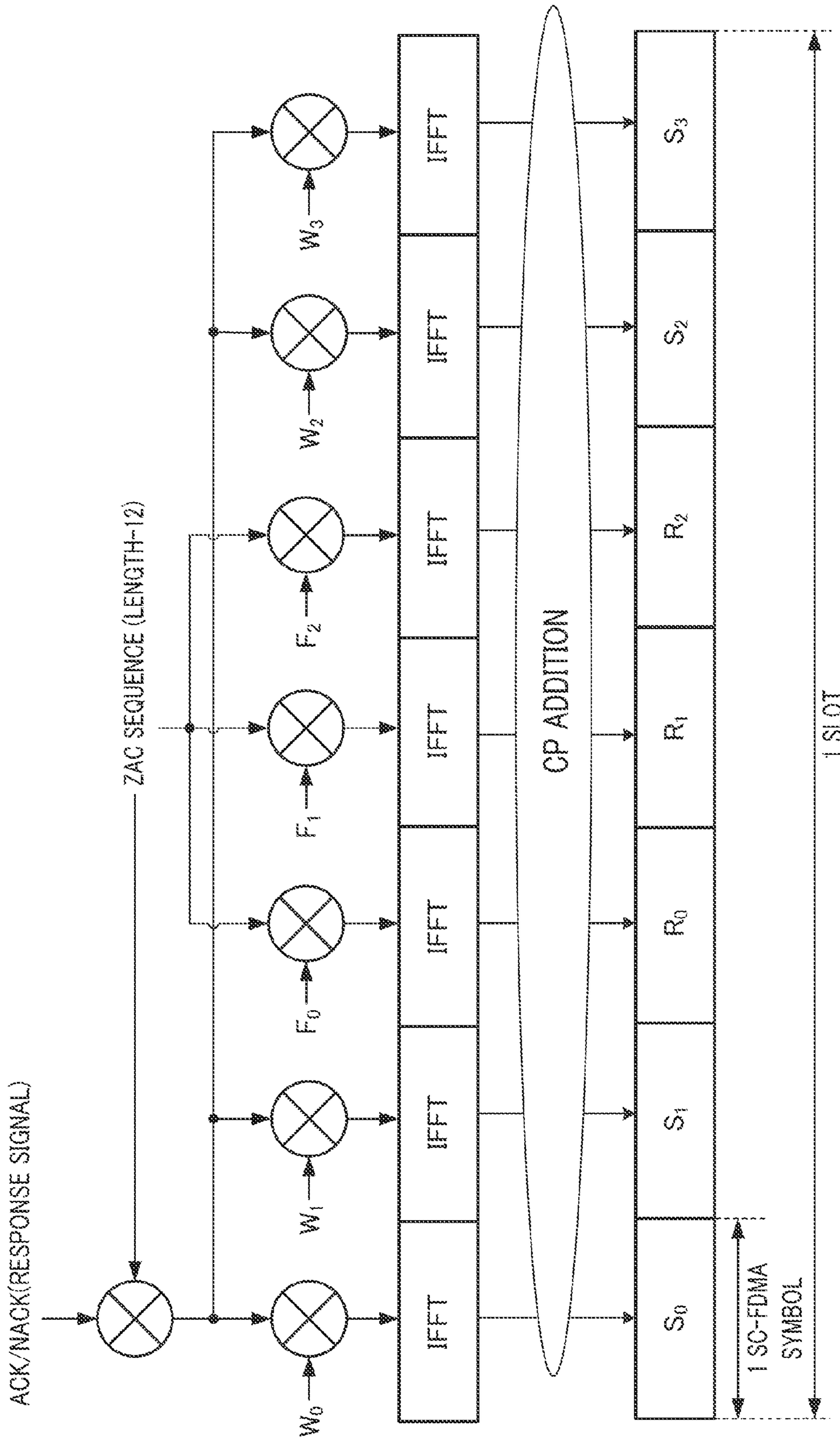
FIG. 1 PRIOR ART
