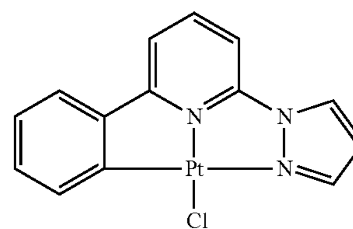
Ph-Py-Pz-PtCl
