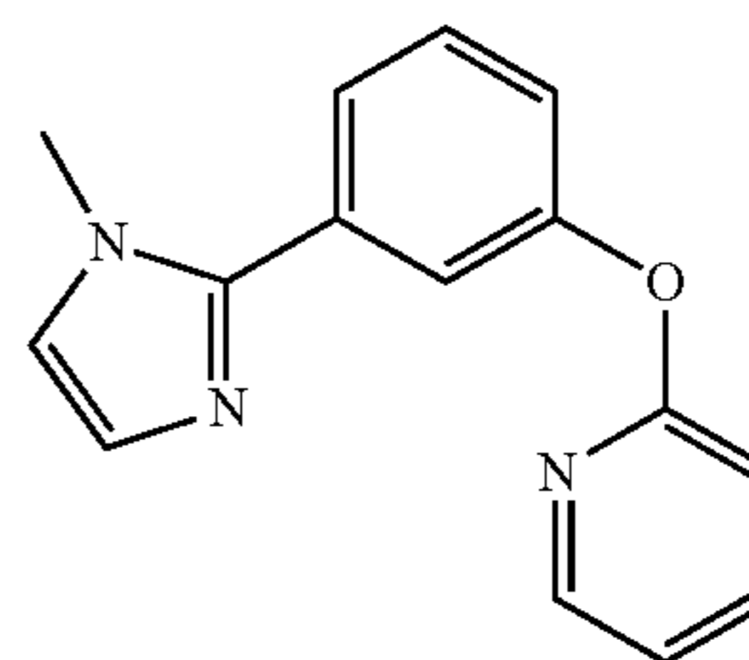
MIz-Ph-O-Py
