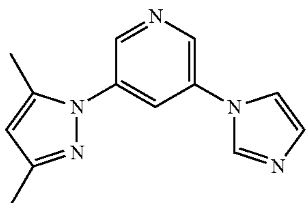
DMPz-Py-Iz
