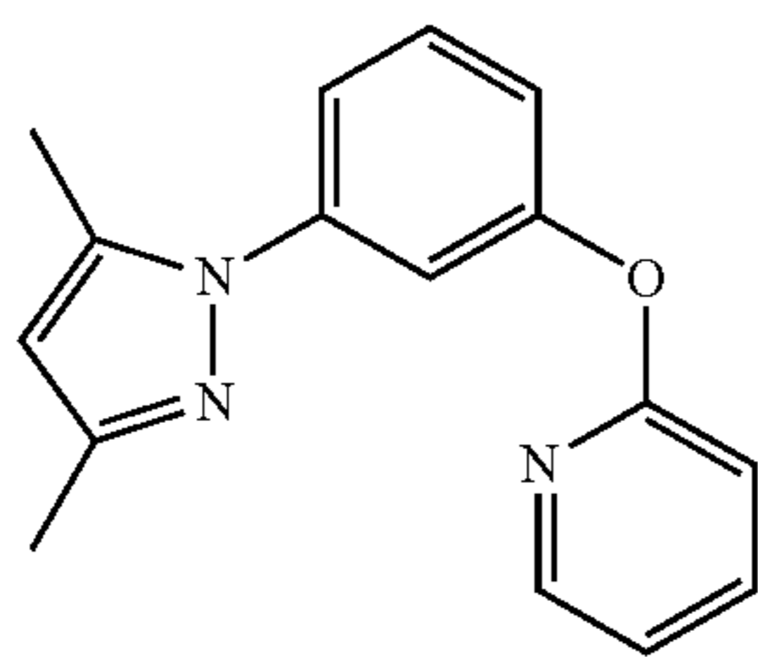
DMPz-Ph-O-Py
