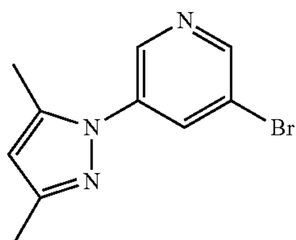
DMPz-Py-Br
