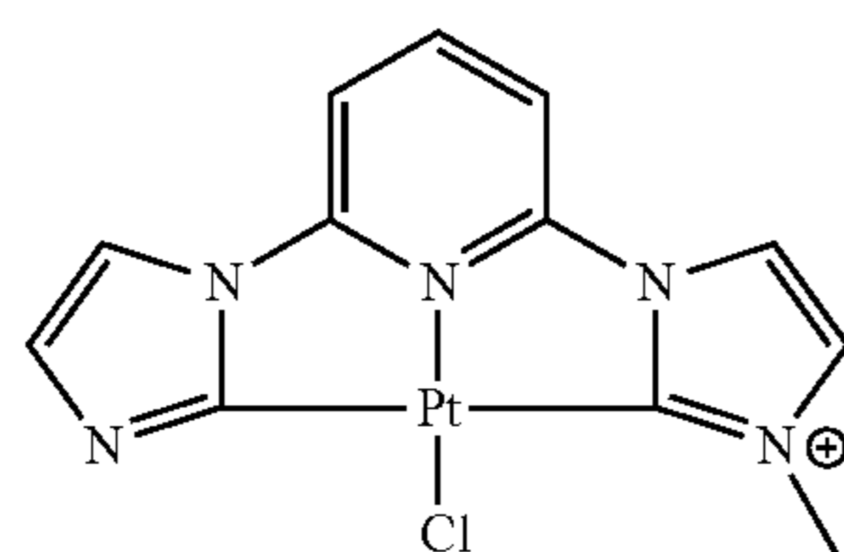
Iz-Py-MIzCb-PtCl
