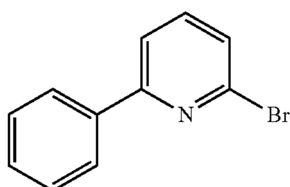
Ph-Py-Br
