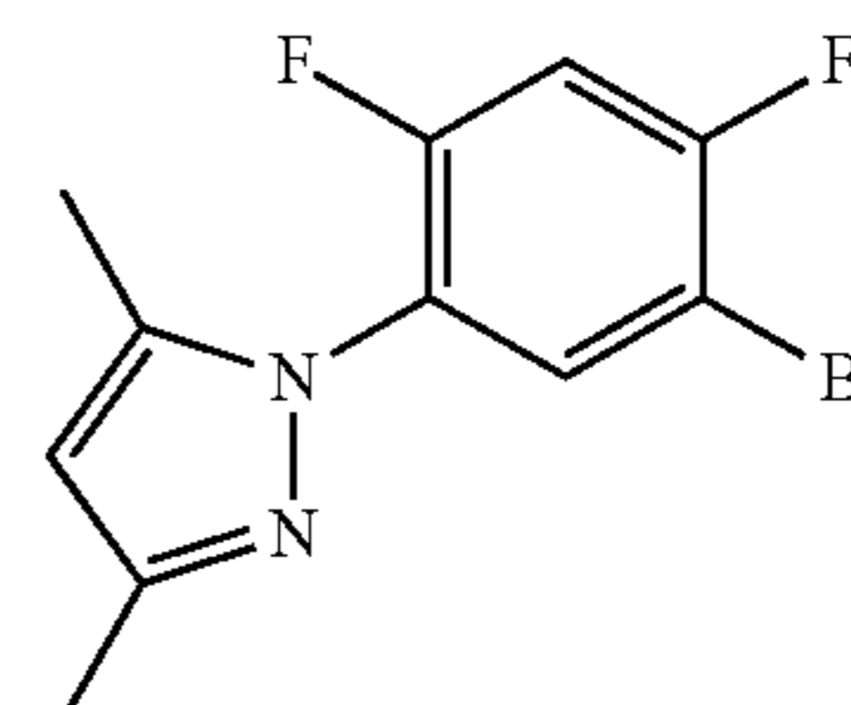
DMPz-DFPh-Br
