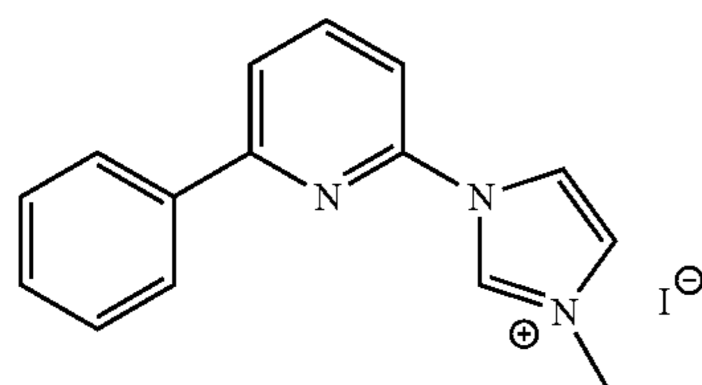
Ph-Py-IMIz
