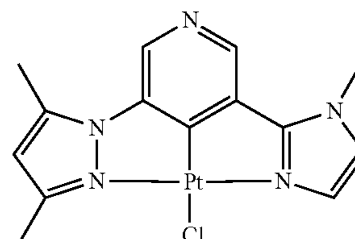
DMPz-Py-MIz-PtCl
