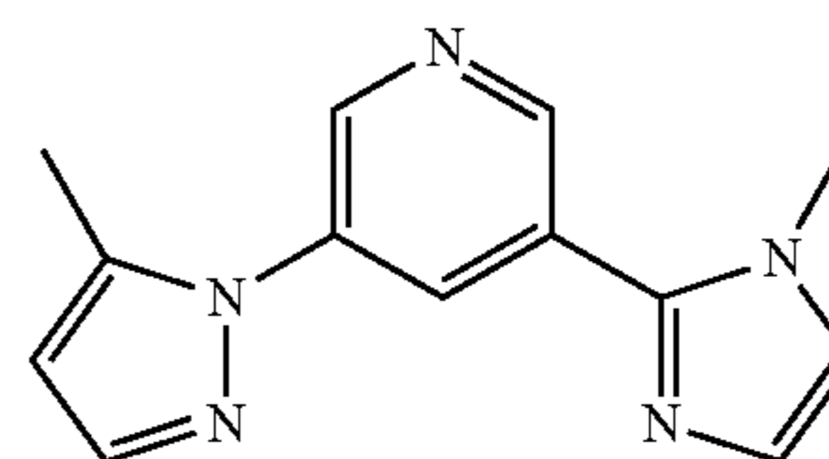
DMPz-Py-IMz
