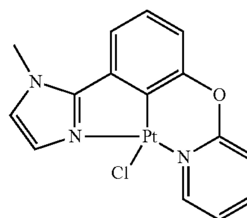
MIz-Ph-O-Py-PtCl
