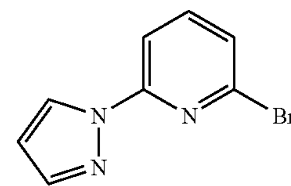
Pz-Py-Br
