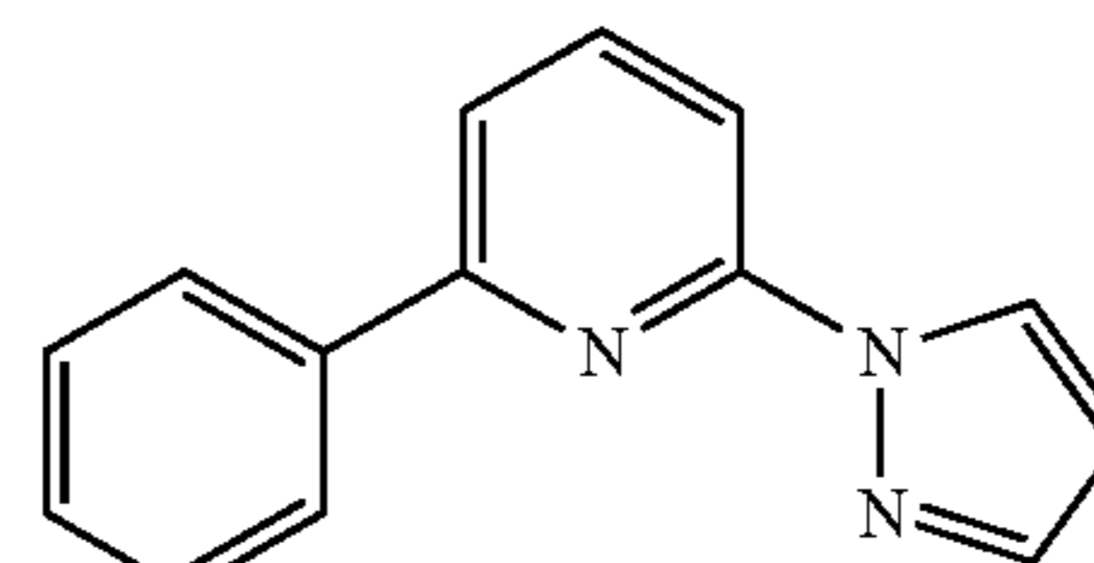
Ph-Py-Pz
