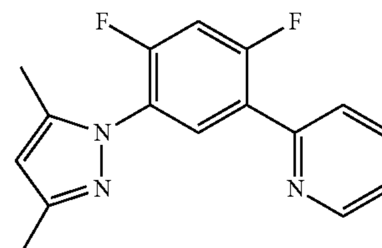
DMPz-DFPh-Py
