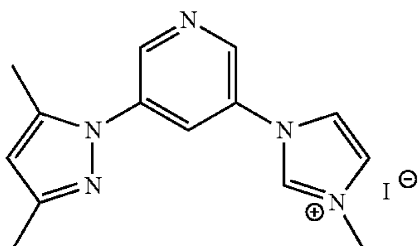
DMPz-Py-IMiz
