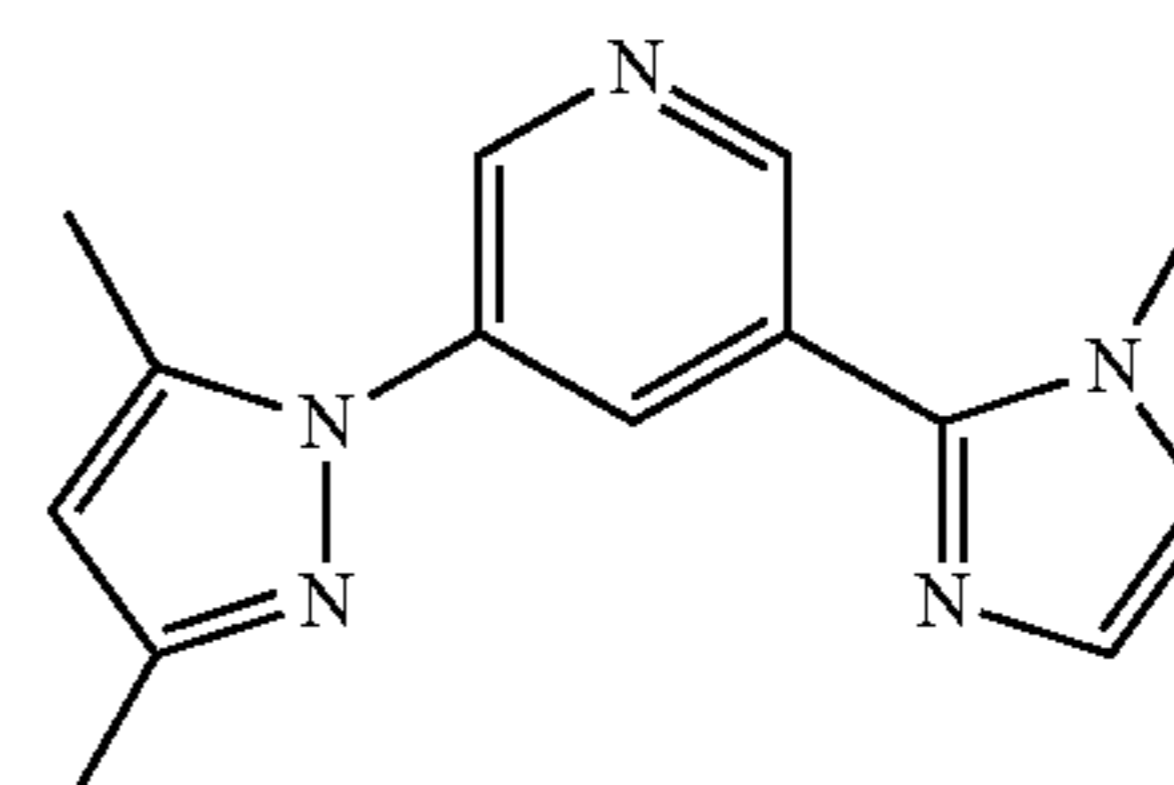
DMPz-Py-IMz
