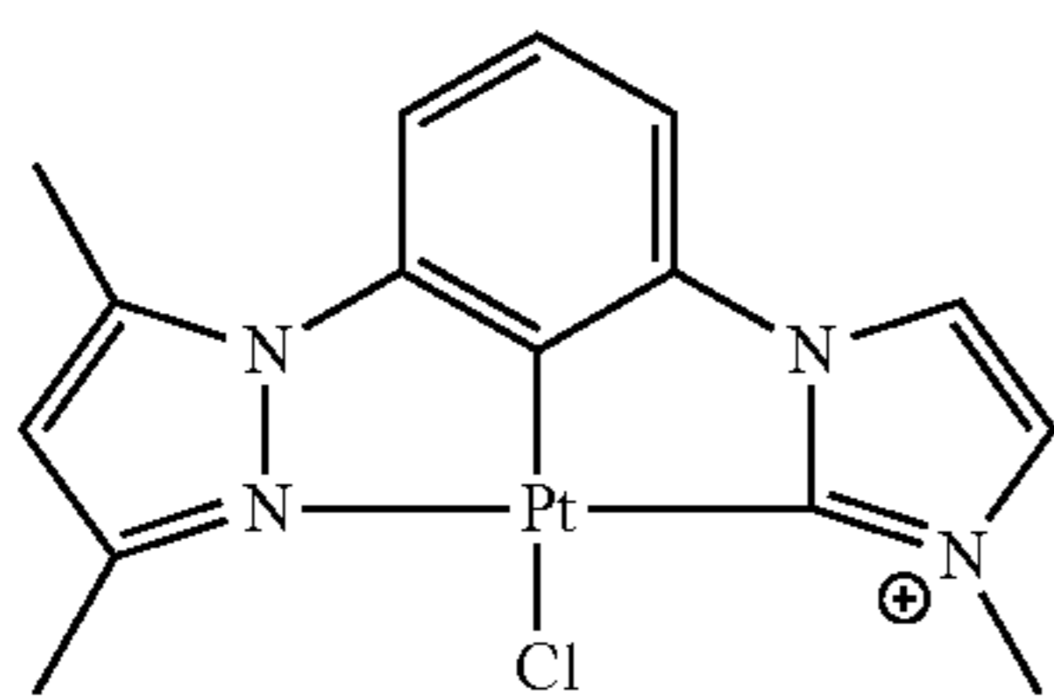
DMPz-Ph-MIzCb-PtCl
