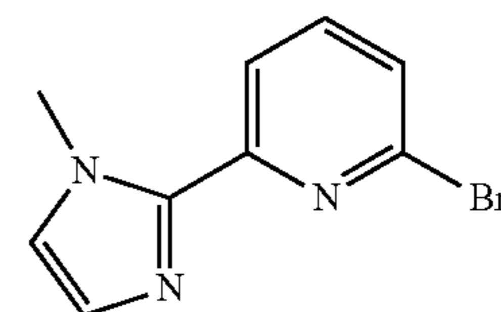
MIz-Py-Br
