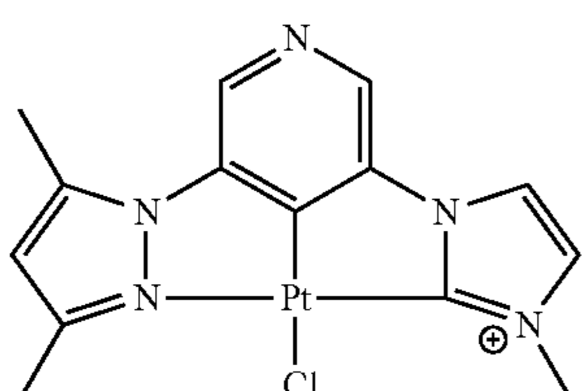
DMPz-Py-IMizCb-PtCl
