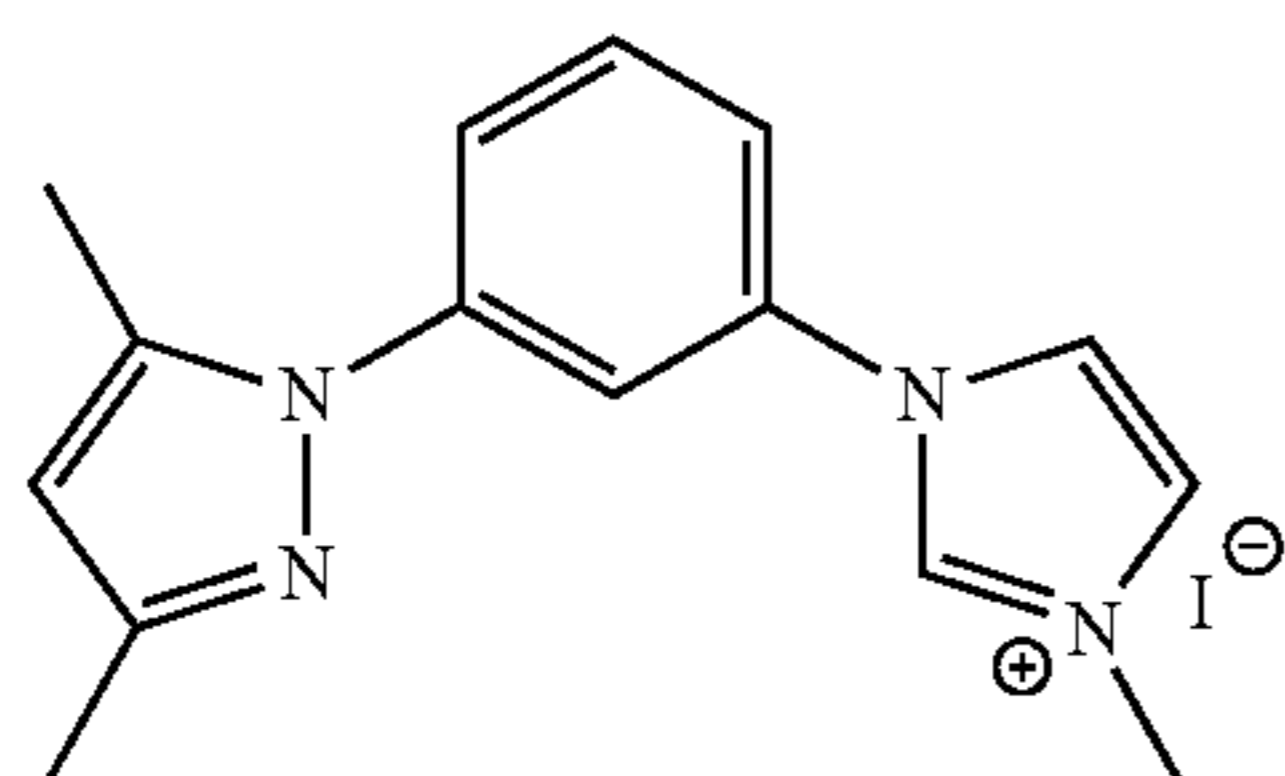
DMPz-Ph-IMiz
