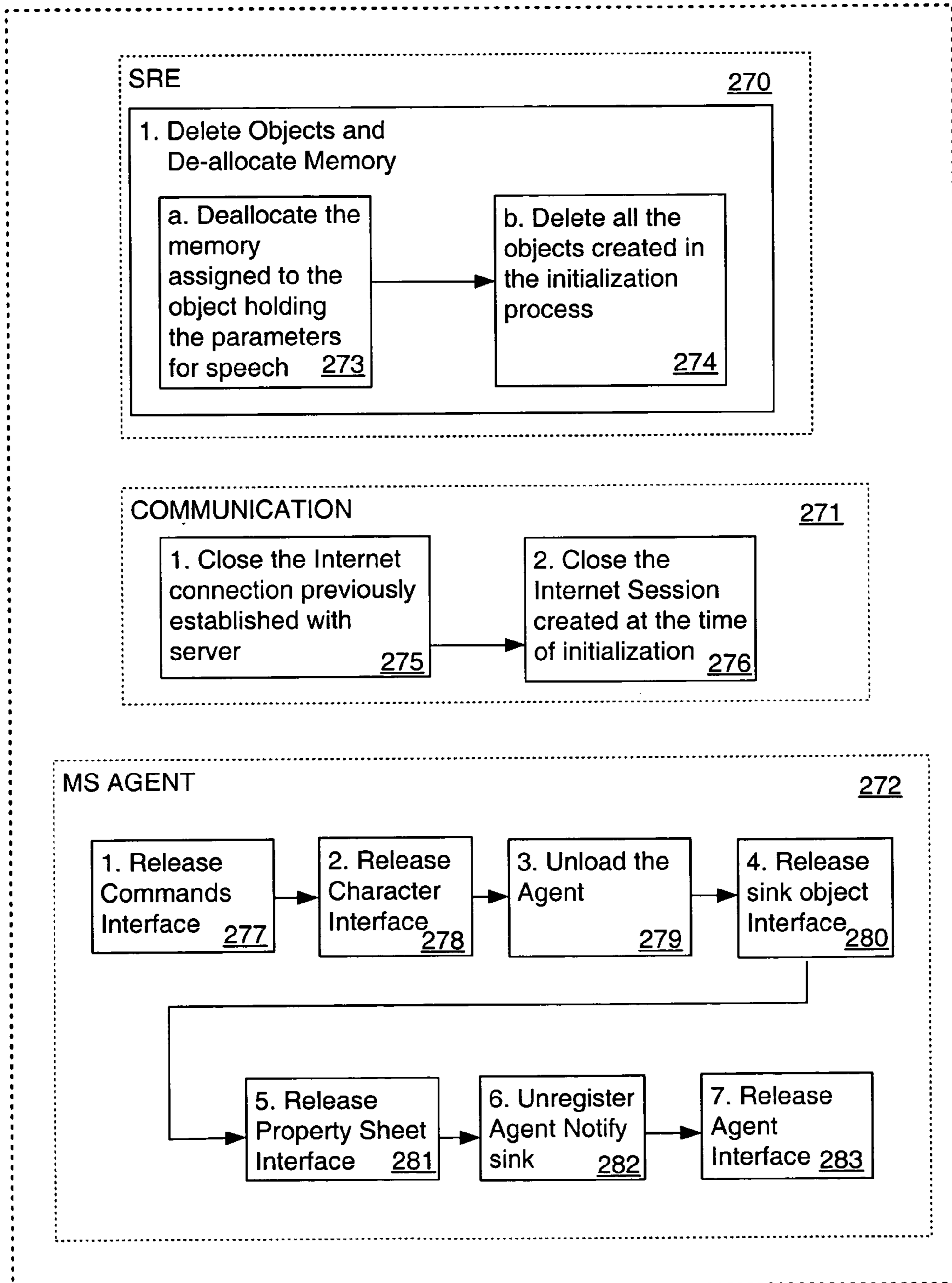
Fig. 4 Client-side Un-Initialization
