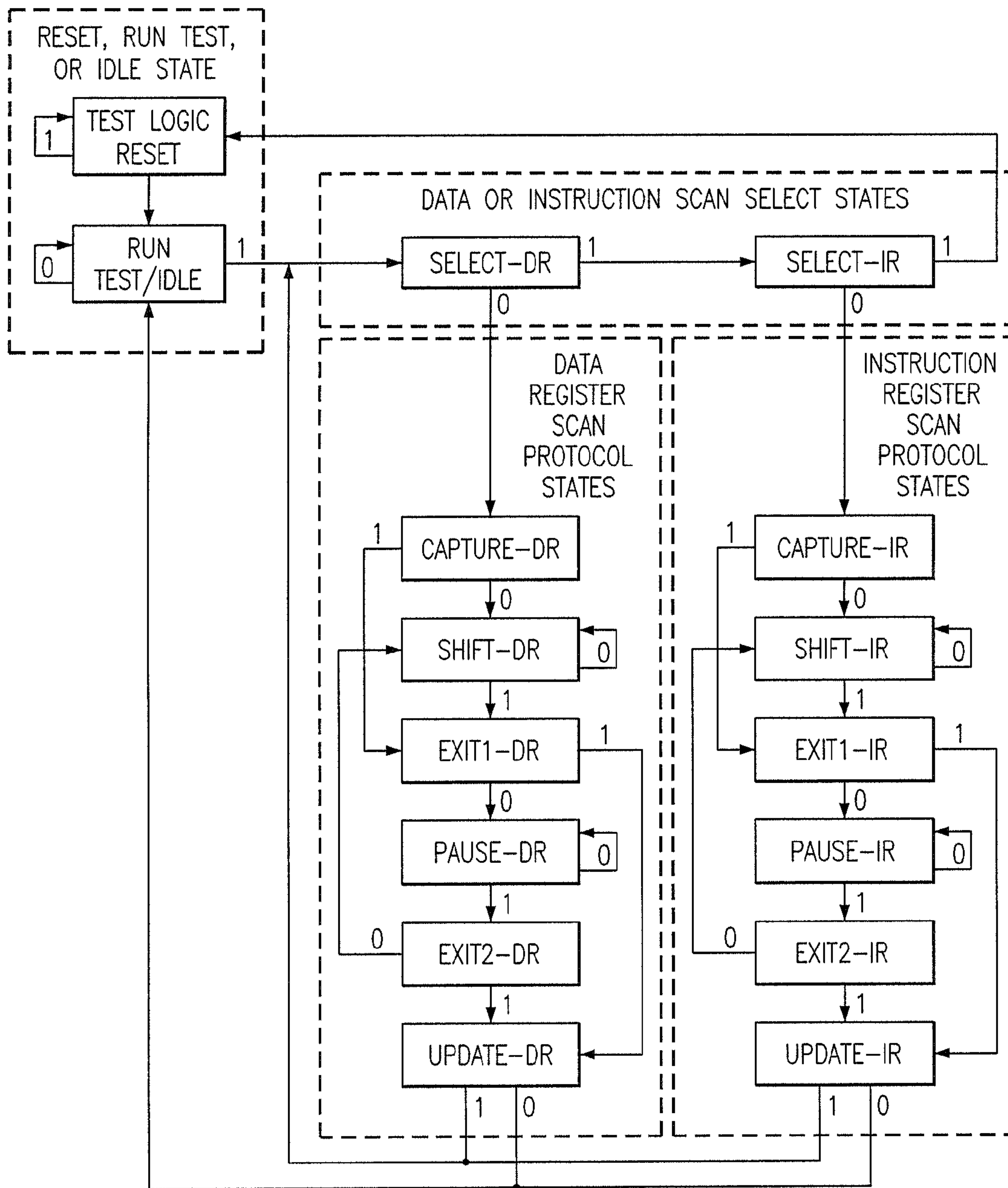
FIG. 2 (PRIOR ART)
