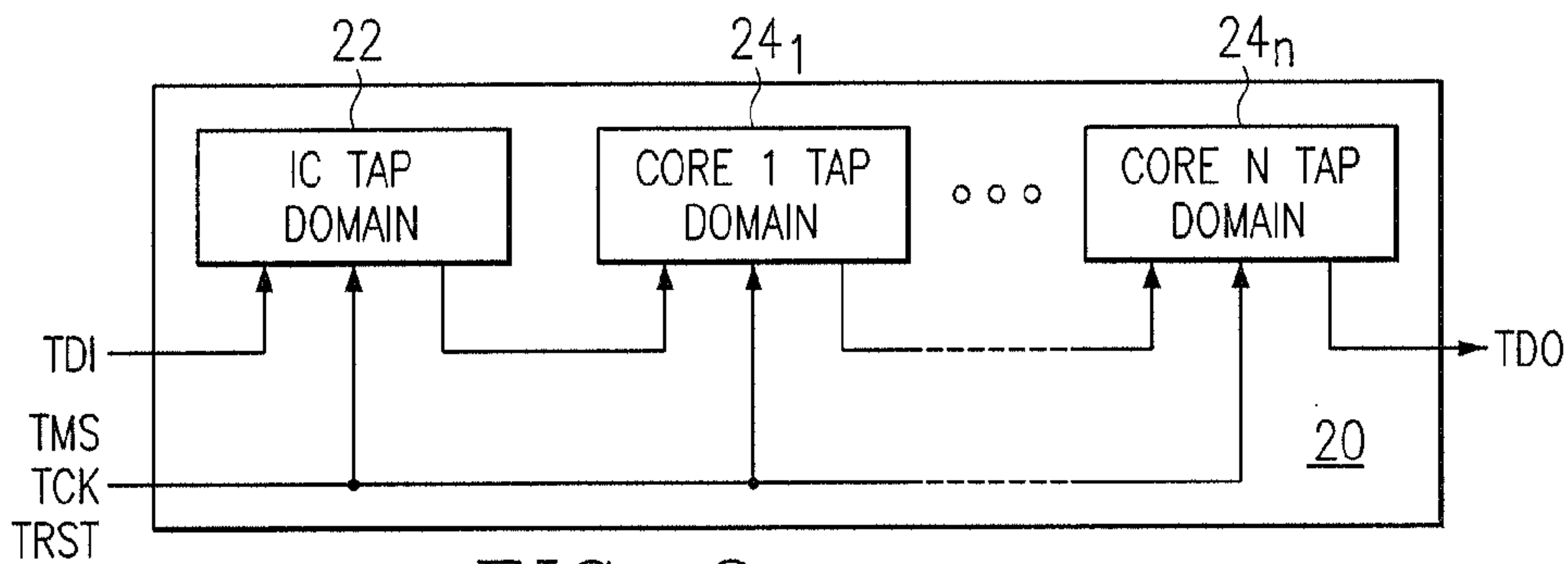
FIG. 3 (PRIOR ART)
