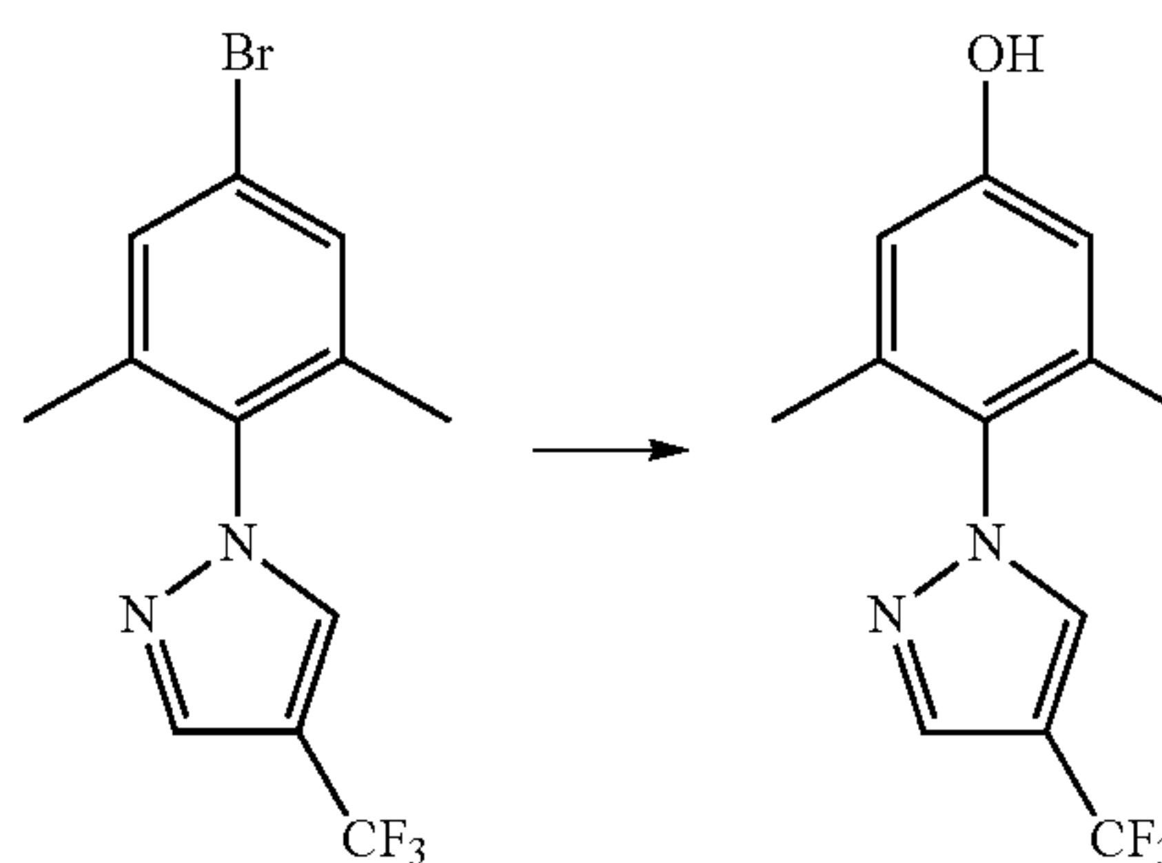
Step (1s): 3,5-dimethyl-4-(4-(trifluoromethyl)-1H-pyrazol-1-yl)phenol
