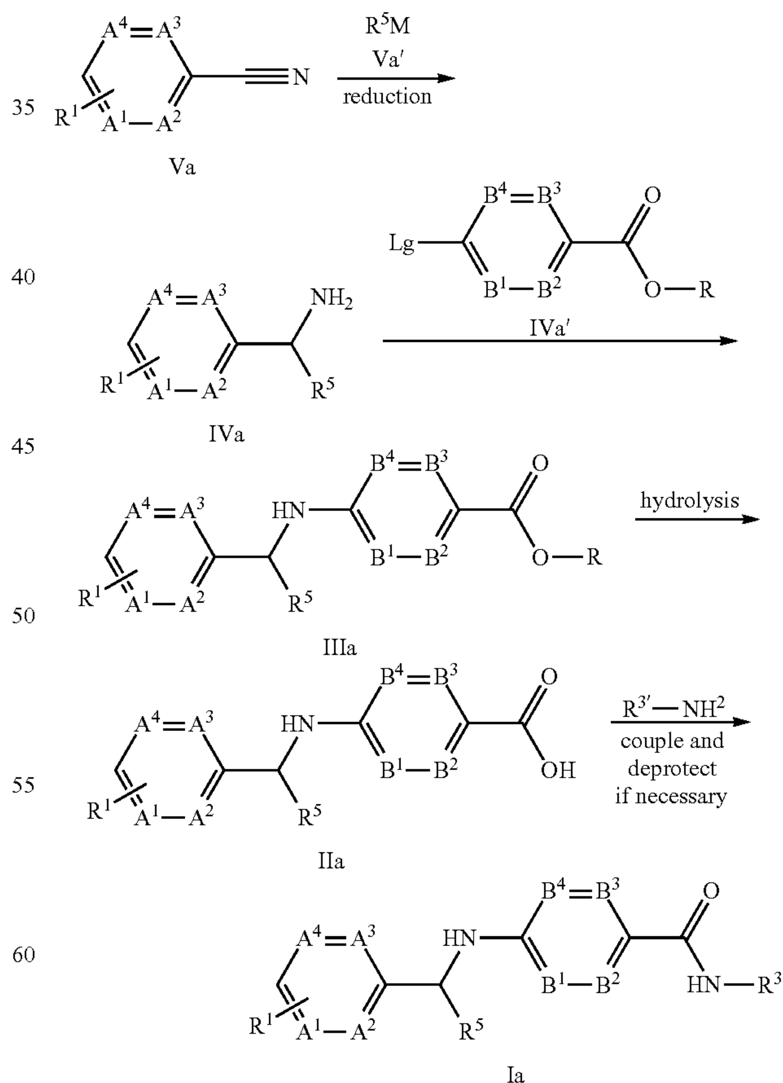
Reaction Scheme III
