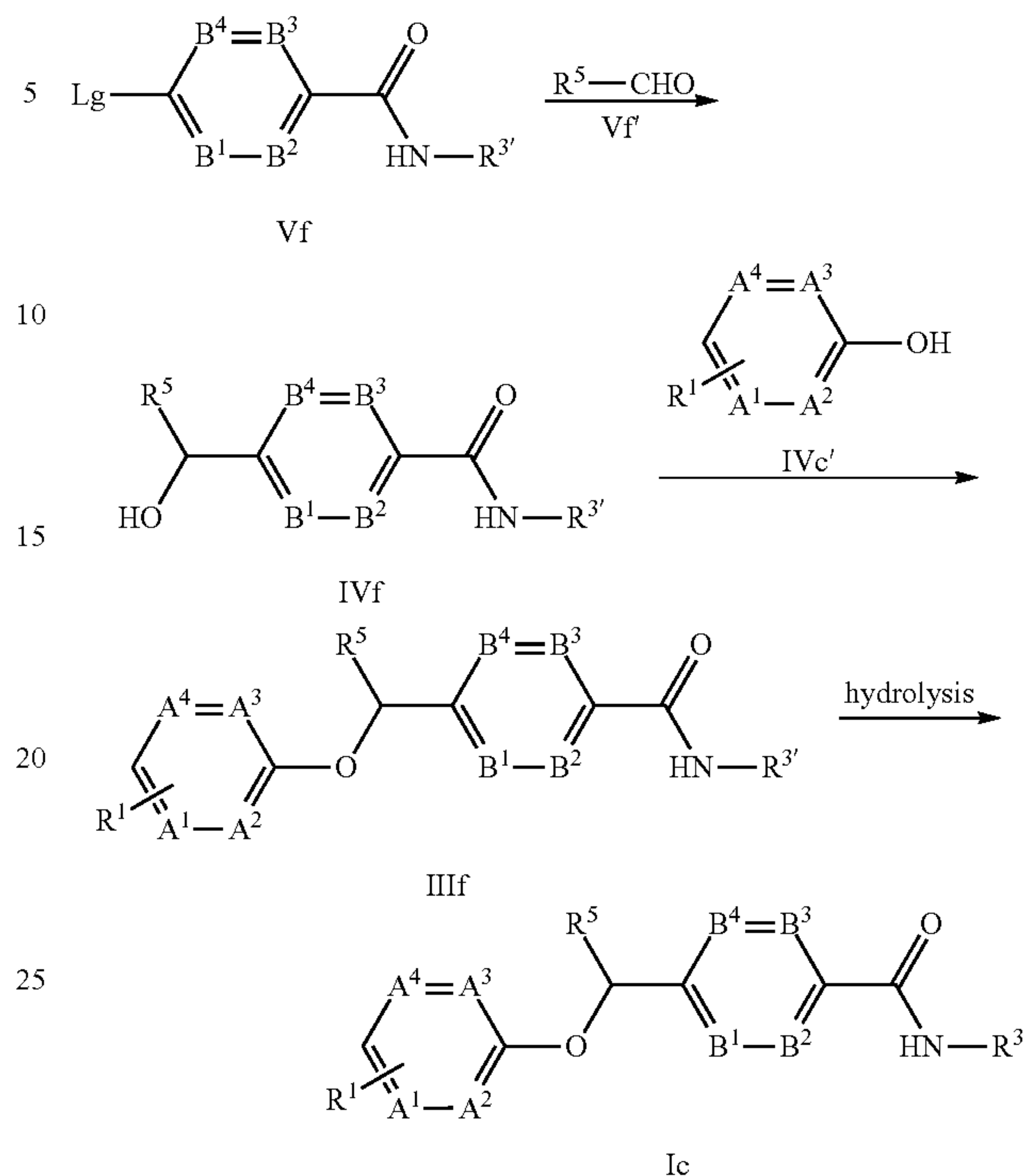
Reaction Scheme VIII
