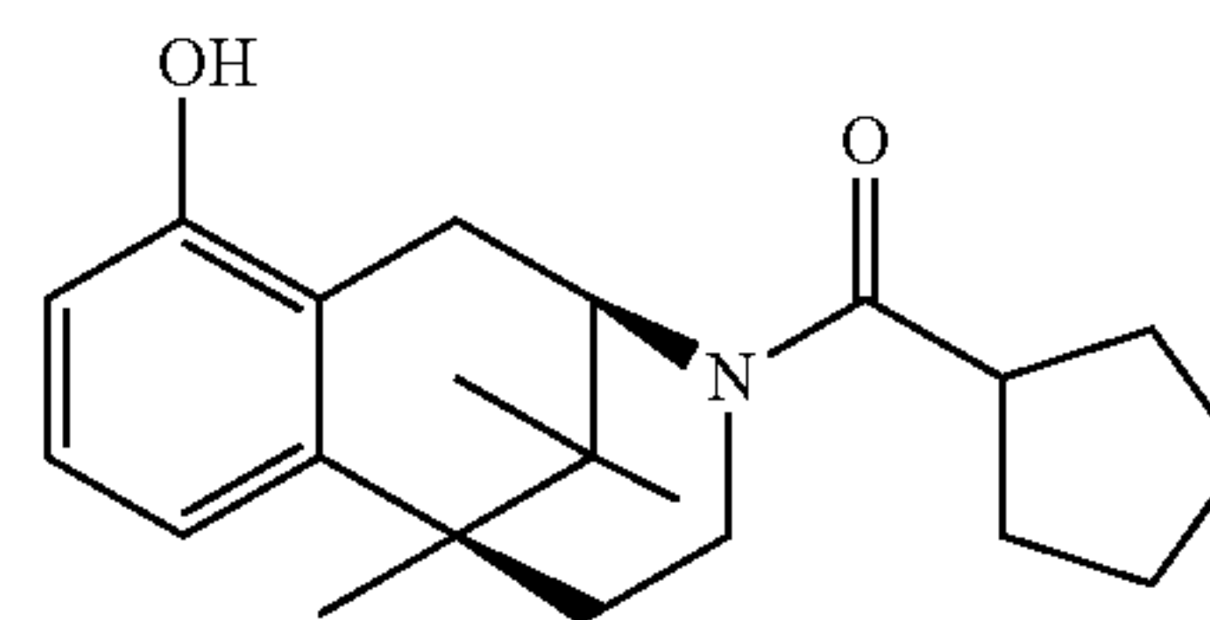
Cyclopentyl-[(2R,6S)-10-hydroxy-6,11,11-trimethyl-1,2,5,6-tetrahydro-4H-2,6-methano-benzo[d]azocin-3-yl]-methanone
