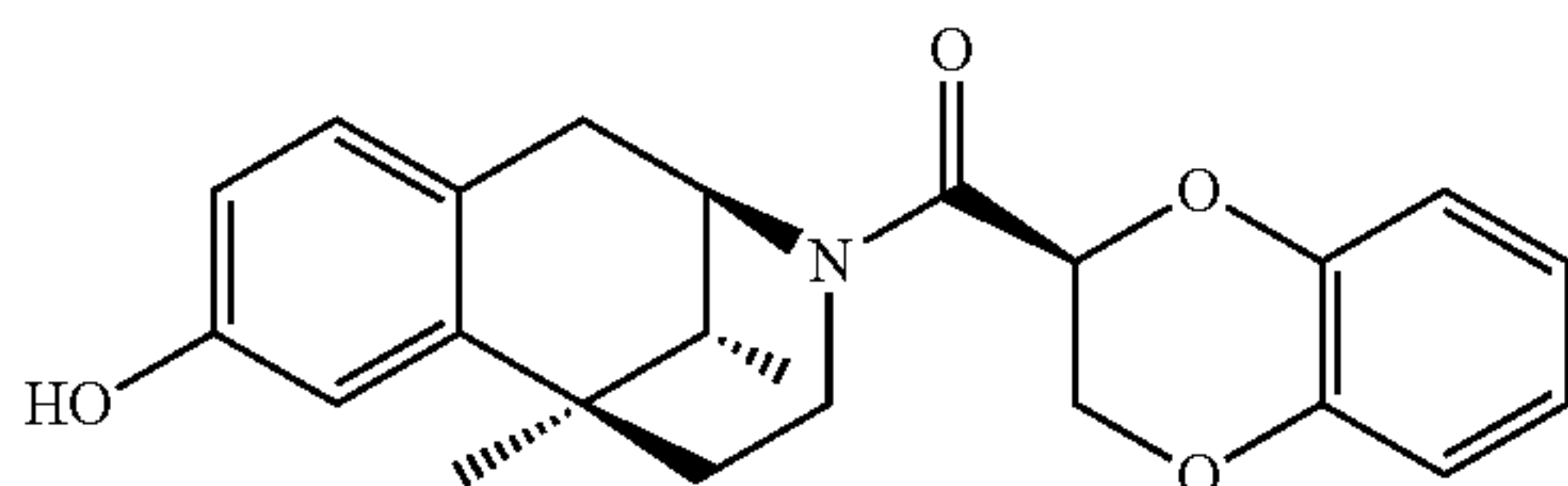
[(2S)-2,3-Dihydro-benzo[1,4]dioxin-2-yl]-[(2R,6R,11R)-8-hydroxy-6,11-dimethyl-1,2,5,6-tetrahydro-4H-2,6-methano-benzo[d]azocin-3-yl]-methanone
