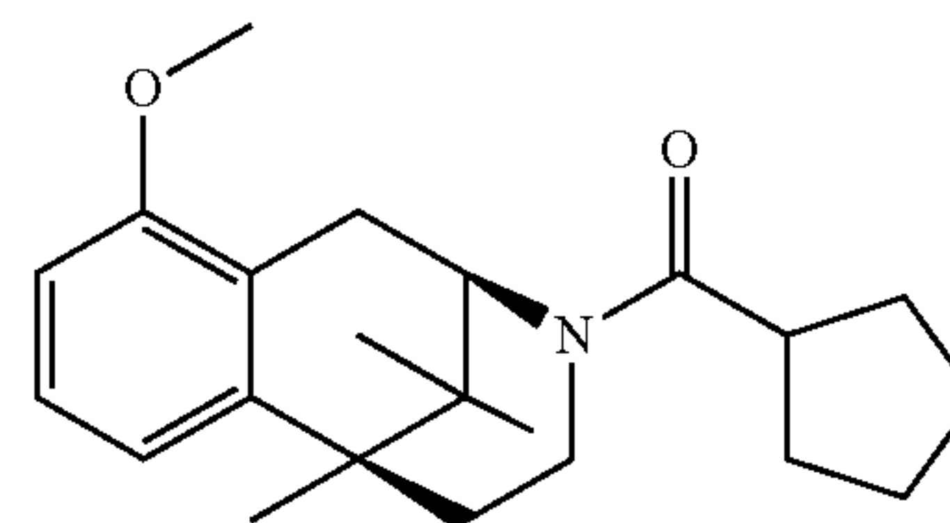
Cyclopentyl-[(2R,6S)-10-methoxy-6,11,11-trimethyl-1,2,5,6-tetrahydro-4H-2,6-methano-benzo[d]azocin-3-yl]-methanone
