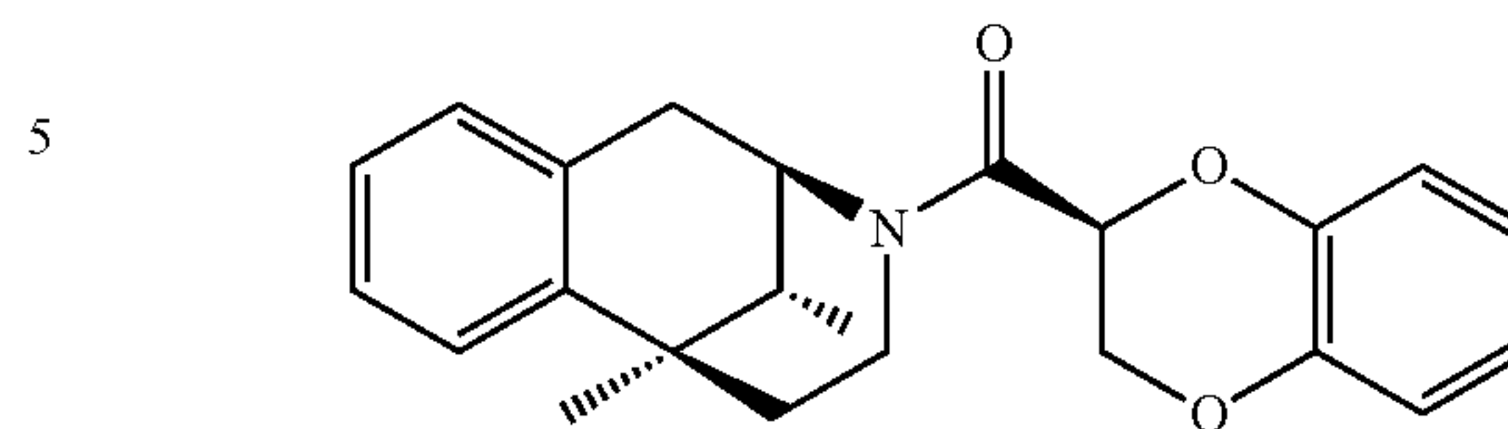
[(S)-2,3-Dihydro-benzo[1,4]dioxin-2-yl]-[(2R,6R,11R)-6,11-dimethyl-1,2,5,6-tetrahydro-4H-2,6-methano-benzo[d]azocin-3-yl]-methanone
