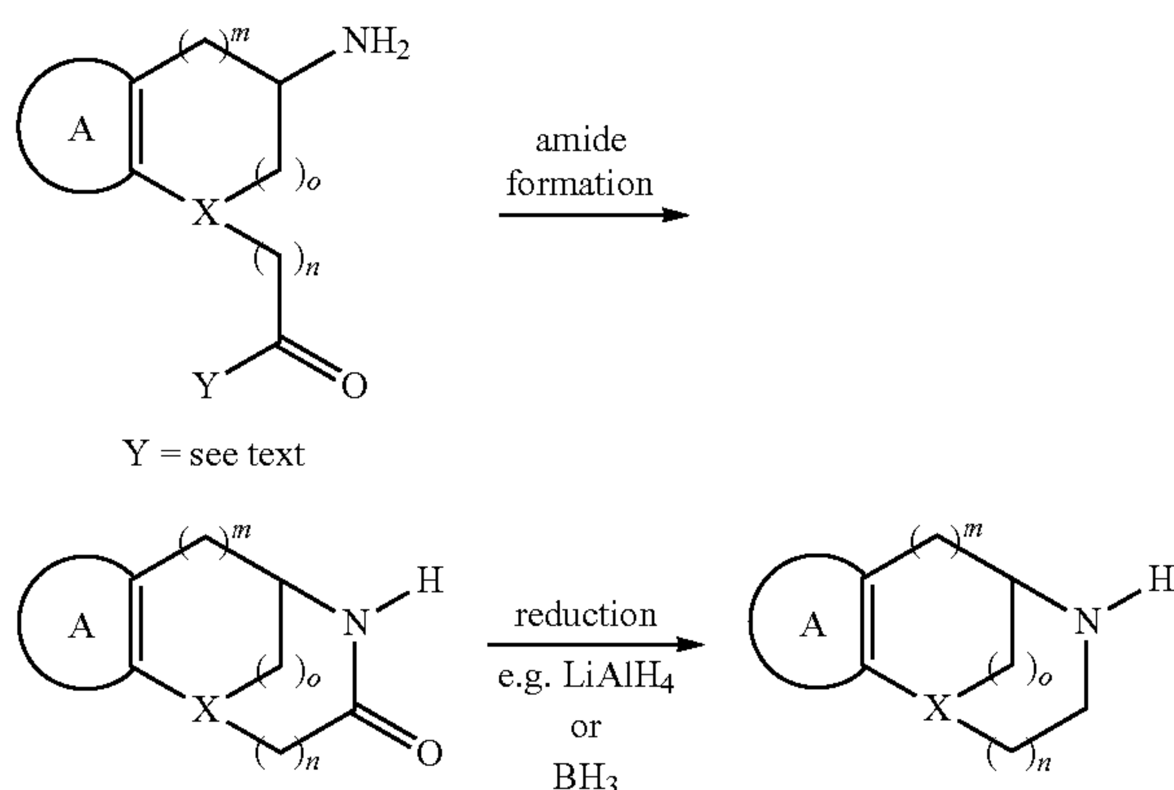
Scheme 1. Strategy 1 to build the bicyclic skeleton
