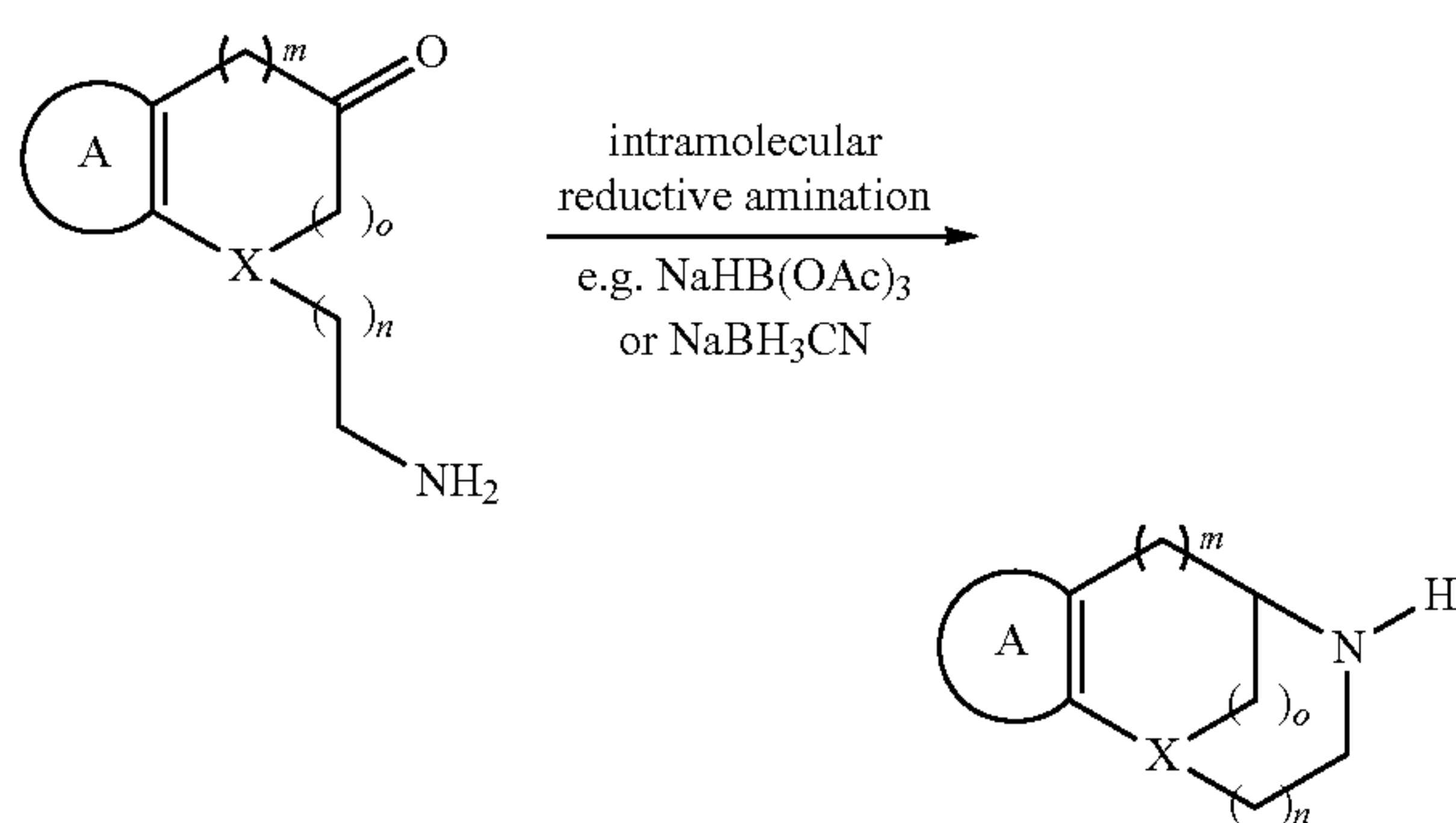
Scheme 2. Strategy 2 to build the bicyclic skeleton
