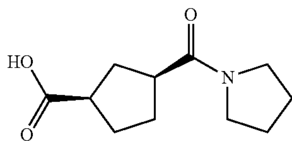
cis-3-(Pyrrolidine-1-carbonyl)-cyclopentanecarboxylic acid
