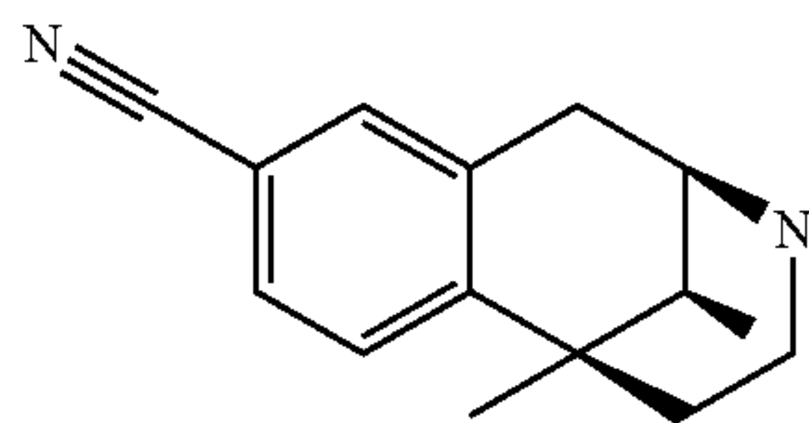
(2R,6R,11S)-6,11-Dimethyl-1,2,3,4,5,6-hexahydro-2,6-methano-benzo[d]azocine-9-carbonitrile
