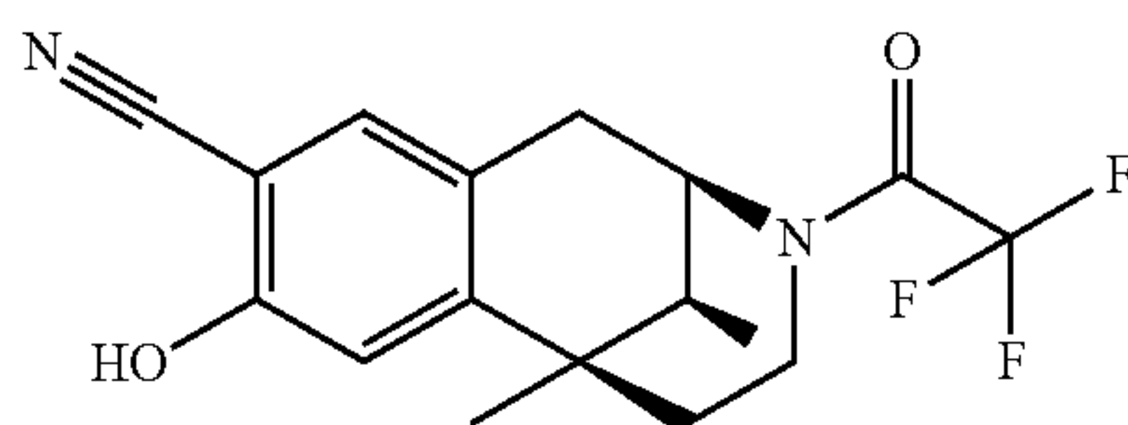
(2R,6R,11S)-8-Hydroxy-6,11-dimethyl-3-(2,2,2-trifluoro-acetyl)-1,2,3,4,5,6-hexahydro-2,6-methano-benzo[d]azocine-9-carbonitrile
