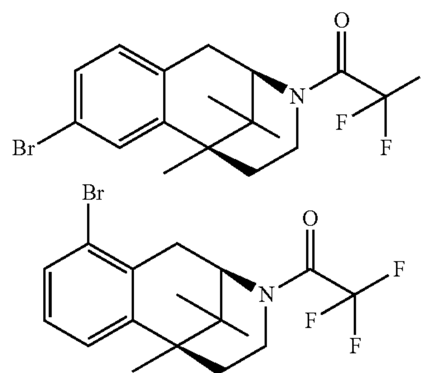
1-[(2R,6S)-8-Bromo-6,11,11-trimethyl-1,2,5,6-tetrahydro-4H-2,6-methano-benzo[d]azocin-3-yl]-2,2,2-trifluoro-ethanone and 1-[(2R,6S)-10-bromo-6,11,11-trimethyl-1,2,5,6-tetrahydro-4H-2,6-methano-benzo[d]azocin-3-yl]-2,2,2-trifluoro-ethanone
