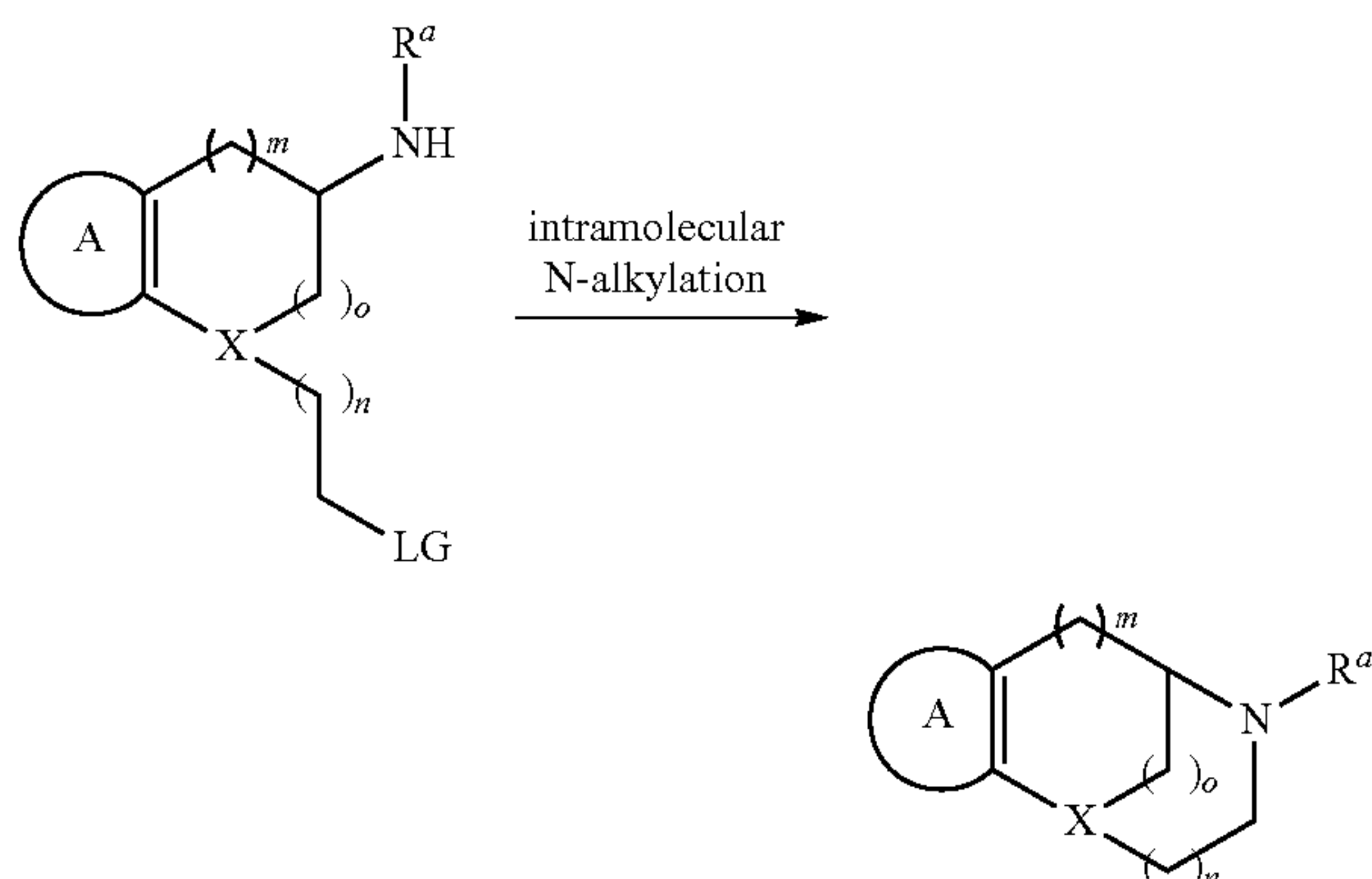
Scheme 4. Strategy 4 to build the bicyclic skeleton
