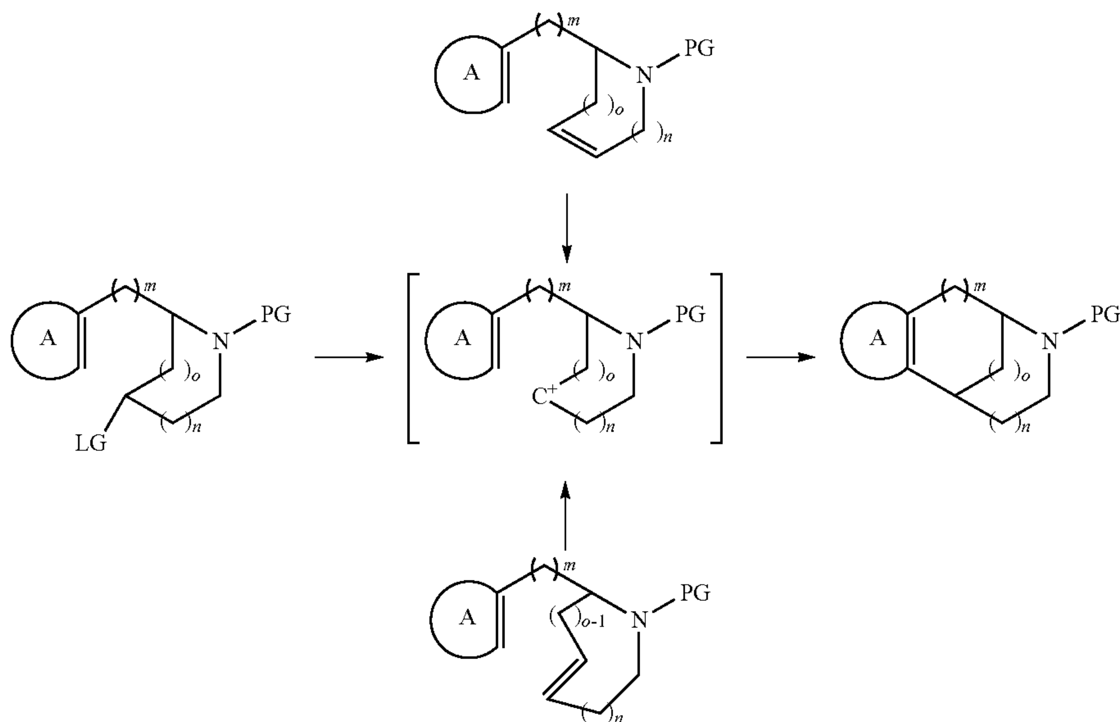
Scheme 5. Strategy 5 to build the bicyclic skeleton
