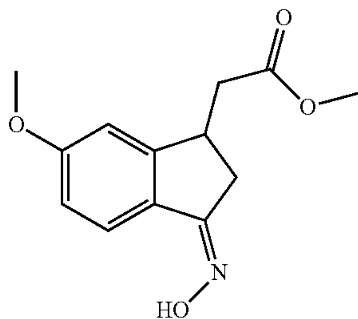
(3-Hydroxyimino-6-methoxy-indan-1-yl)-acetic acid methyl ester
