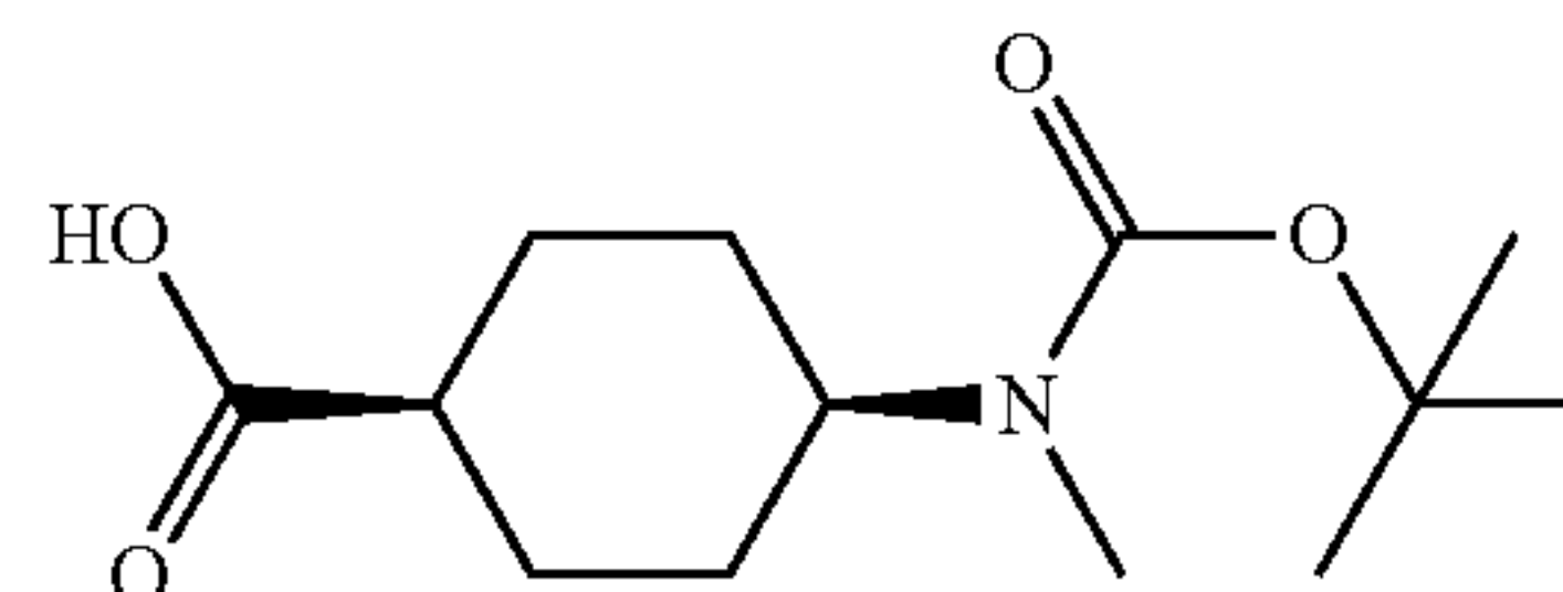
cis-4-(tert-Butoxycarbonyl-methyl-amino)-cyclohexanecarboxylic acid
