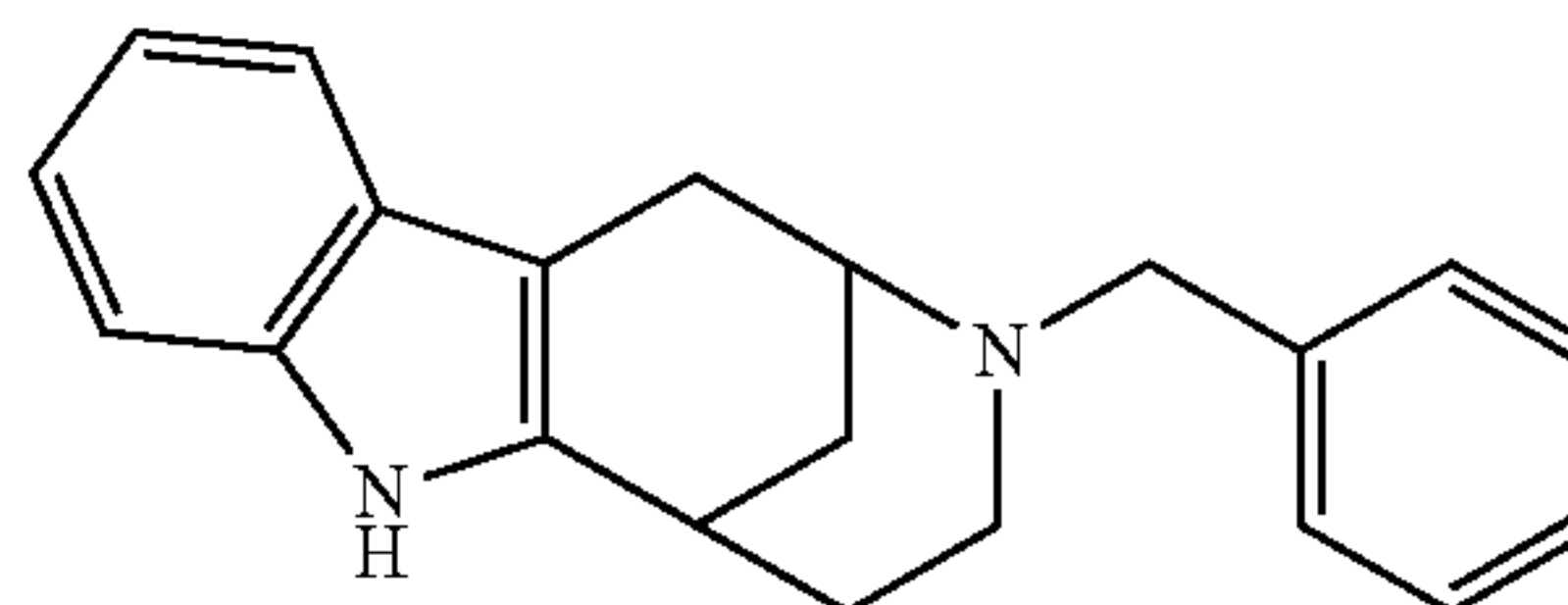
3-Benzyl-2,3,4,5,6,7-hexahydro-2,6-methano-1H-azocino[5,4-b]indole
