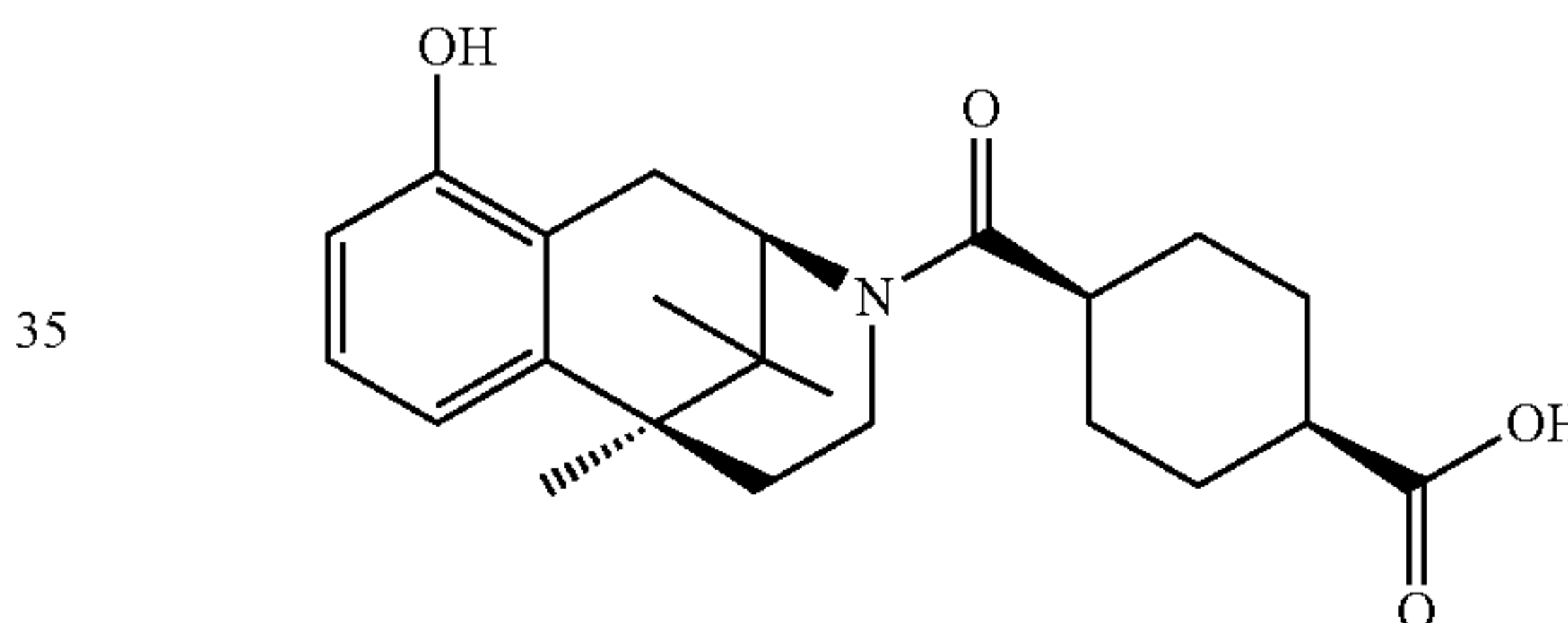
cis-4-[(2R,6S)-10-Hydroxy-6,11,11-trimethyl-1,2,5,6-tetrahydro-4H-2,6-methano-benzo[d]azocine-3-carbonyl]-cyclohexane carboxylic acid
