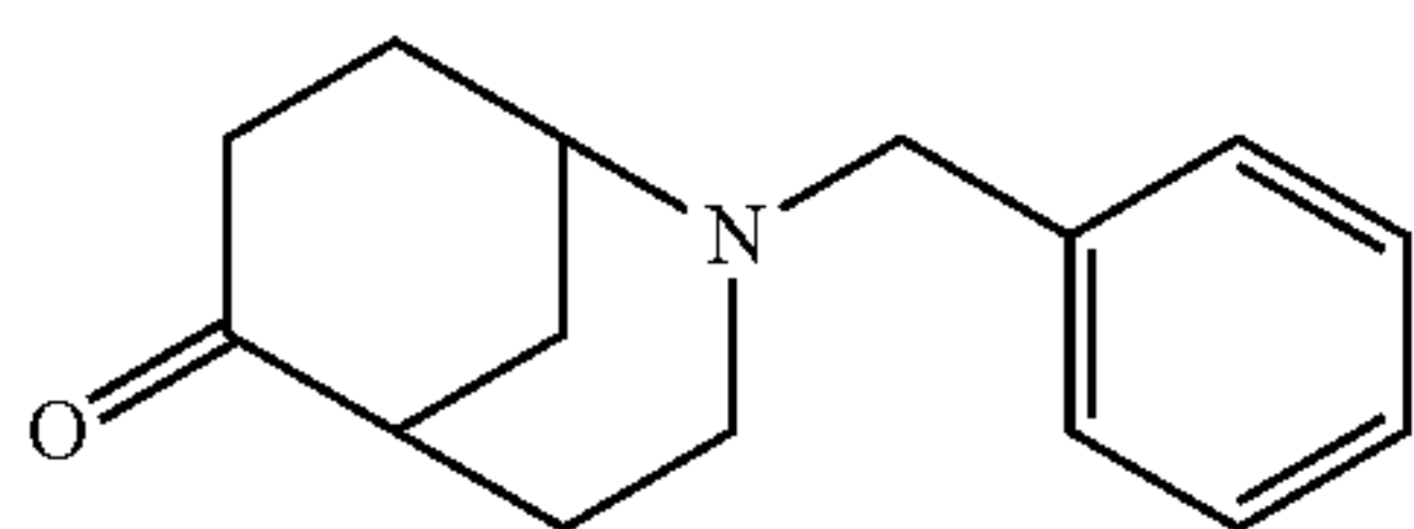
2-Benzyl-2-aza-bicyclo[3.3.1]nonan-6-one
