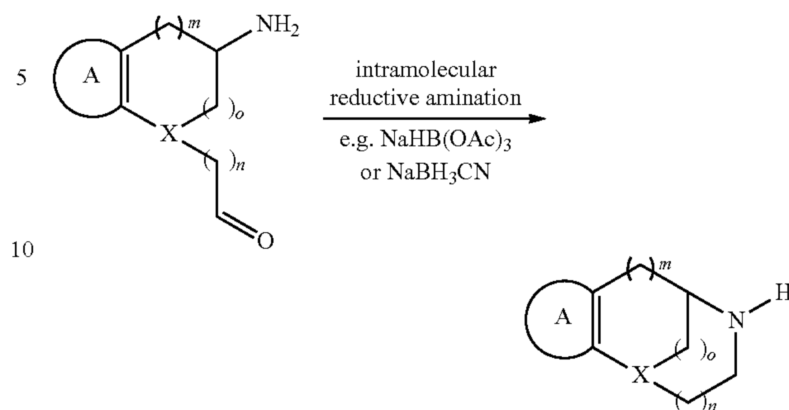
Scheme 3. Strategy 3 to build the bicyclic skeleton
