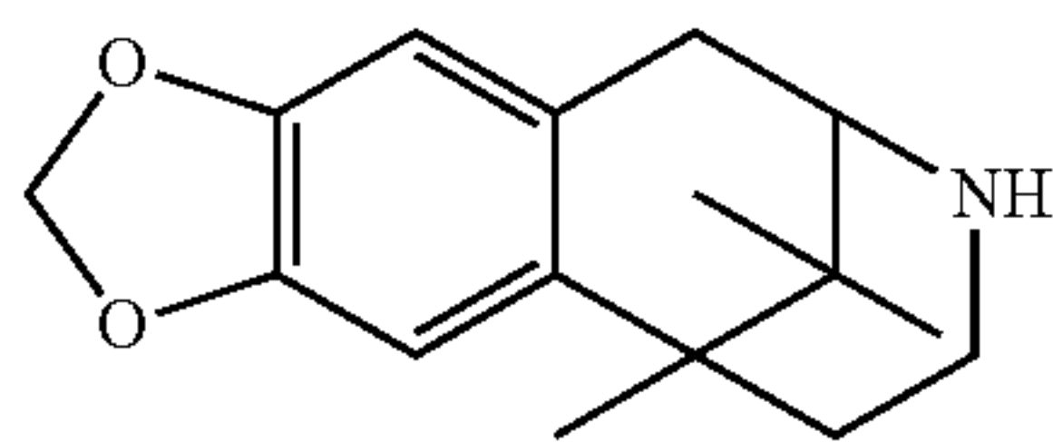
8,9-Methylenedioxy-6,11,11-trimethyl-1,2,3,4,5,6-hexahydro-2,6-methano-benzo[d]azocine
