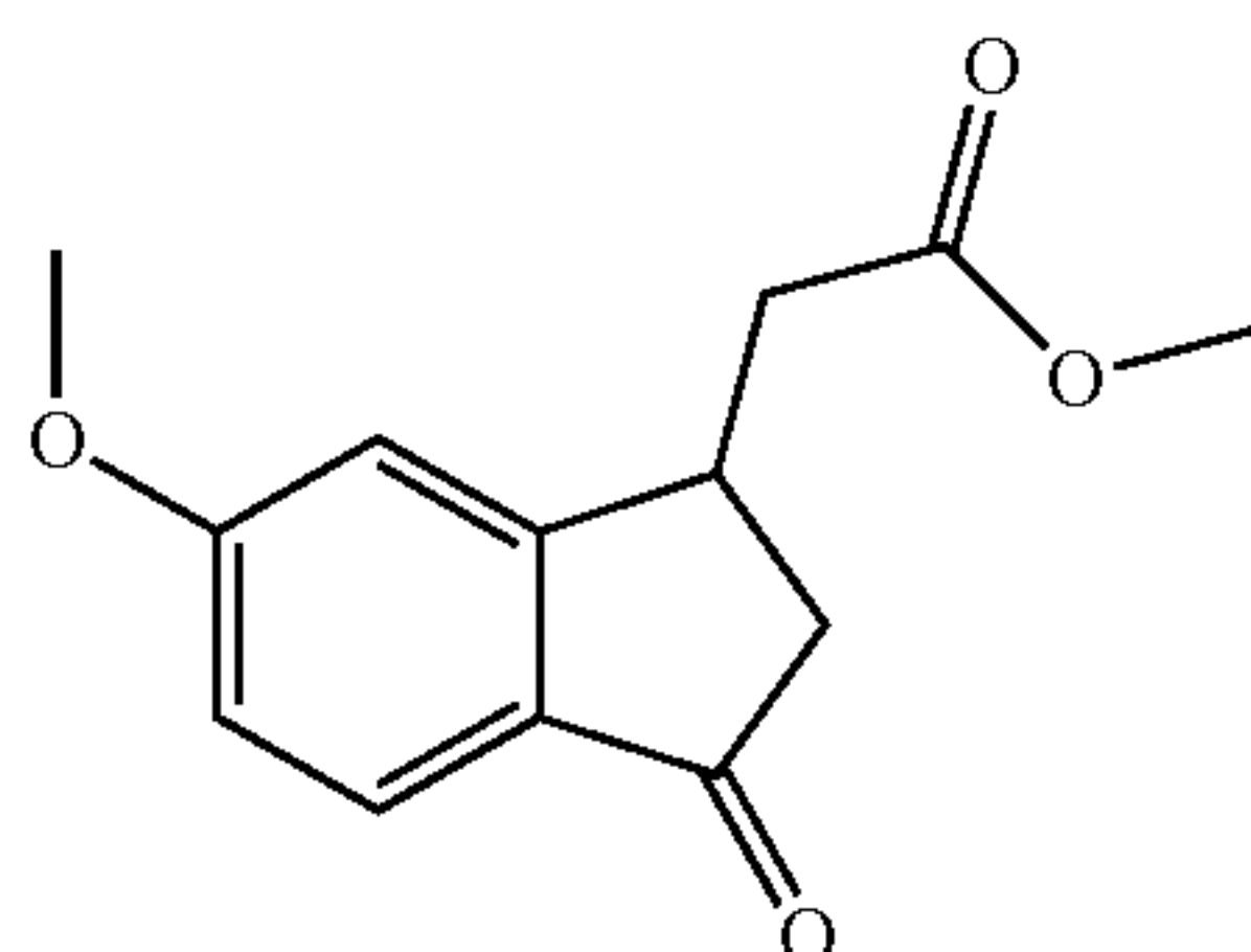
(6-Methoxy-3-oxo-indan-1-yl)-acetic acid methyl ester
