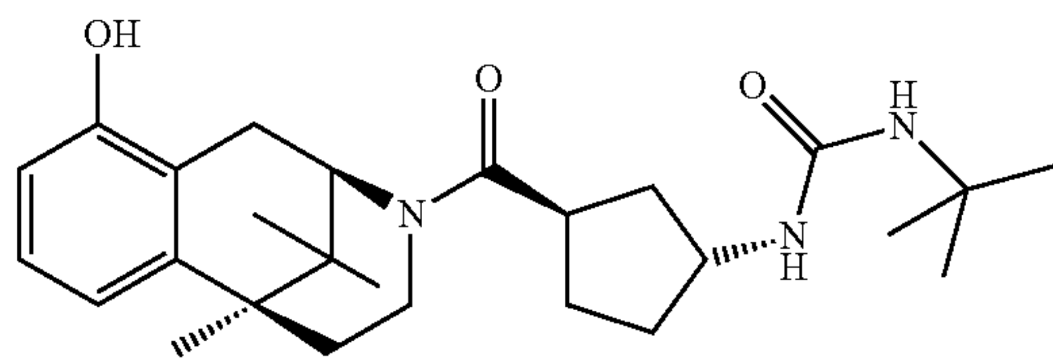
1-tert-Butyl-3-[(1R,3R)-3-[(2R,6S)-10-hydroxy-6,11,11-trimethyl-1,2,5,6-tetrahydro-4H-2,6-methano-benzo[d]azocine-3-carbonyl]-cyclopentyl]-urea
