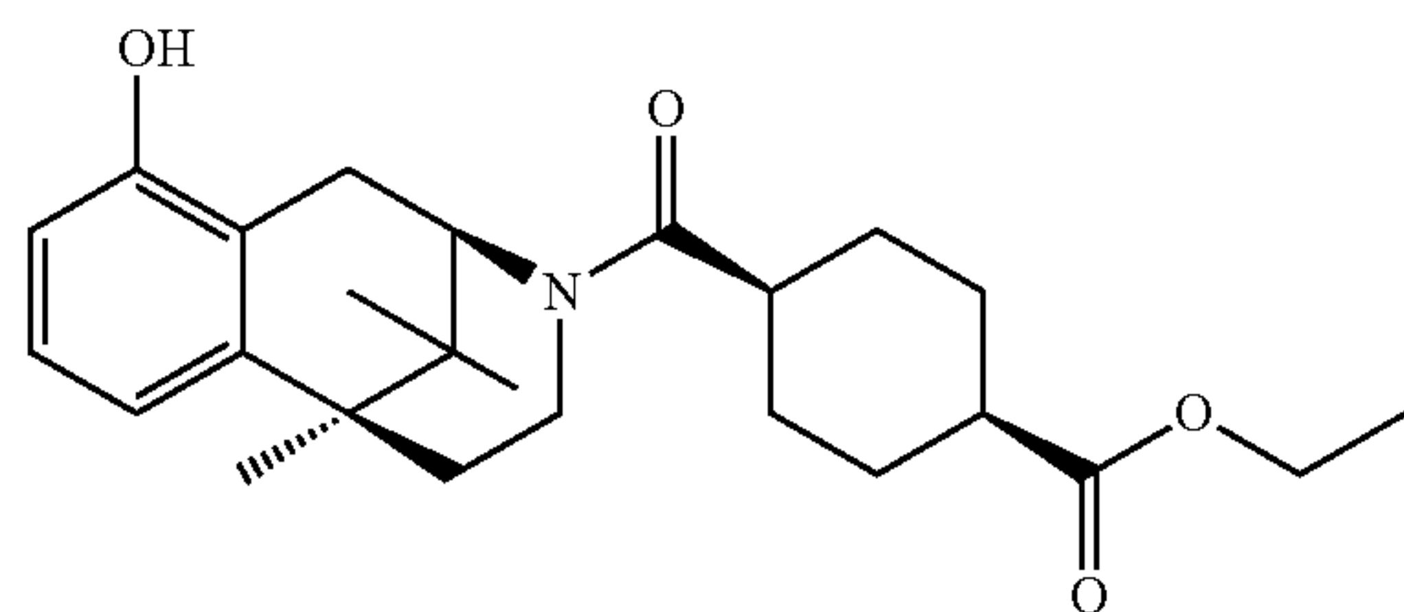
4-[(2R,6S)-10-Hydroxy-6,11,11-trimethyl-1,2,5,6-tetrahydro-4H-2,6-methano-benzo[d]azocine-3-carbonyl]-cyclohexanecarboxylic acid ethyl ester
