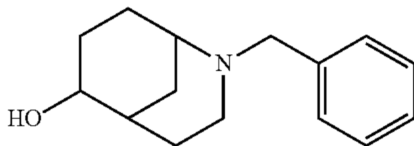
2-Benzyl-2-aza-bicyclo[3.3.1]nonan-6-ol
