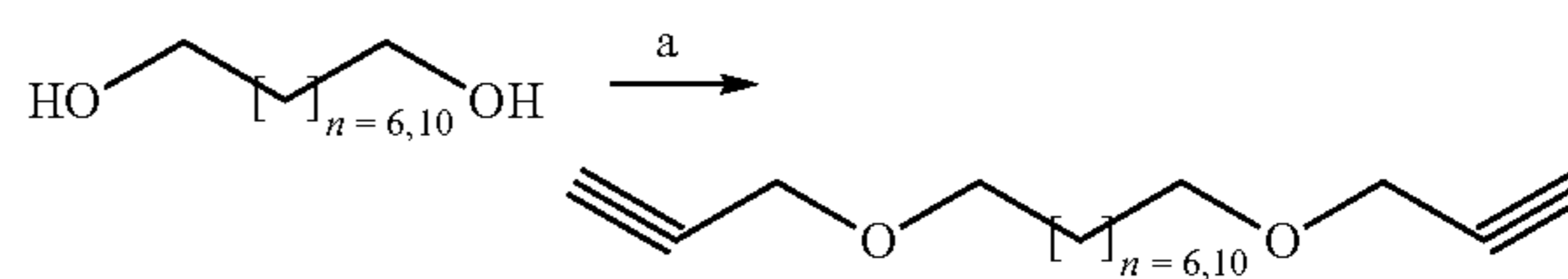
Scheme 10: Synthesis scheme of dialkynes used in the synthesis of Neomycin Neomycin dimer's.
