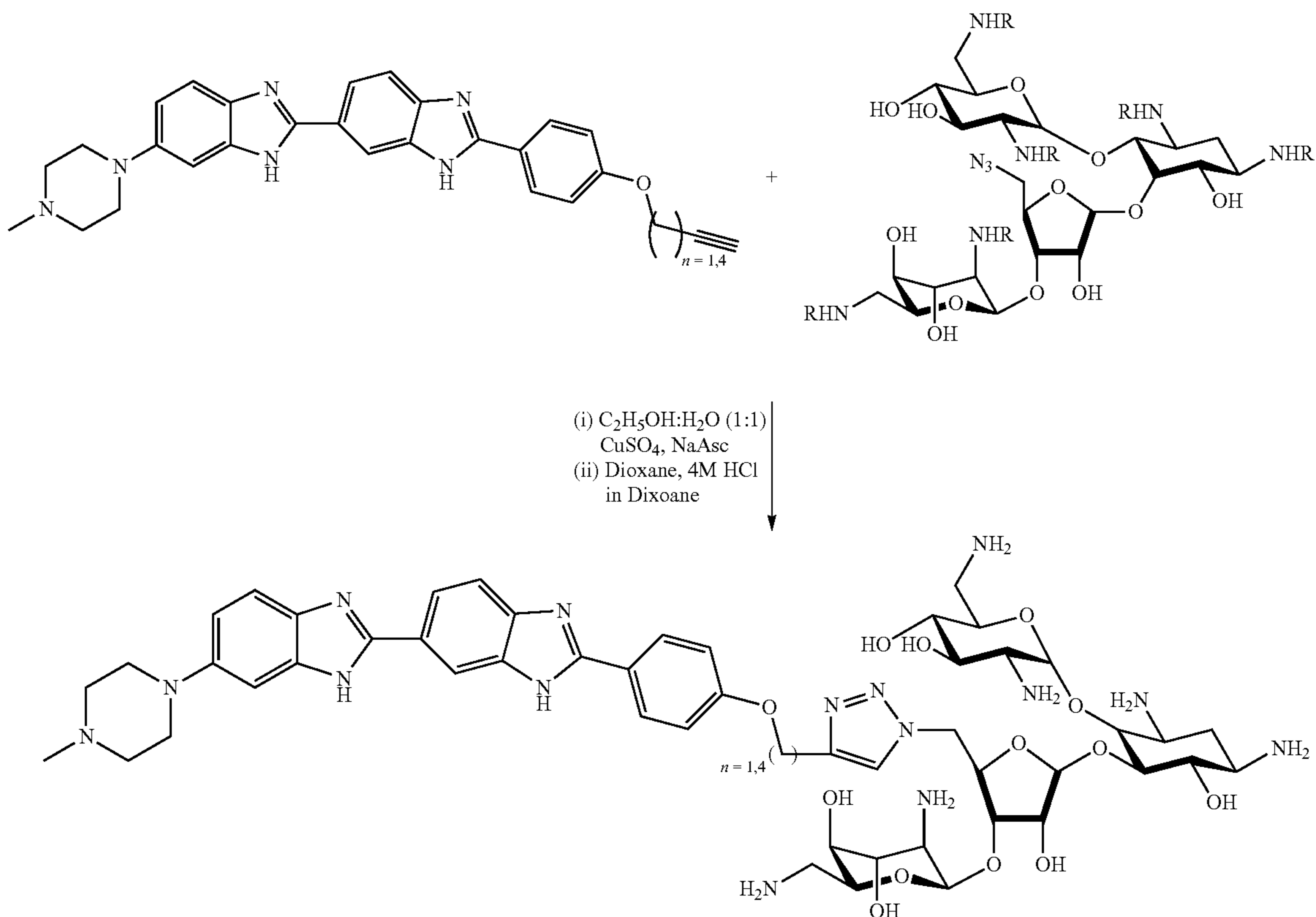
Scheme 9: Synthesis of Neomycin-Hoechst conjugates using click chemistry
