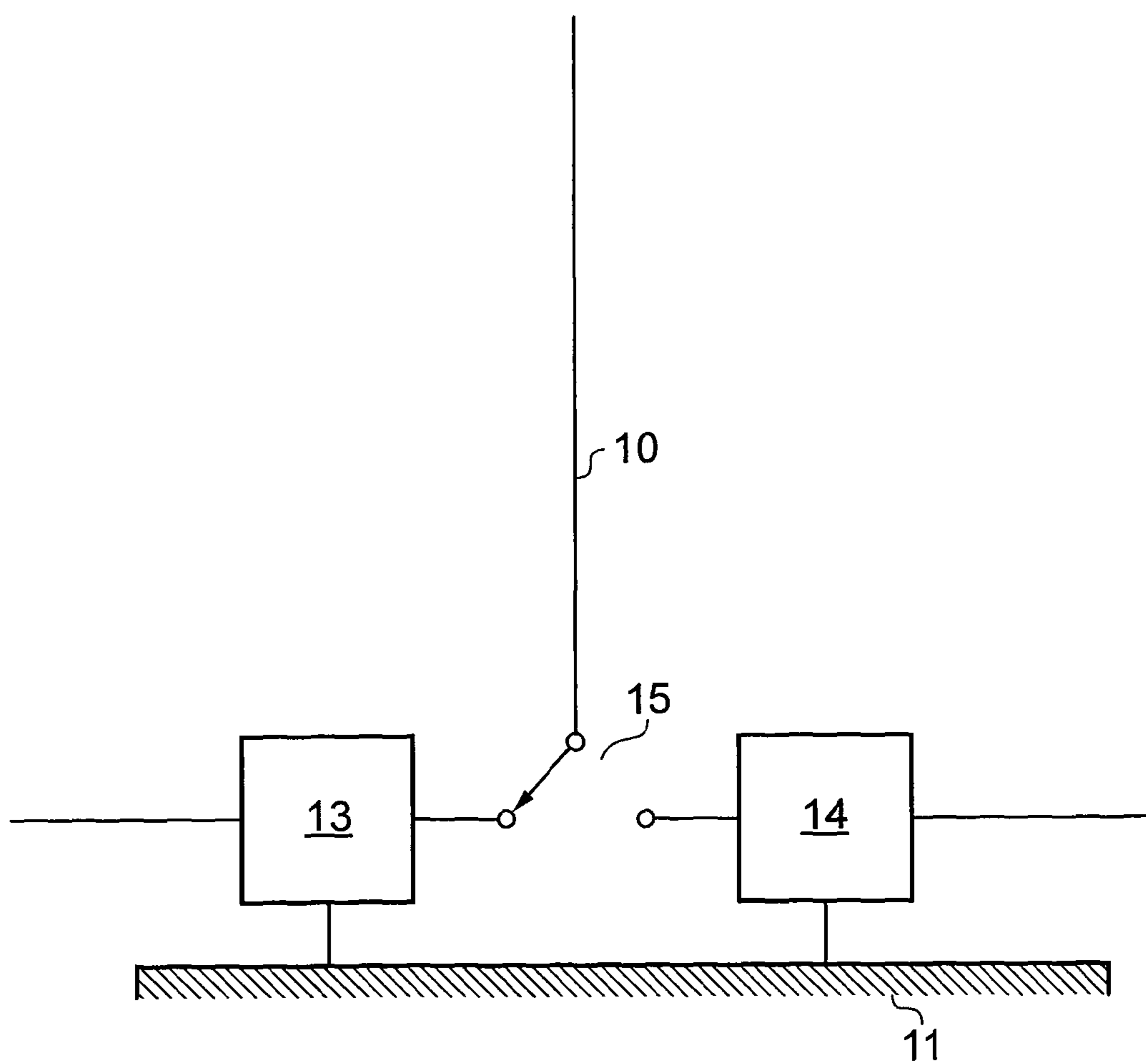
FIG. 2 (Prior Art)
