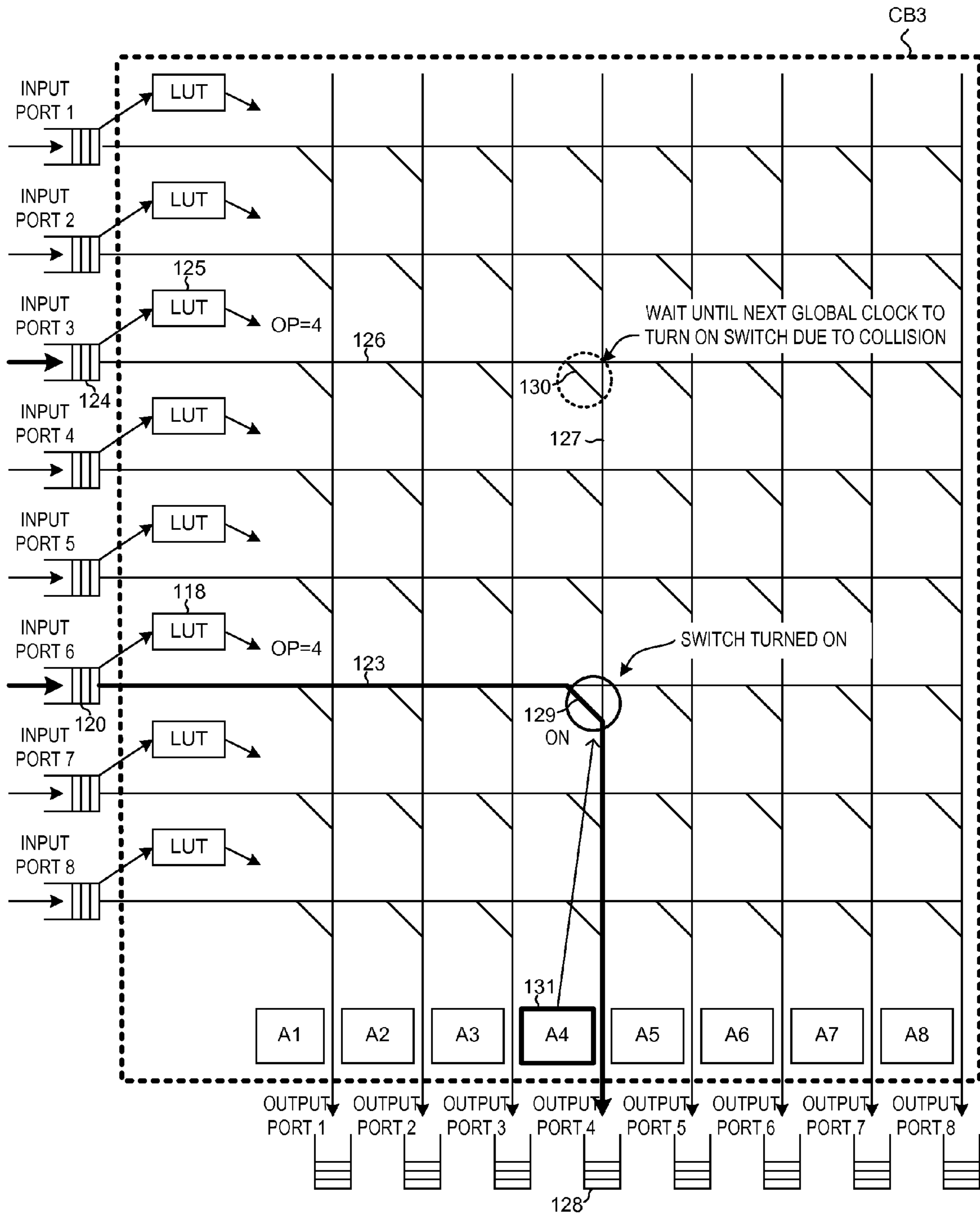
8-WAY CROSSBAR SWITCH FIG. 13
