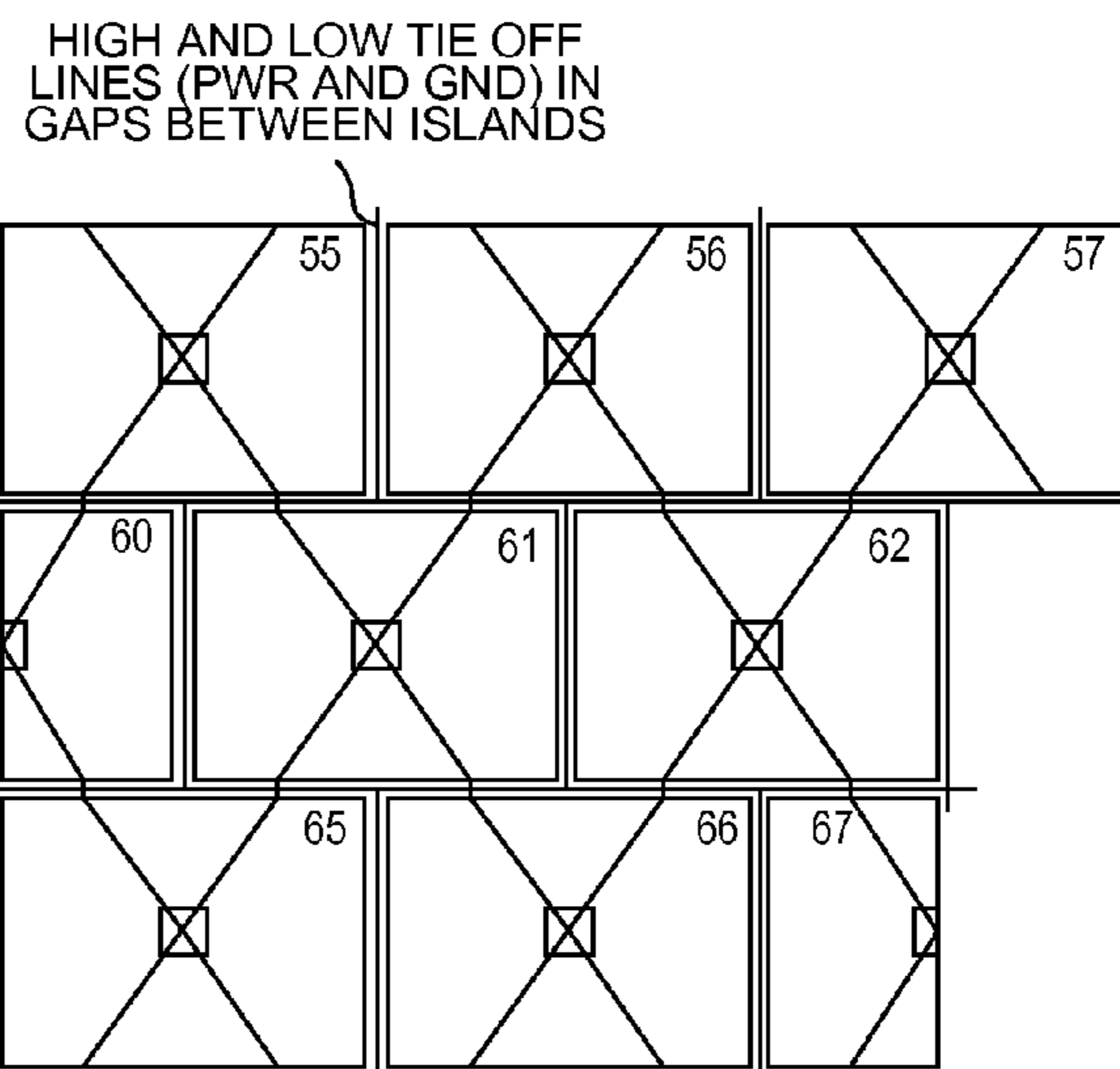
CONFIGURABLE MESH CONTROL BUS FIG. 27
