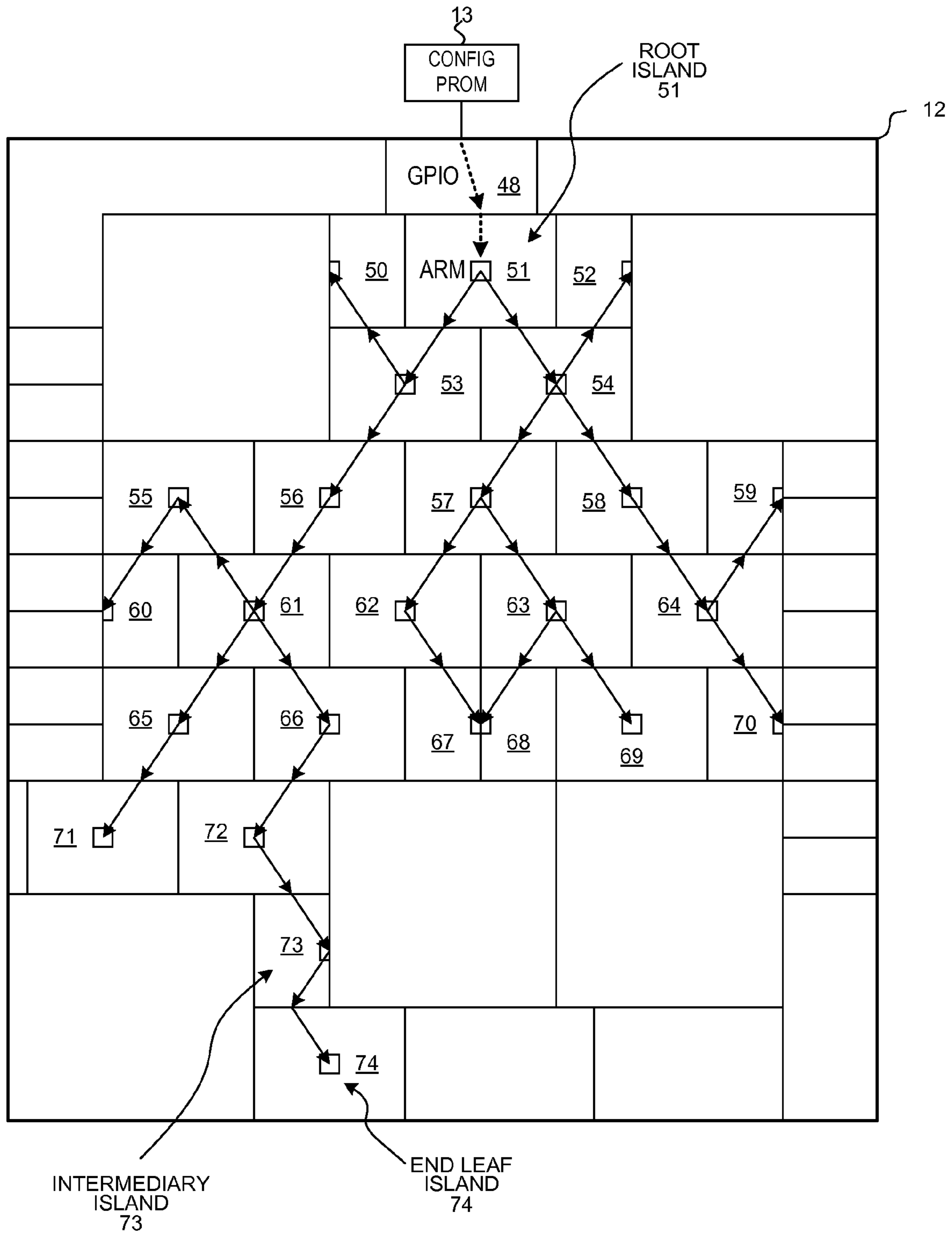
CONFIGURED CONFIGURABLE MESH CONTROL BUS
