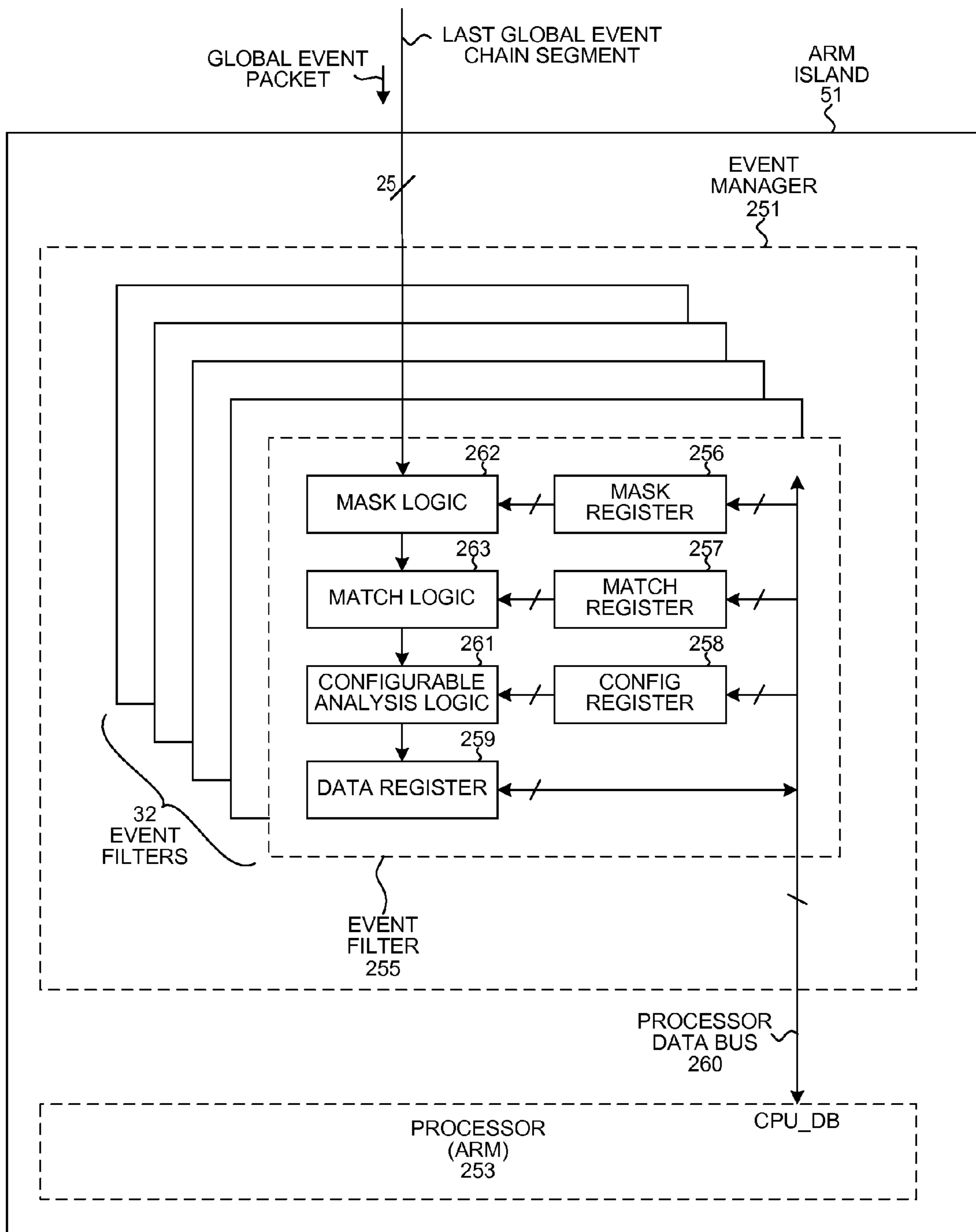
EVENT MANAGER
