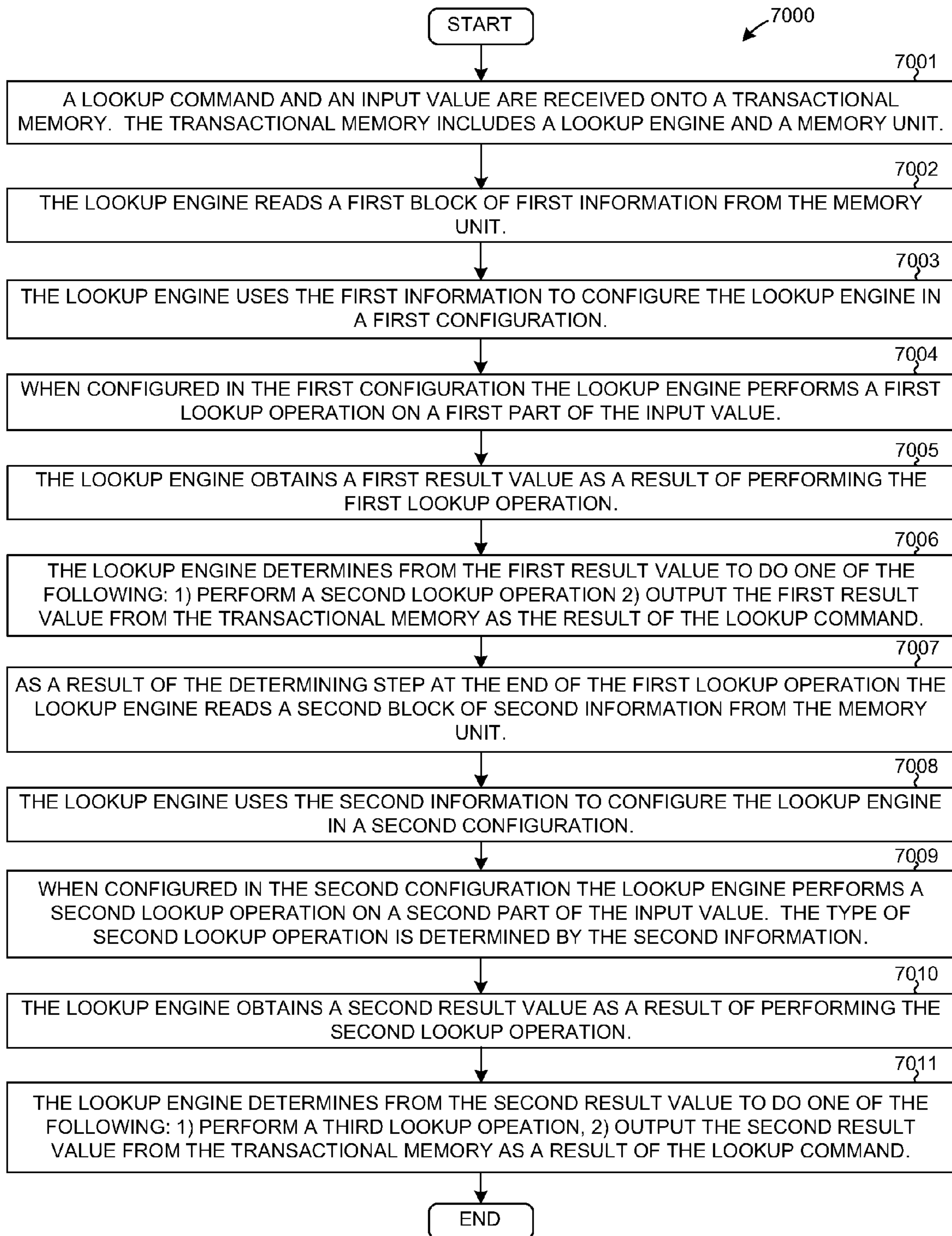
RECURSIVE USE OF MULTIPLE HARDWARE LOOKUP STRUCTURES
