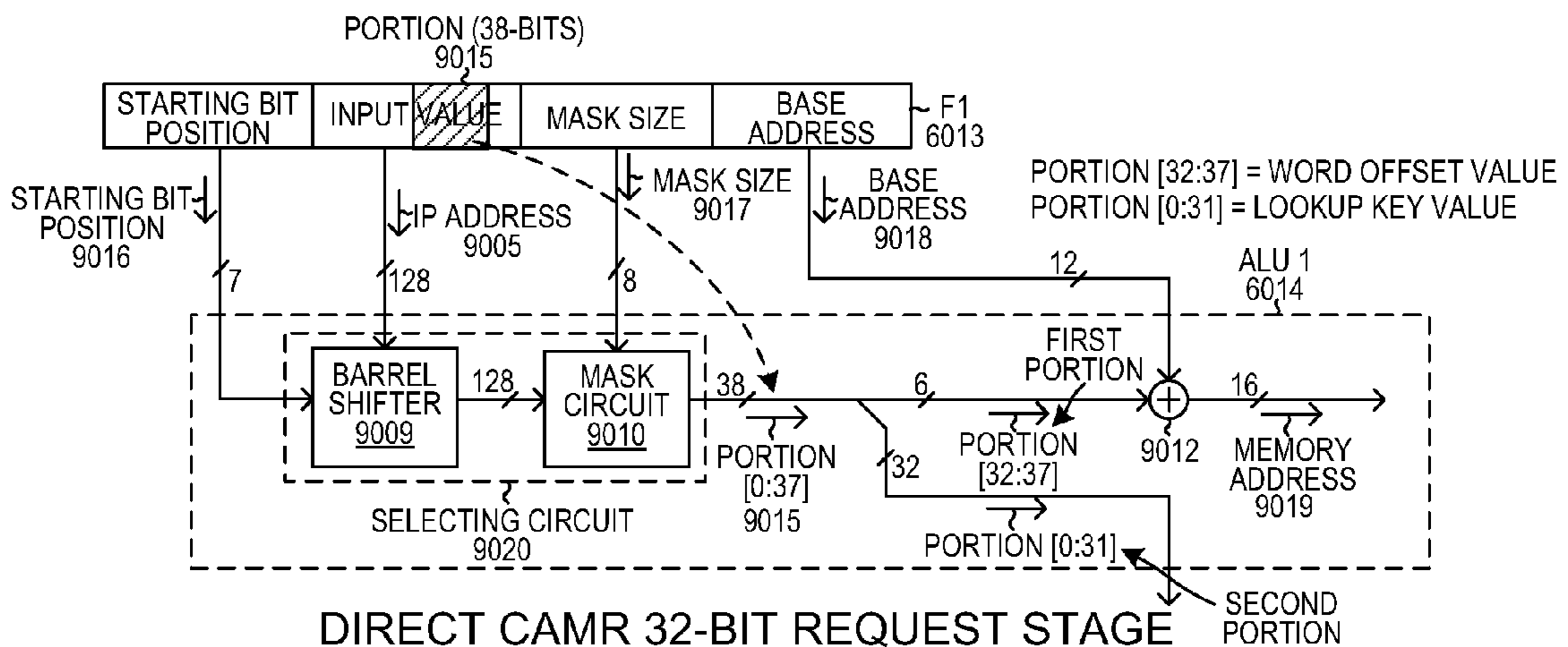
DIRECT CAMR 32-BIT LOOKUP MEMORY PACKING FIG. 52
