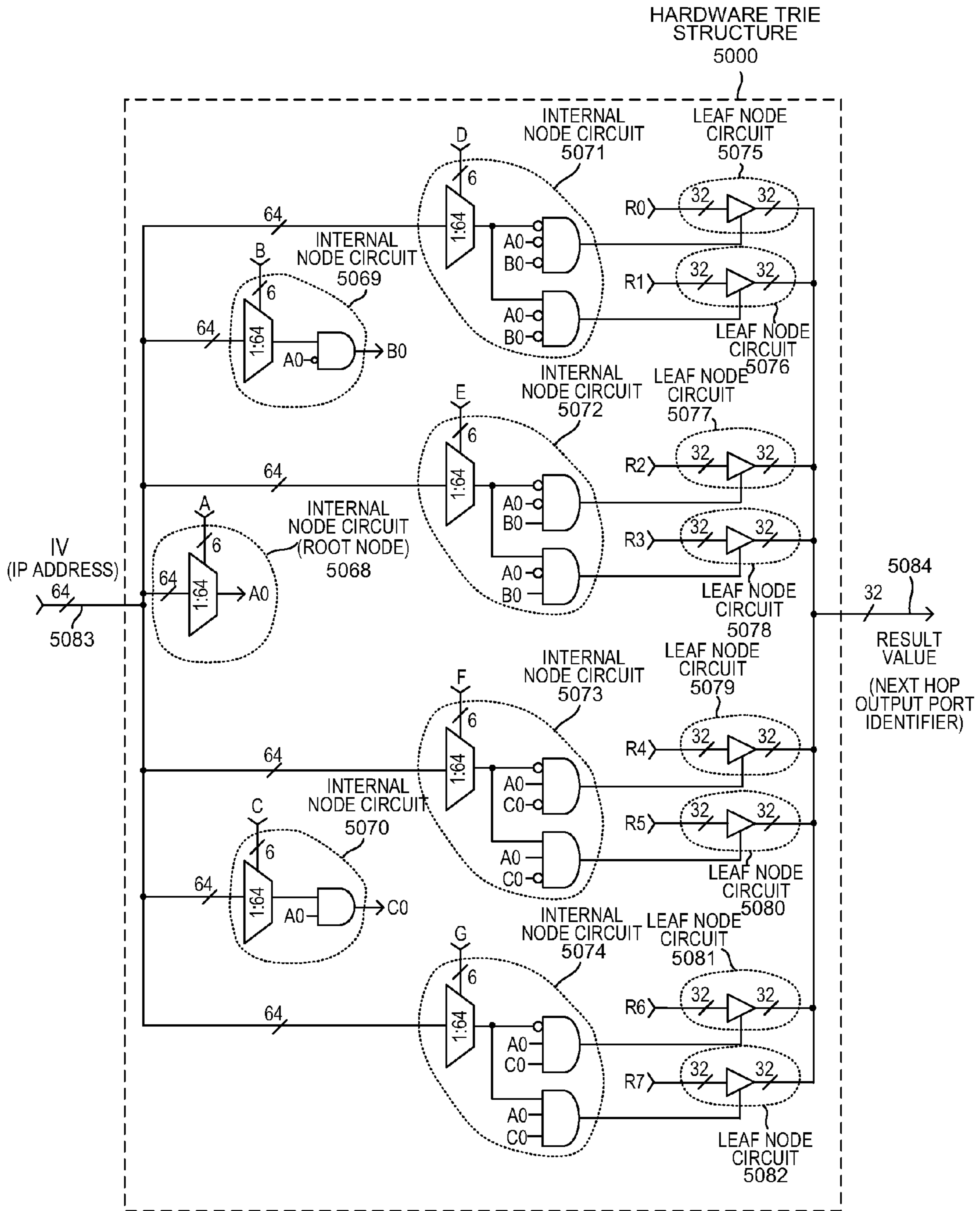
HARDWARE TRIE STRUCTURE
