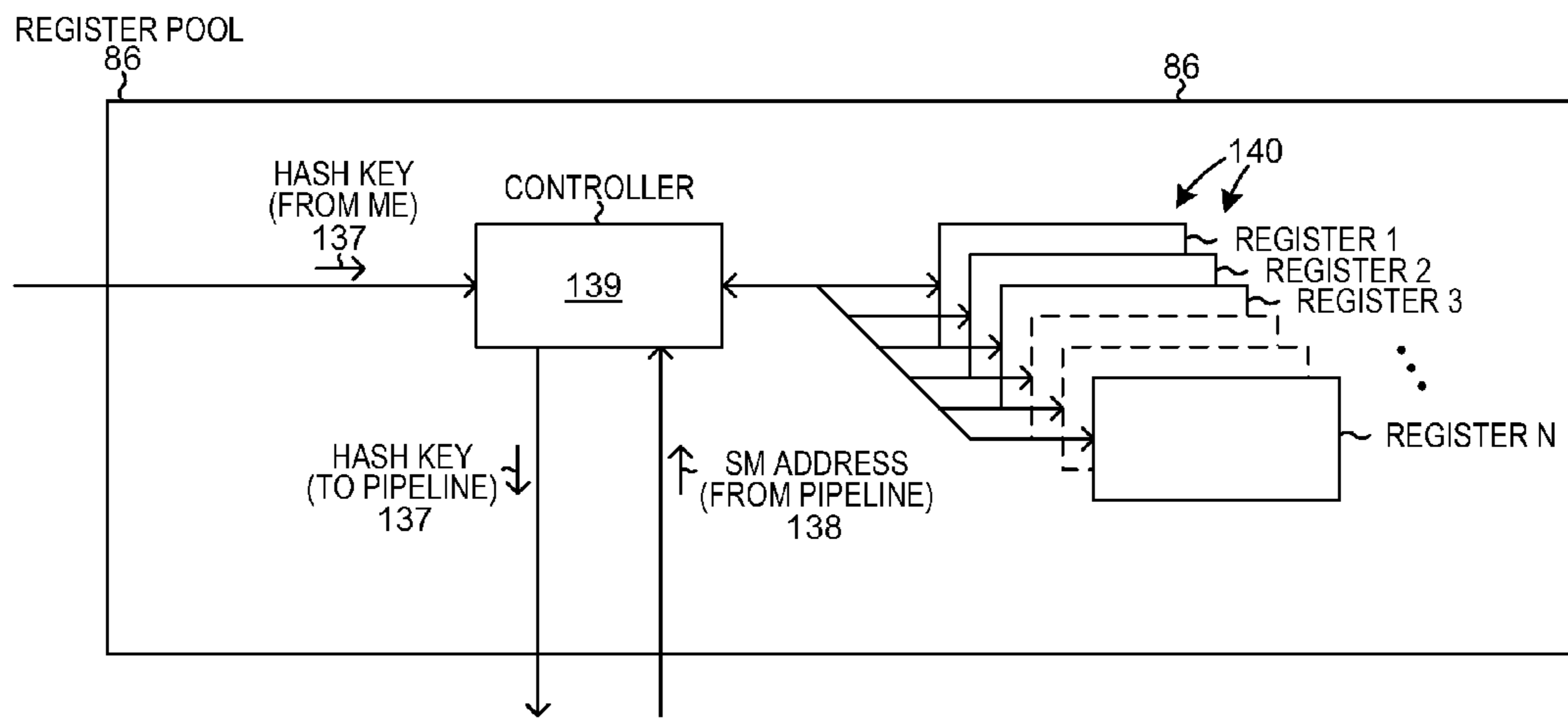
REGISTER POOL FIG. 17
