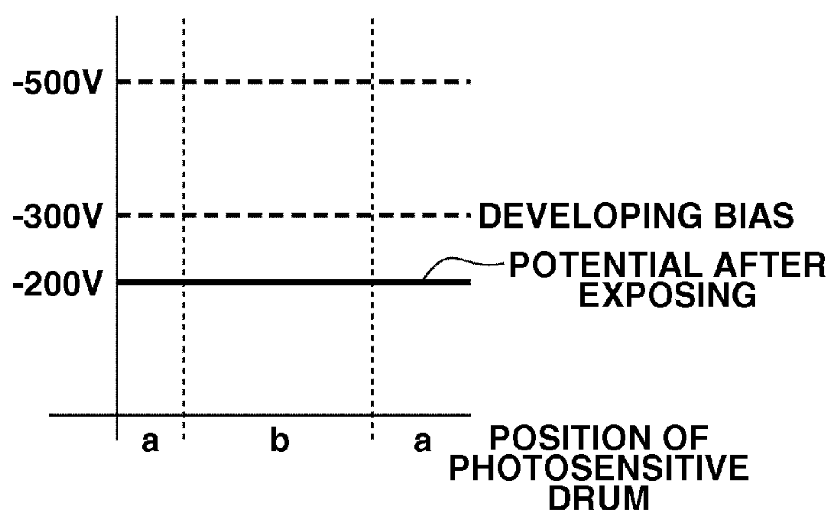
FIG.5C AFTER PASSING THROUGH EXPOSURE POSITION
