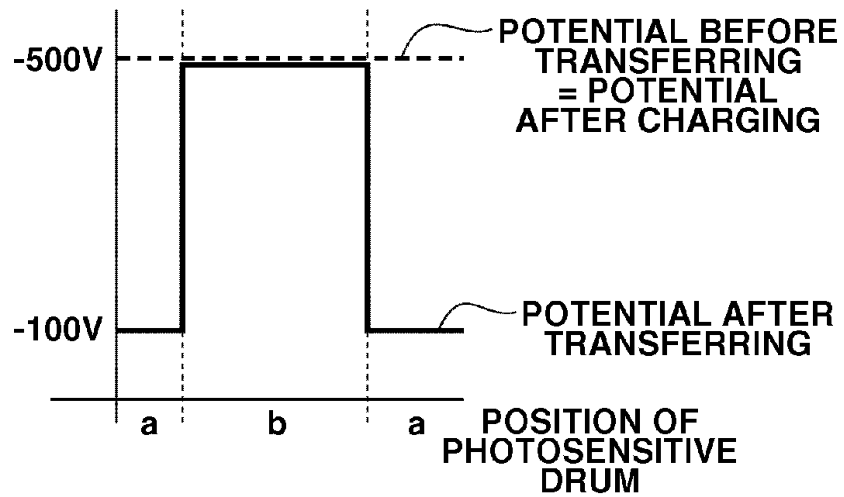
FIG.3A AFTER PASSING THROUGH TRANSFER POSITION
