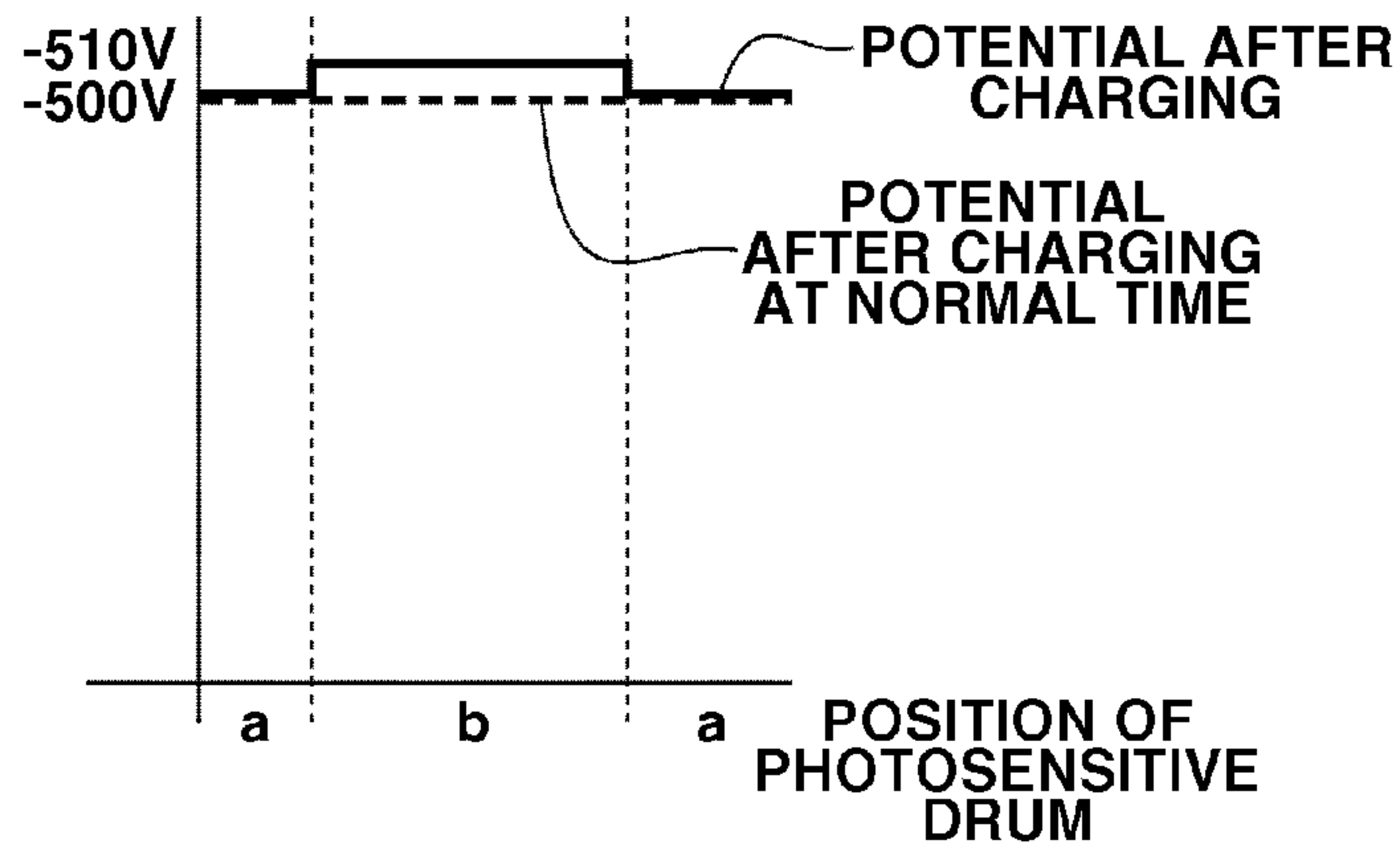
FIG.3B AFTER PASSING THROUGH CHARGING POSITION
