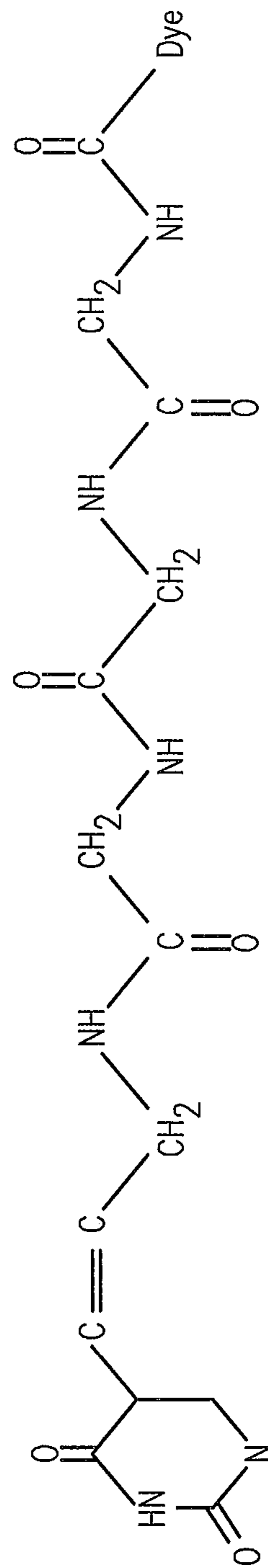
Tetraglycinylnyl linker
