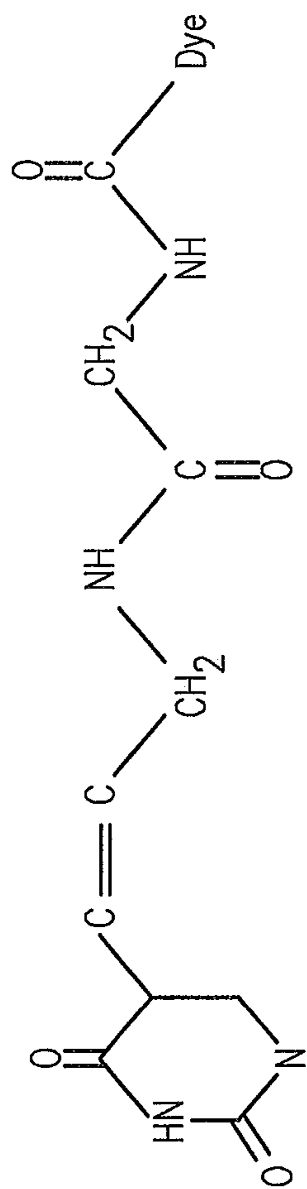
Diglycinylnyl linker
