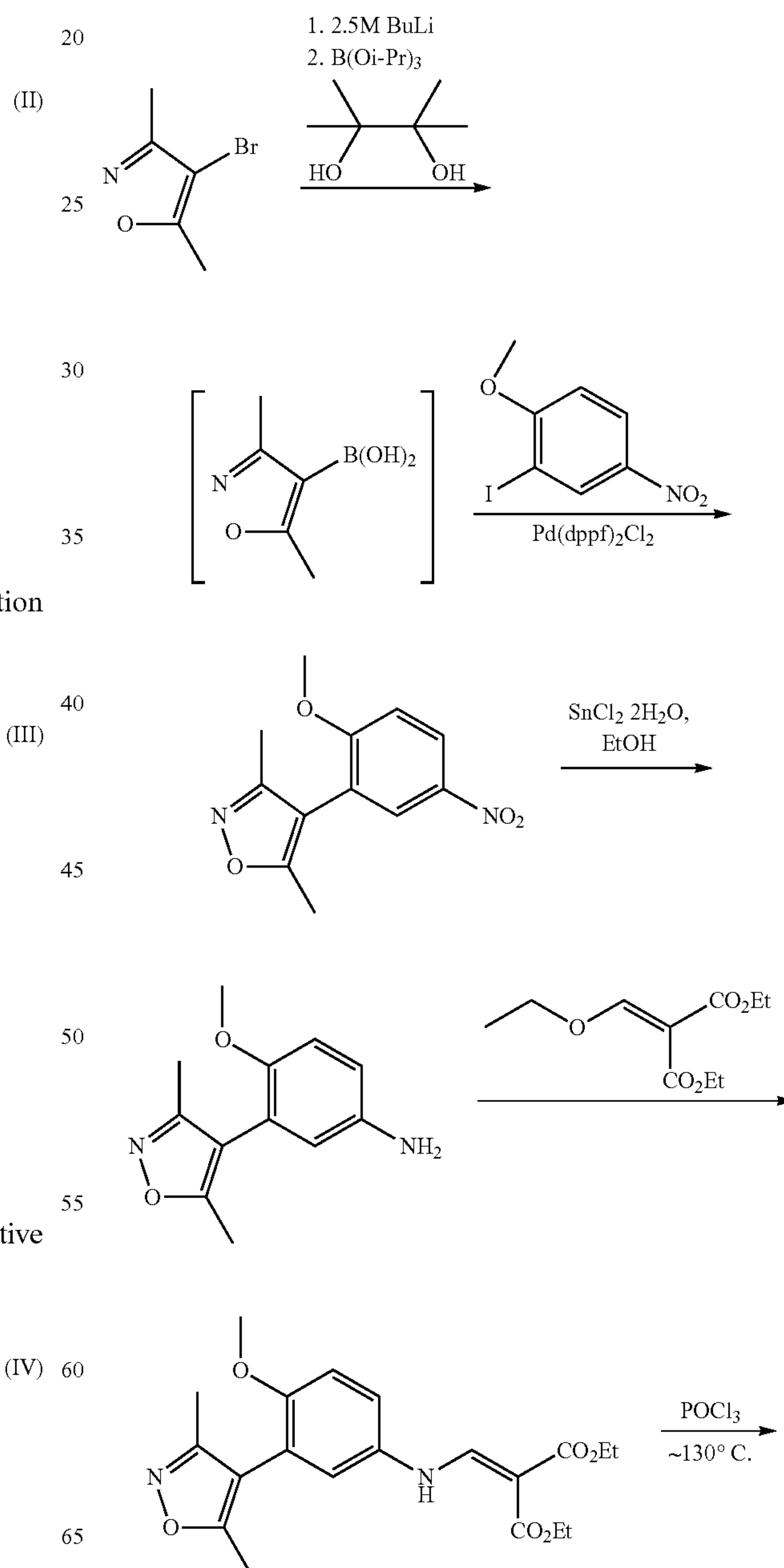
Scheme 1
